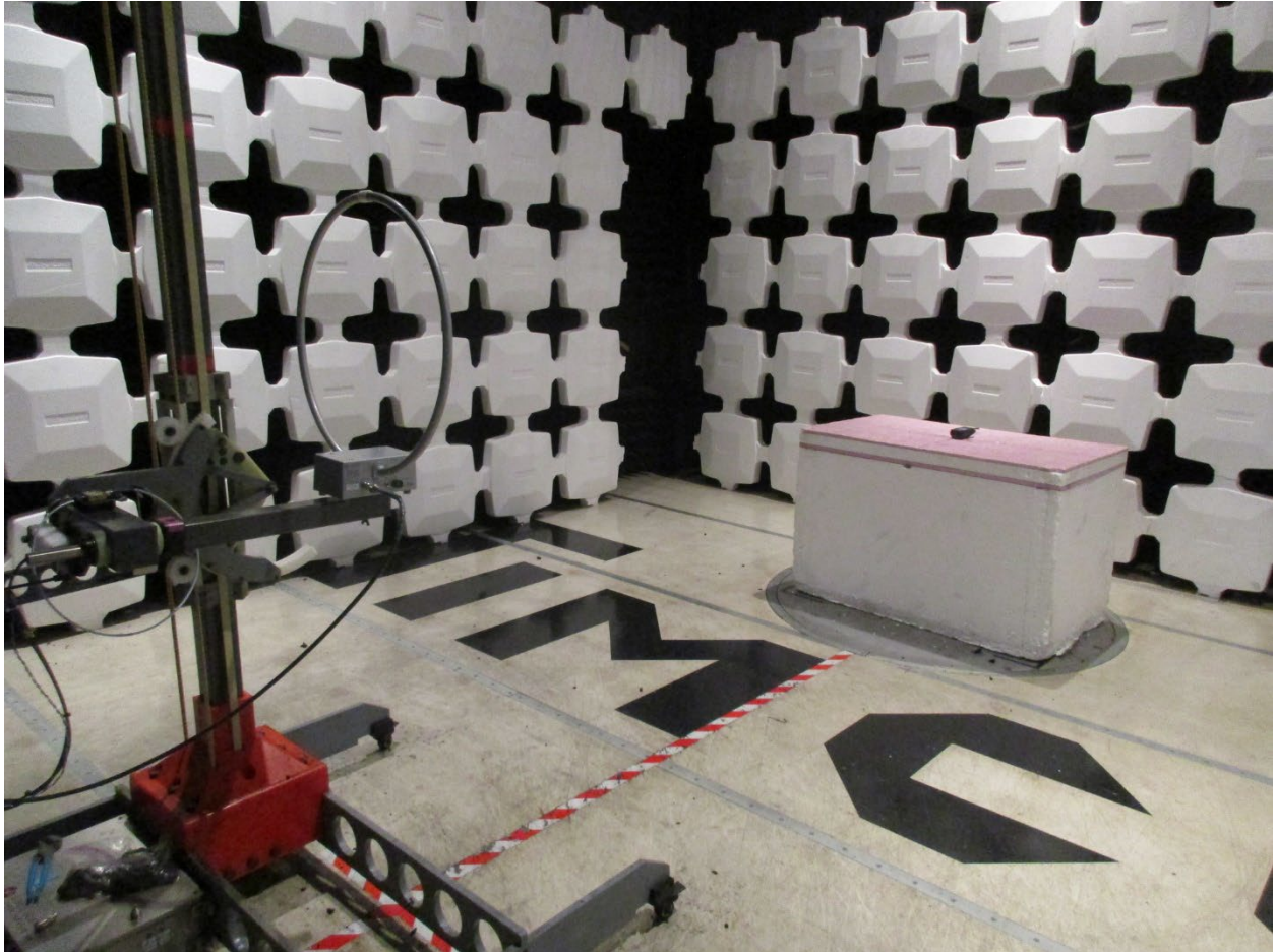
Radiated Test Setup, Below 30 MHz
