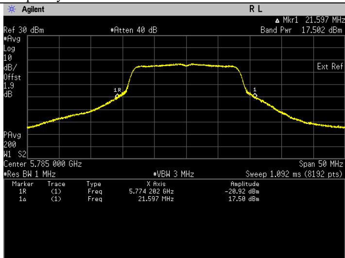
Frequency 5785 MHz.
