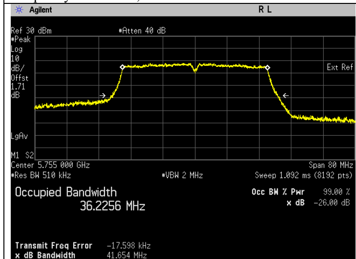
Frequency 5755 MHz
