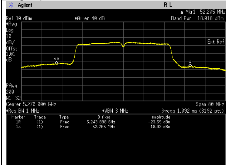
Frequency 5270 MHz
