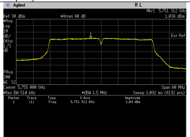
Frequency 5755 MHz
