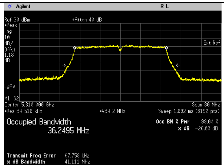
Frequency 5310 MHz
