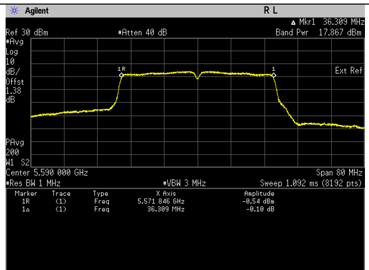
Frequency 5590 MHz
