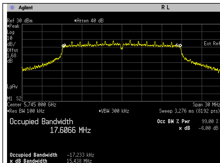
Frequency 5745 MHz
