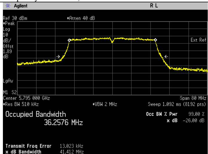
Frequency 5795 MHz
