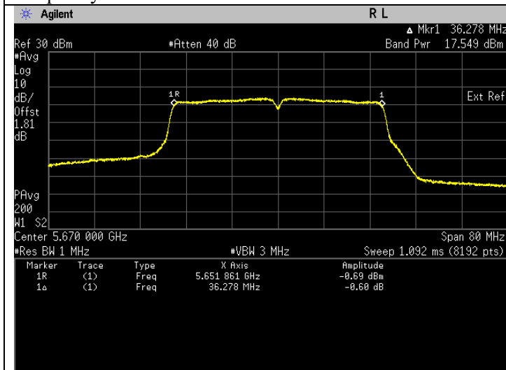
Frequency 5670 MHz
