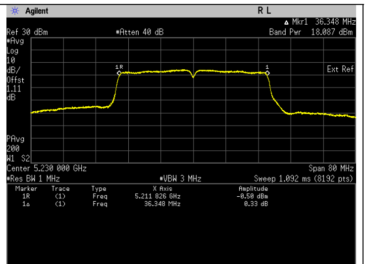
Frequency 5230 MHz
