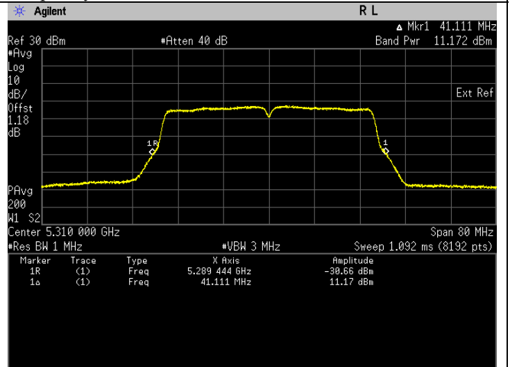
Frequency 5310 MHz
