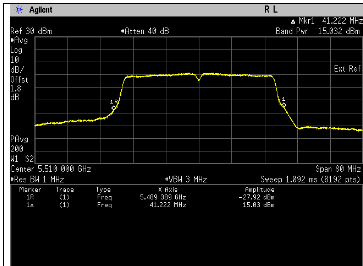
Frequency 5510 MHz
