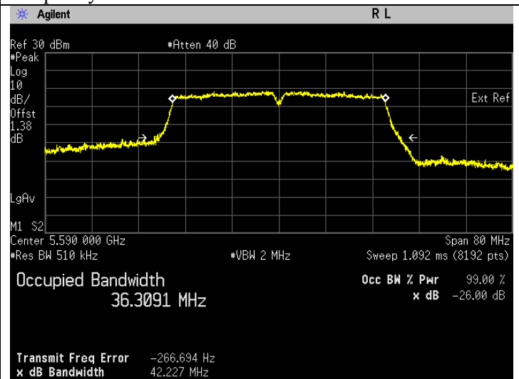
Frequency 5590 MHz
