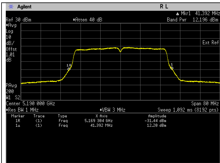
Frequency 5190 MHz
