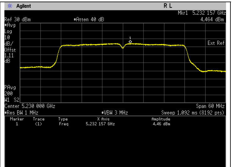
Frequency 5230 MHz
