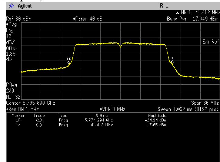
Frequency 5795 MHz
