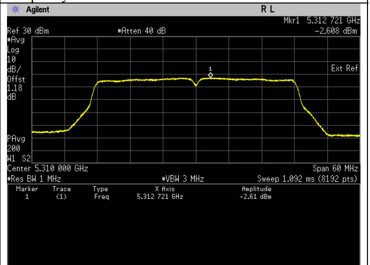
Frequency 5310 MHz
