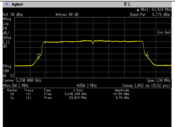
Frequency 5290 MHz
