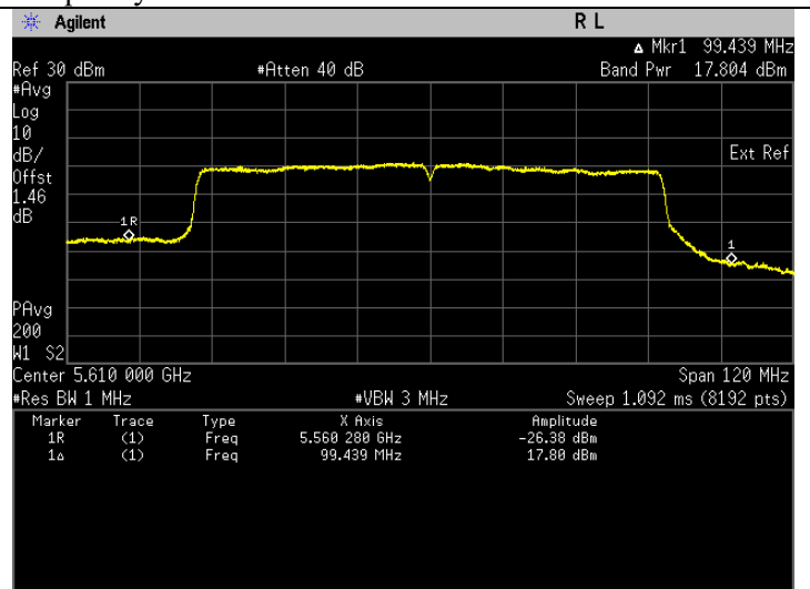
Frequency 5610 MHz
