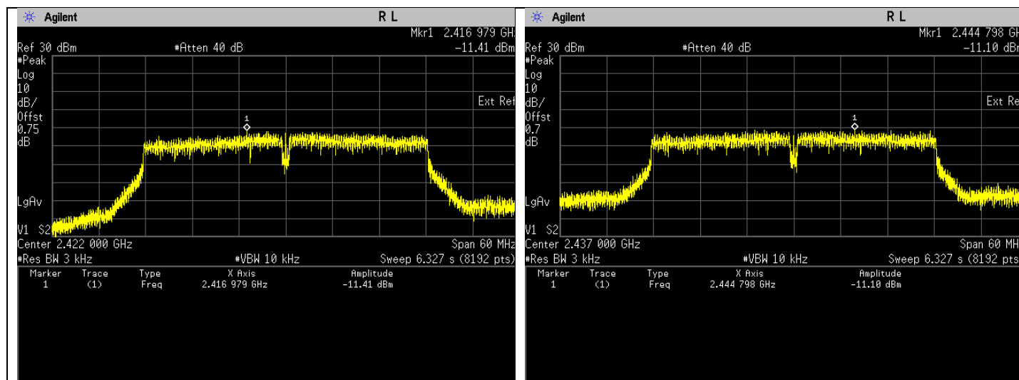
Maximum Power Spectral Density. 802.11n Frequency 2422 MHz
