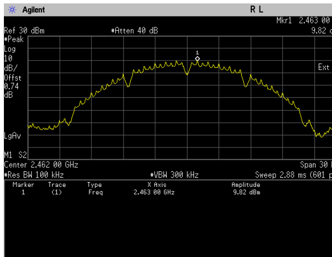
Conducted Emissions(Peak). 802.11b, Frequency 2462 MHz Reference Level
