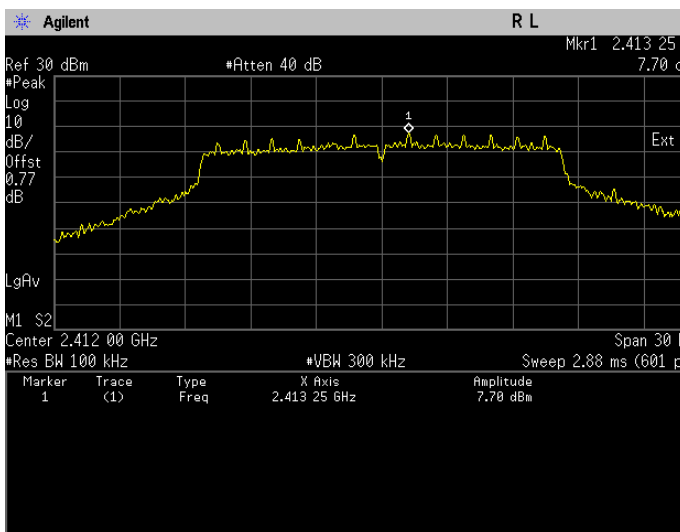
Conducted Emissions(Peak). 802.11g, Frequency 2412 MHz Reference Level
