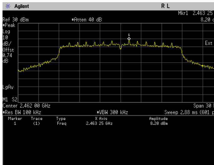
Conducted Emissions(Peak). 802.11n, Frequency 2462 MHz Reference Level
