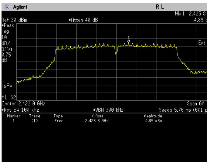
Conducted Emissions(Peak). 802.11n, Frequency 2422 MHz Reference Level
