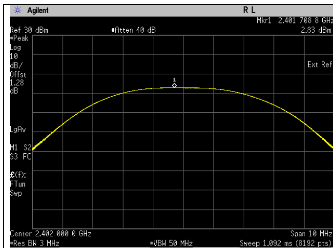
Frequency 2402 MHz
