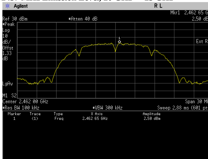
Conducted Emissions(Average). 802.11b, Frequency 2462 MHz Reference Level
