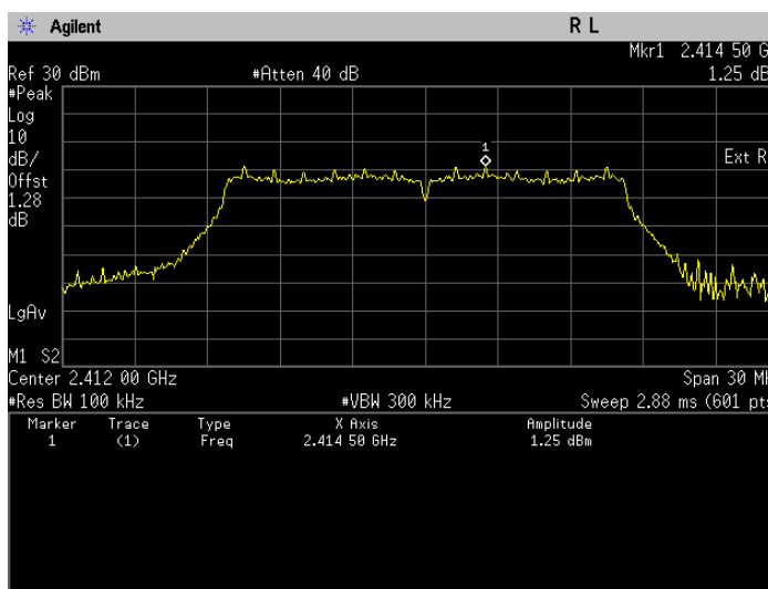
Conducted Emissions(Average). 802.11g, Frequency 2412 MHz Reference Level
