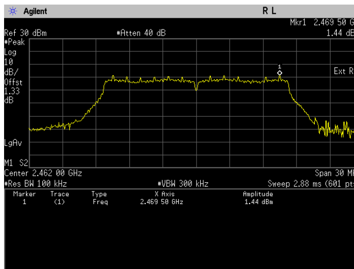
Conducted Emissions(Average). 802.11g, Frequency 2462 MHz Reference Level
