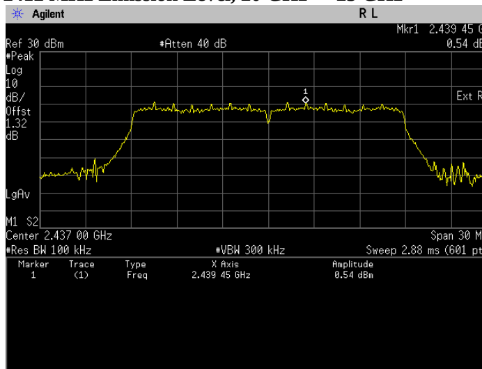
Conducted Emissions(Average). 802.11n, Frequency 2437 MHz Reference Level
