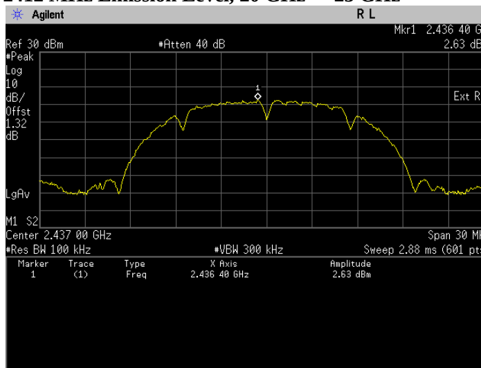
Conducted Emissions(Average). 802.11b, Frequency 2437 MHz Reference Level
