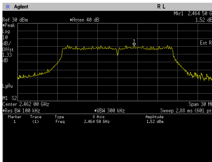
Conducted Emissions(Average). 802.11n, Frequency 2462 MHz Reference Level
