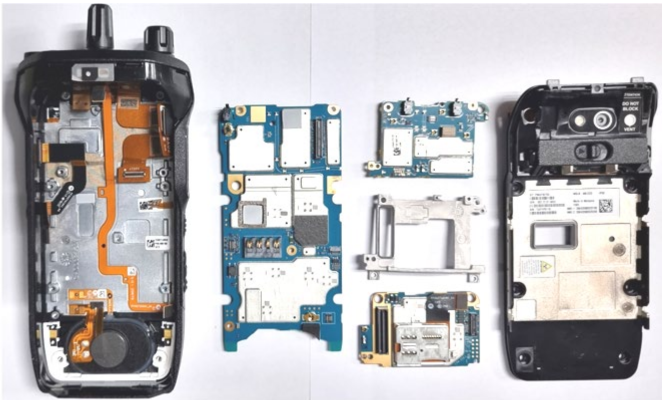
Exhibit 9N: Chassis and housing (Back Side)
