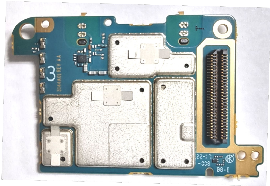
Exhibit 9B: LTE RF board with Shields (Top)
