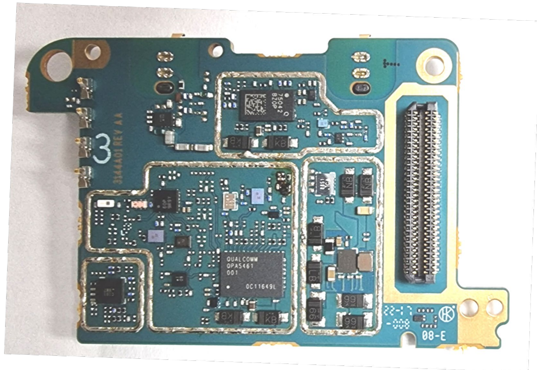
Exhibit 9E: LTE RF board without Shields (Top)
