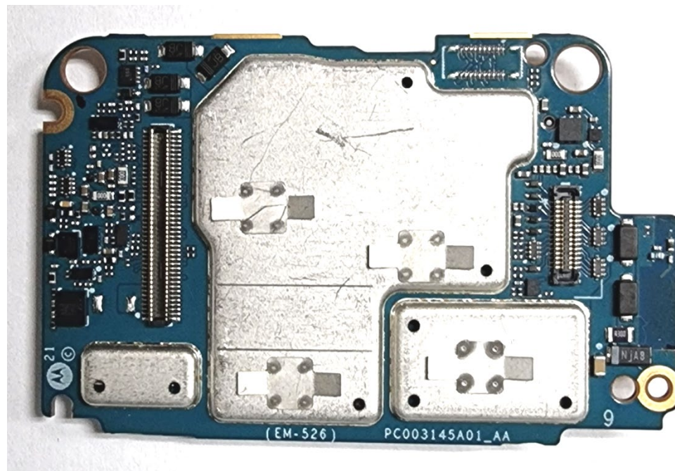
Exhibit 9C: AP board with Shields (Top)
