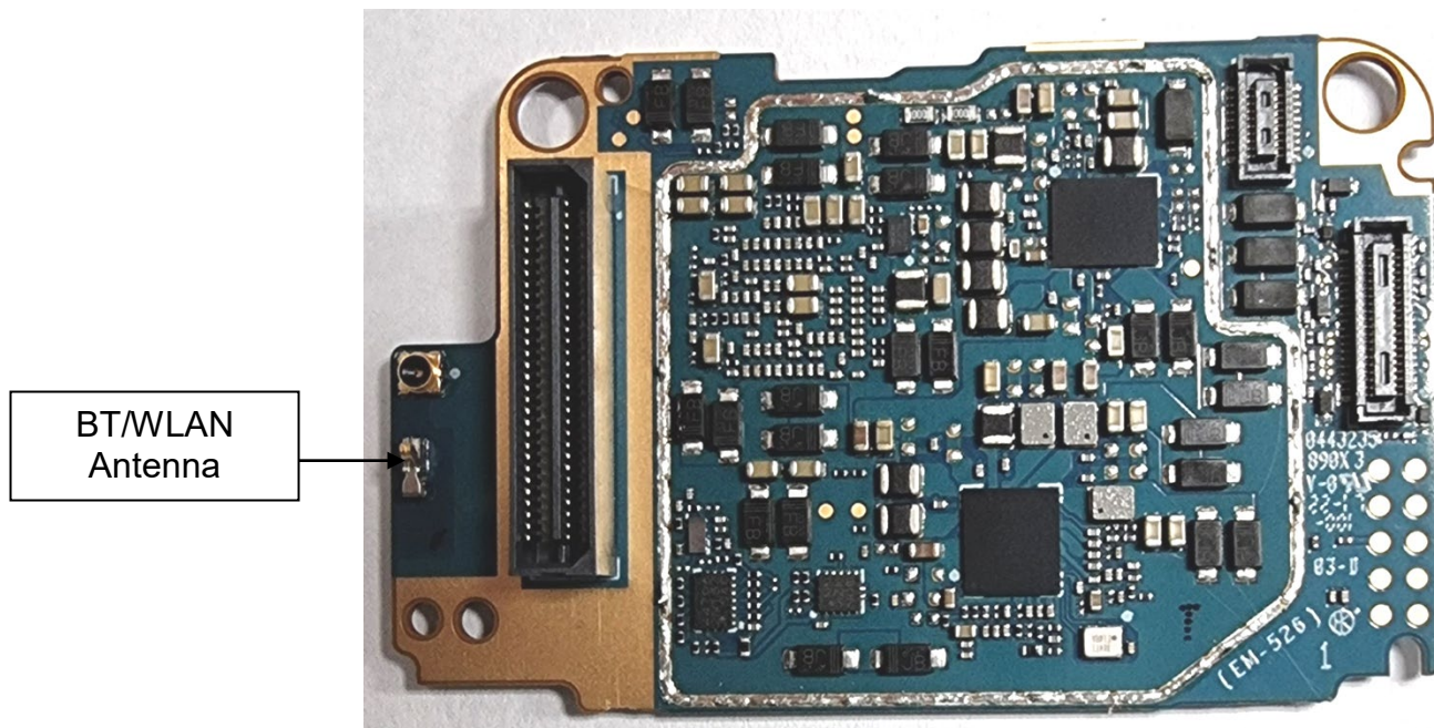
Exhibit 9L: AP board without Shields (Bottom)
