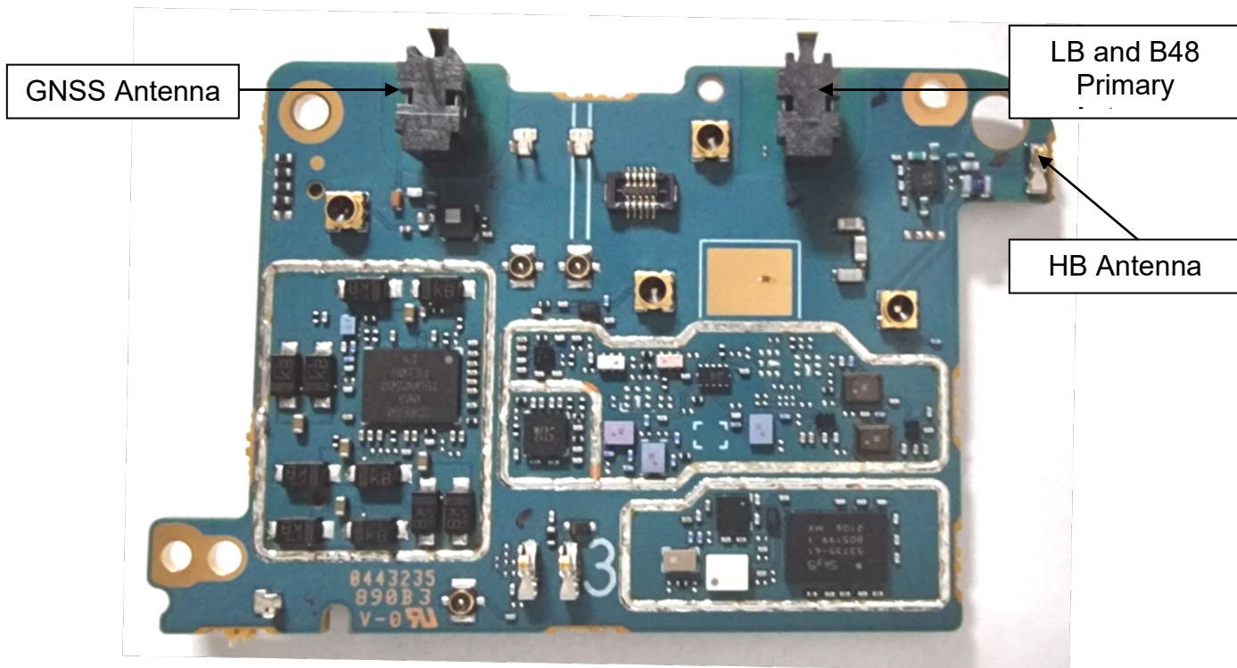
Exhibit 9K: LTE RF board without Shields (Bottom)
