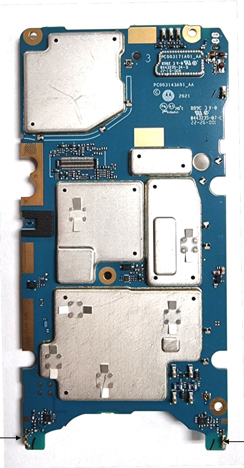
Exhibit 9A: LMR RF board with Shields (Top)
