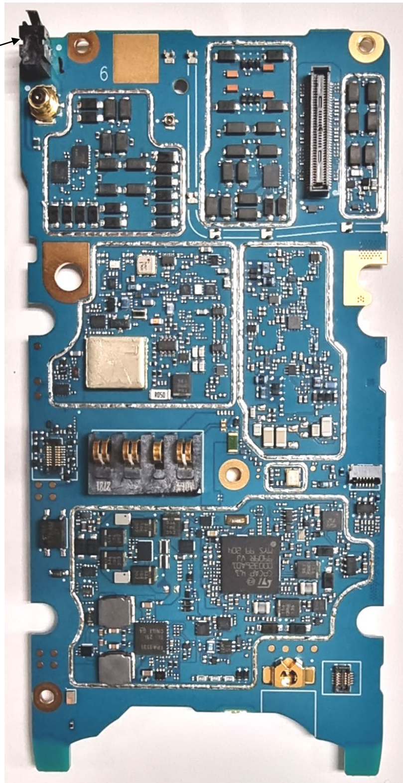
Exhibit 9J: LMR RF board without Shields (Bottom)
