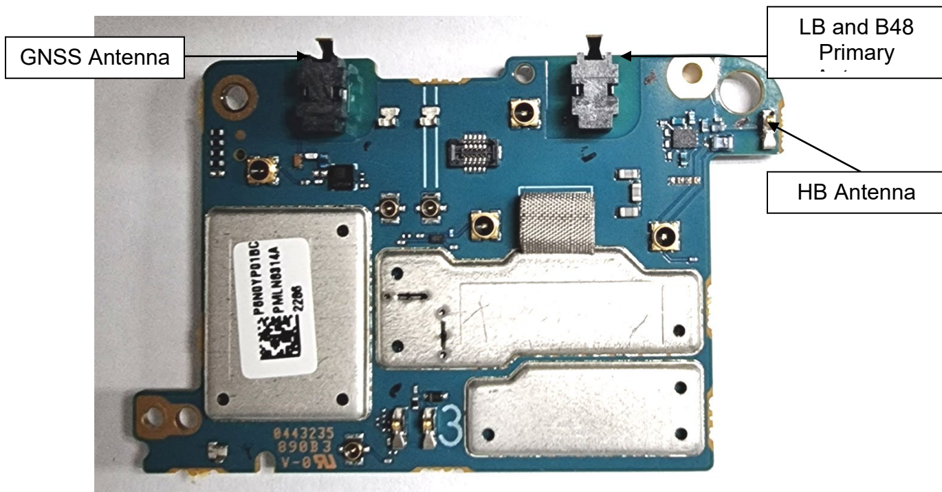
Exhibit 9H: LTE RF board with Shields (Bottom)
