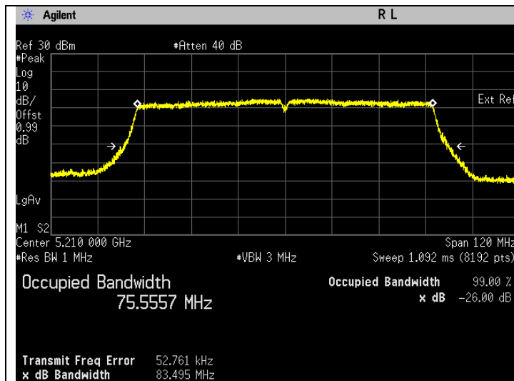
Frequency 5210 MHz
