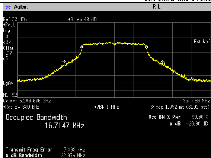
Frequency 5260 MHz
