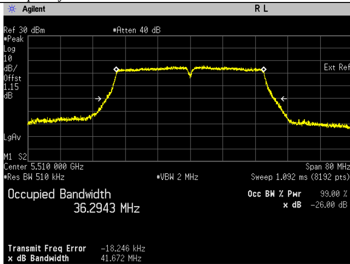
Frequency 5510 MHz
