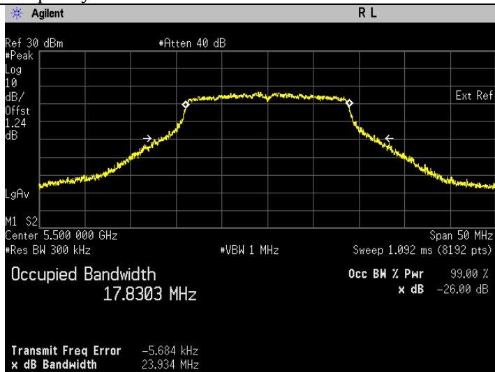
Frequency 5500 MHz
