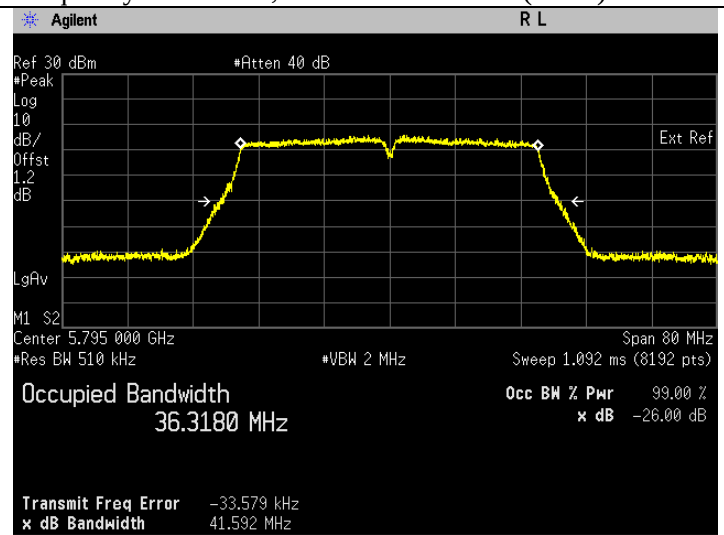
Frequency 5795 MHz
