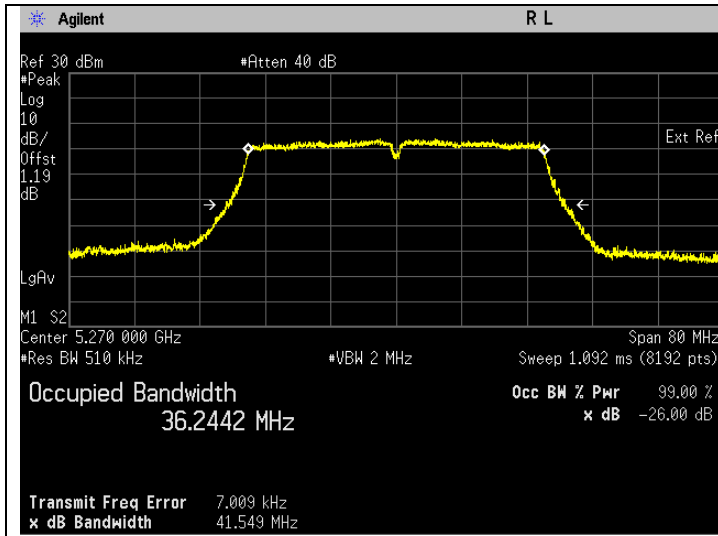
Frequency 5270 MHz
