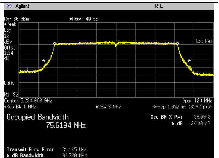
Frequency 5290 MHz
