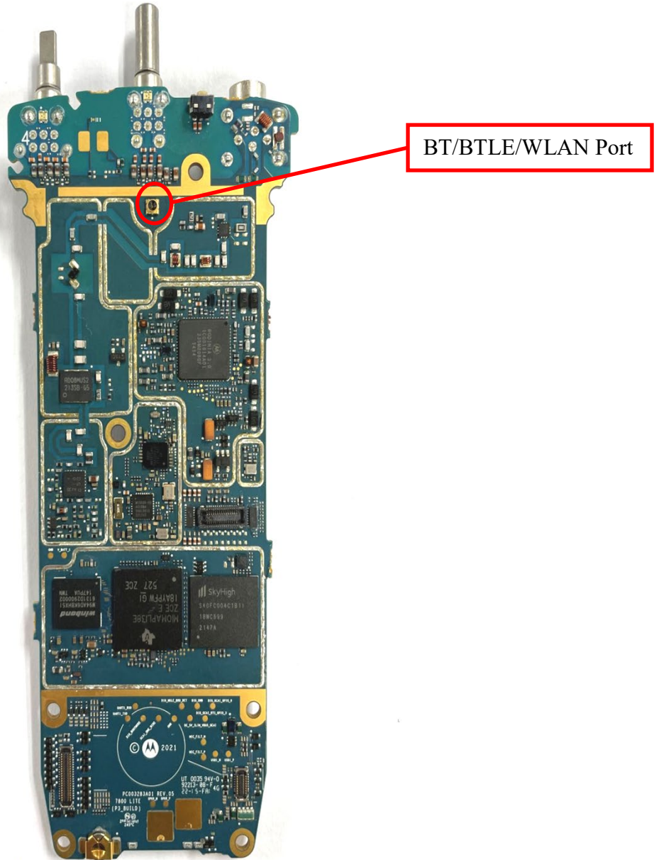
Main board without Shields (Top) (APX N30)
