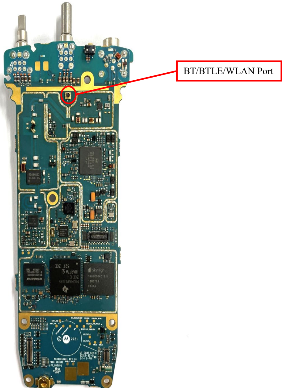
Main board without Shields (Top) (APX N50)
