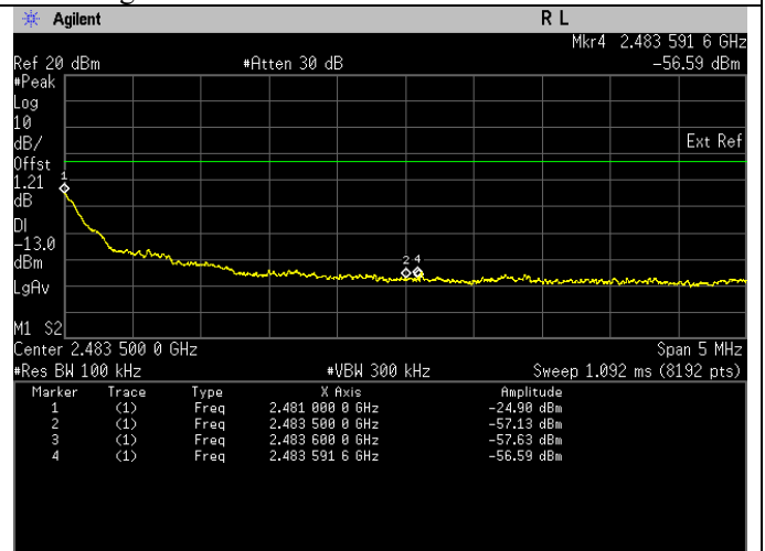
Band Edge(Peak). Bluetooth LE Frequency 2480 MHz Band Edge
