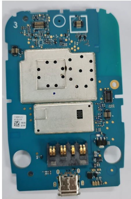
PCB with Shields (Bottom)
