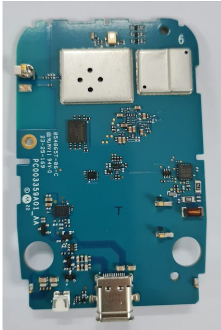
PCB with Shields (Top)
