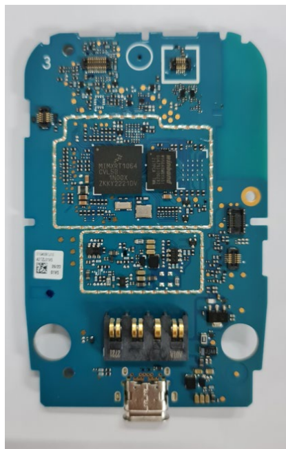
PCB without Shields (Bottom)
