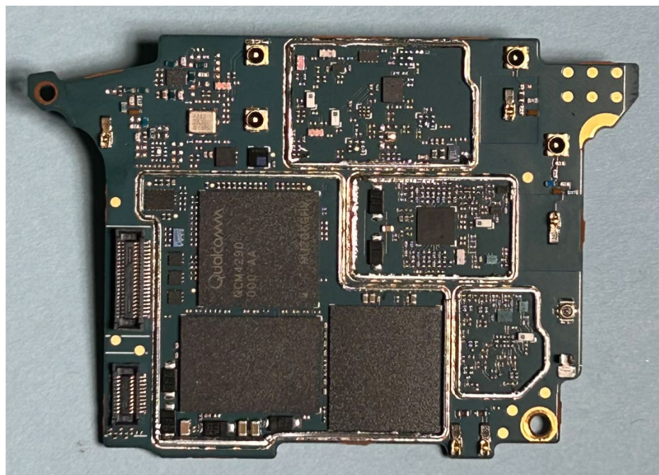
Exhibit 9H – AP board without Shields (Top)
