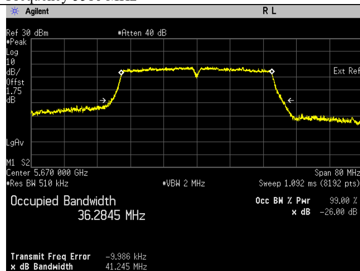
Frequency 5670 MHz
