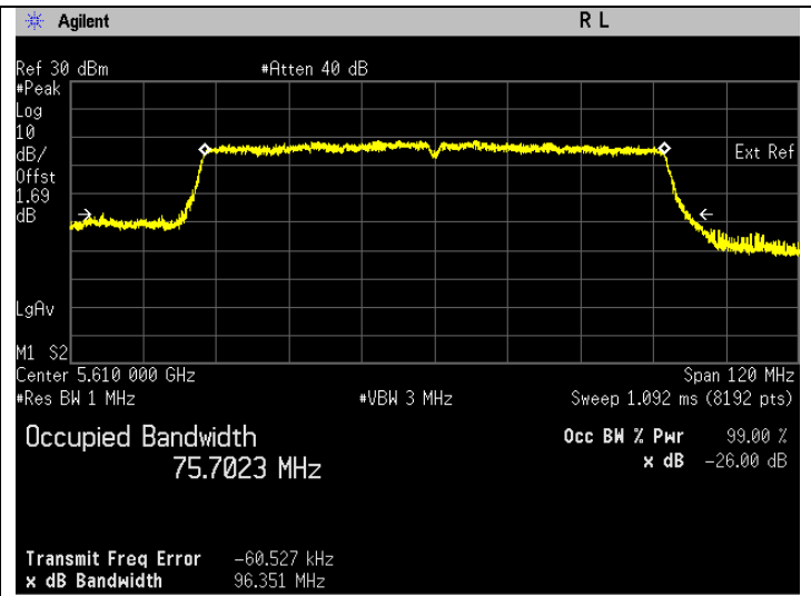
Frequency 5610 MHz
