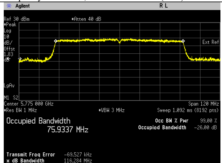
Frequency 5775 MHz
