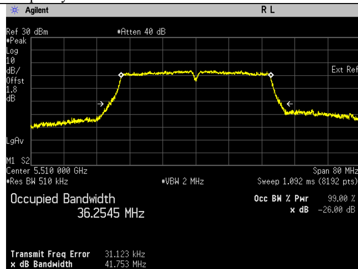
Frequency 5510 MHz
