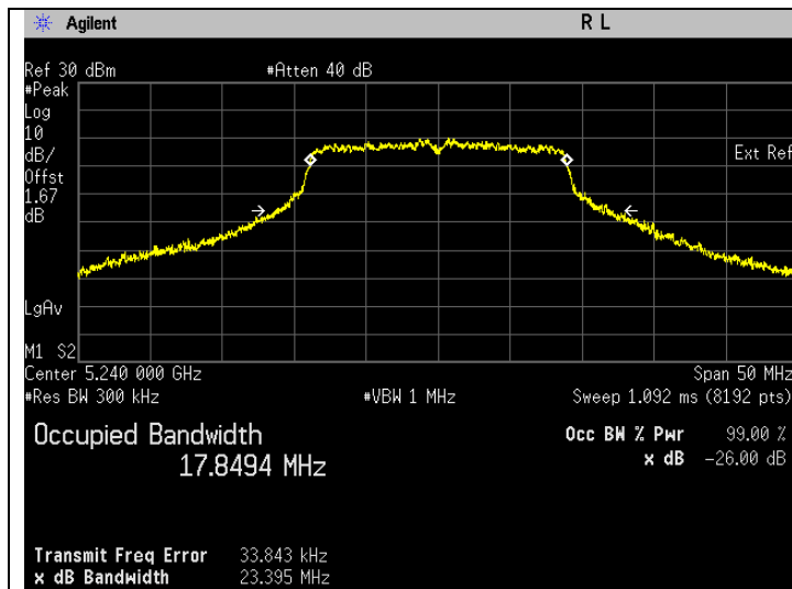
Frequency 5240 MHz
