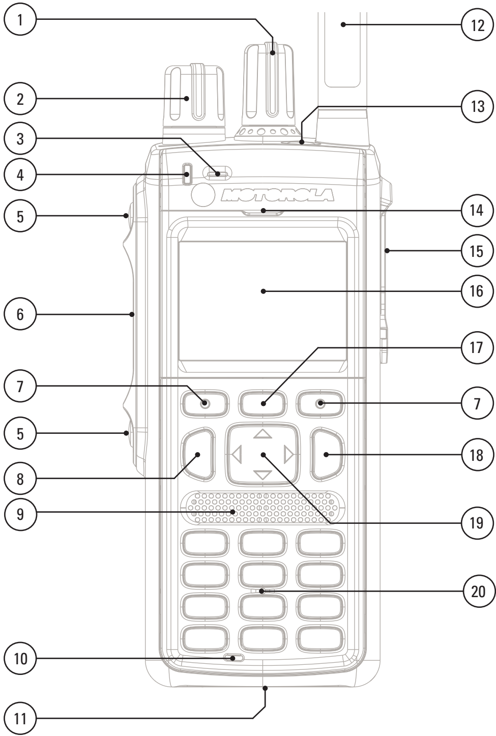
Figure 2: MTP3x50 Series Controls and Indicators
