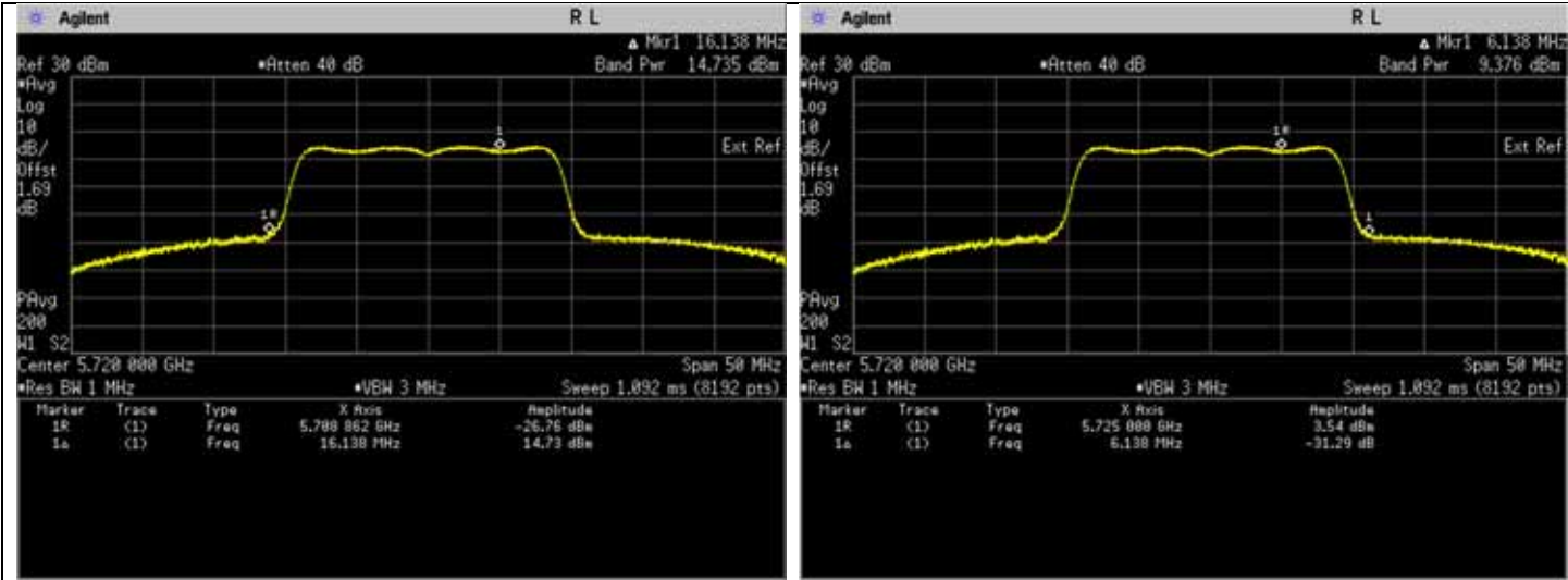
Frequency 5720 MHz, U-NII-2C. *Note: The band power is captured before the 5725 MHz. Frequency 5720 MHz, U-NII-3. *Note: The band power is captured after the 5725 MHz.
