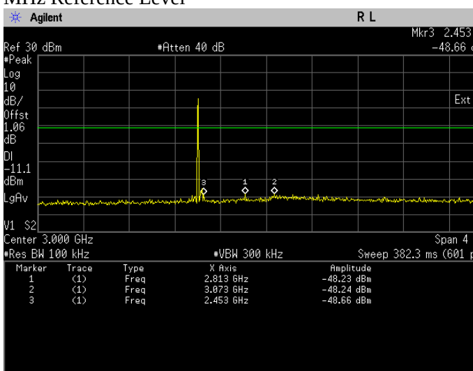
Conducted Emissions. Bluetooth LE, Frequency 2404 MHz Emission Level, 1 GHz -> 5 GHz
