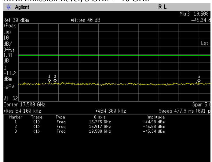
Conducted Emissions. Bluetooth LE, Frequency 2478 MHz Emission Level, 15 GHz -> 20 GHz
