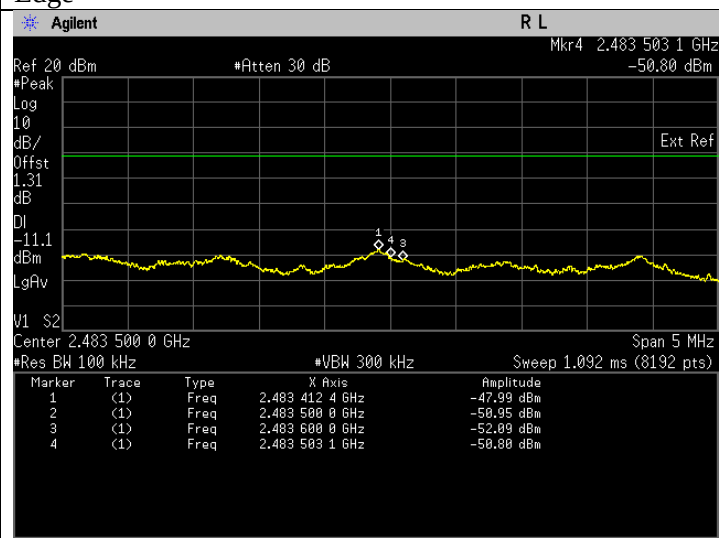
Band Edge. Bluetooth LE Frequency 2478 MHz Band Edge
