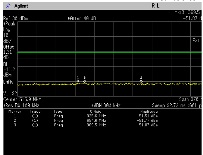
Conducted Emissions. Bluetooth LE, Frequency 2478 MHz Emission Level, 30 MHz -> 1 GHz
