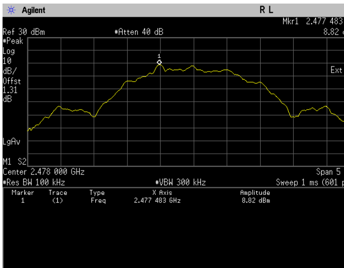
Conducted Emissions. Bluetooth LE, Frequency 2478 MHz Reference Level
