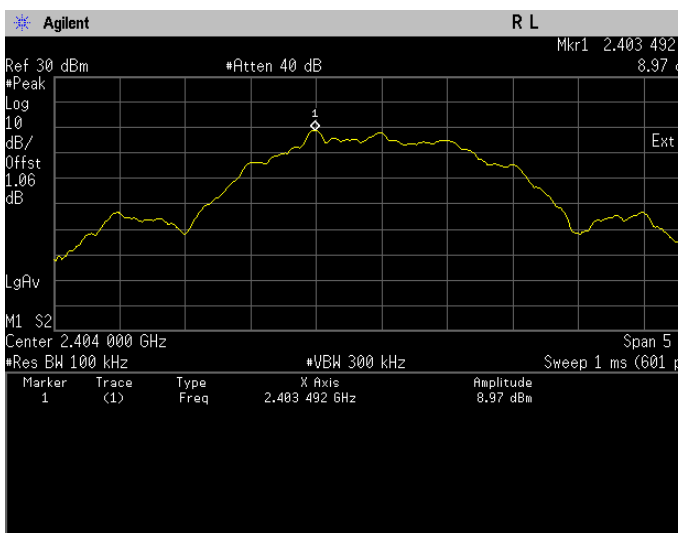
Conducted Emissions. Bluetooth LE, Frequency 2404 MHz Reference Level
