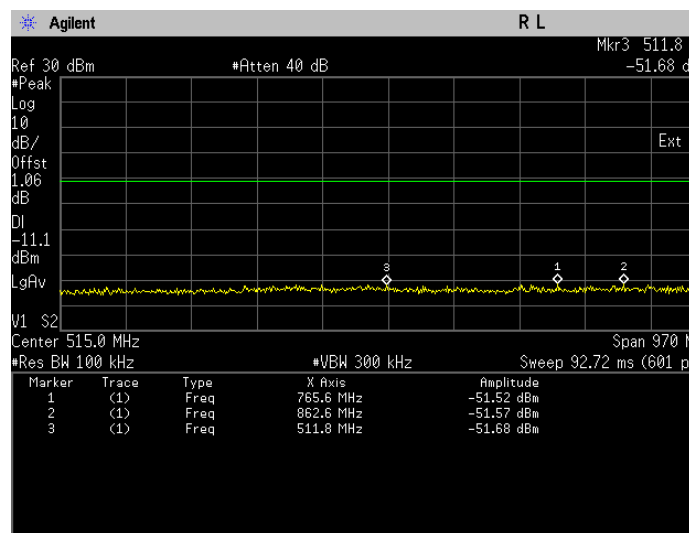
Conducted Emissions. Bluetooth LE, Frequency 2404 MHz Emission Level, 30 MHz -> 1 GHz
