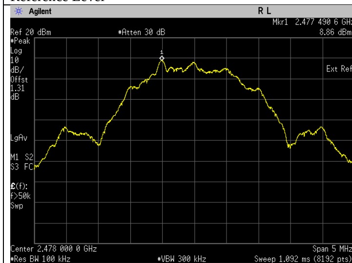
Band Edge. Bluetooth LE Frequency 2478 MHz Reference Level
