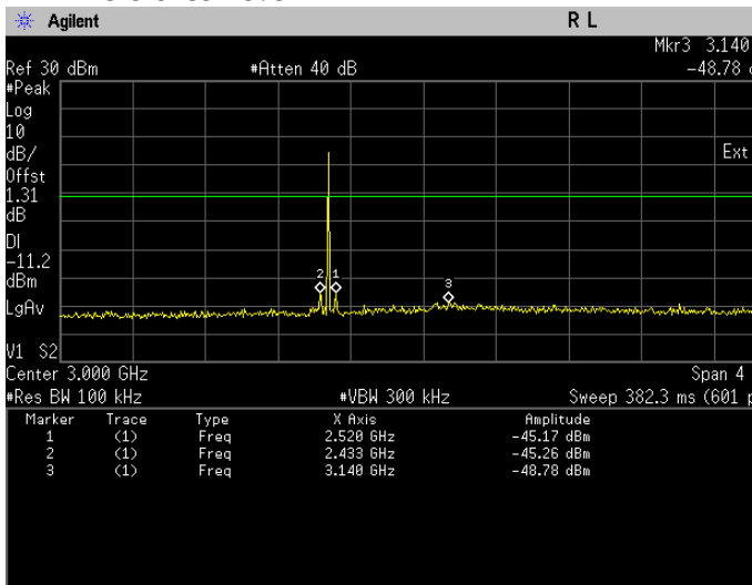
Conducted Emissions. Bluetooth LE, Frequency 2478 MHz Emission Level, 1 GHz -> 5 GHz
