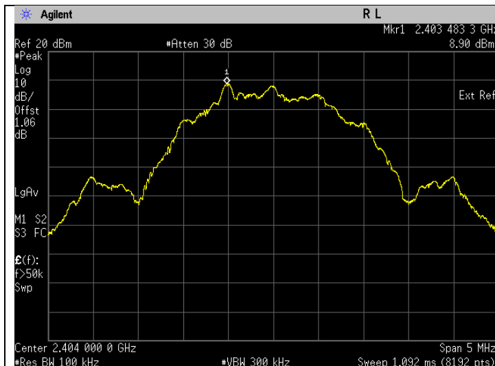
Band Edge. Bluetooth LE Frequency 2404 MHz Reference Level
