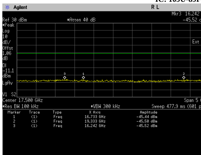
Conducted Emissions. Bluetooth LE, Frequency 2404 MHz Emission Level, 15 GHz -> 20 GHz
