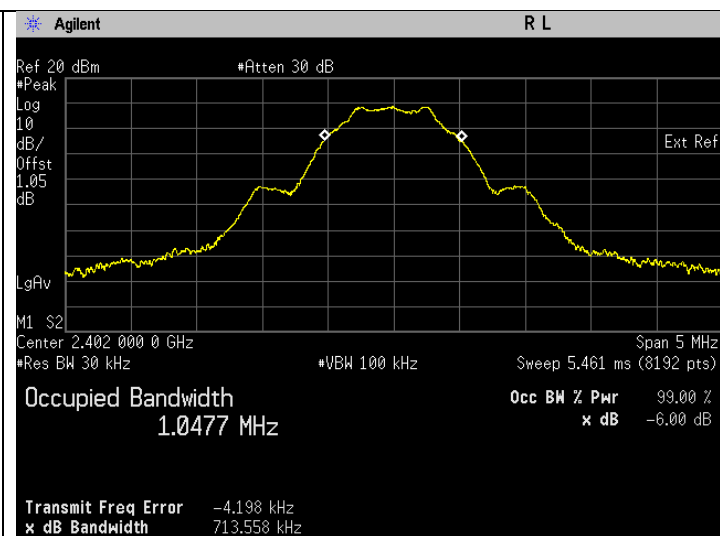
99% Bandwidth. Bluetooth LE Frequency 2402 MHz
