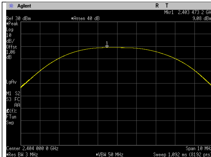
Frequency 2404 MHz
