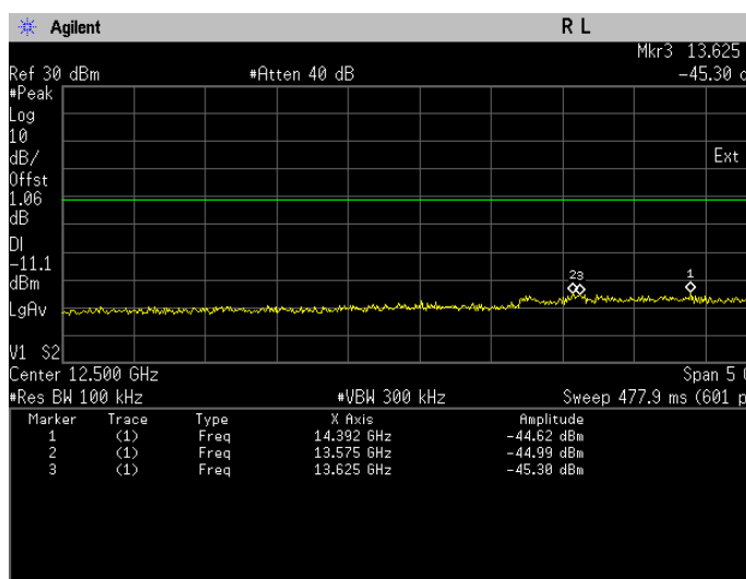
Conducted Emissions. Bluetooth LE, Frequency 2404 Emission Level, 10 GHz -> 15 GHz
