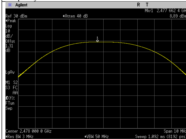
Frequency 2478 MHz
