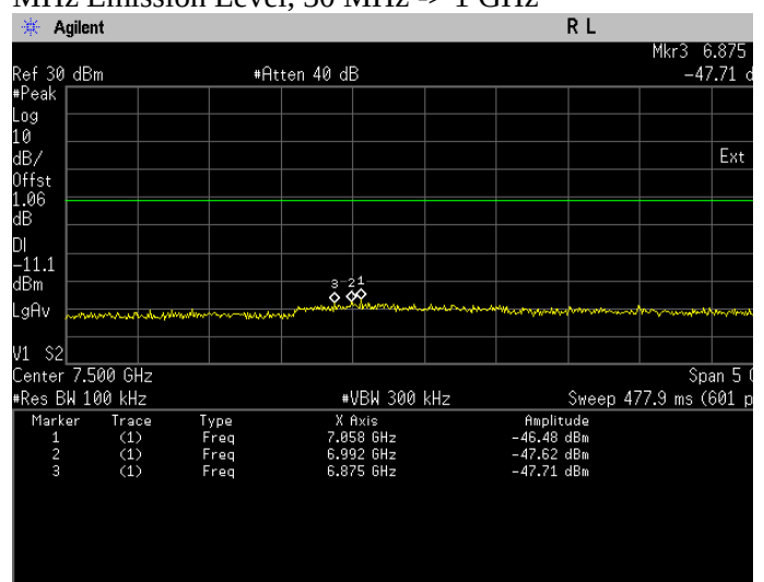
Conducted Emissions. Bluetooth LE, Frequency 2404 MHz Emission Level, 5 GHz -> 10 GHz
