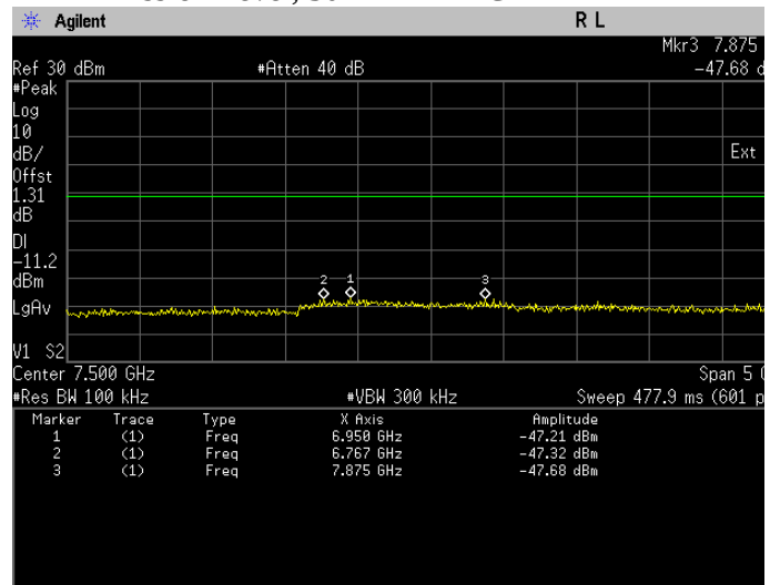
Conducted Emissions. Bluetooth LE, Frequency 2478 MHz Emission Level, 5 GHz -> 10 GHz
