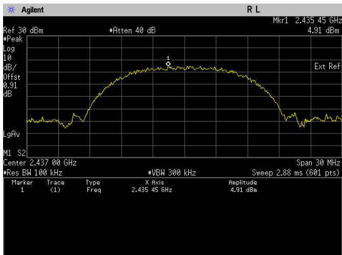
Conducted Emissions. 802.11b, Frequency 2437 MHz Reference Level
