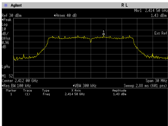
Conducted Emissions. 802.11g, Frequency 2412 MHz Reference Level
