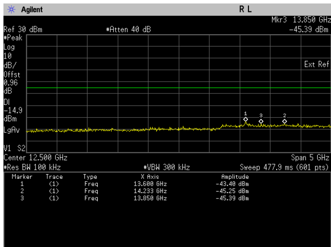
Conducted Emissions. 802.11b, Frequency 2412 Emission Level, 10 GHz -> 15 GHz
