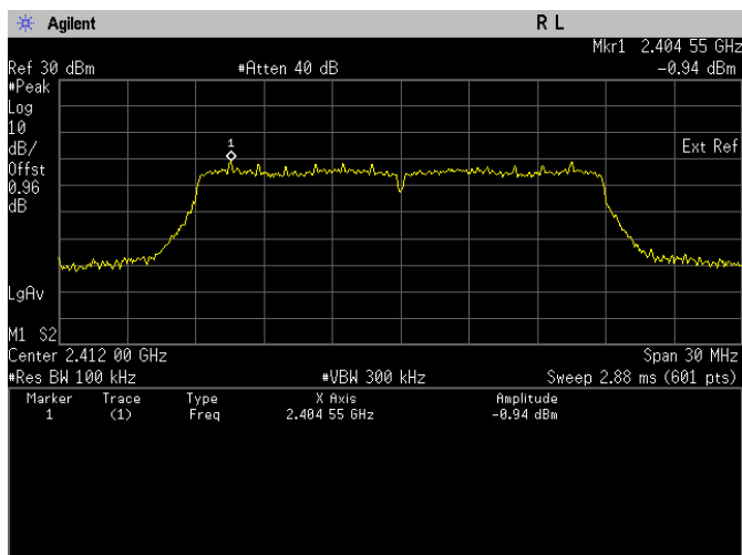
Conducted Emissions. 802.11n, Frequency 2412 MHz Reference Level
