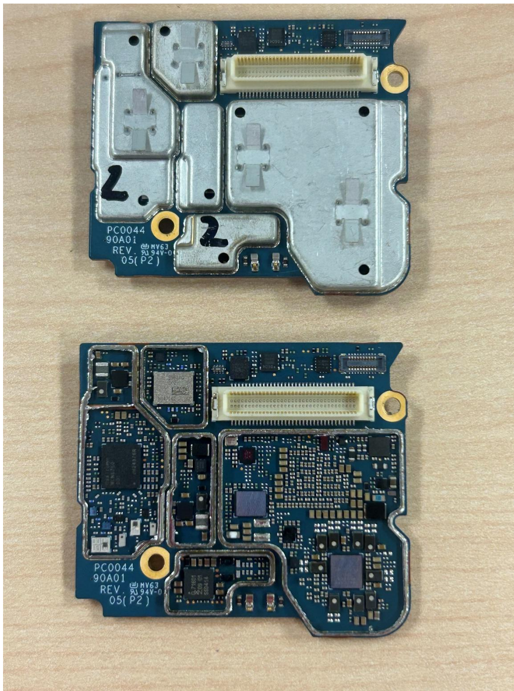
AP board with & without Shields (Bottom), APX NEXT Model
