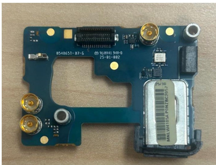
IPCB board (Bottom), APX NEXT Model
