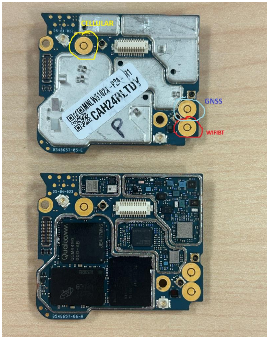
AP board with & without Shields (Top), APX NEXT Model
