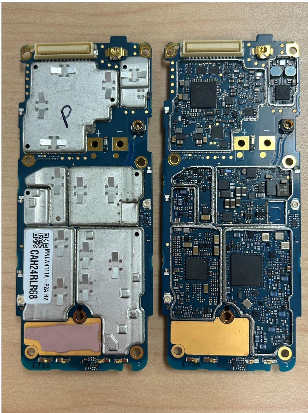
Main board with & without Shields (Bottom), APX NEXT Model
