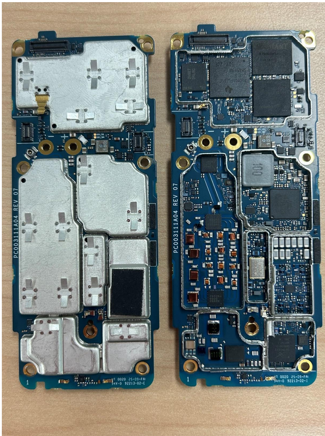
Main board with & without Shields (Top), APX NEXT Model
