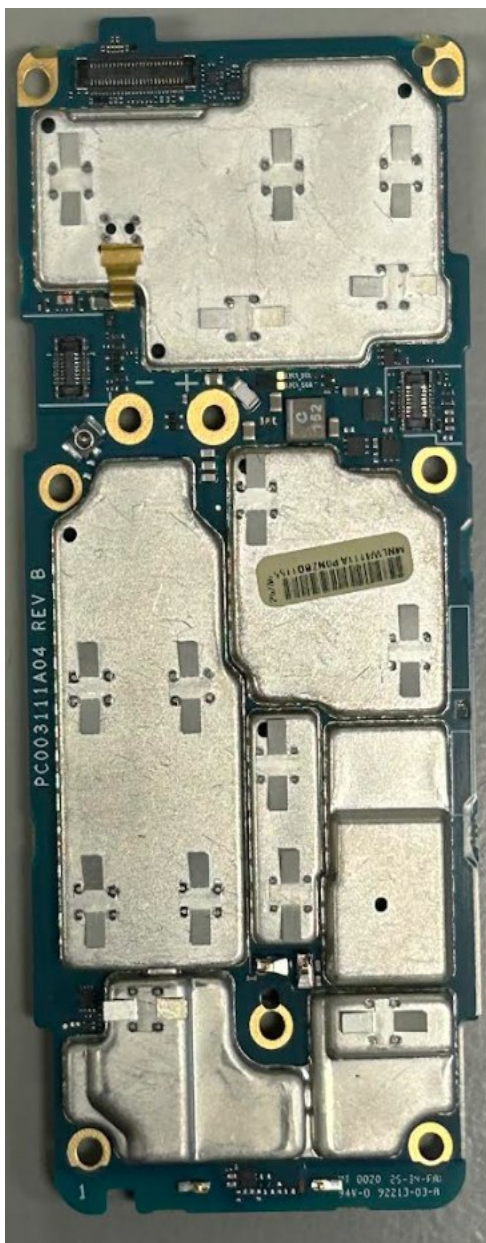
H55TGT9PW8BN / NUW4100A (APX NEXT XE) in Green
