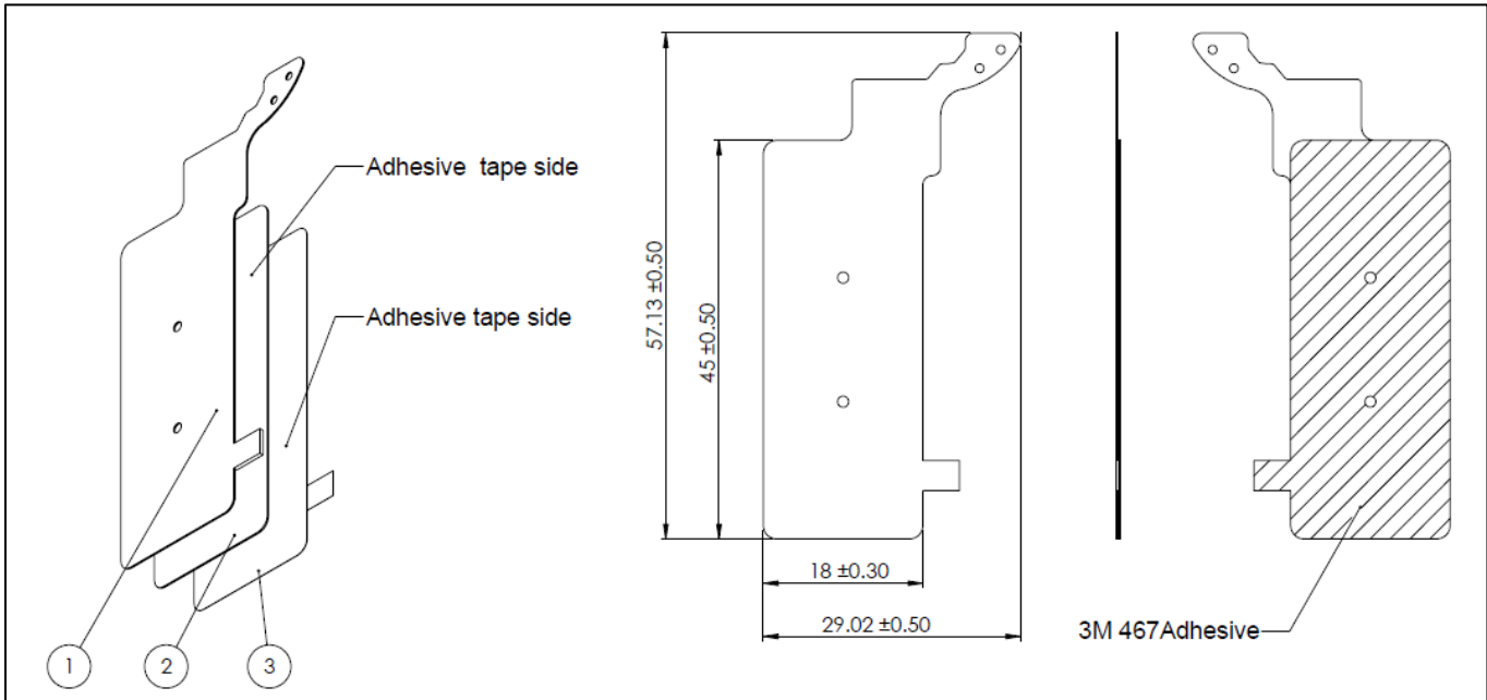
Figure 2: NFC Antenna Dimension
