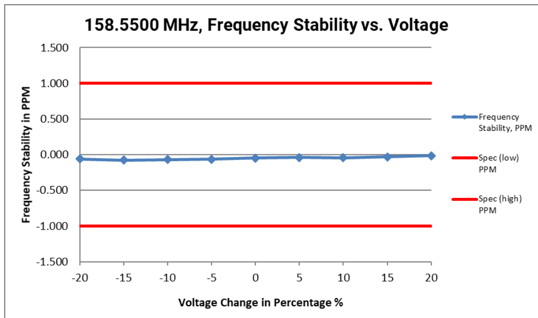
(i) Frequency Stability VS Voltage
