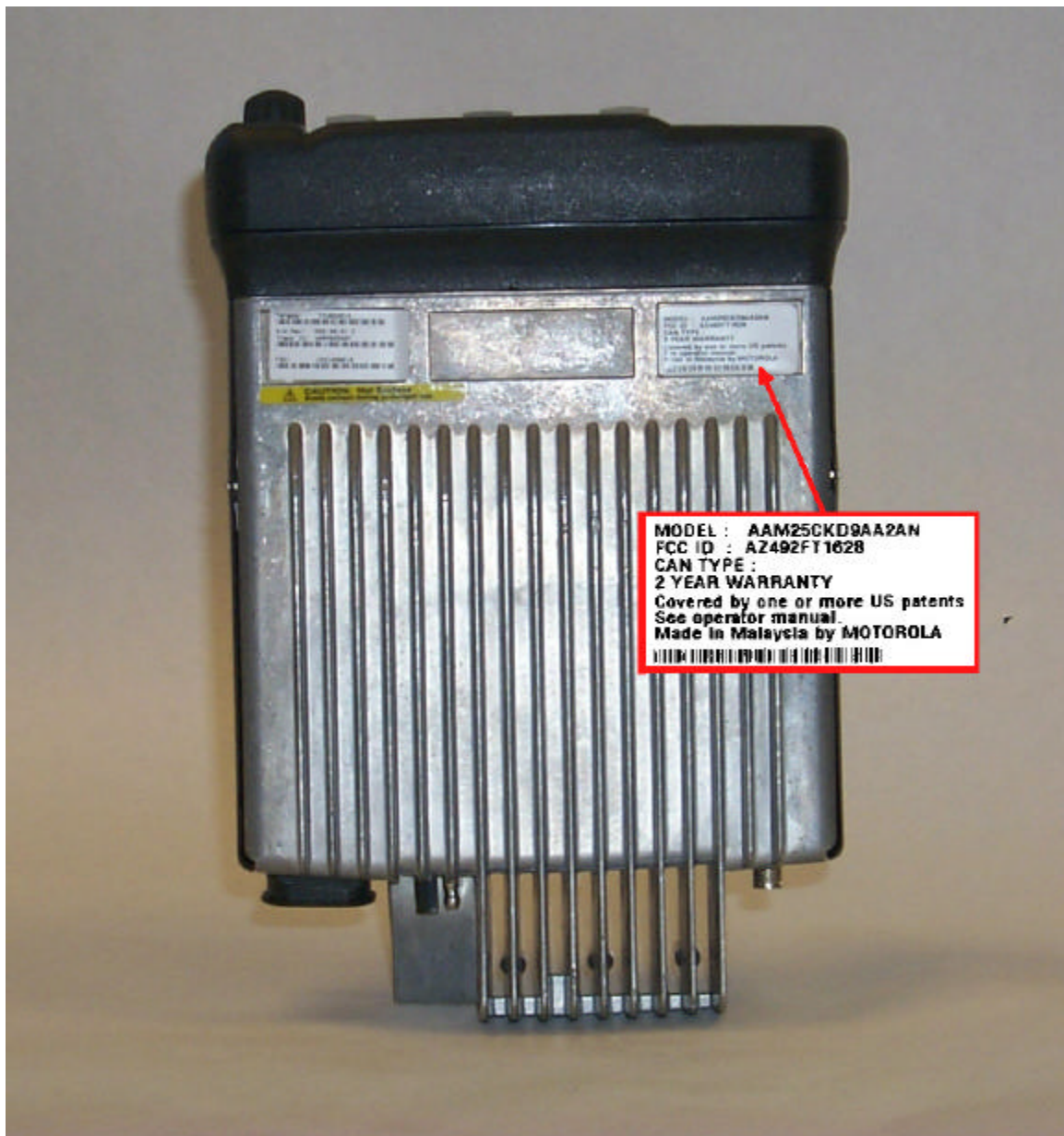
BOTTOM VIEW, SHOWING FCC ID LABEL
