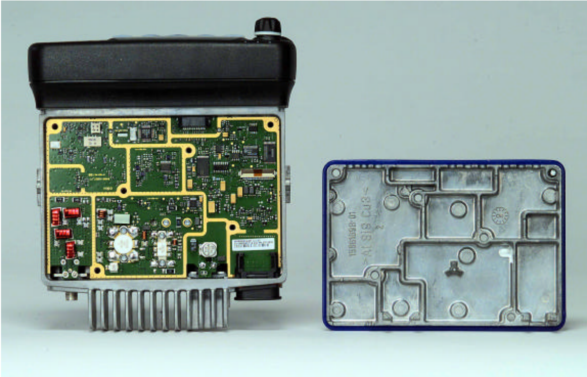
TOP VIEW, WITH METAL SHIELD COVER REMOVED (TOP SIDE OF CIRCUIT BOARD VISIBLE)
