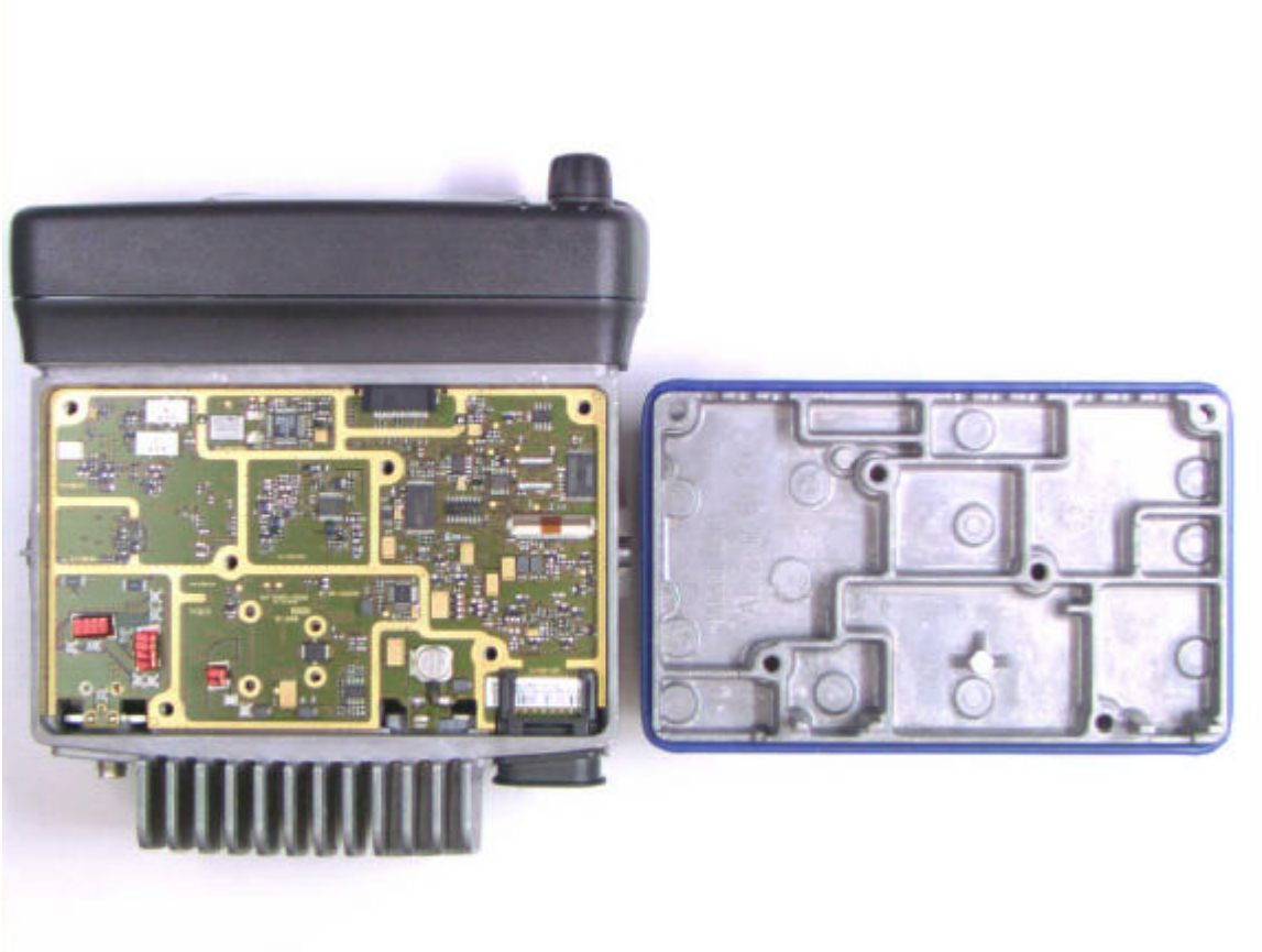
TOP VIEW, WITH METAL SHIELD COVER REMOVED (TOP SIDE OF CIRCUIT BOARD VISIBLE)
