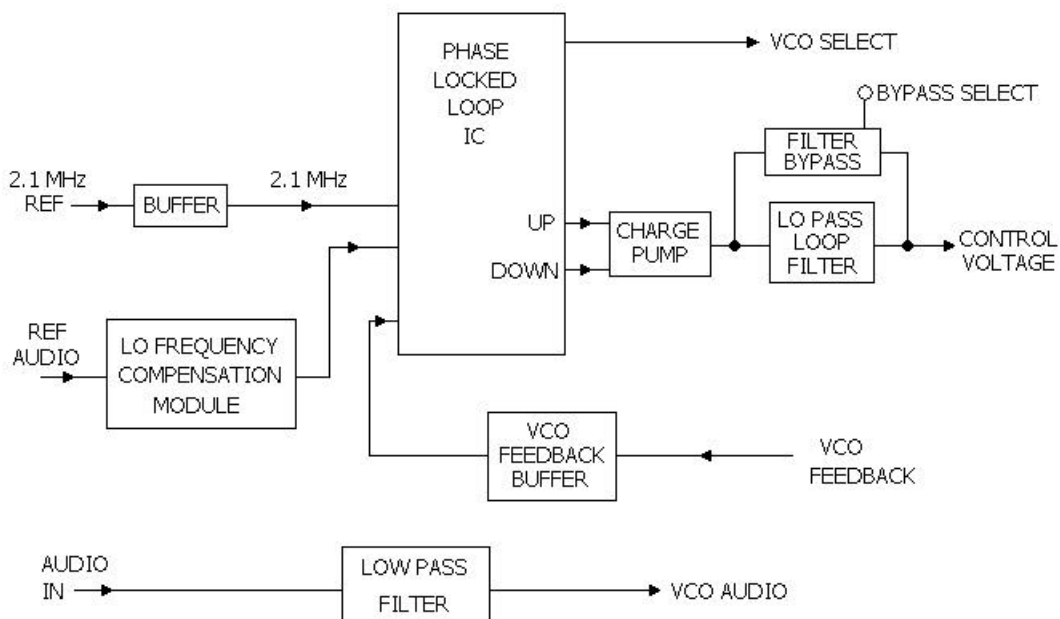
Figure 2: Phase Locked Loop Circuit
