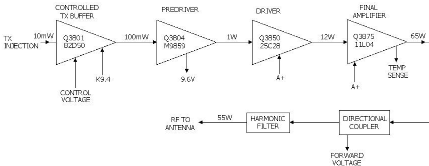
Figure 7: Power Amplifier Circuitry
