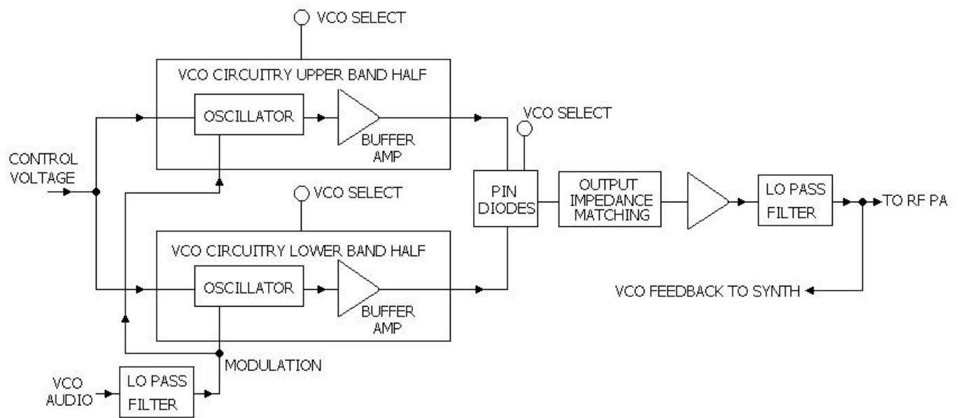
Figure 3: VCO Circuitry
