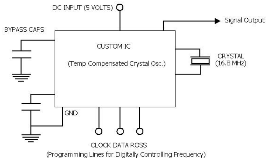
Figure 4: Reference Oscillator
