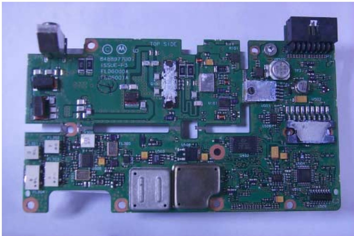
Figure 9-3: Top Side of PCB with shields.
