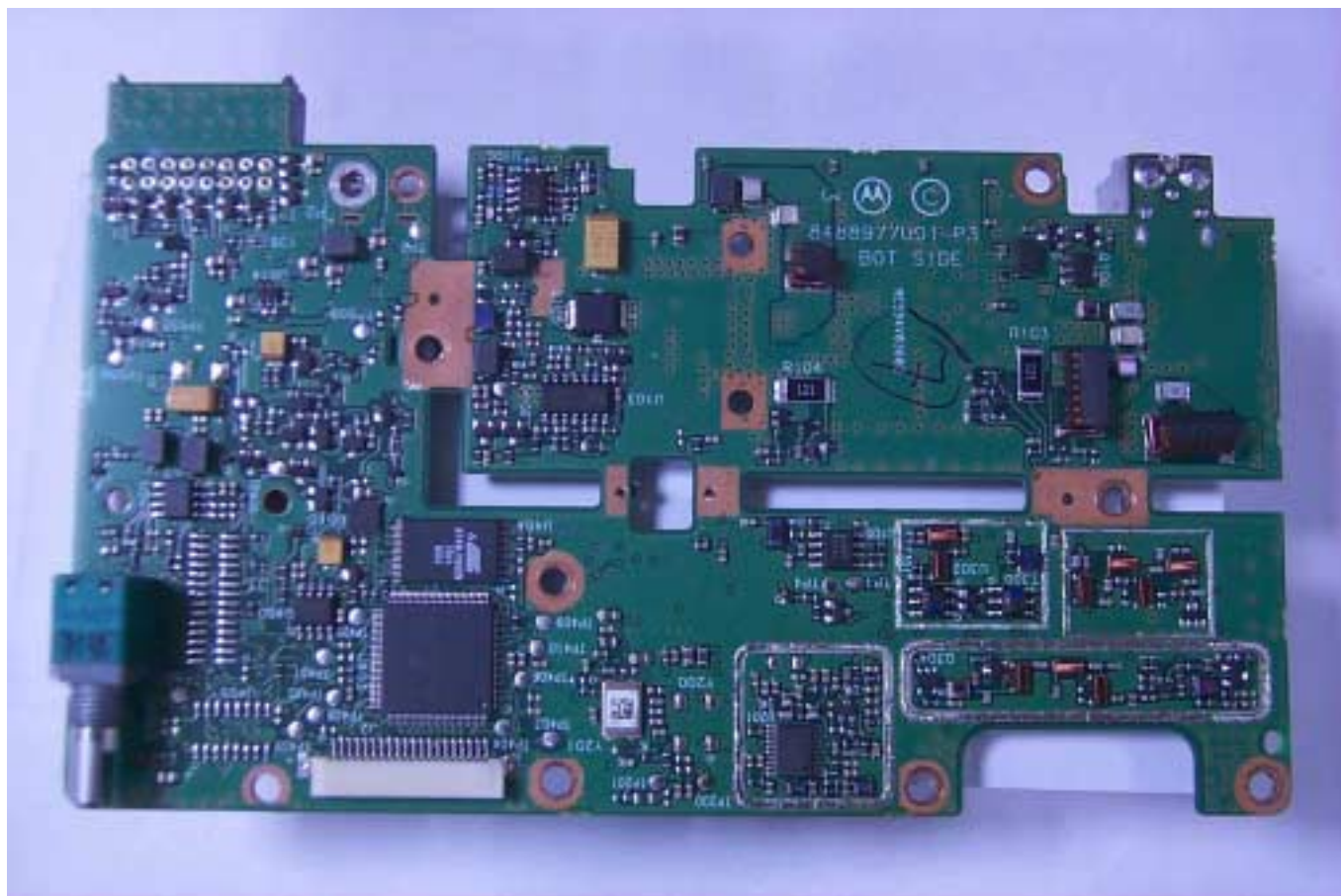
Figure 9-2: Bottom Side of PCB without shields.
