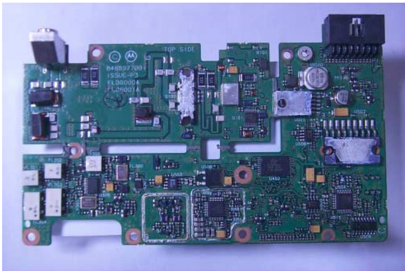
Figure 9-1: Top Side of PCB without shields.
