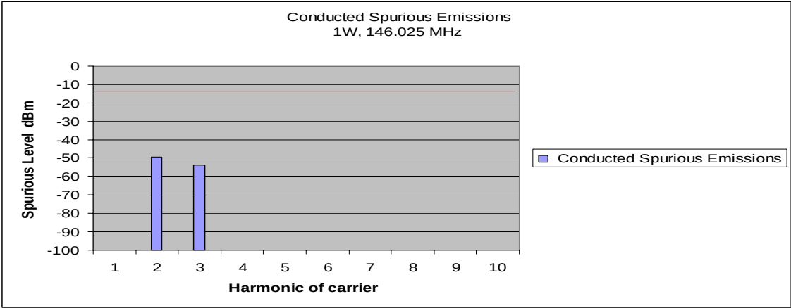
Figure 6F-4: 1 Watt, 146.025 MHz
