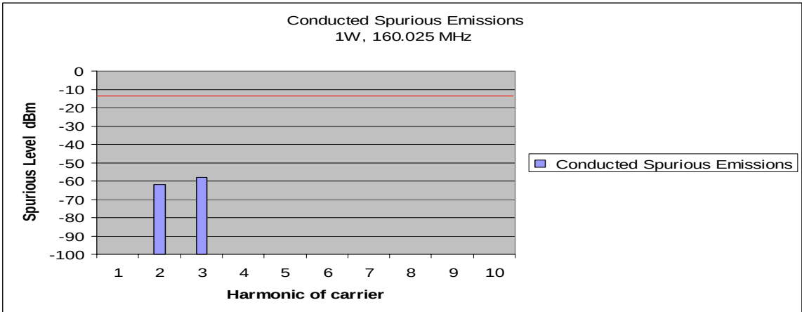
Figure 6F-5: 1 Watt, 160.025 MHz
