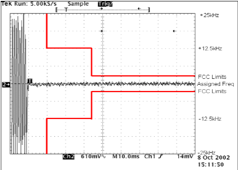
Figure 6I-7: 1 Watt, 25 KHz Key-Up Attack Time
