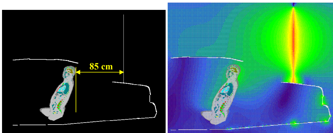
Figure 2: Passenger model exposed to a trunk-mount gain antenna (121.5 cm) operating at 136 MHz: XFDTD geometry and H-field distribution. The antenna is mounted at 85 cm from the passenger.
