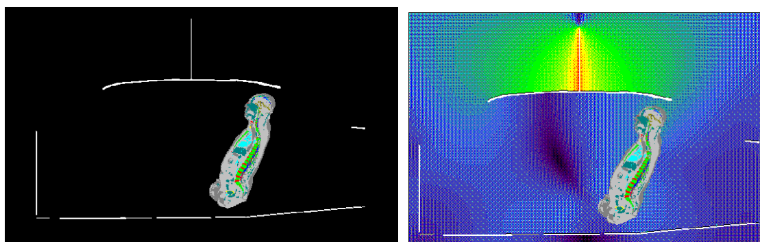
Figure 3: Passenger model exposed to a roof-mount quarter-wave antenna operating at 136 MHz: XFDTD geometry and H-field distribution. The antenna is mounted in the center of the roof.
