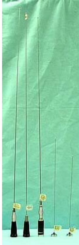
Antenna kit numbers, from left to right: RAD4010ARB, RAD4000A, HAD4014AR, HAD4006A, HAD4009A
