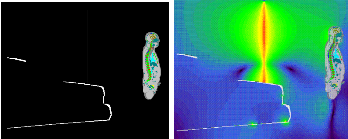
Figure 1: Bystander model exposed to a trunk-mount gain antenna (121.5 cm) operating at 155 MHz: XFDTD geometry and H-field distribution. The antenna is mounted in the center of the trunk.
