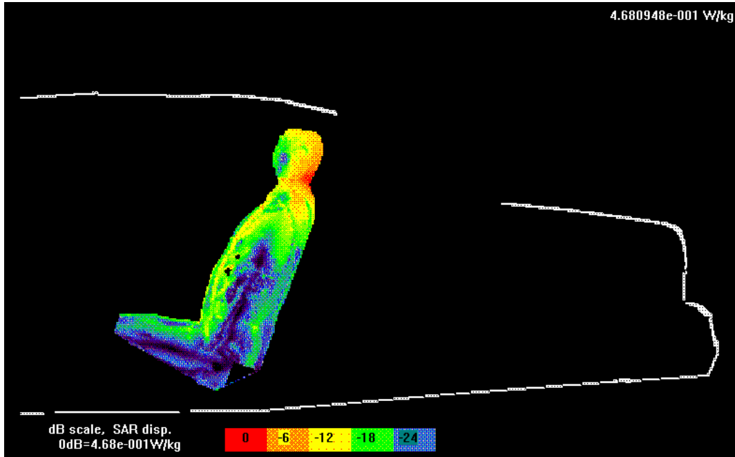
Figure 5. SAR distribution in the passenger in the center of the car back-seat exposed to the 121.5 cm gain antenna mounted on the trunk at a distance of 85 cm from the head.
