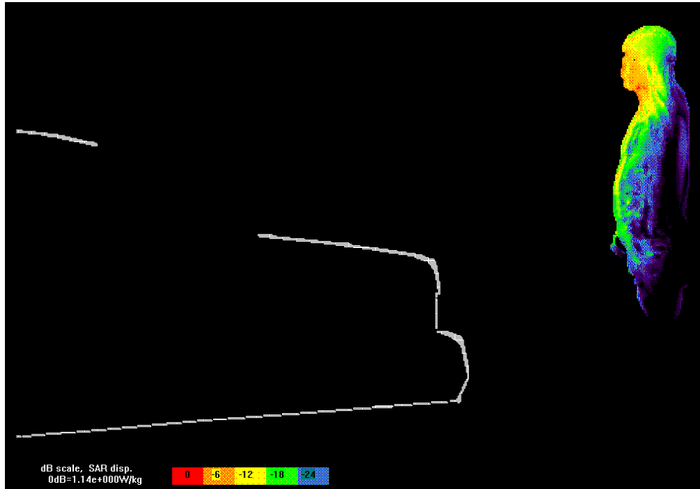
Figure 4. SAR distribution in the bystander at 90 cm from the 117 cm gain antenna, placed in the center of the trunk, when facing the car at 0 degrees.
