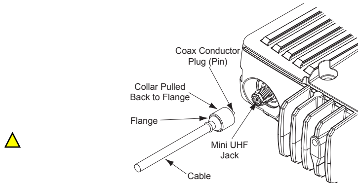
Figure 2-23. Mini-UHF Connection
