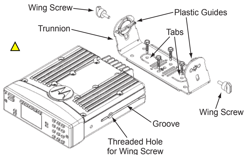
Figure 2-12. Transmission Hump Trunnion Mounting
