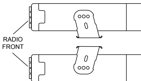
Figure 2-11. Trunnion Orientation
