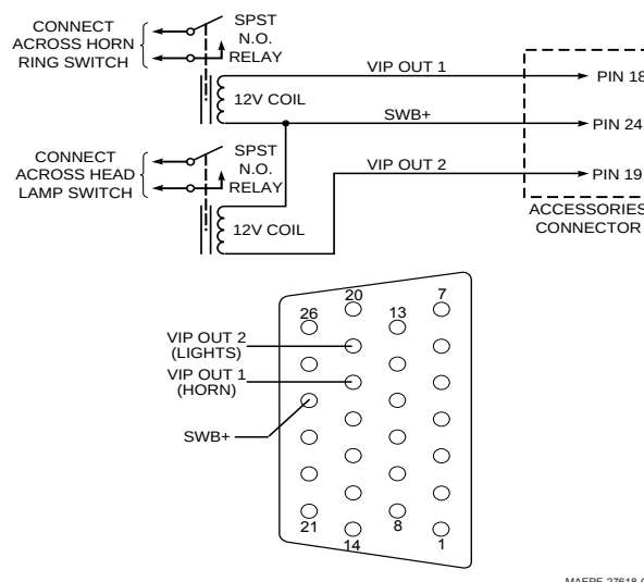
Figure 3-3. Horn/Light Wiring Diagram for W4/5/7/9
