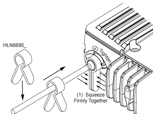
Figure 2-24. Mini-UHF Connector Tool
