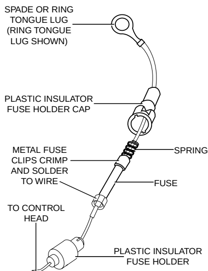
Figure 2-19. Fuseholder Assembly for Orange and Green Control Cables
