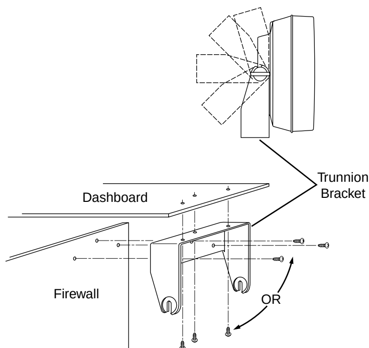
Figure 2-25. Speaker Mounting
