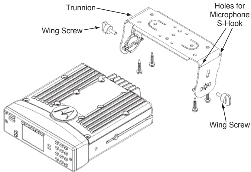
Figure 2-13. Below Dash Trunnion Mounting
