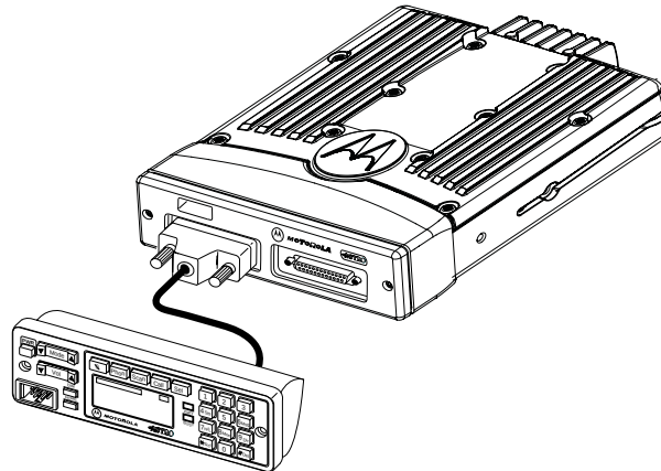
Figure 1-4. Remote Mount Configuration
