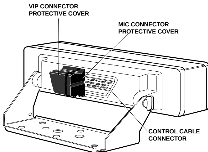
Figure 2-17. W4, W5, and W7 Control Head Rear View
