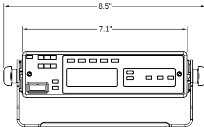
Figure 1-1. Front View of Dash Mount Radio
