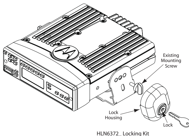
Figure 2-20. Locking Kit (Optional)
