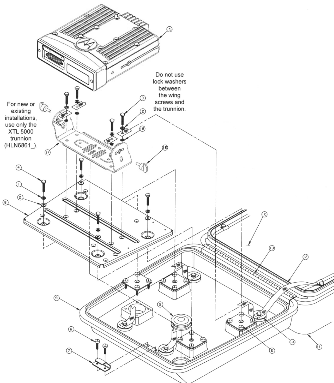
Figure 4-9. Installing the Transceiver
