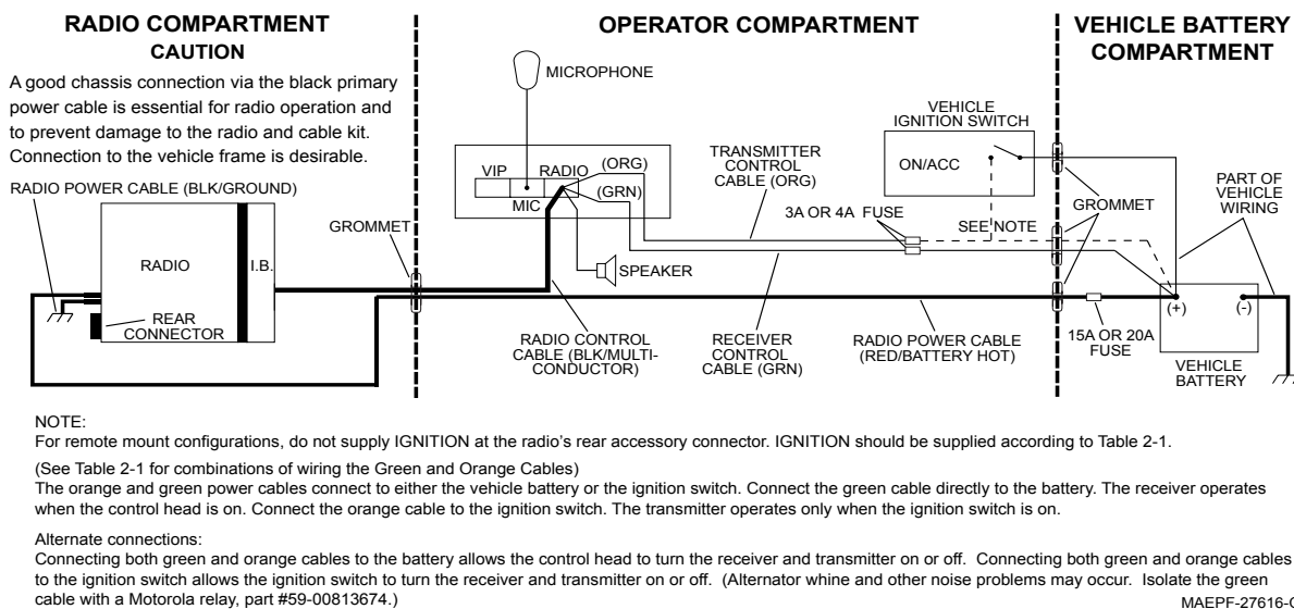
Figure 2-21. Cabling Interconnect Diagram for Remote Mount
