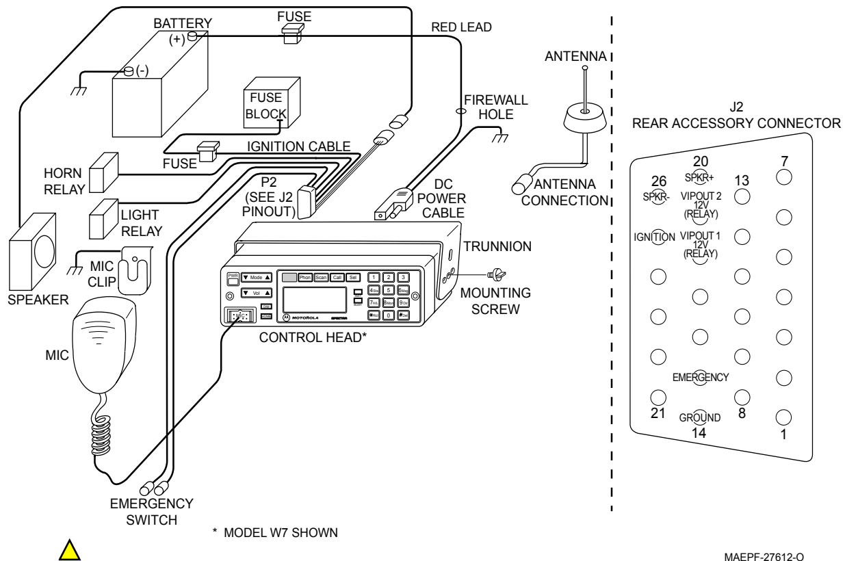
Figure 2-7. Radio Installation (Dash Mount) Using W4, W5, or W7 Control Heads
