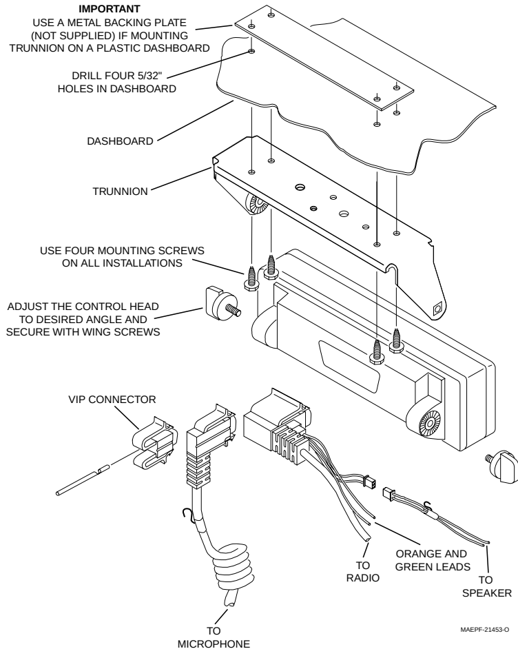
Figure 2-15. W4, W5, and W7 Control Head Installation Exploded View
