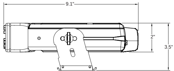
Figure 1-2. Side View of Dash Mount Radio
