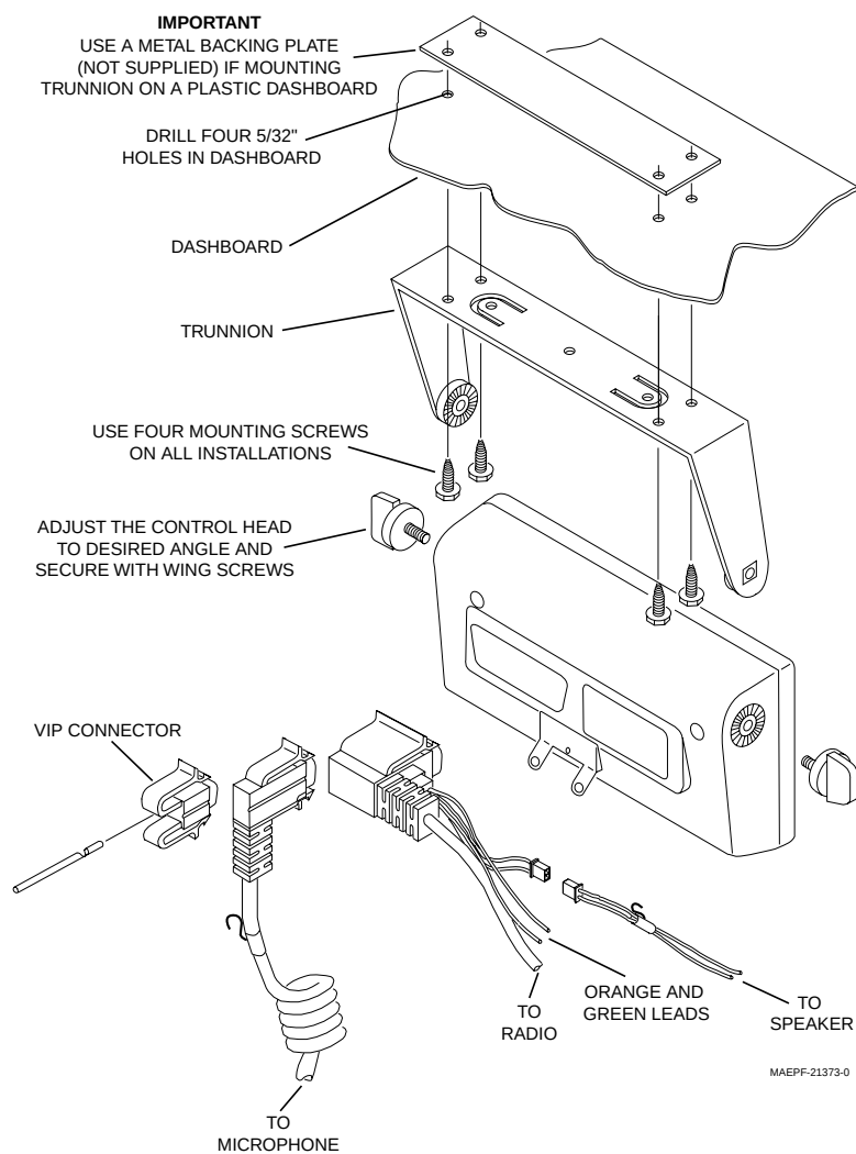
Figure 2-16. W9 Control Head Installation Exploded View
