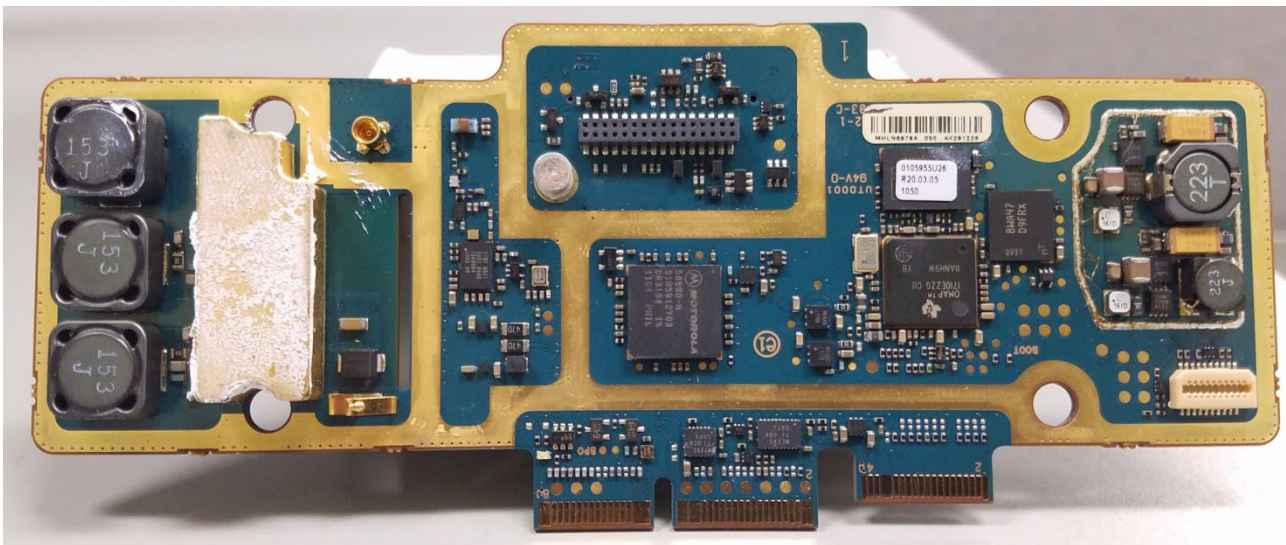
Transceiver Board without Shields (Top)
