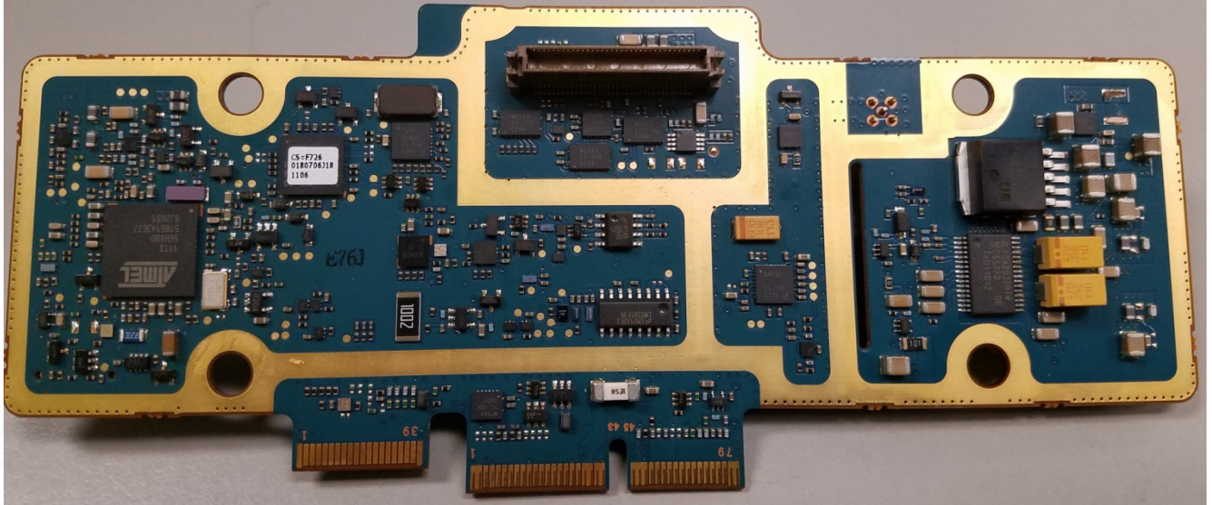
Transceiver Board (Bottom)
