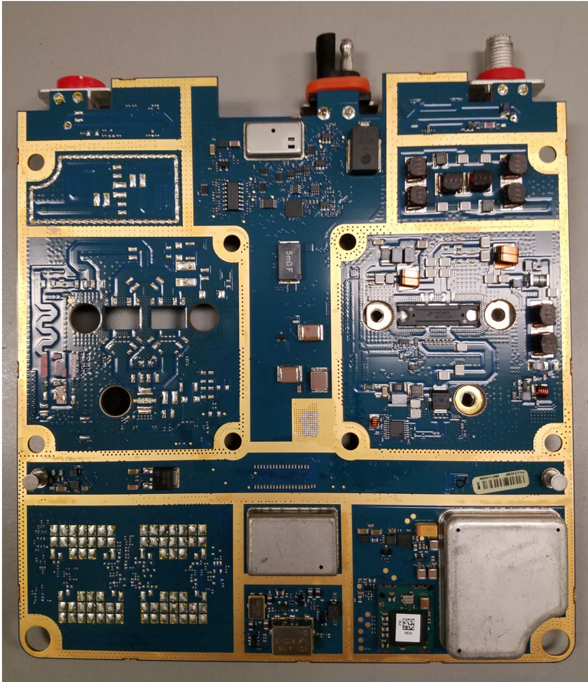
Transmitter board VCO with Shields (Top)
