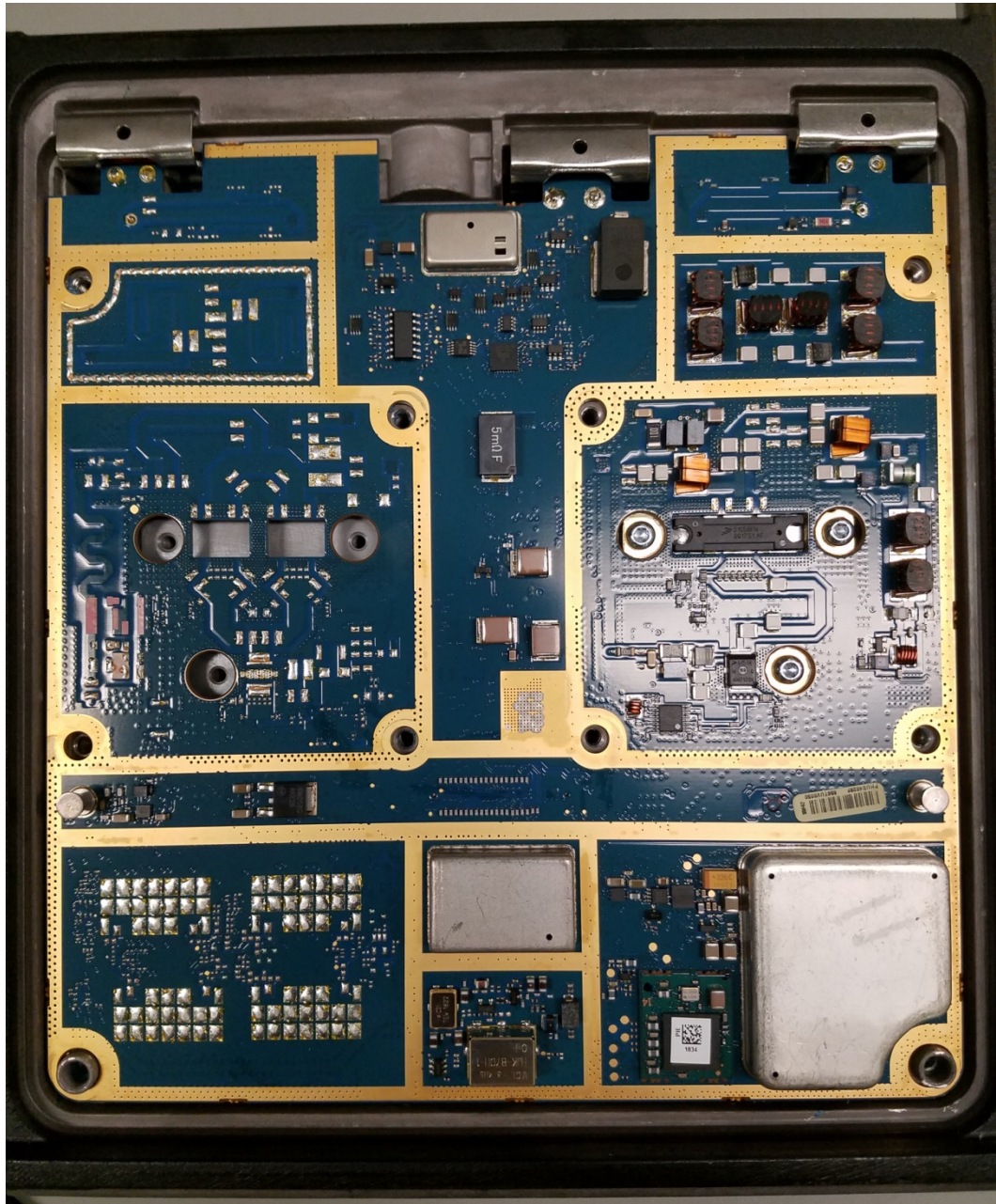
Radio Assembly – Transmitter Board (Top)
