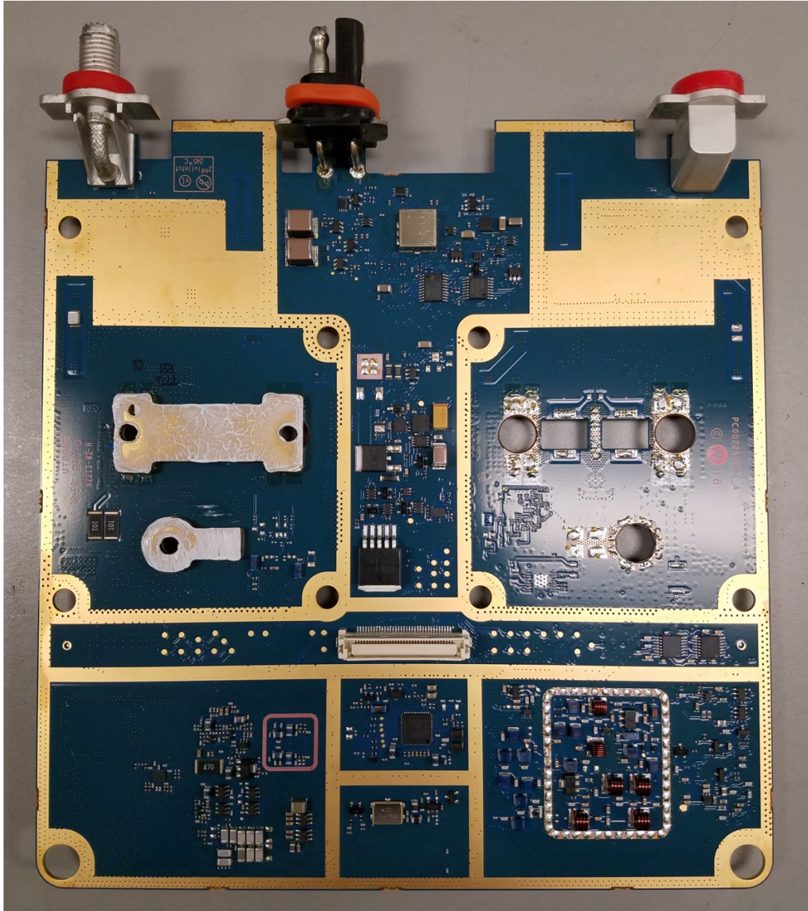
Transmitter board (Bottom)
