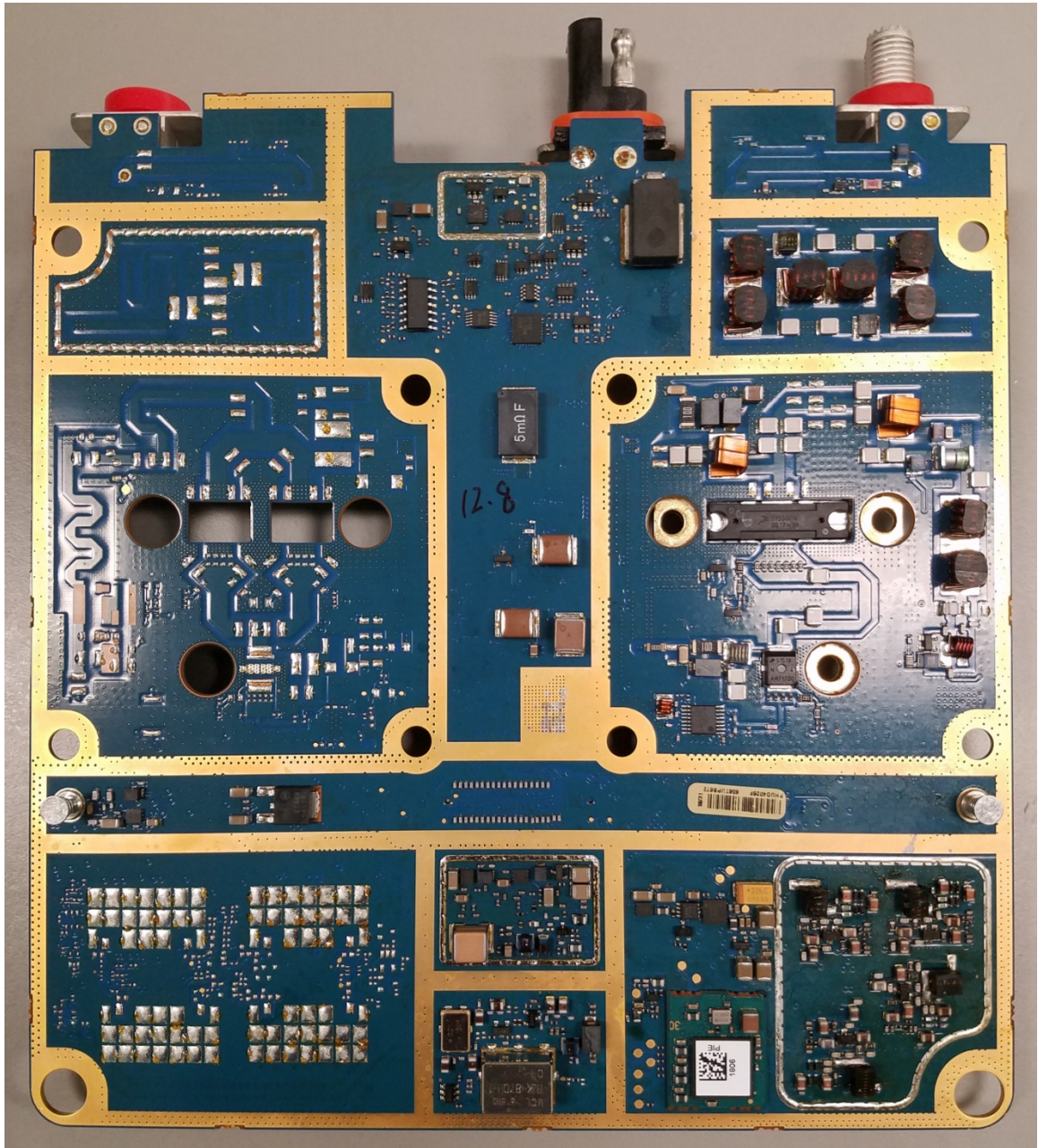
Transmitter board VCO without Shields (Top)
