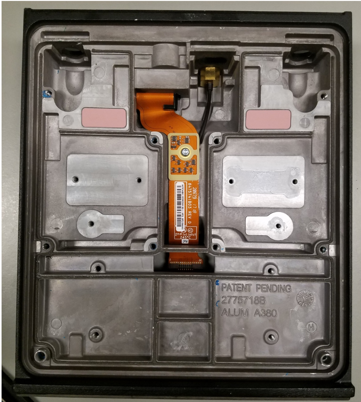
Radio Assembly – Middle Chassis (Top)
