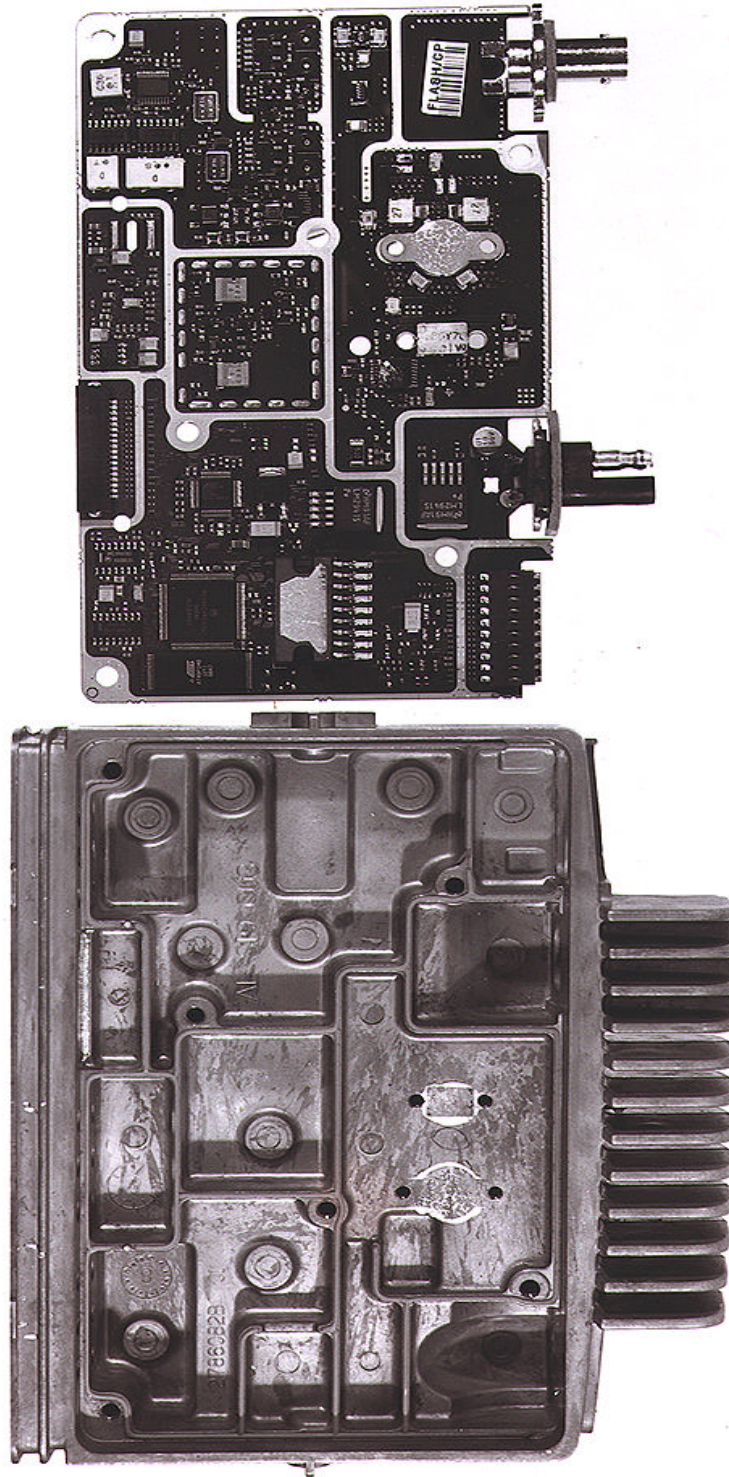
Transceiver Top View with Circuit Board and Control Head Removed (circuit board placed along side the chassis, component-side of board showing)
