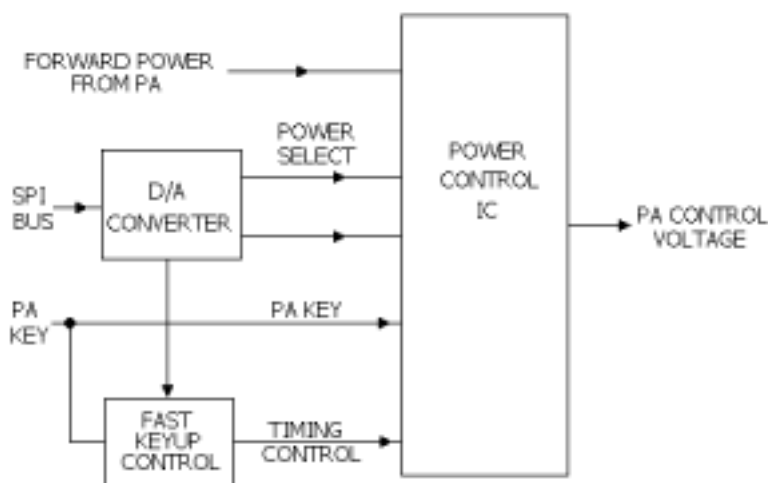
Figure 6: TX Power Control Circuitry
