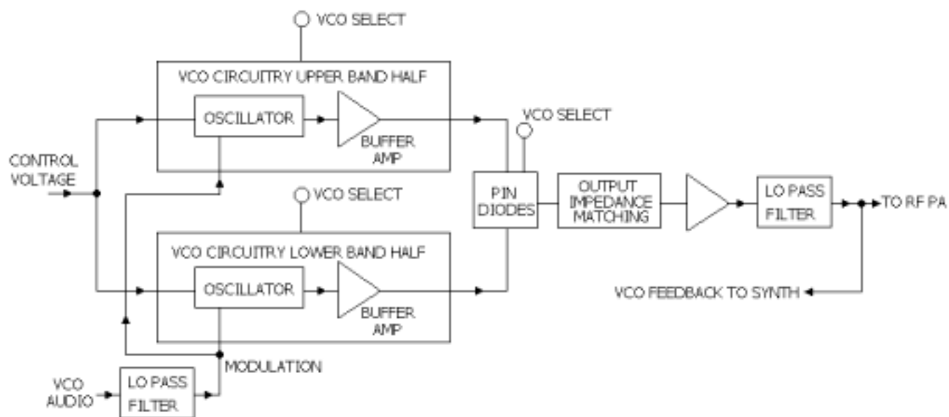
Figure 3: VCO Circuitry
