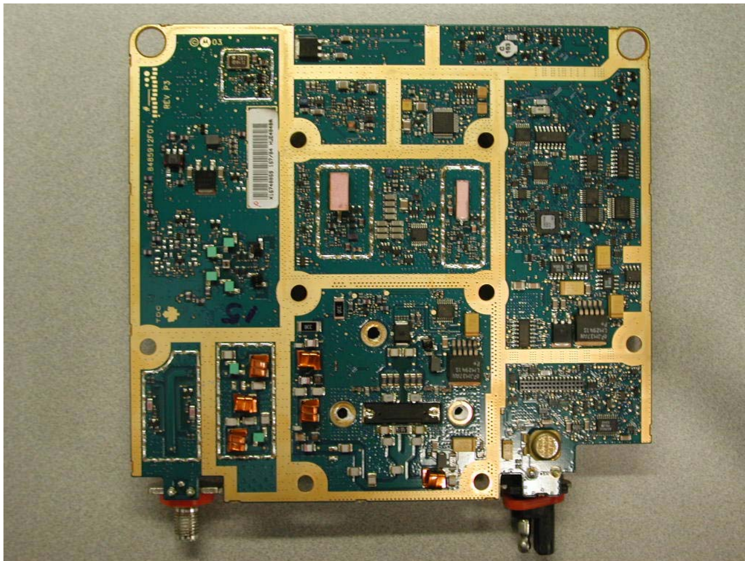
RADIO BOARD, less shield (TOP VIEW)
