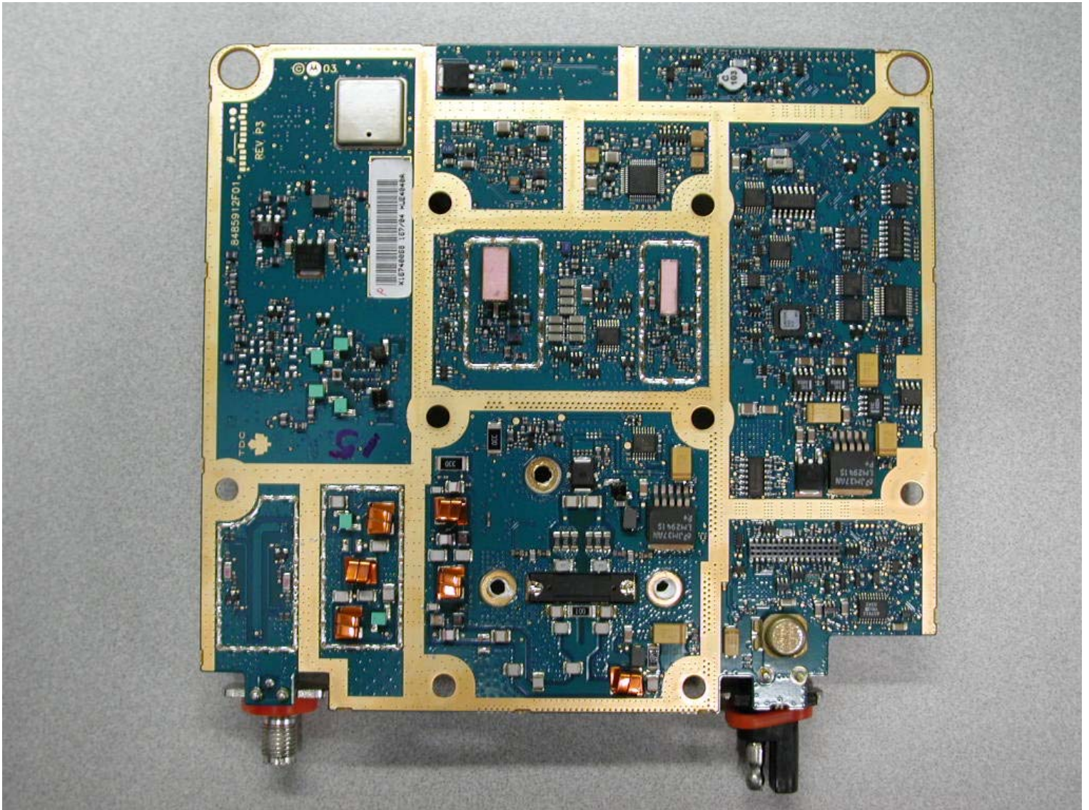
RADIO BOARD (TOP VIEW)
