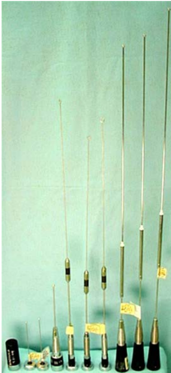
Antenna kit numbers, from left to right; HAE6016A, HAE4004A, HAE4003A, HAE6015A, HAE4011A, HAE4013A, HAE4012A, RAE4016ARB, RAE4015ARB, RAE4014ARB
