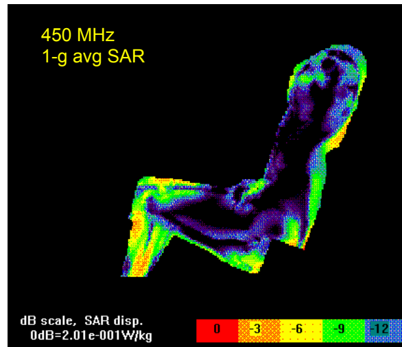
Figure 4: SAR distribution in the passenger model placed in the center of the rear seat, with a trunk-mount antenna operating at 450 MHz.
