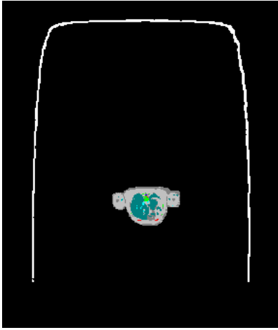
Figure 3: Car passenger model exposed to a quarter wave antenna. Top view.
