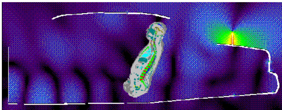
Figure 1: Car passenger model exposed to a quarter wave antenna operating at 450 MHz Lateral view including a time snapshot of the H-field distribution.
