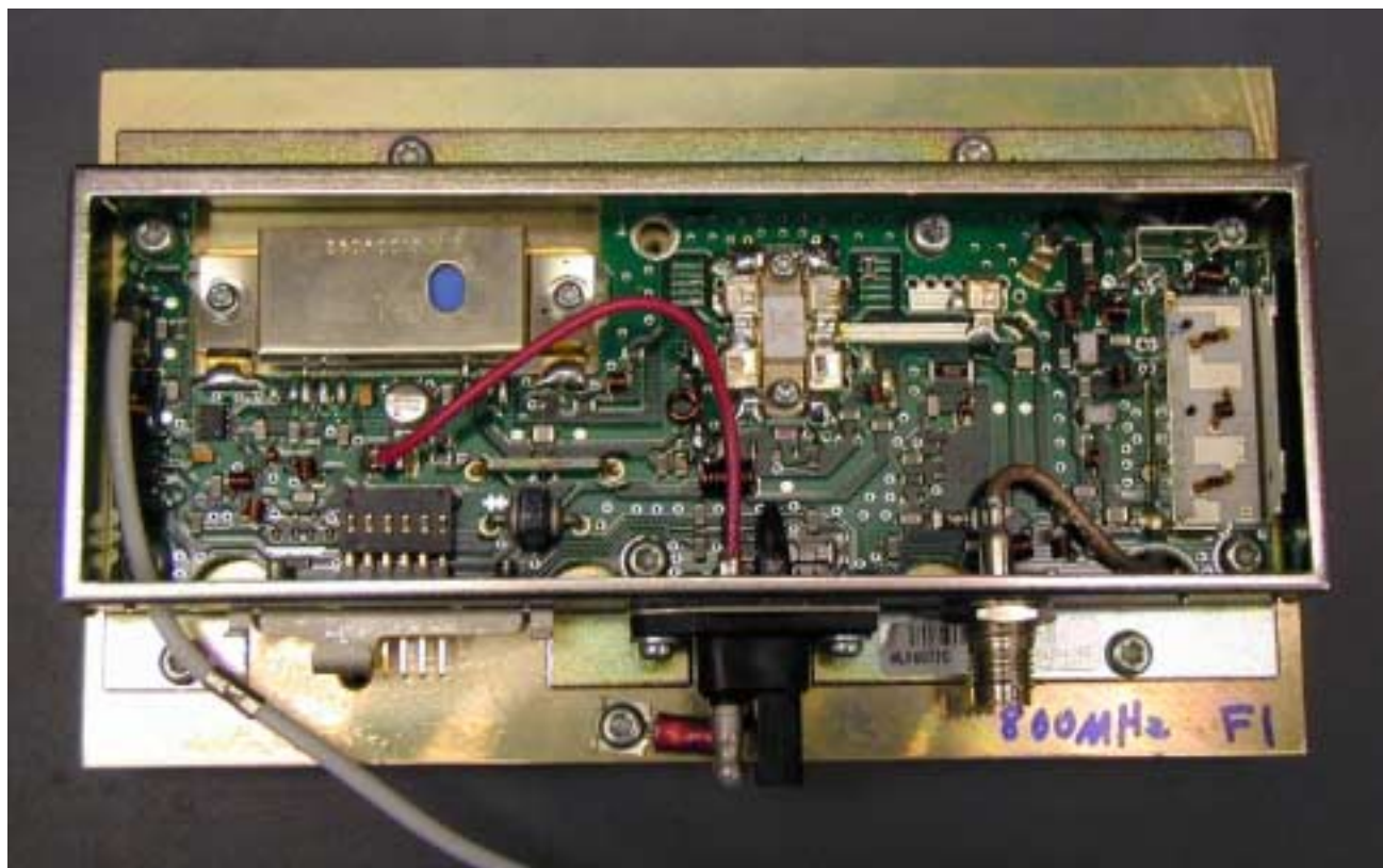
FINAL RF POWER AMPLIFIER MODULE WITH SHIELDS REMOVED
