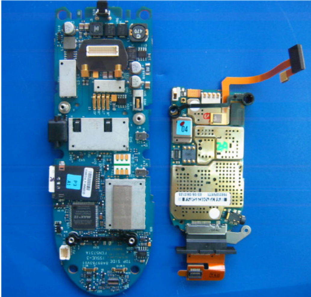
Photograph No.4 M710 main PCB with radio module removed
