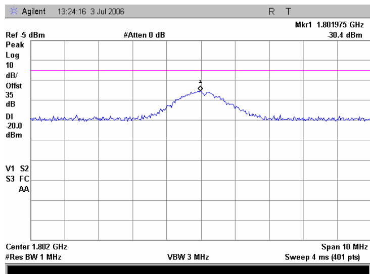
Plot 7.5.30 Conducted spurious emission measurements at the 2 nd harmonic of high carrier frequency, iDEN 900
