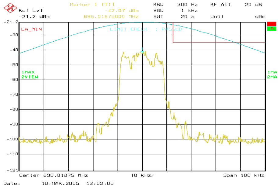
Figure 6a-19 . iDEN 900 MHz Band, Quad-QPSK, Minimum Power, EA Emission Mask
