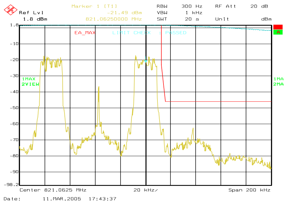
Figure 6a-56 . WiDEN_50_Split 800 MHz Band, QAM16, Maximum Power, EA Emission Mask
