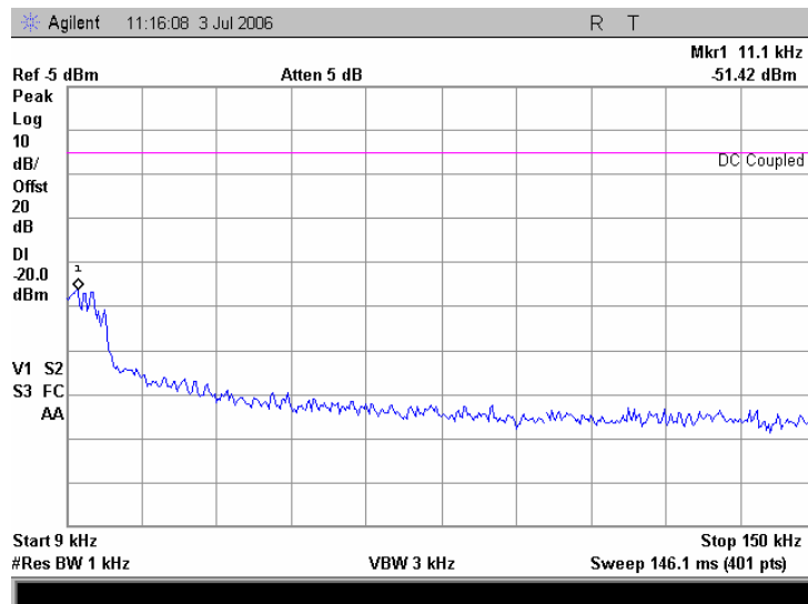
Plot 7.5.6 Spurious emission measurements in 9 - 150 kHz range at high carrier frequency, iDEN 900
