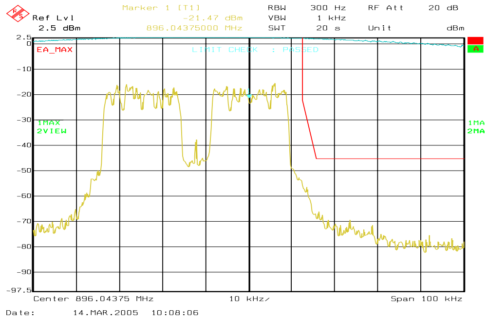
Figure 6a-68 . WiDEN50 900 MHz Band, Continuous QAM16, Maximum Power, EA Emission Mask
