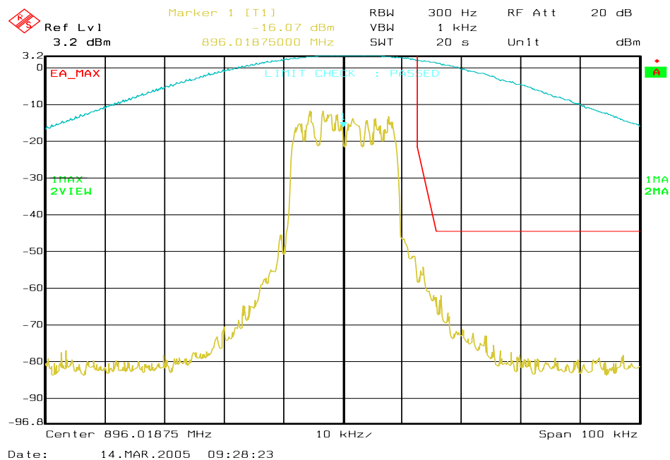
Figure 6a-62 . WiDEN25 900 MHz Band, QAM16, Maximum Power, EA Emission Mask
