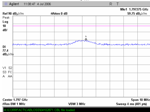
Plot 7.4.36 Radiated emission measurements at the 2 nd harmonic iDEN 900
