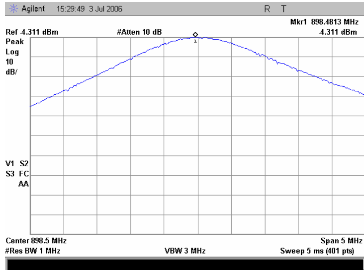
Plot 7.2.9 Reference peak power level at mid frequency, iDEN 900
