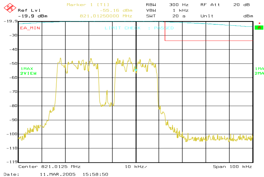
Figure 6a-37 . WiDEN50 800 MHz Band, Continuous Quad-QPSK, Minimum Power, EA Emission Mask
