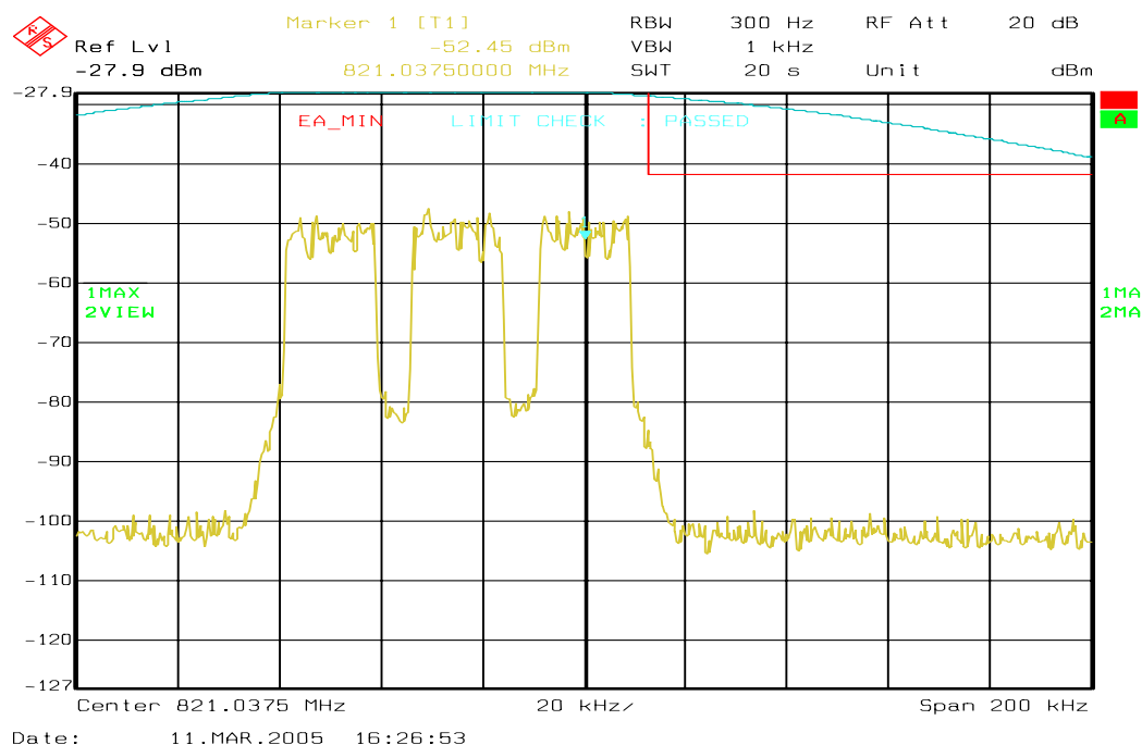
Figure 6a-47 . WiDEN75 800 MHz Band, QAM64, Minimum Power, EA Emission Mask
