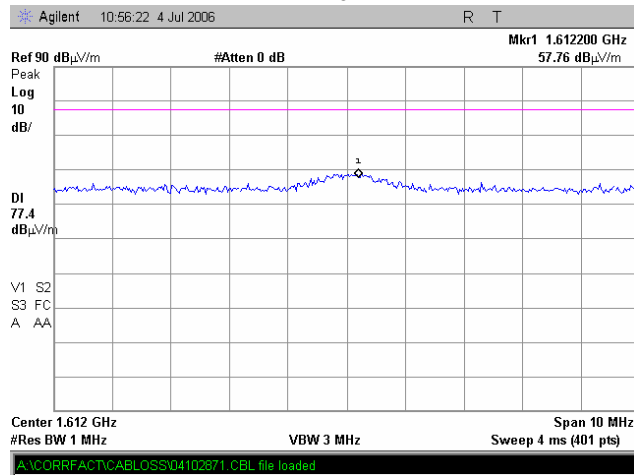
Plot 7.4.32 Radiated emission measurements at the 2 nd harmonic iDEN 800
