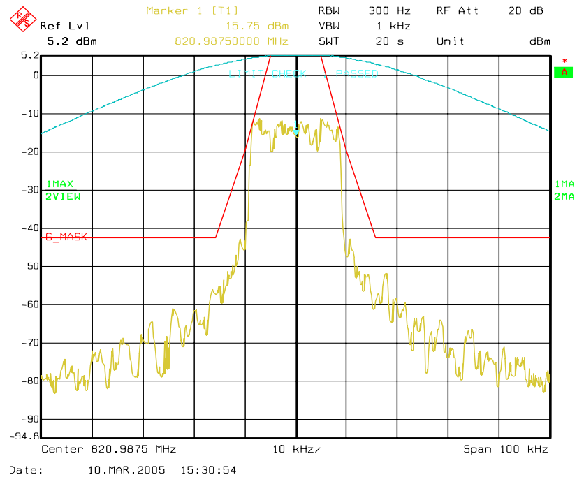
Figure 6a-6 . iDEN 800 MHz Band, QPSK, Maximum Power, Emission Mask G
