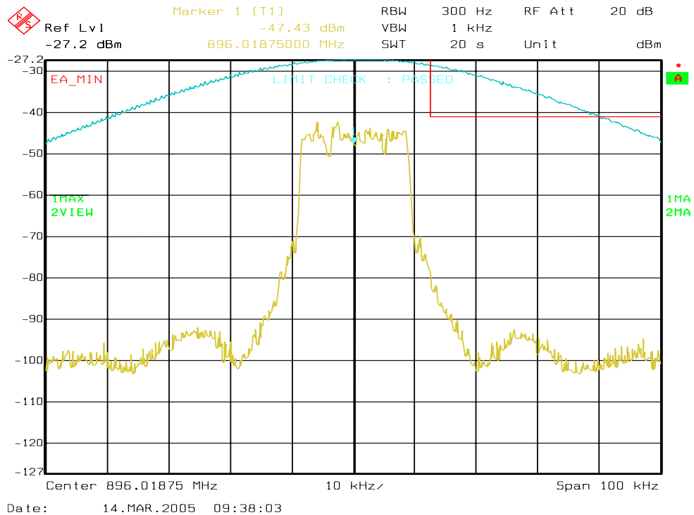
Figure 6a-65 . WiDEN25 900 MHz Band, QAM64, Minimum Power, EA Emission Mask
