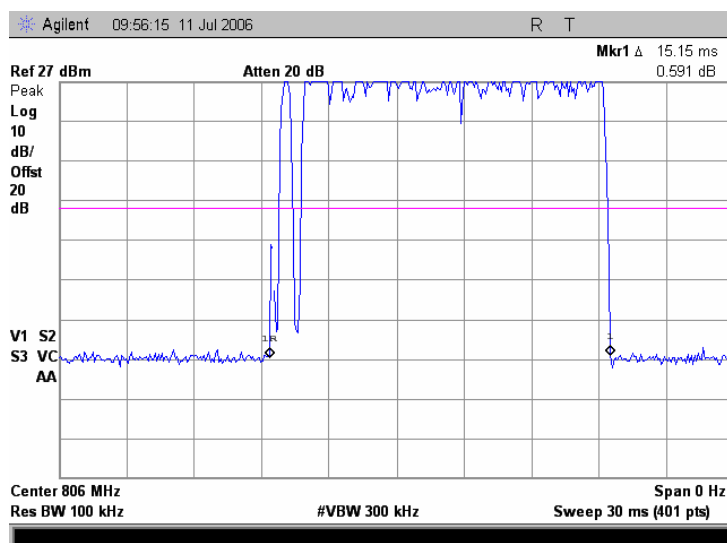
Plot 7.1.2 TDM pulse width at iDEN 800
