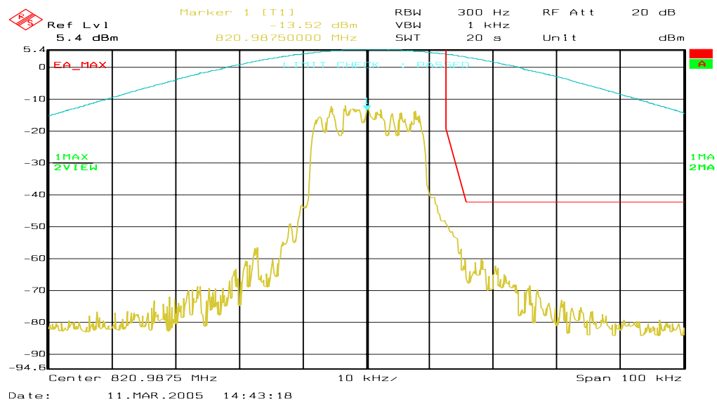
Figure 6a-30 . WiDEN25 800 MHz Band, QAM16, Maximum Power, EA Emission Mask
