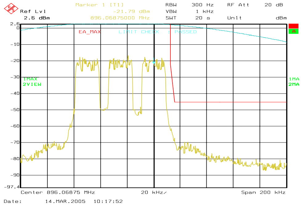
Figure 6a-74 . WiDEN75 900 MHz Band, QAM16, Maximum Power, EA Emission Mask
