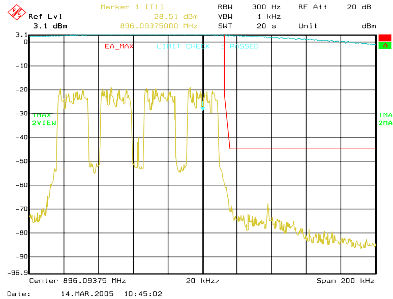
Figure 6a-78 . WiDEN100 900 MHz Band, Quad-QPSK, Maximum Power, EA Emission Mask
