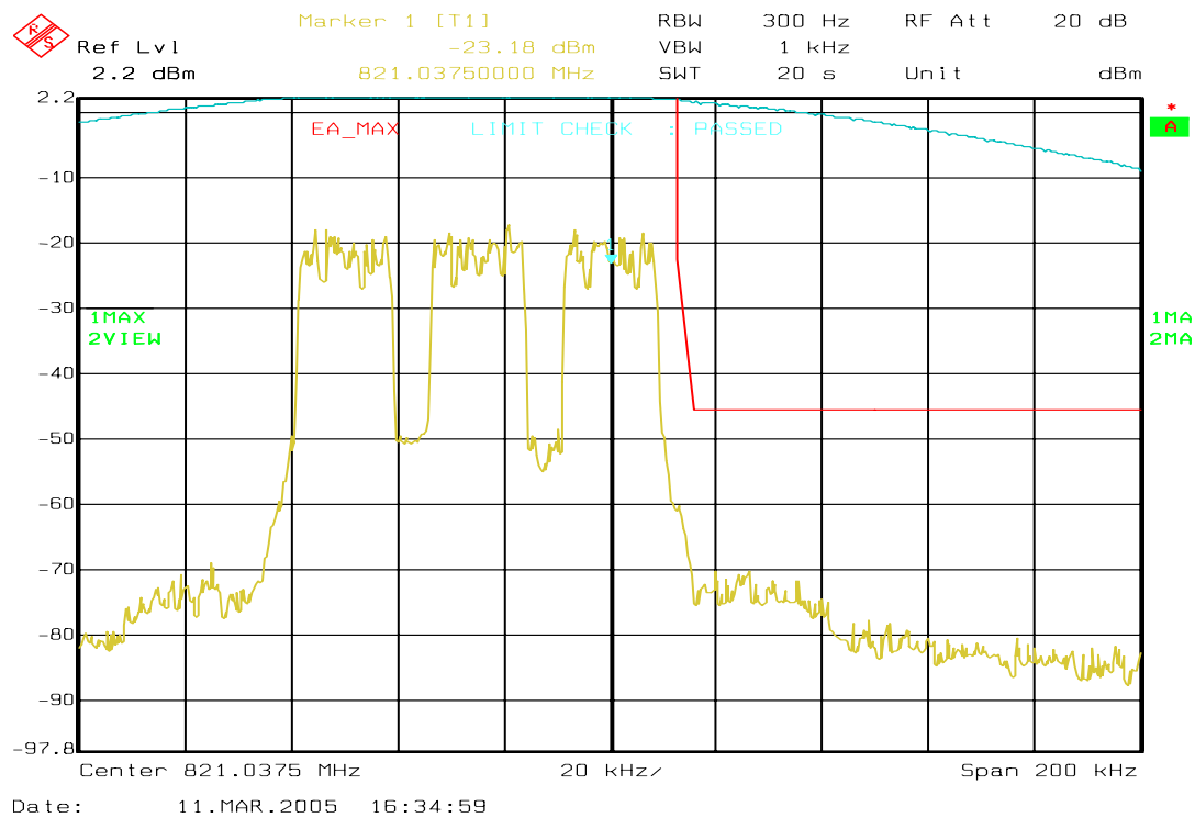
Figure 6a-44 . WiDEN75 800 MHz Band, QAM16, Maximum Power, EA Emission Mask
