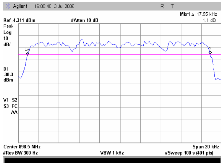
Plot 7.2.10 Occupied bandwidth test result at mid frequency, iDEN 900
