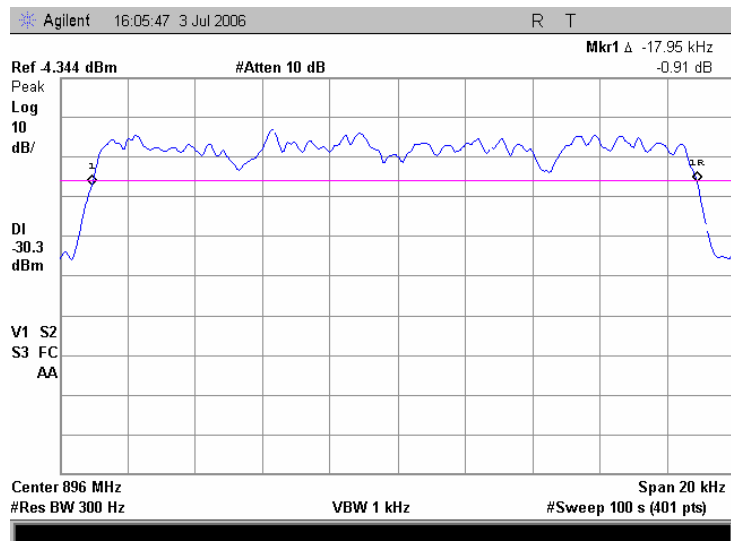
Plot 7.2.8 Occupied bandwidth test result at low frequency, iDEN 900
