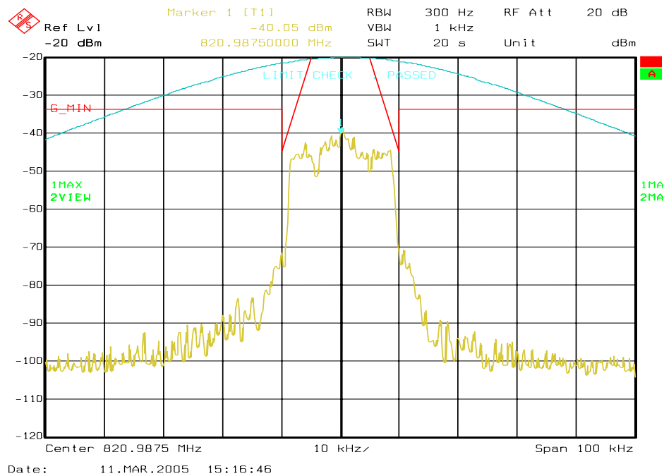
Figure 6a-33 . WiDEN25 800 MHz Band, QAM64, Minimum Power, Emission Mask G
