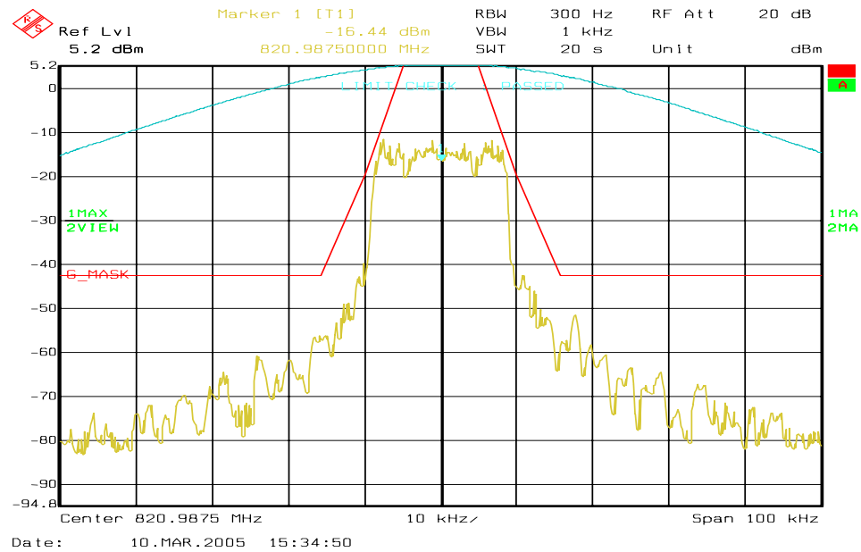
Figure 6a-10 . iDEN 800 MHz Band, QAM16, Maximum Power, Emission Mask G
