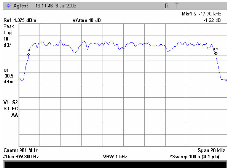
Plot 7.2.12 Occupied bandwidth test result at high frequency, iDEN 900
