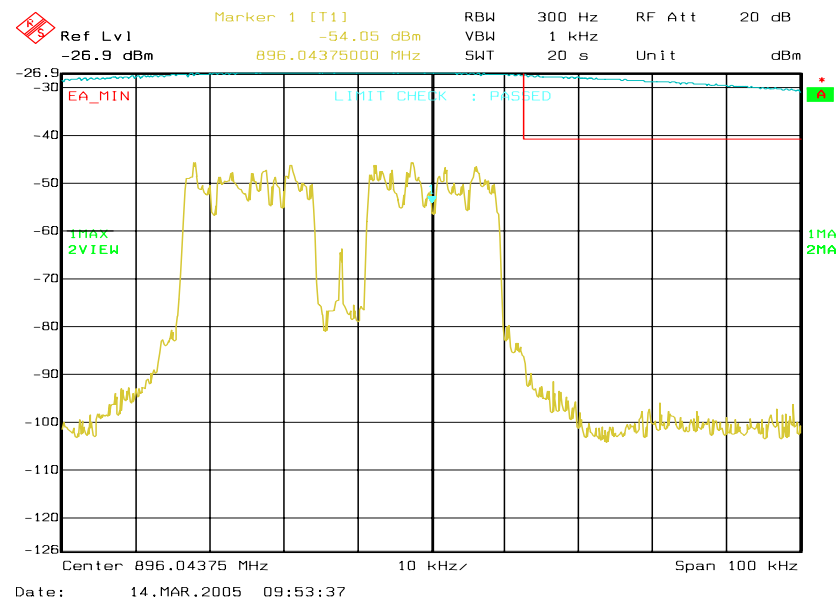
Figure 6a-67 . WiDEN50 900 MHz Band, Continuous Quad-QPSK, Minimum Power, EA Emission Mask
