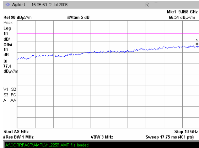
Plot 7.4.26 Radiated emission measurements in 2900 – 10000 MHz range
