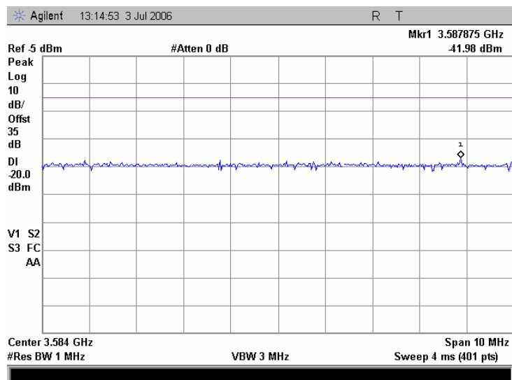
Plot 7.5.40 Conducted spurious emission measurements at the 4 th harmonic of low carrier frequency, iDEN 900
