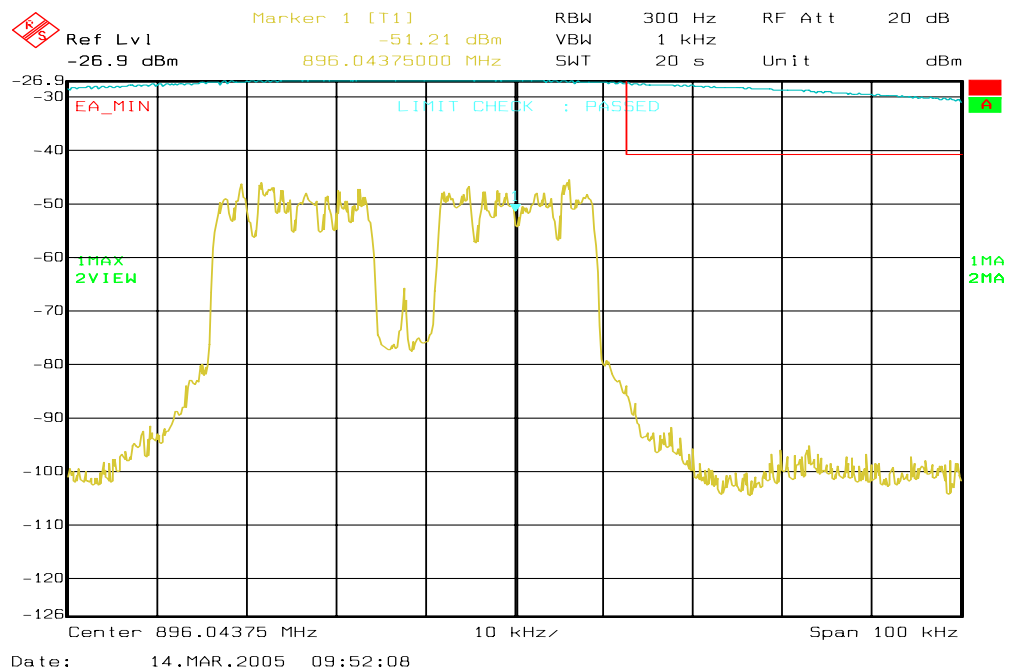
Figure 6a-69 . WiDEN50 900 MHz Band, Continuous QAM16, Minimum Power, EA Emission Mask
