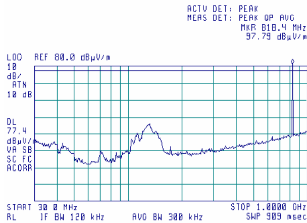
Plot 7.4.16 Radiated emission measurements in 30 - 1000 MHz range
