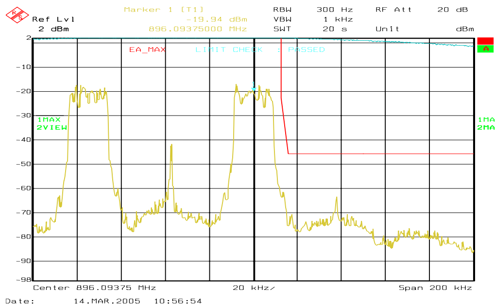
Figure 6a-86 . WiDEN_50_Split 900 MHz Band, QAM16, Maximum Power, EA Emission Mask
