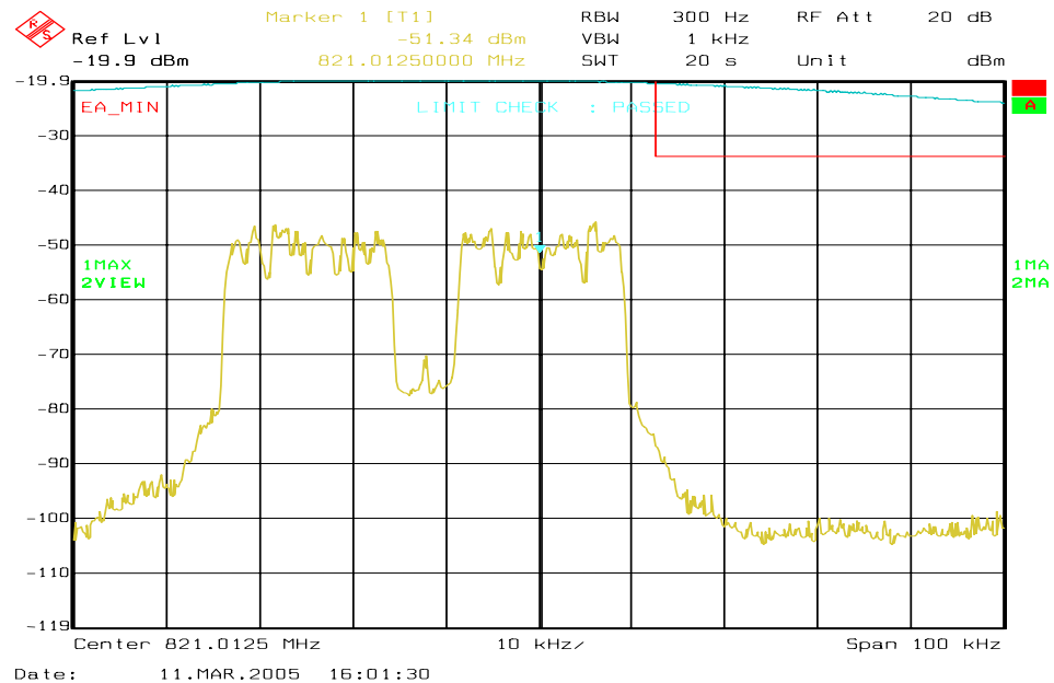
Figure 6a-39 . WiDEN50 800 MHz Band, Continuous QAM16, Minimum Power, EA Emission Mask
