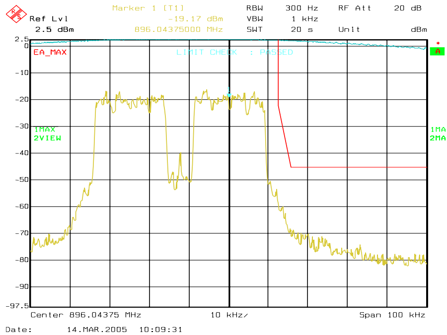
Figure 6a- 70. WiDEN50 900 MHz Band, Continuous QAM64, Maximum Power, EA Emission Mask
