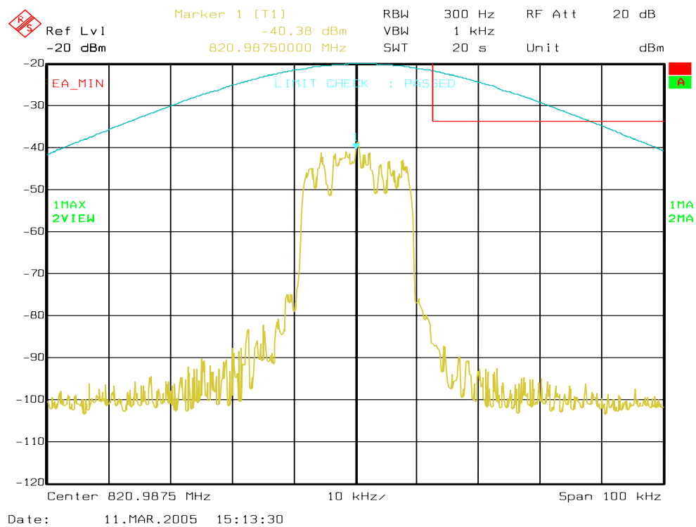
Figure 6a-31 . WiDEN25 800 MHz Band, QAM16, Minimum Power, EA Emission Mask
