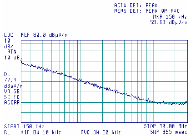
Plot 7.4.12 Radiated emission measurements in 0.15 - 30 MHz range
