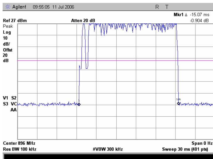
Plot 7.1.4 TDM pulse width at iDEN 900
