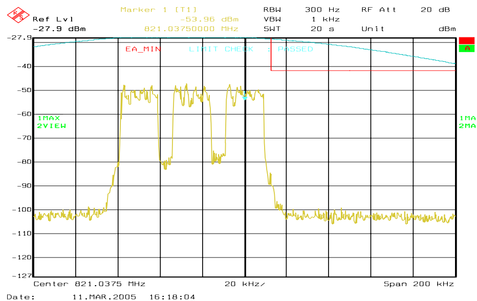
Figure 6a-43 . WiDEN75 800 MHz Band, Quad-QPSK, Minimum Power, EA Emission Mask
