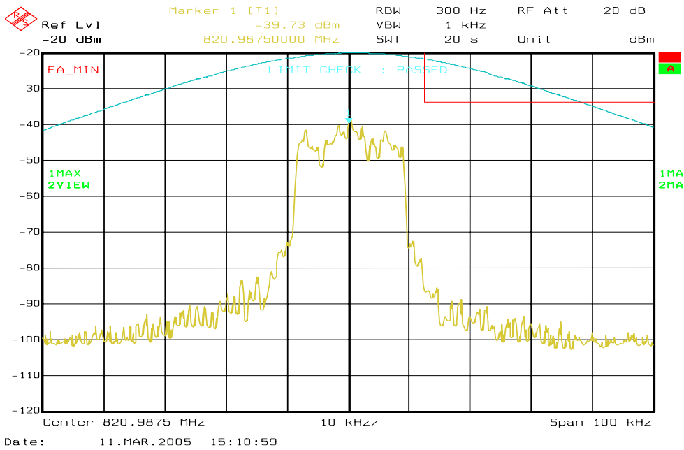
Figure 6a- 27. WiDEN25 800 MHz Band, Quad-QPSK, Minimum Power, EA Emission Mask
