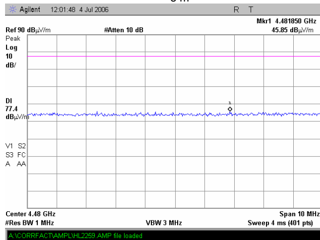
Plot 7.4.52 Radiated emission measurements at the 5 th harmonic iDEN 900
