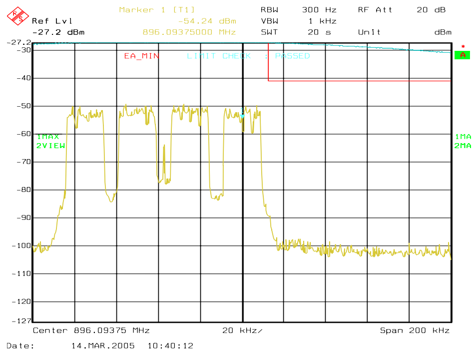
Figure 6a-83 . WiDEN100 900 MHz Band, QAM64, Minimum Power, EA Emission Mask
