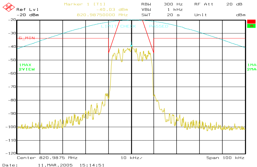
Figure 6a-29 . WiDEN25 800 MHz Band, QAM16, Minimum Power, Emission Mask G
