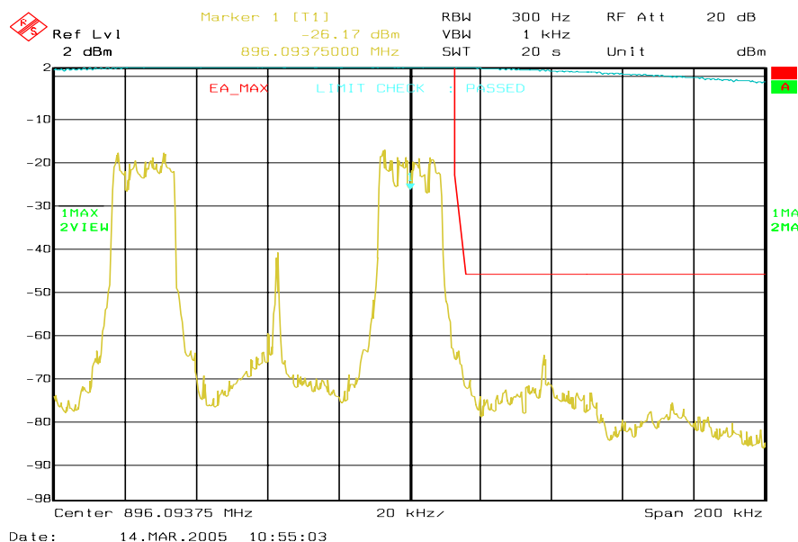
Figure 6a-84 . WiDEN_50_Split 900 MHz Band, Quad-QPSK, Maximum Power, EA Emission Mask
