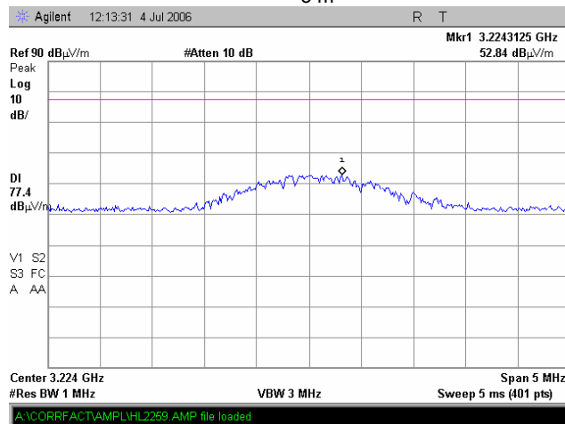
Plot 7.4.44 Radiated emission measurements at the 4 th harmonic iDEN 800
