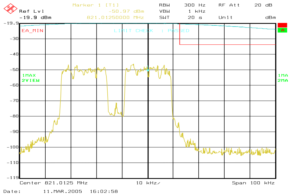
Figure 6a-41 . WiDEN50 800 MHz Band, Continuous QAM64, Minimum Power, EA Emission Mask
