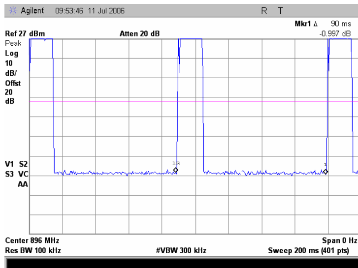
Plot 7.1.3 TDM period at iDEN 900
