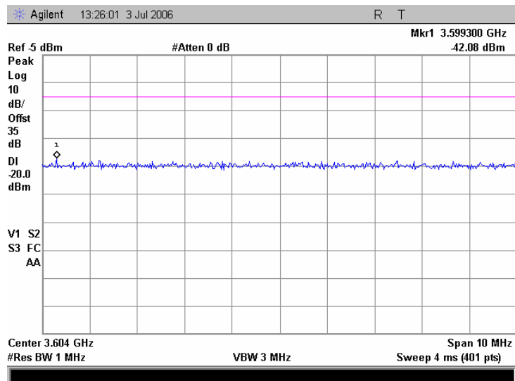
Plot 7.5.42 Conducted spurious emission measurements at the 4 th harmonic of high carrier frequency, iDEN 900
