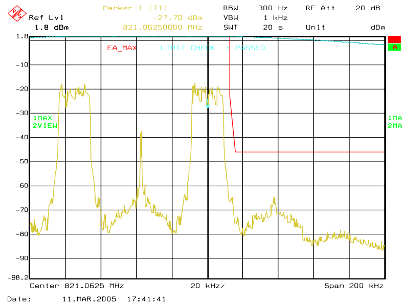
Figure 6a-54 . WiDEN_50_Split 800 MHz Band, Quad-QPSK, Maximum Power, EA Emission Mask
