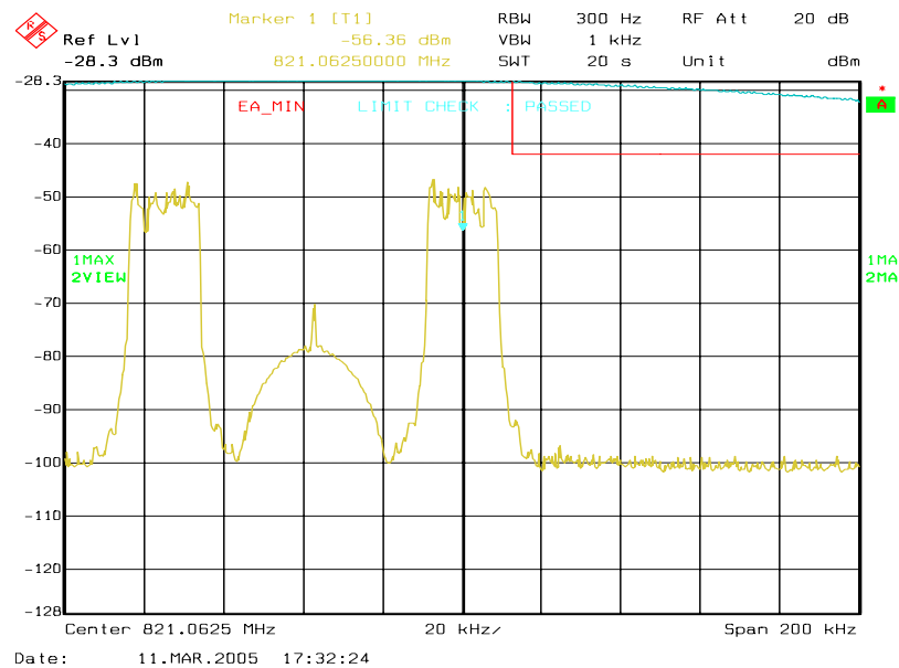
Figure 6a-55 . WiDEN_50_Split 800 MHz Band, Quad-QPSK, Minimum Power, EA Emission Mask
