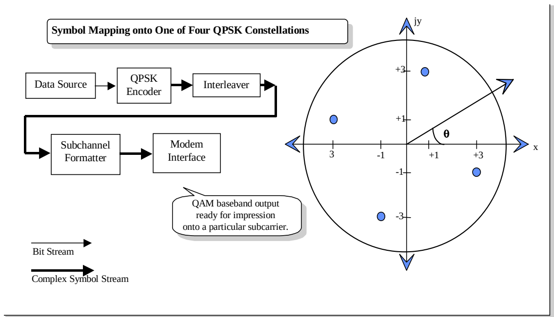
Figure 6a-3. Symbol Mapping onto One of Four QPSK Constellations
