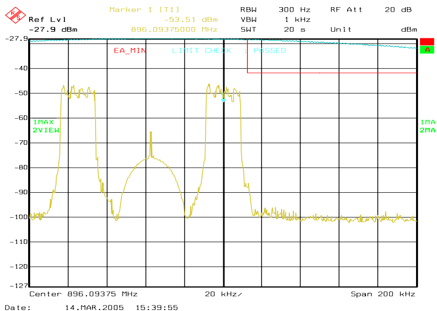
Figure 6a-85 . WiDEN_50_Split 900 MHz Band, Quad-QPSK, Minimum Power, EA Emission Mask
