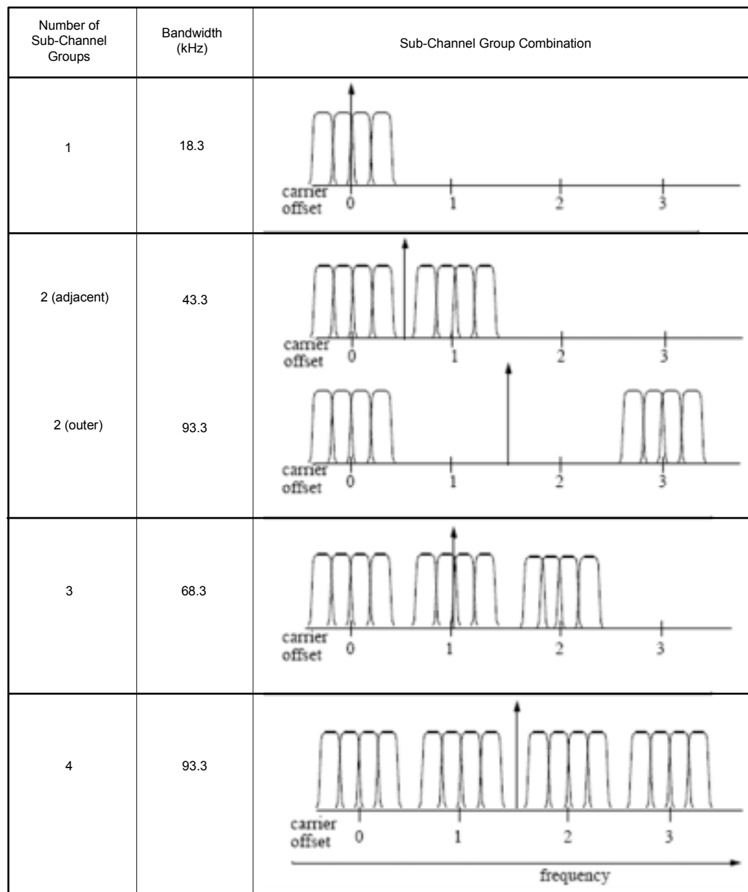
Figure 6a-2: Sub-Channel Group Combination Bandwidths
