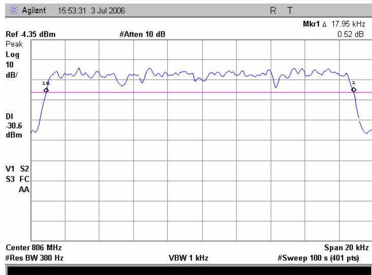
Plot 7.2.2 Occupied bandwidth test result at low frequency, iDEN 800
