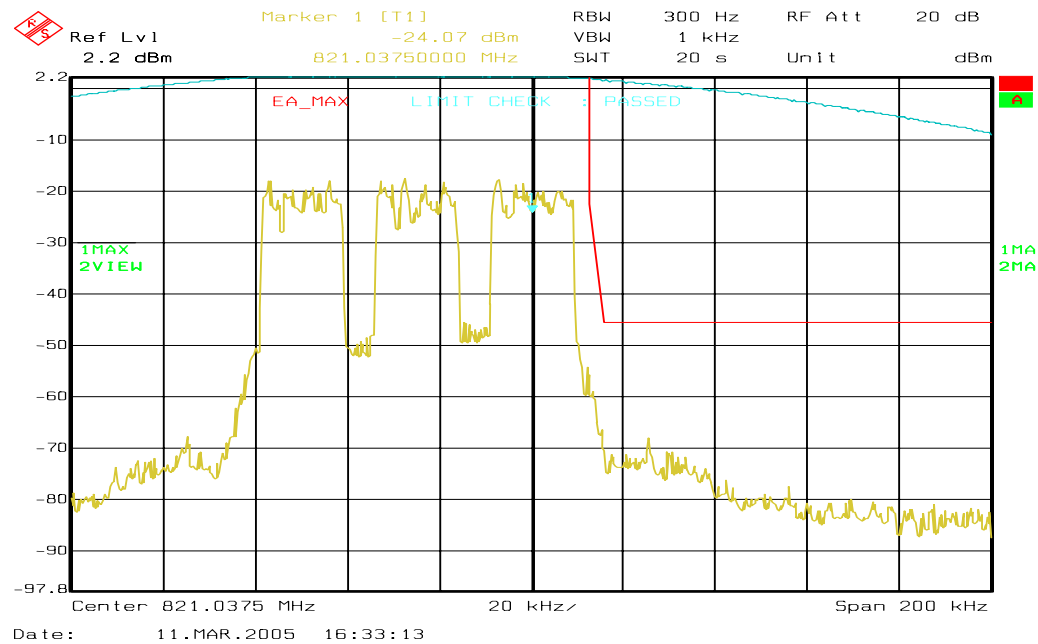
Figure 6a-42 . WiDEN75 800 MHz Band, Quad-QPSK, Maximum Power, EA Emission Mask
