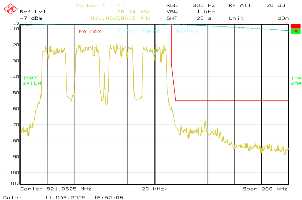
Figure 6a-52 . WiDEN100 800 MHz Band, QAM64, Maximum Power, EA Emission Mask
