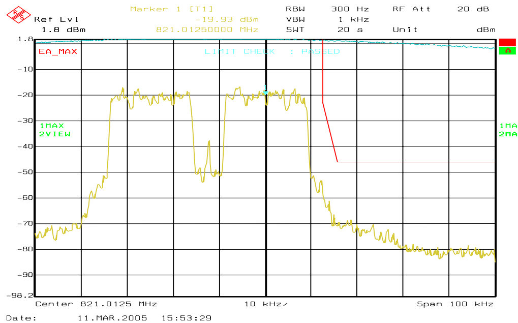
Figure 6a-40 . WiDEN50 800 MHz Band, Continuous QAM64, Maximum Power, EA Emission Mask
