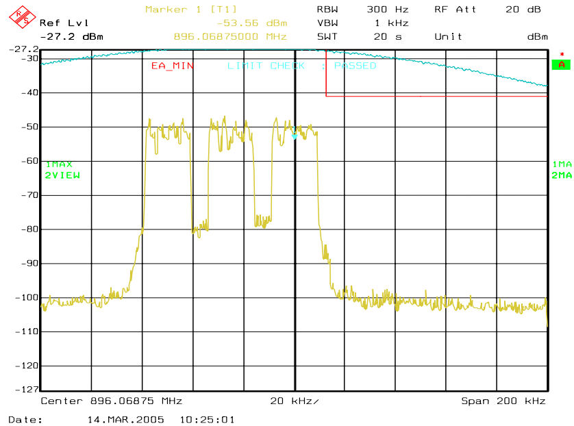
Figure 6a-73 . WiDEN75 900 MHz Band, Quad-QPSK, Minimum Power, EA Emission Mask
