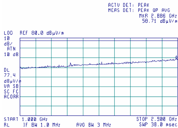
Plot 7.4.20 Radiated emission measurements in 1000 – 2900 MHz range
