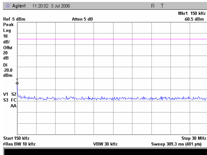
Plot 7.5.10 Spurious emission measurements in 0.15 - 30.0 MHz range at low carrier frequency, iDEN 900
