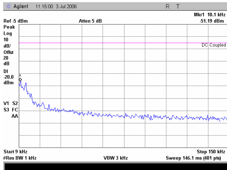
Plot 7.5.5 Spurious emission measurements in 9 - 150 kHz range at mid carrier frequency, iDEN 900
