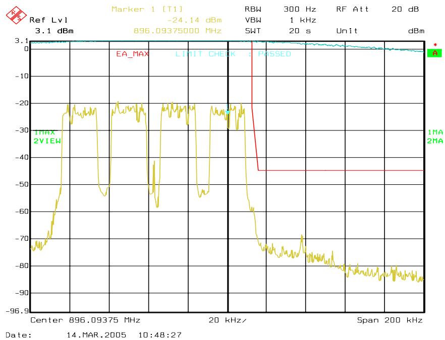
Figure 6a-82 . WiDEN100 900 MHz Band, QAM64, Maximum Power, EA Emission Mask
