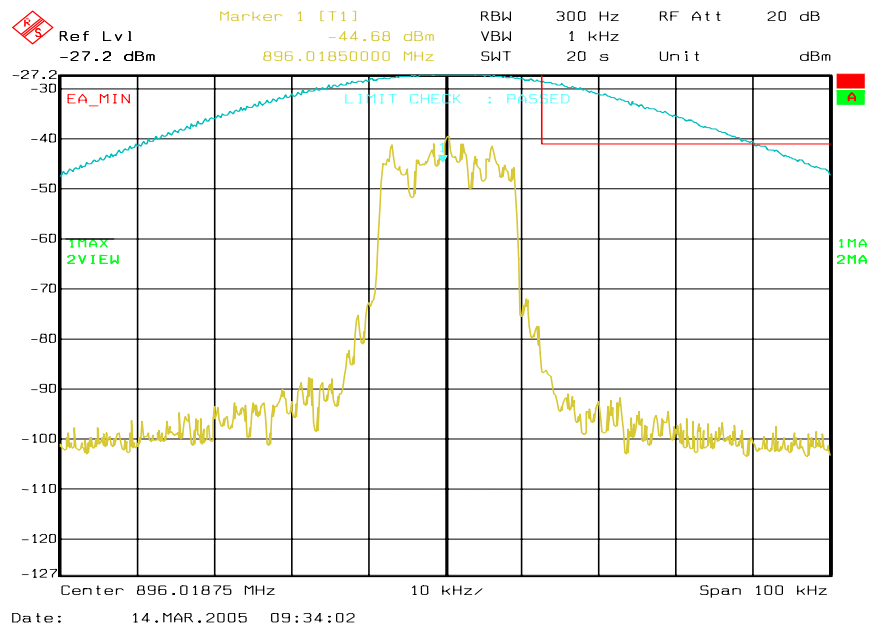
Figure 6a-61 . WiDEN25 900 MHz Band, Quad-QPSK, Minimum Power, EA Emission Mask
