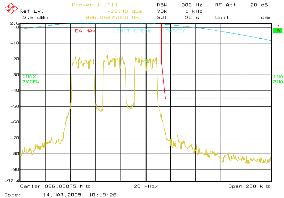
Figure 6a-76 . WiDEN75 900 MHz Band, QAM64, Maximum Power, EA Emission Mask
