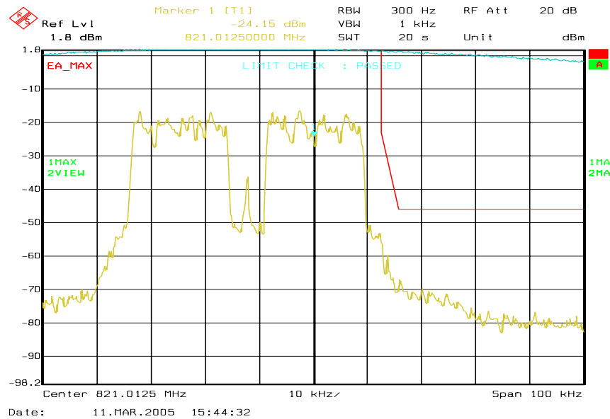
Figure 6a-36 . WiDEN50 800 MHz Band, Continuous Quad-QPSK, Maximum Power, EA Emission Mask
