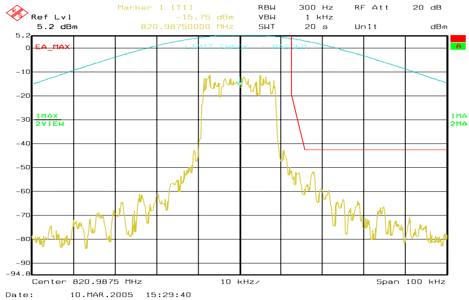
Figure 6a-8 . iDEN 800 MHz Band, Quad-QPSK, Maximum Power, EA Emission Mask
