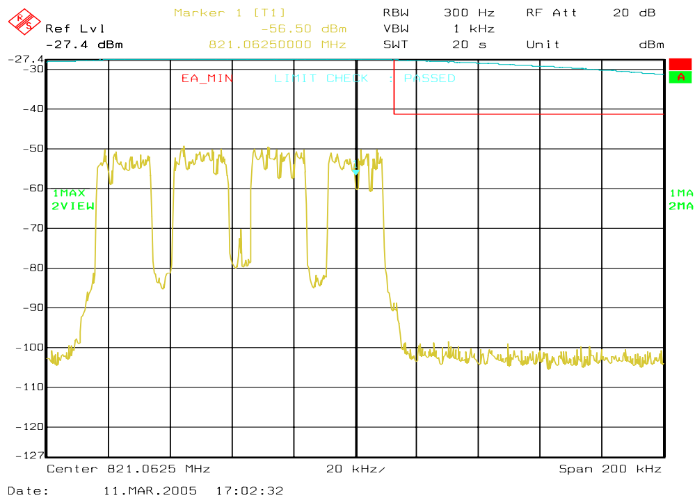
Figure 6a-53 . WiDEN100 800 MHz Band, QAM64, Minimum Power, EA Emission Mask
