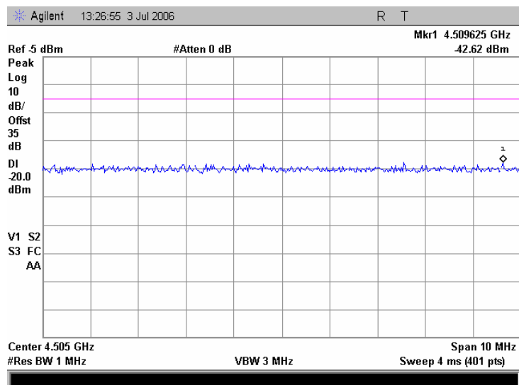
Plot 7.5.48 Conducted spurious emission measurements at the 5 th harmonic of high carrier frequency, iDEN 900
