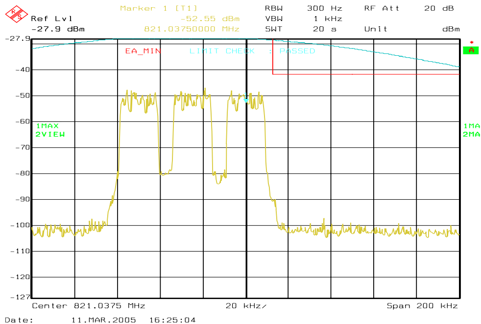
Figure 6a-45 . WiDEN75 800 MHz Band, QAM16, Minimum Power, EA Emission Mask
