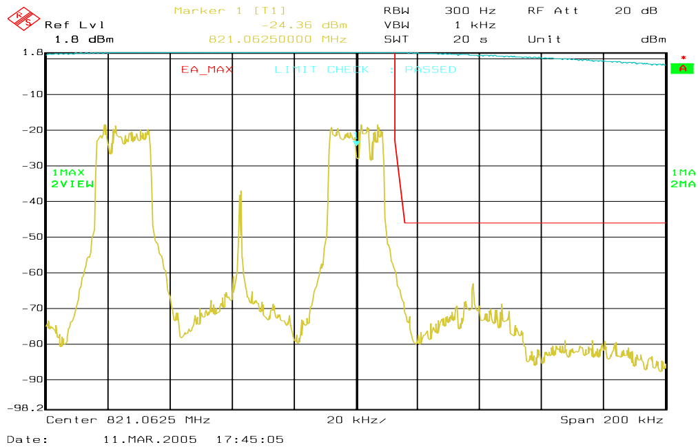
Figure 6a-58 . WiDEN_50_Split 800 MHz Band, QAM64, Maximum Power, EA Emission Mask
