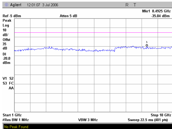
Plot 7.5.24 Spurious emission measurements in 1000 - 10000 MHz at high carrier frequency, iDEN 900
