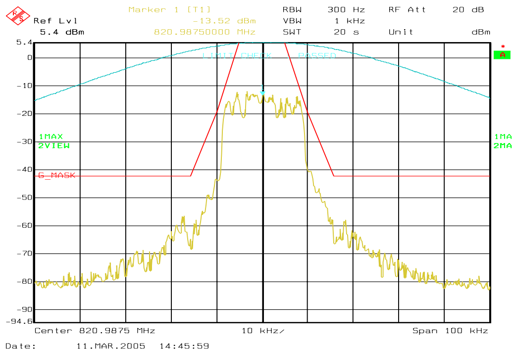
Figure 6a-28 . WiDEN25 800 MHz Band, QAM16, Maximum Power, Emission Mask G
