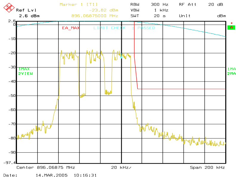
Figure 6a-72 . WiDEN75 900 MHz Band, Quad-QPSK, Maximum Power, EA Emission Mask
