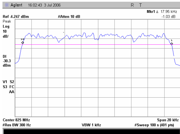
Plot 7.2.6 Occupied bandwidth test result at high frequency, iDEN 800
