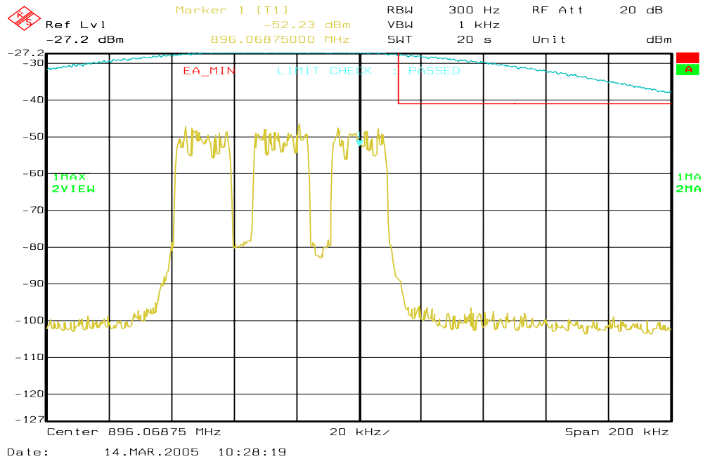
Figure 6a-75 . WiDEN75 900 MHz Band, QAM16, Minimum Power, EA Emission Mask
