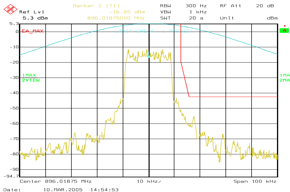
Figure 6a-22 . iDEN 900 MHz Band, QAM64, Maximum Power, EA Emission Mask
