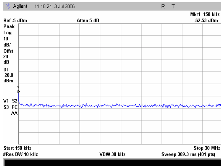
Plot 7.5.8 Spurious emission measurements in 0.15 - 30.0 MHz range at mid carrier frequency, iDEN 800
