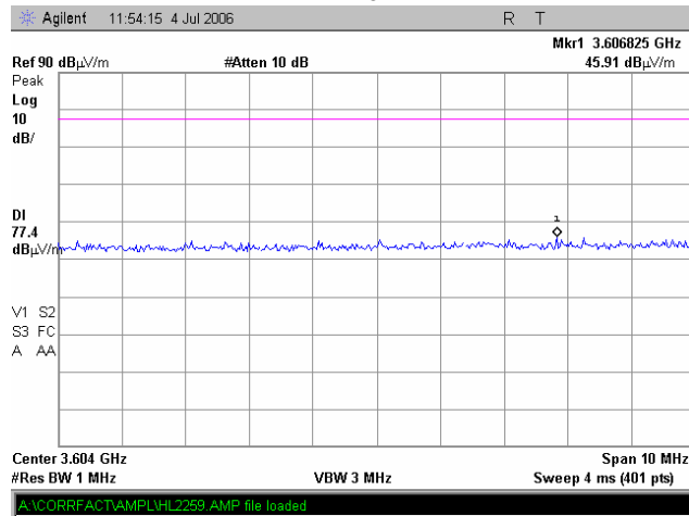
Plot 7.4.48 Radiated emission measurements at the 4 th harmonic iDEN 900
