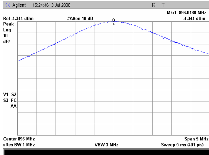
Plot 7.2.7 Reference peak power level at low frequency, iDEN 900
