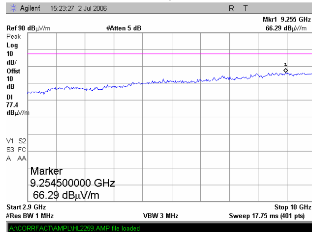
Plot 7.4.30 Radiated emission measurements in 2900 – 10000 MHz range
