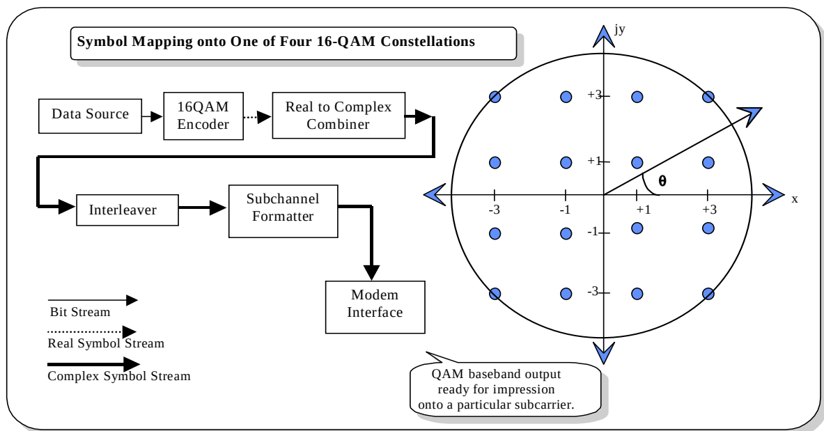
Figure 6a-4. Symbol Mapping onto One of Four 16-QAM Constellations
