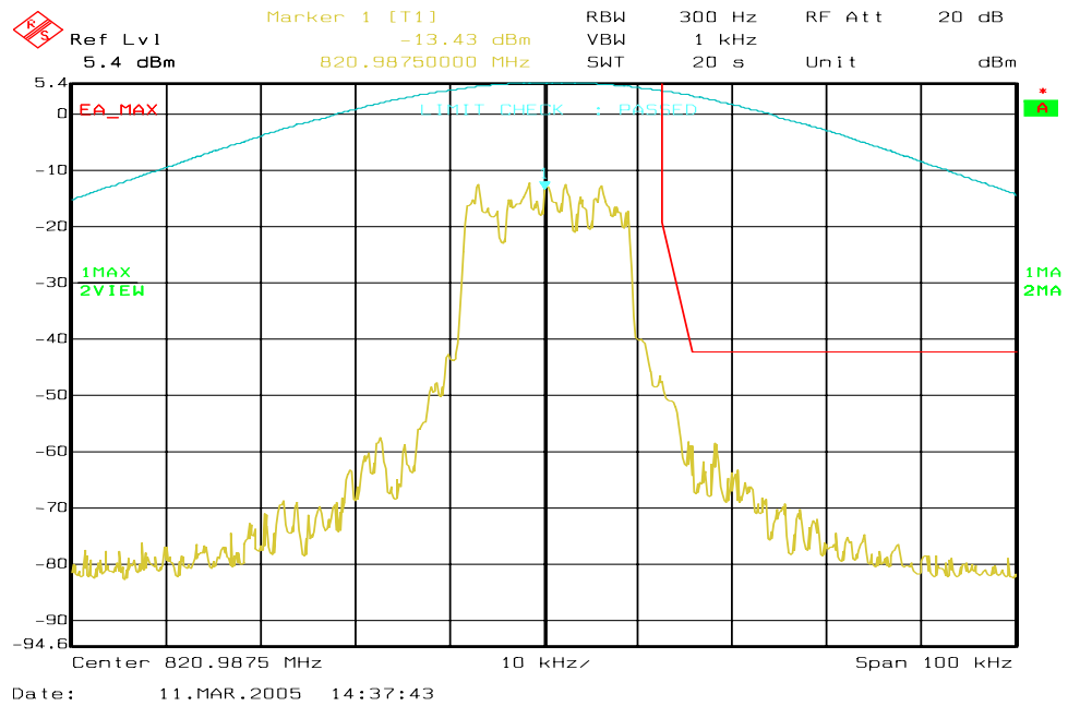
Figure 6a-26 . WiDEN25 800 MHz Band, Quad-QPSK, Maximum Power, EA Emission Mask
