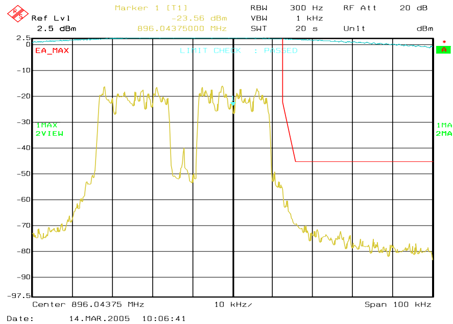
Figure 6a-66 . WiDEN50 900 MHz Band, Continuous Quad-QPSK, Maximum Power, EA Emission Mask
