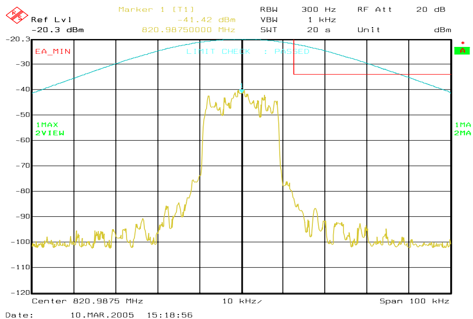
Figure 6a-17 . iDEN 800 MHz Band, QAM64, Minimum Power, EA Emission Mask
