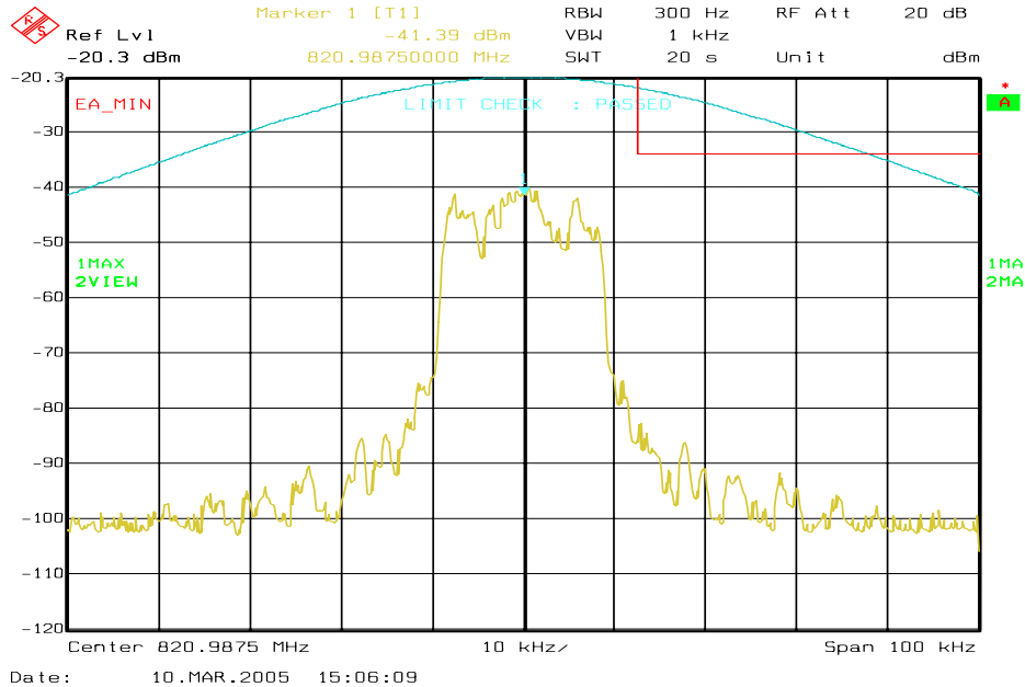
Figure 6a- 9. iDEN 800 MHz Band, QPSK, Minimum Power, EA Emission Mask
