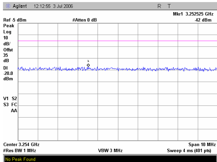
Plot 7.5.38 Conducted spurious emission measurements at the 4 th harmonic of mid carrier frequency, iDEN 800
