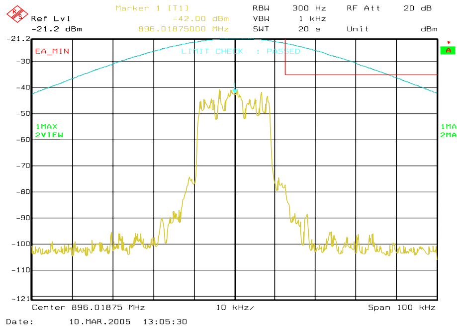
Figure 6a-21 . iDEN 900 MHz Band, QAM16, Minimum Power, EA Emission Mask
