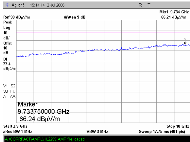
Plot 7.4.28 Radiated emission measurements in 2900 – 10000 MHz range
