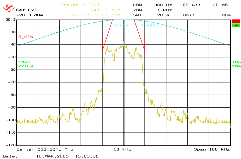
Figure 6a-7. iDEN 800 MHz Band, QPSK, Minimum Power, Emission Mask G
