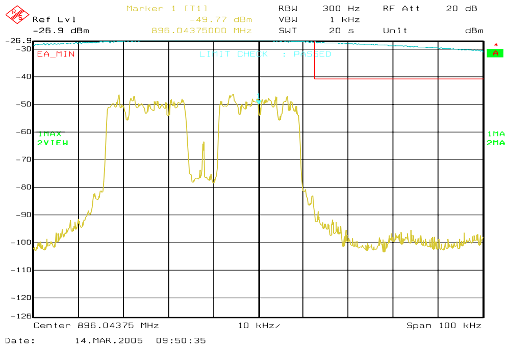
Figure 6a-71 . WiDEN50 900 MHz Band, Continuous QAM64, Minimum Power, EA Emission Mask
