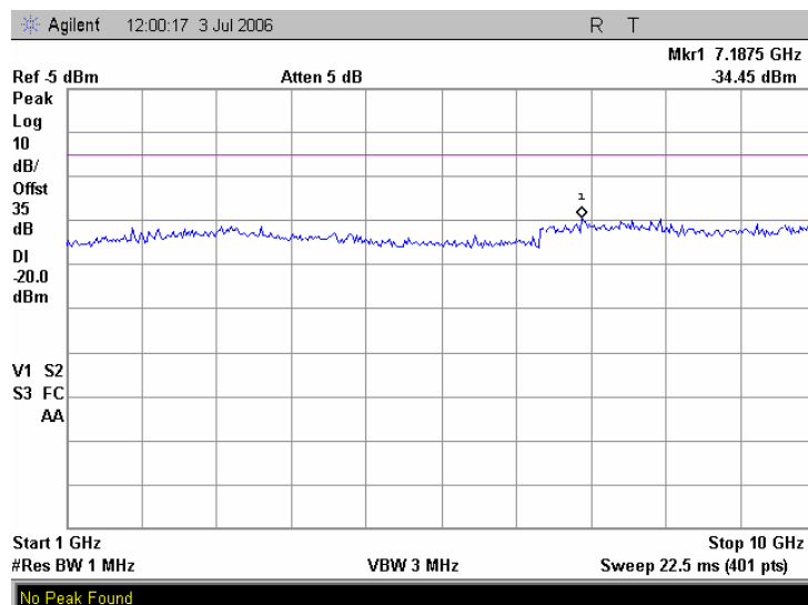
Plot 7.5.22 Spurious emission measurements in 1000 - 10000 MHz range at low carrier frequency, iDEN 900
