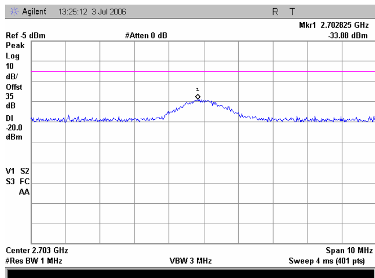
Plot 7.5.36 Conducted spurious emission measurements at the 3 rd harmonic of high carrier frequency, iDEN 900
