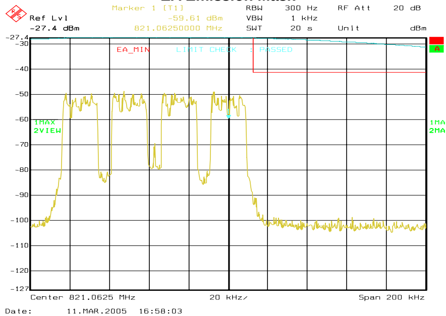
Figure 6a-49 . WiDEN100 800 MHz Band, Quad-QPSK, Minimum Power, EA Emission Mask
