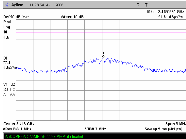
Plot 7.4.38 Radiated emission measurements at the 3 rd harmonic iDEN 800
