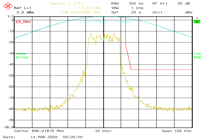
Figure 6a-60 . WiDEN25 900 MHz Band, Quad-QPSK, Maximum Power, EA Emission Mask
