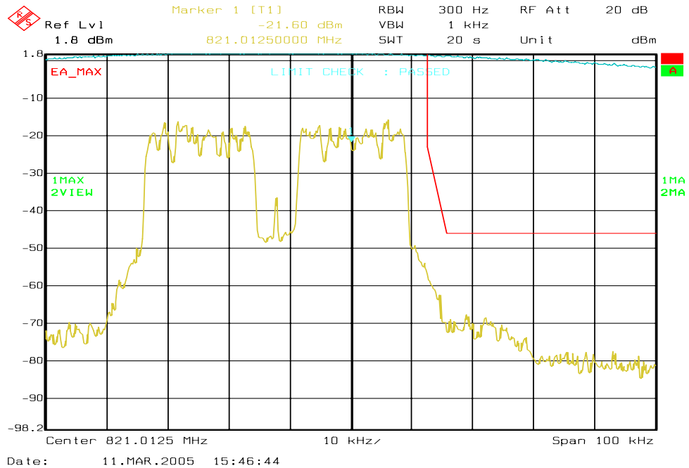
Figure 6a- 38. WiDEN50 800 MHz Band, Continuous QAM16, Maximum Power, EA Emission Mask
