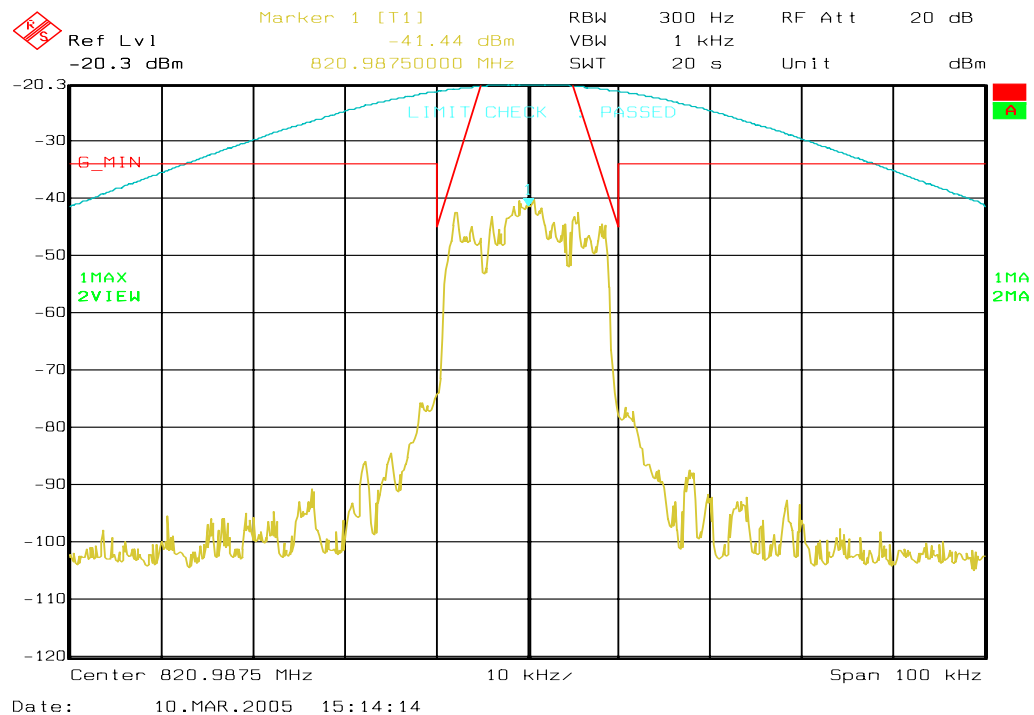
Figure 6a-15 . iDEN 800 MHz Band, QAM64, Minimum Power, Emission Mask G
