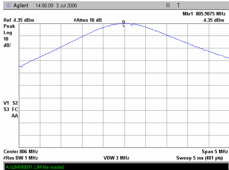
Plot 7.2.1 Reference peak power level at low frequency, iDEN 800
