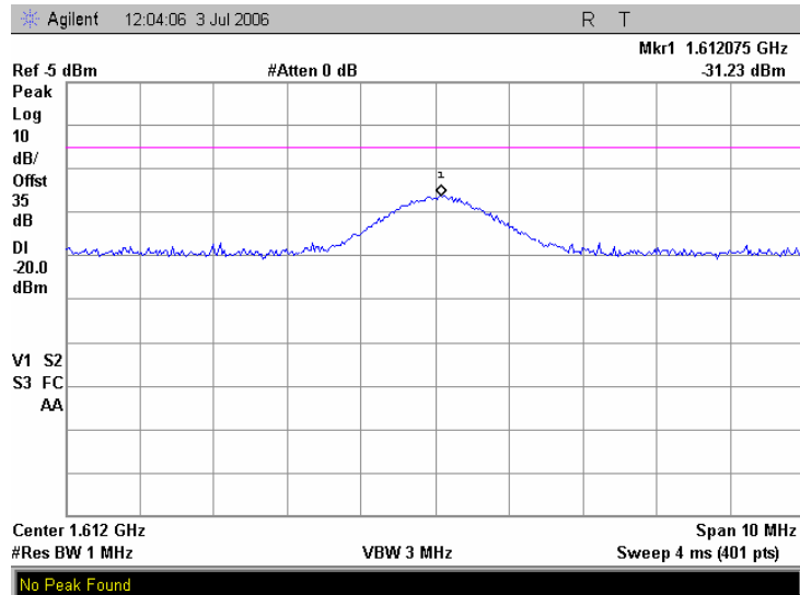
Plot 7.5.26 Conducted spurious emission measurements at the 2 nd harmonic of mid carrier frequency, iDEN 800
