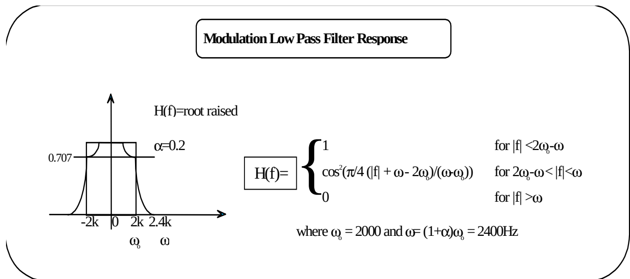
Figure 6a-1: Modulation Low Pass Filter Response
