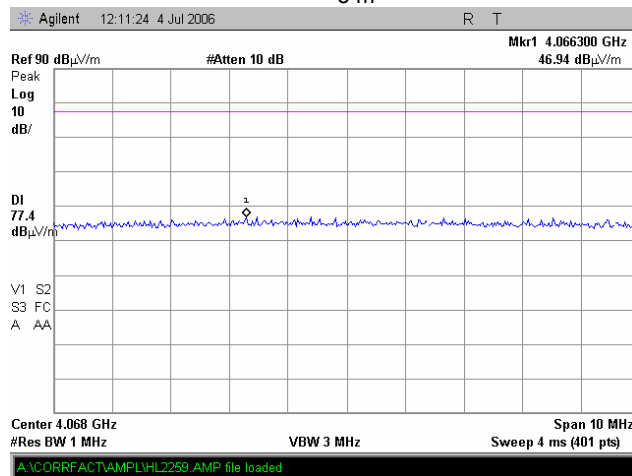
Plot 7.4.50 Radiated emission measurements at the 5 th harmonic iDEN 800
