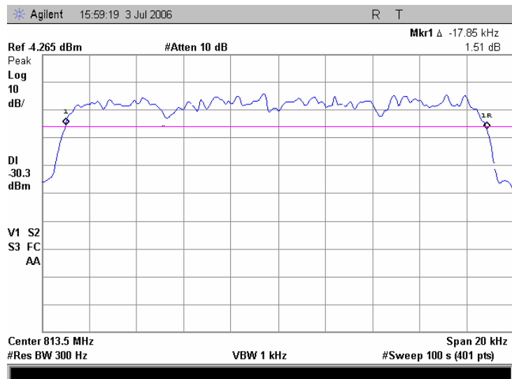
Plot 7.2.4 Occupied bandwidth test result at mid frequency, iDEN 800
