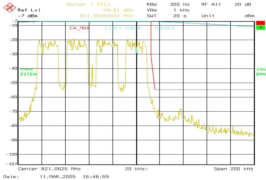
Figure 6a-48 . WiDEN100 800 MHz Band, Quad-QPSK, Maximum Power, EA Emission Mask
