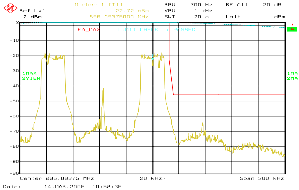
Figure 6a-88 . WiDEN_50_Split 900 MHz Band, QAM64, Maximum Power, EA Emission Mask
