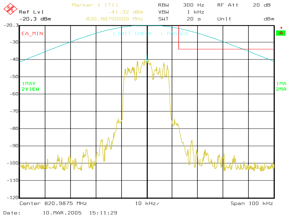
Figure 6a-13 . iDEN 800 MHz Band, QAM16, Minimum Power, EA Emission Mask
