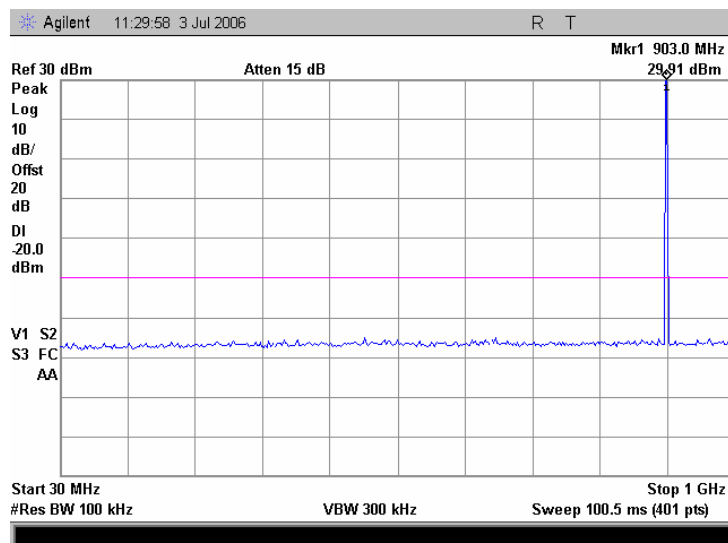
Plot 7.5.18 Spurious emission measurements in 30.0 - 1000 MHz range at high carrier frequency, iDEN 900
