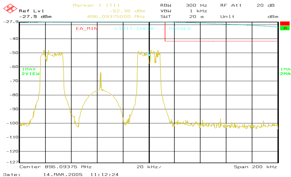
Figure 6a-89 . WiDEN_50_Split 900 MHz Band, QAM64, Minimum Power, EA Emission Mask
