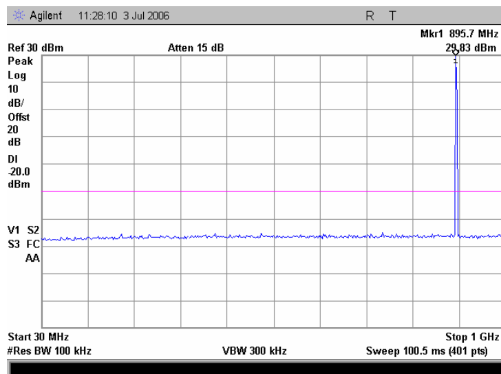
Plot 7.5.16 Spurious emission measurements in 30.0 - 1000 MHz range at low carrier frequency, iDEN 900
