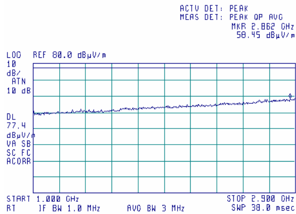
Plot 7.4.24 Radiated emission measurements in 1000 – 2900 MHz range
