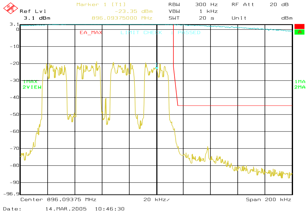
Figure 6a-80 . WiDEN100 900 MHz Band, QAM16, Maximum Power, EA Emission Mask
