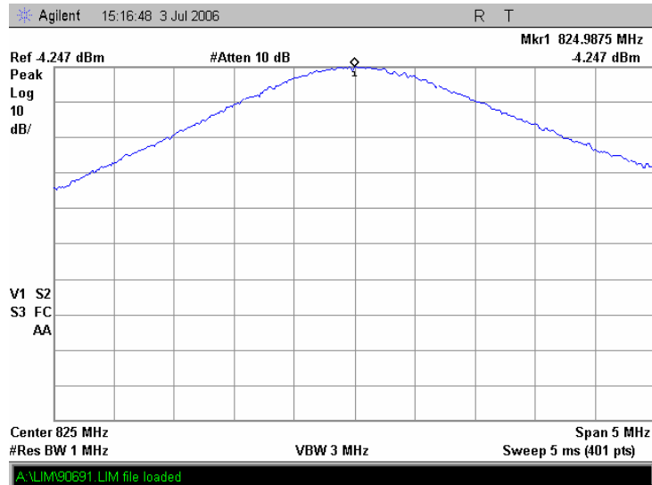
Plot 7.2.5 Reference peak power level at high frequency, iDEN 800
