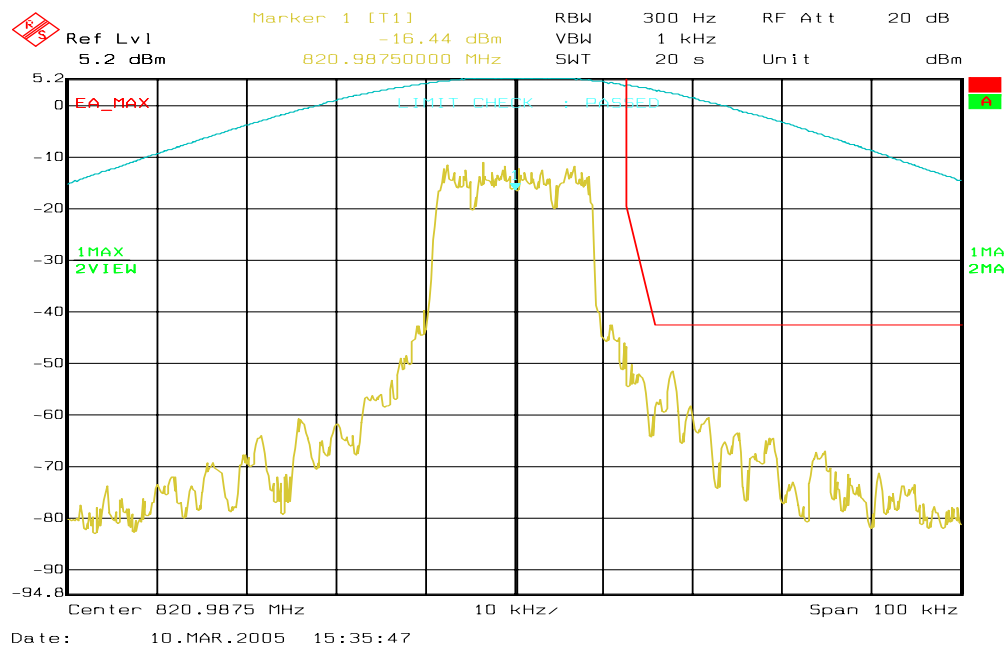
Figure 6a-12 . iDEN 800 MHz Band, QAM16, Maximum Power, EA Emission Mask
