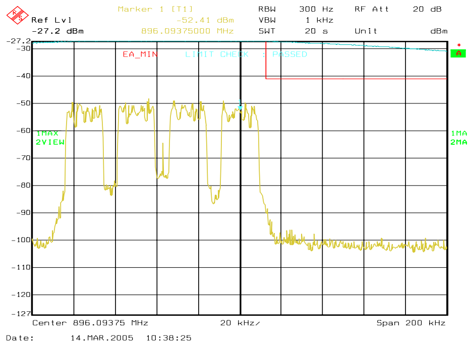
Figure 6a-81 . WiDEN100 900 MHz Band, QAM16, Minimum Power, EA Emission Mask
