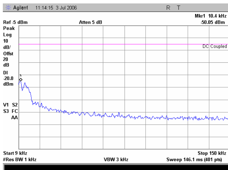
Plot 7.5.4 Spurious emission measurements in 9 - 150 kHz range at low carrier frequency, iDEN 900
