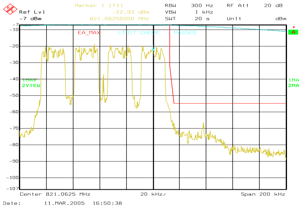
Figure 6a-50 . WiDEN100 800 MHz Band, QAM16, Maximum Power, EA Emission Mask
