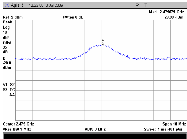
Plot 7.5.33 Conducted spurious emission measurements at the 3 rd harmonic of high carrier frequency, iDEN 800
