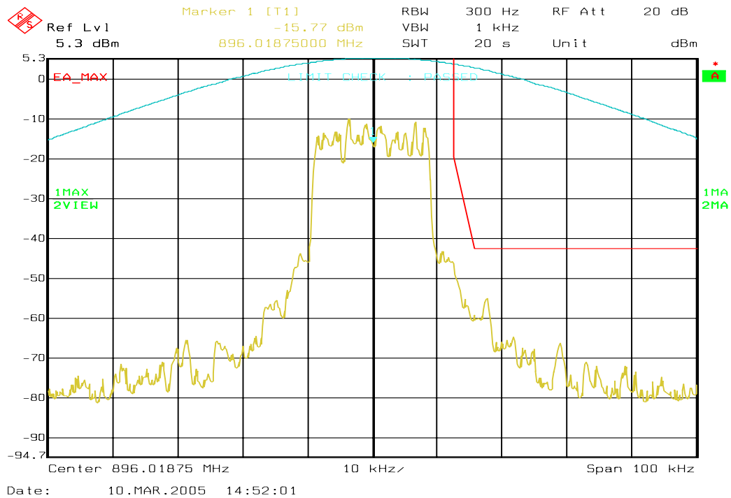
Figure 6a-20 . iDEN 900 MHz Band, QAM16, Maximum Power, EA Emission Mask
