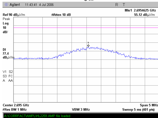
Plot 7.4.42 Radiated emission measurements at the 3 rd harmonic iDEN 900
