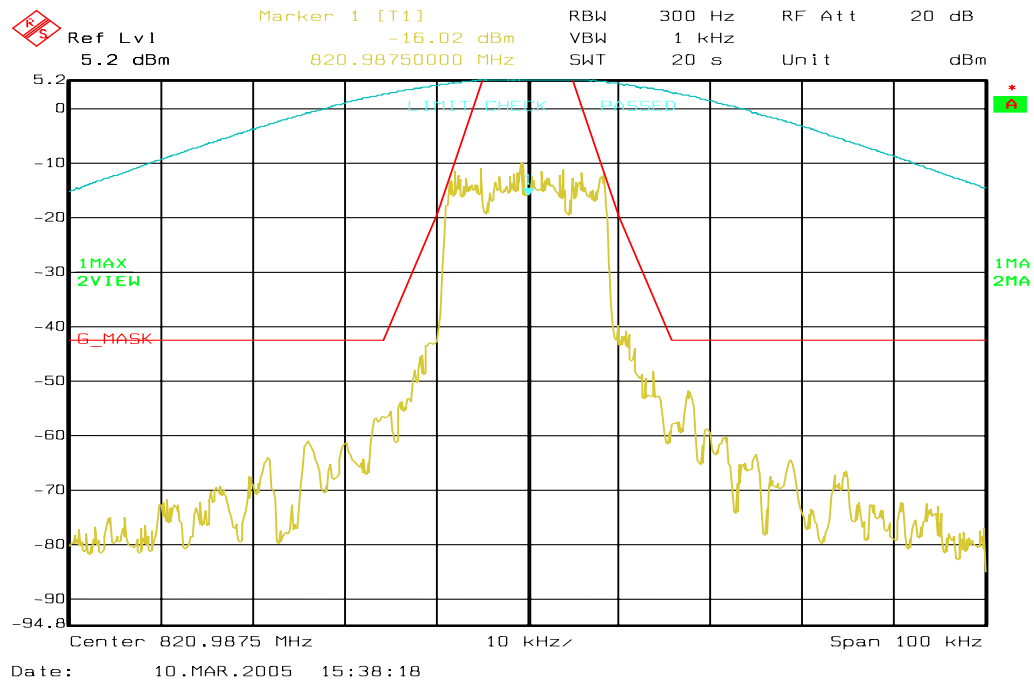
Figure 6a-14 . iDEN 800 MHz Band, QAM64, Maximum Power, Emission Mask G
