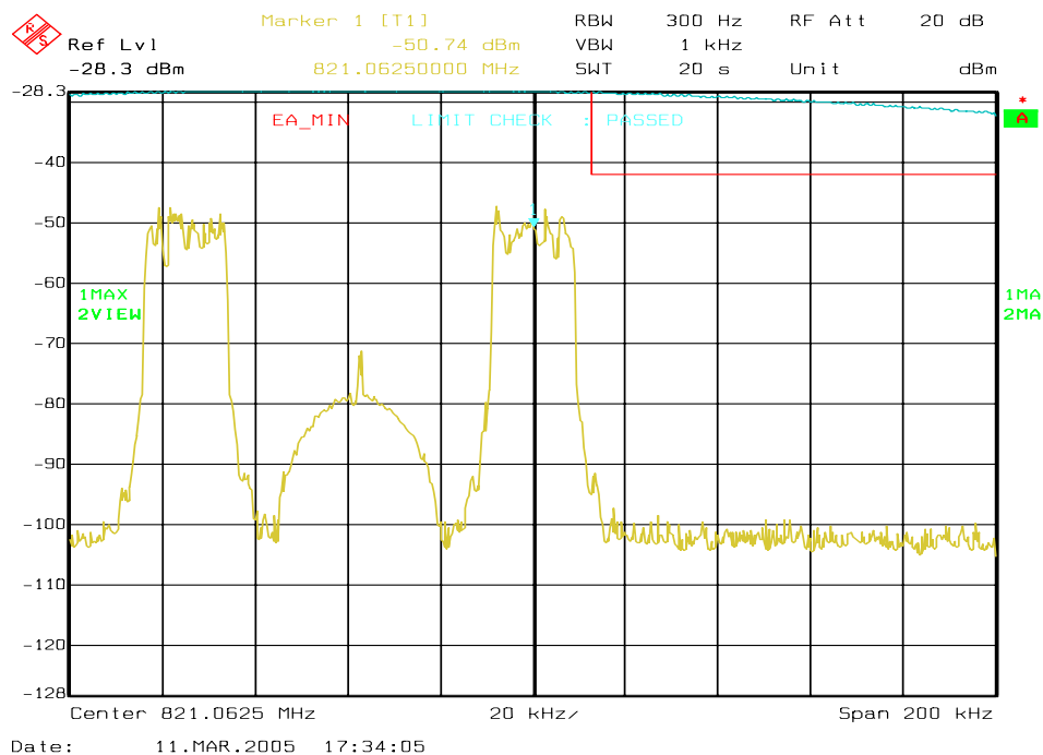
Figure 6a-57 . WiDEN_50_Split 800 MHz Band, QAM16, Minimum Power, EA Emission Mask
