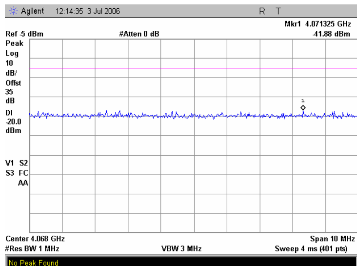
Plot 7.5.44 Conducted spurious emission measurements at the 5 th harmonic of mid carrier frequency, iDEN 800
