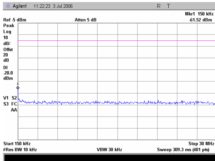
Plot 7.5.12 Spurious emission measurements in 0.15 - 30.0 MHz range at high carrier frequency, iDEN 900
