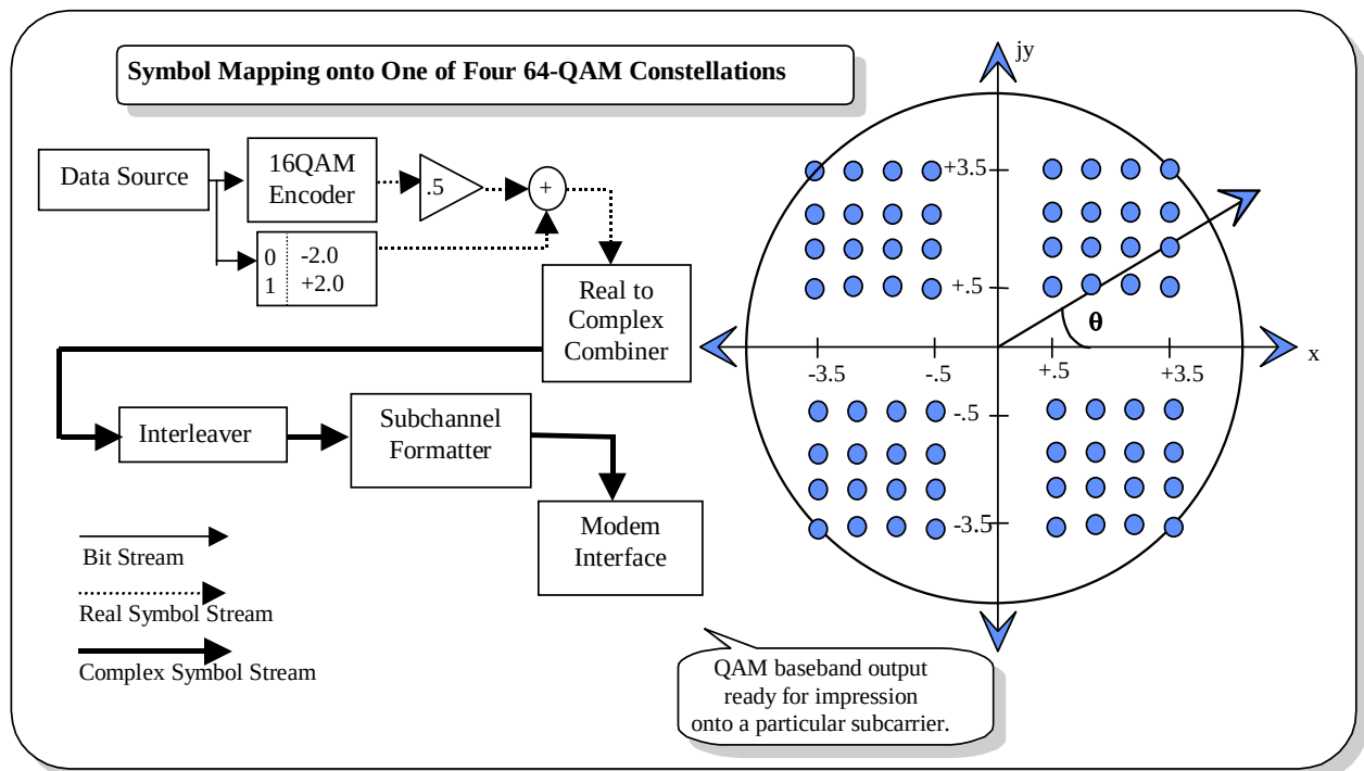
Figure 6a-5. Symbol Mapping onto One of Four 64-QAM Constellations
