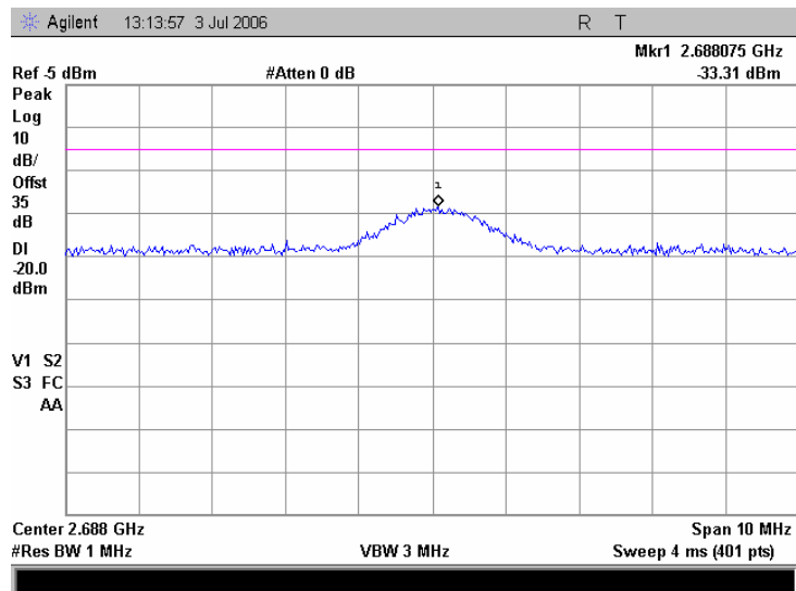
Plot 7.5.34 Conducted spurious emission measurements at the 3 rd harmonic of low carrier frequency, iDEN 900
