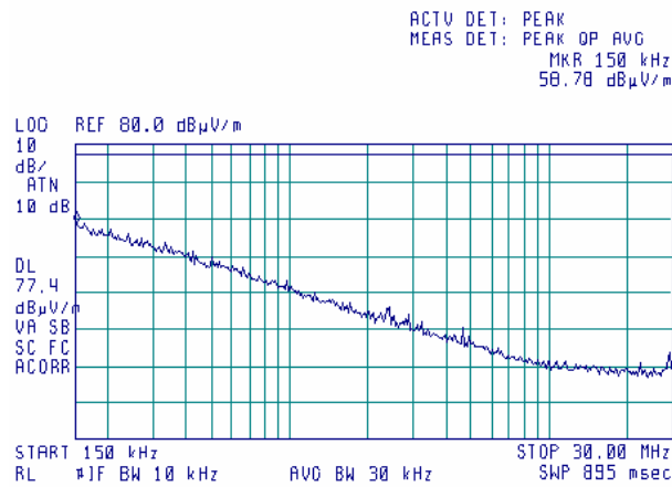
Plot 7.4.10 Radiated emission measurements in 0.15 - 30 MHz range
