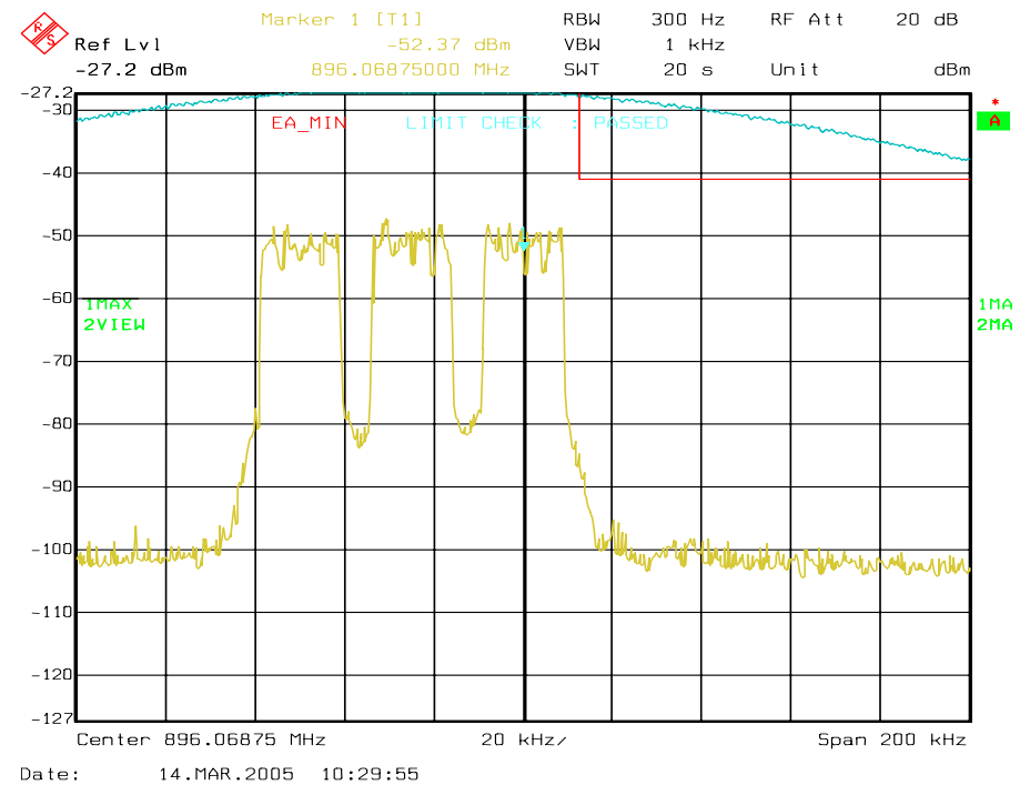
Figure 6a-77 . WiDEN75 900 MHz Band, QAM64, Minimum Power, EA Emission Mask
