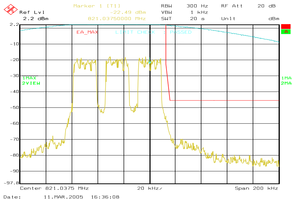
Figure 6a-46 . WiDEN75 800 MHz Band, QAM64, Maximum Power, EA Emission Mask
