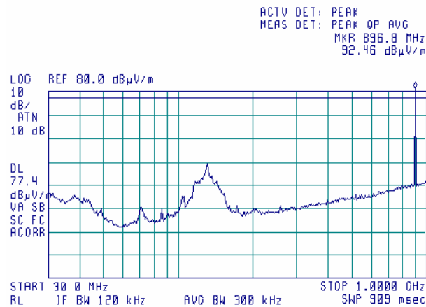
Plot 7.4.18 Radiated emission measurements in 30 - 1000 MHz range
