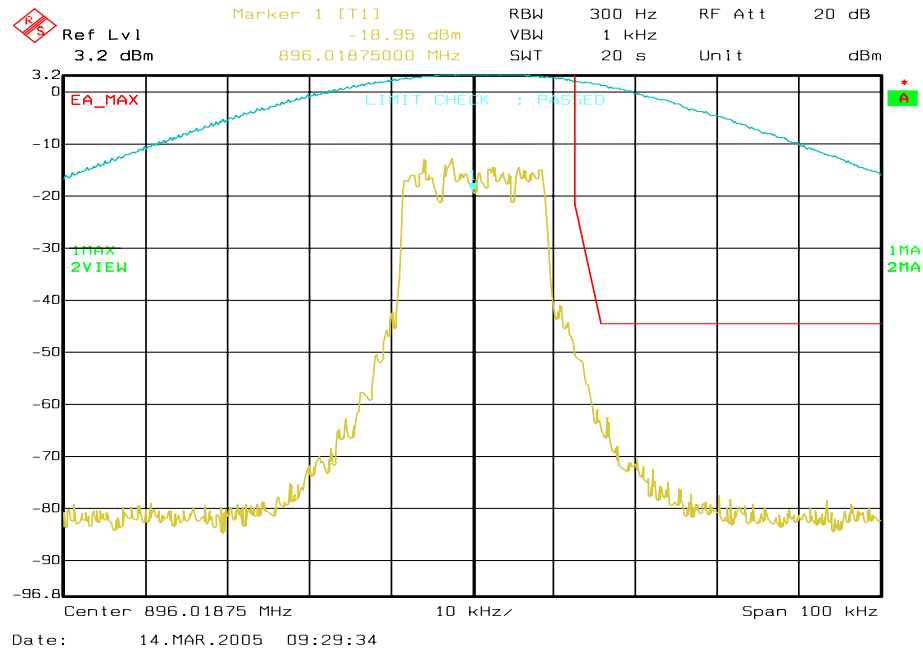
Figure 6a-64 . WiDEN25 900 MHz Band, QAM64, Maximum Power, EA Emission Mask
