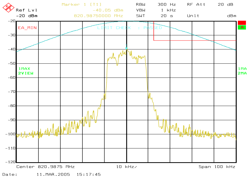
Figure 6a-35 . WiDEN25 800 MHz Band, QAM64, Minimum Power, EA Emission Mask
