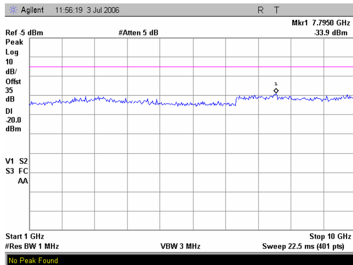
Plot 7.5.20 Spurious emission measurements in 1000 - 10000 MHz at mid carrier frequency, iDEN 800
