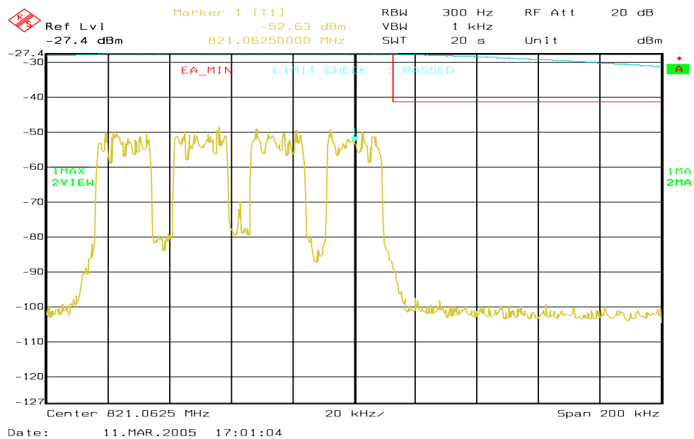
Figure 6a-51 . WiDEN100 800 MHz Band, QAM16, Minimum Power, EA Emission Mask
