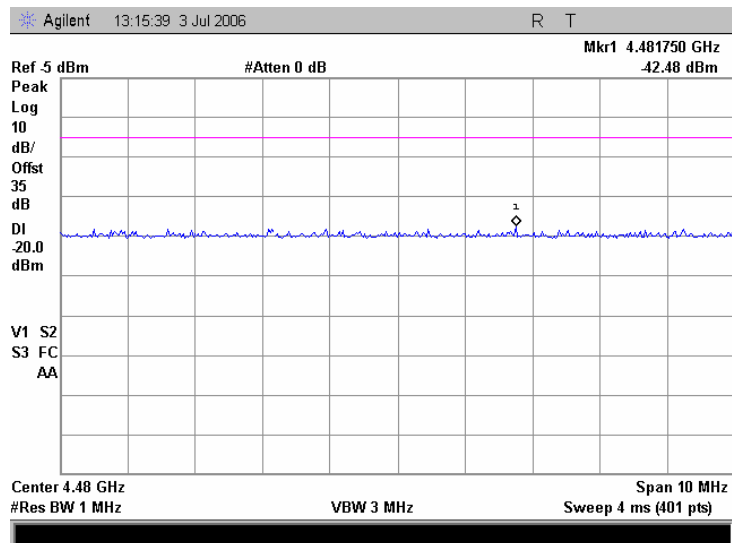
Plot 7.5.46 Conducted spurious emission measurements at the 5 th harmonic of low carrier frequency, iDEN 900
