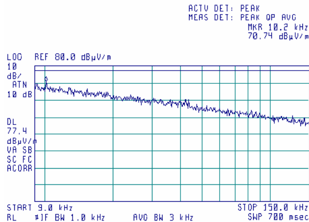
Plot 7.4.6 Radiated emission measurements in 9 - 150 kHz range
