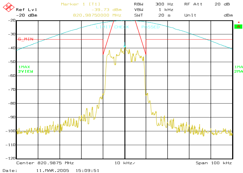
Figure 6a-25 . WiDEN25 800 MHz Band, Quad-QPSK, Minimum Power, Emission Mask G
