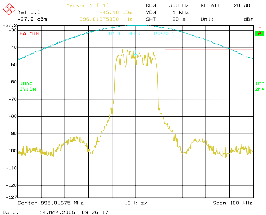
Figure 6a-63 . WiDEN25 900 MHz Band, QAM16, Minimum Power, EA Emission Mask
