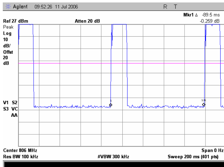
Plot 7.1.1 TDM period at iDEN 800
