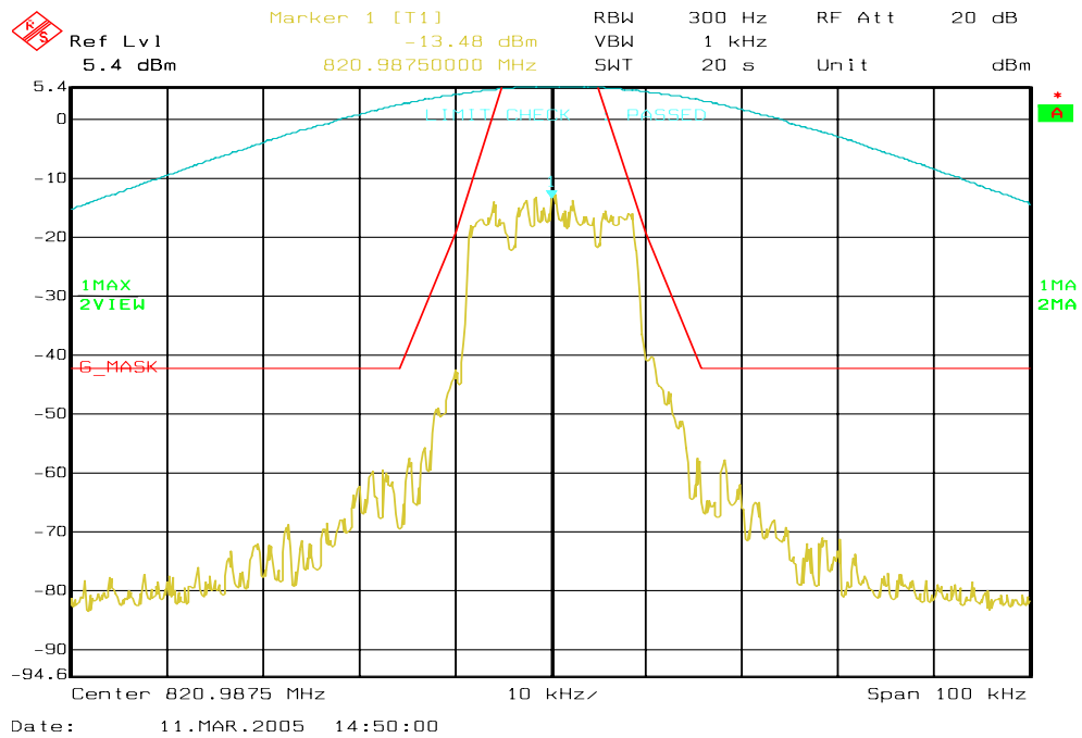
Figure 6a-32 . WiDEN25 800 MHz Band, QAM64, Maximum Power, Emission Mask G
