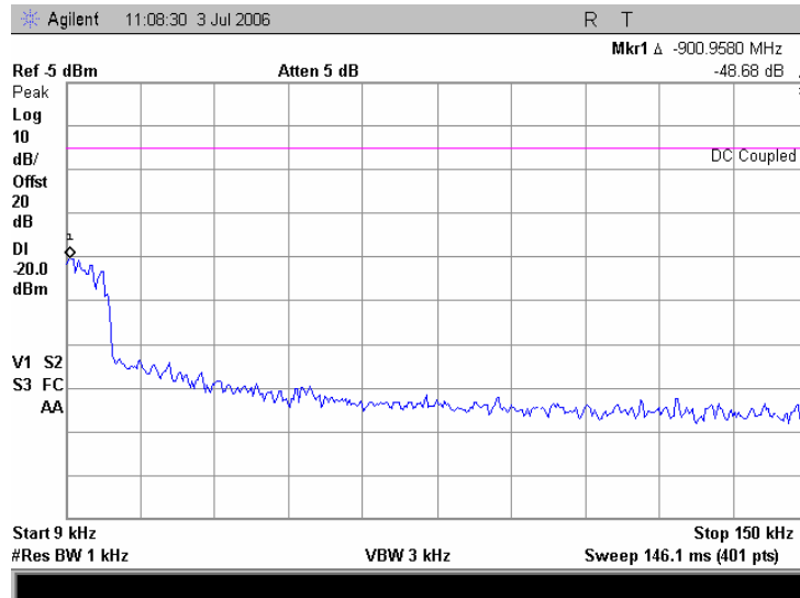
Plot 7.5.2 Spurious emission measurements in 9 - 150 kHz range at mid carrier frequency, iDEN 800
