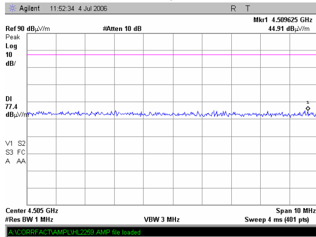
Plot 7.4.54 Radiated emission measurements at the 5 th harmonic iDEN 900
