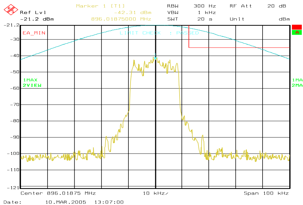
Figure 6a-23 . iDEN 900 MHz Band, QAM64, Minimum Power, EA Emission Mask
