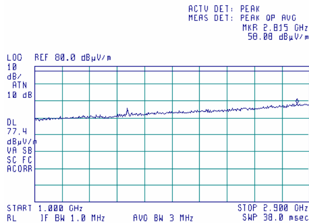
Plot 7.4.22 Radiated emission measurements in 1000 – 2900 MHz range
