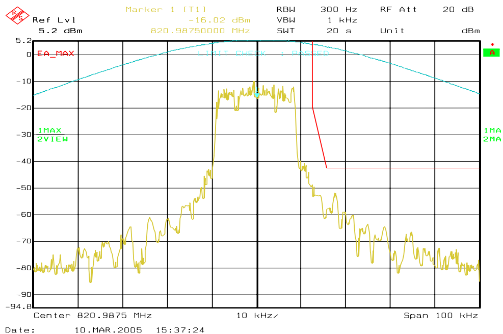
Figure 6a-16 . iDEN 800 MHz Band, QAM64, Maximum Power, EA Emission Mask
