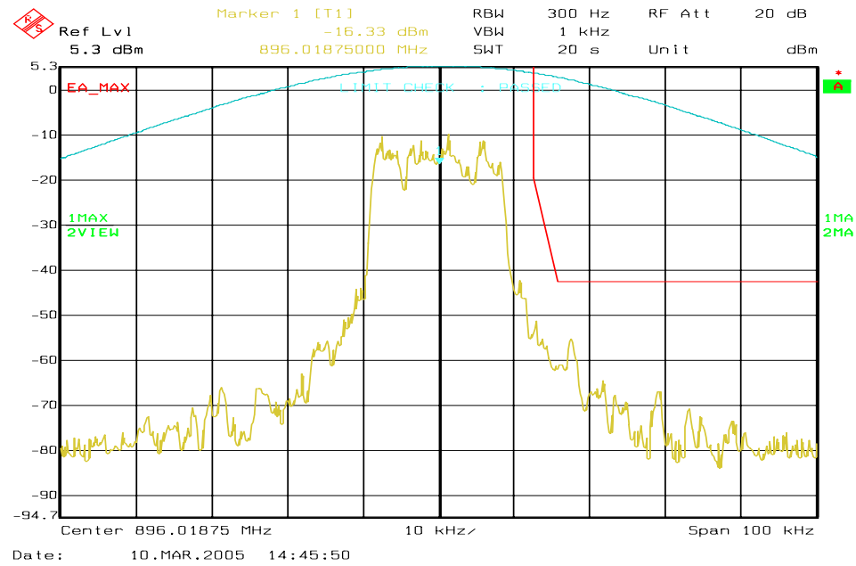
Figure 6a-18 . iDEN 900 MHz Band, Quad-QPSK, Maximum Power, EA Emission Mask
