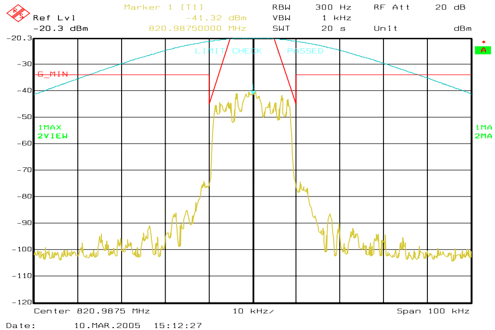
Figure 6a-11 . iDEN 800 MHz Band, QAM16, Minimum Power, Emission Mask G
