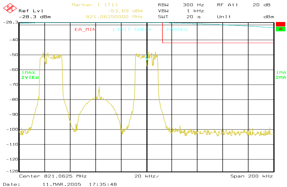
Figure 6a-59 . WiDEN_50_Split 800 MHz Band, QAM64, Minimum Power, EA Emission Mask
