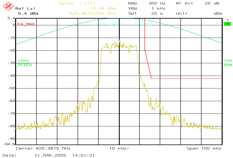
Figure 6a-34 . WiDEN25 800 MHz Band, QAM64, Maximum Power, EA Emission Mask
