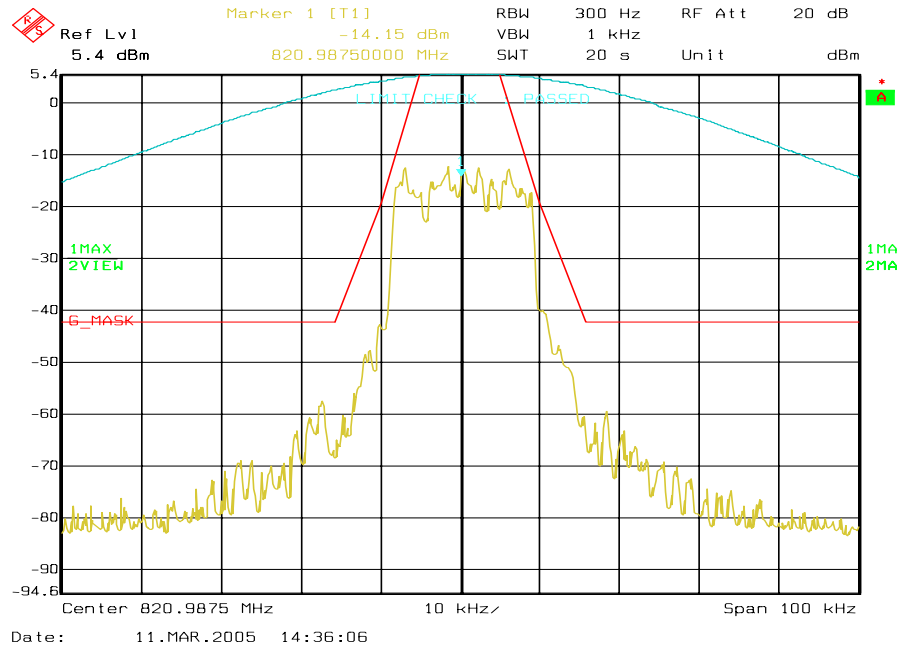
Figure 6a-24 . WiDEN25 800 MHz Band, Quad-QPSK, Maximum Power, Emission Mask G
