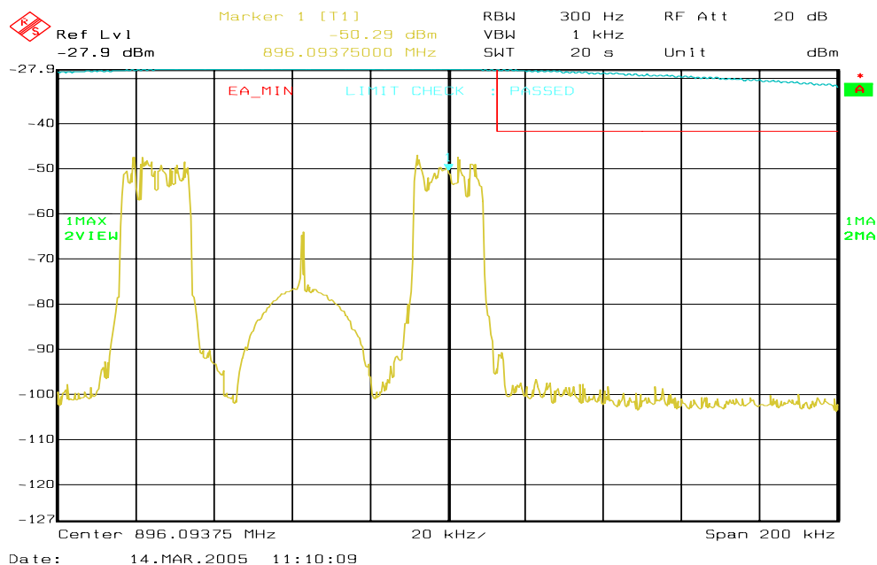
Figure 6a-87 . WiDEN_50_Split 900 MHz Band, QAM16, Minimum Power, EA Emission Mask
