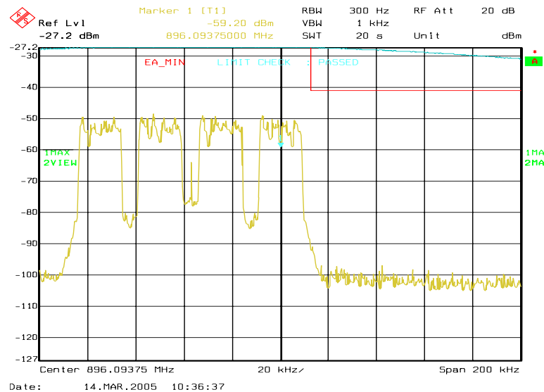
Figure 6a-79 . WiDEN100 900 MHz Band, Quad-QPSK, Minimum Power, EA Emission Mask
