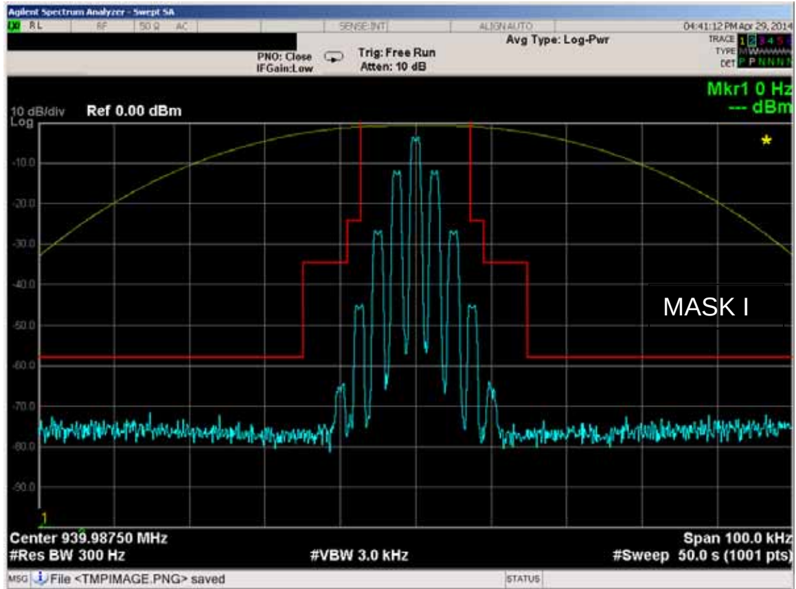
Figure 6E-41: 939.9875 MHz, 12.5 kHz Channel Spacing, 2500Hz Audio and DPL Tone Modulation, 11K0F3E Mask I
