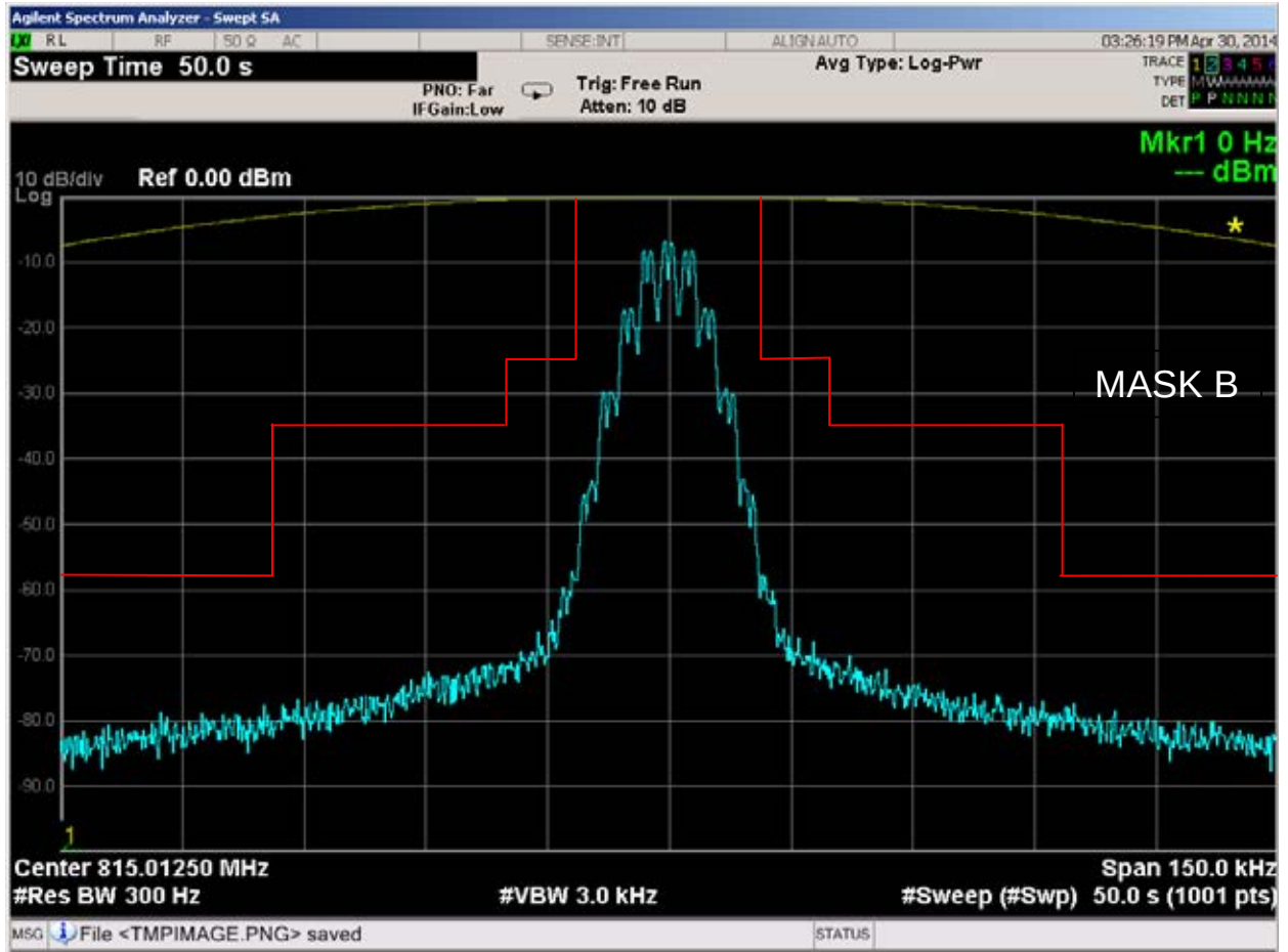
Figure 6E-14: 815.0125 MHz, 25 kHz Channel Spacing, 2000/3000 Hz FSK Data and TPL Tone Modulation, 16K0F3E Mask B
