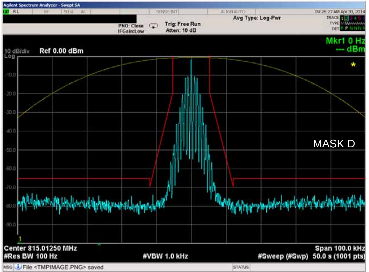
Figure 6E-25: 815.0125 MHz, 12.5 kHz Channel Spacing, DTMF Modulation only, 11K0F3E Mask D
