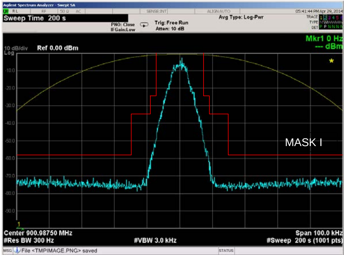
Figure 6E-57: 900.9875 MHz, 4-Level FSK Data Modulation only, 7K60FXD Mask I
