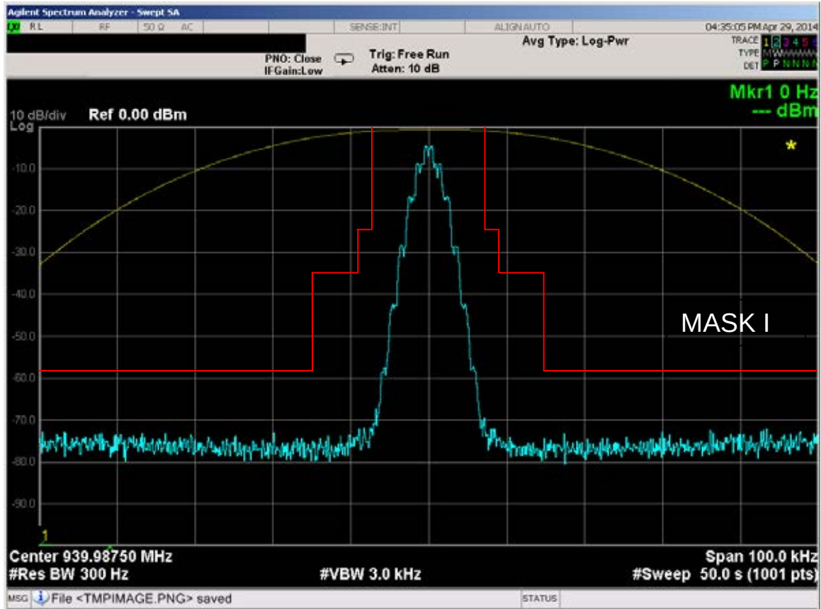
Figure 6E-47: 939.9875 MHz, 12.5 kHz Channel Spacing, DTMF and DPL Tone Modulation, 11K0F3E Mask I
