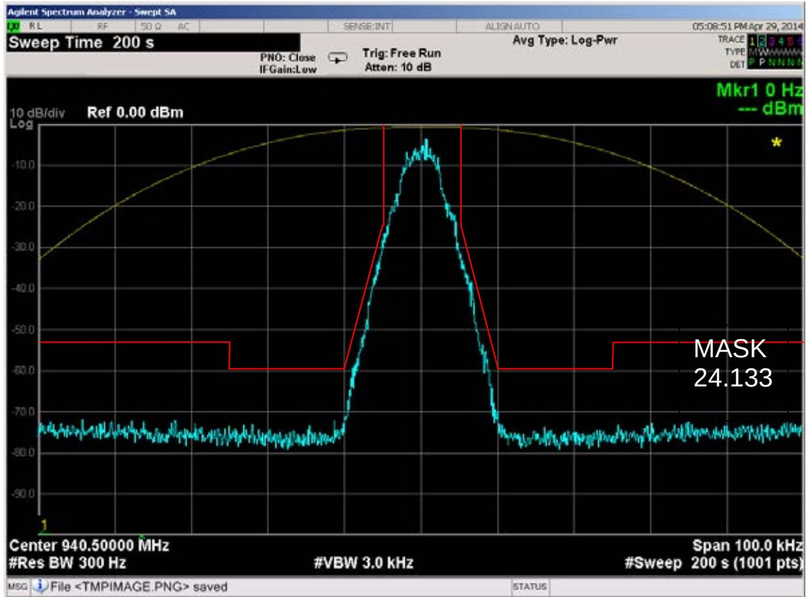
Figure 6E-66: 940.5 MHz, 9W, 4-Level FSK Voice and Data Modulation, 7K60F1W Mask 24.133
