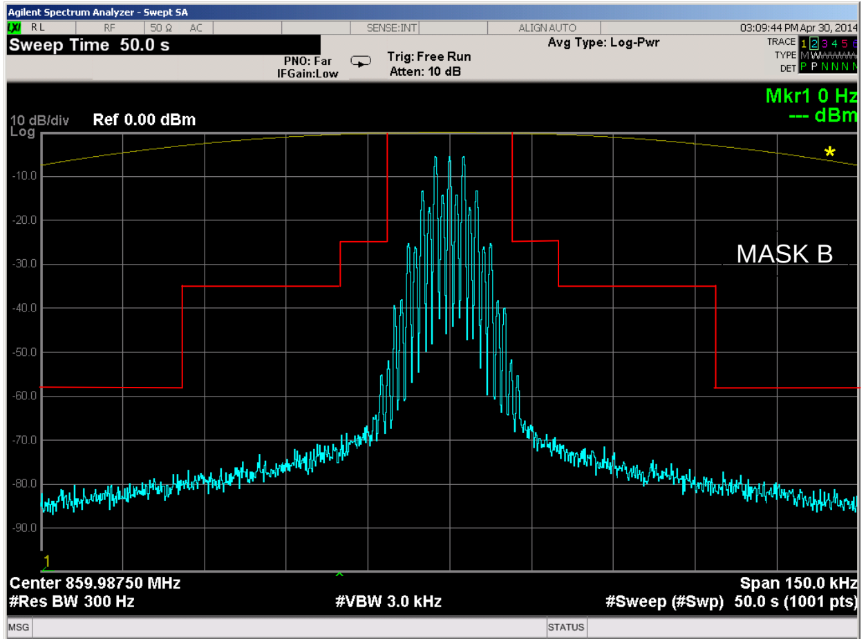
Figure 6E-18: 859.9875 MHz, 25 kHz Channel Spacing, 2000/3000 Hz FSK Data Modulation Only, 16K0F3E Mask B
