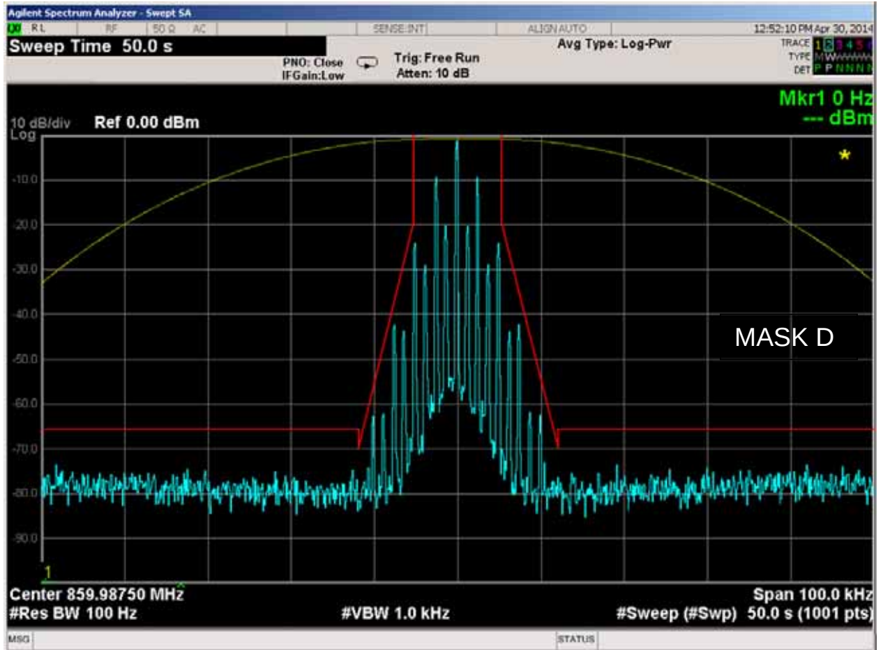
Figure 6E-34: 859.9875 MHz, 12.5 kHz Channel Spacing, 2000/3000 Hz FSK Data Modulation Only, 11K0F3E Mask D
