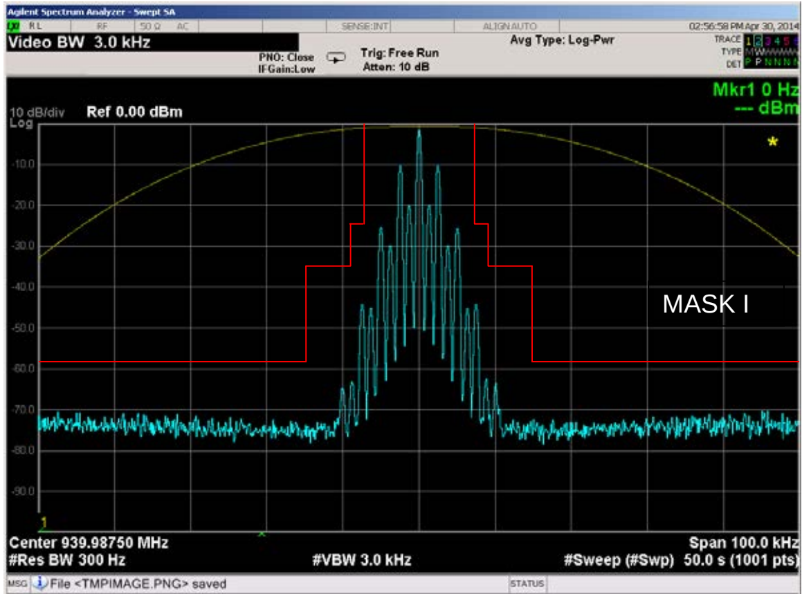
Figure 6E-52: 939.9875 MHz, 12.5 kHz Channel Spacing, 2000/3000 Hz FSK Data Modulation Only, 11K0F3E Mask I
