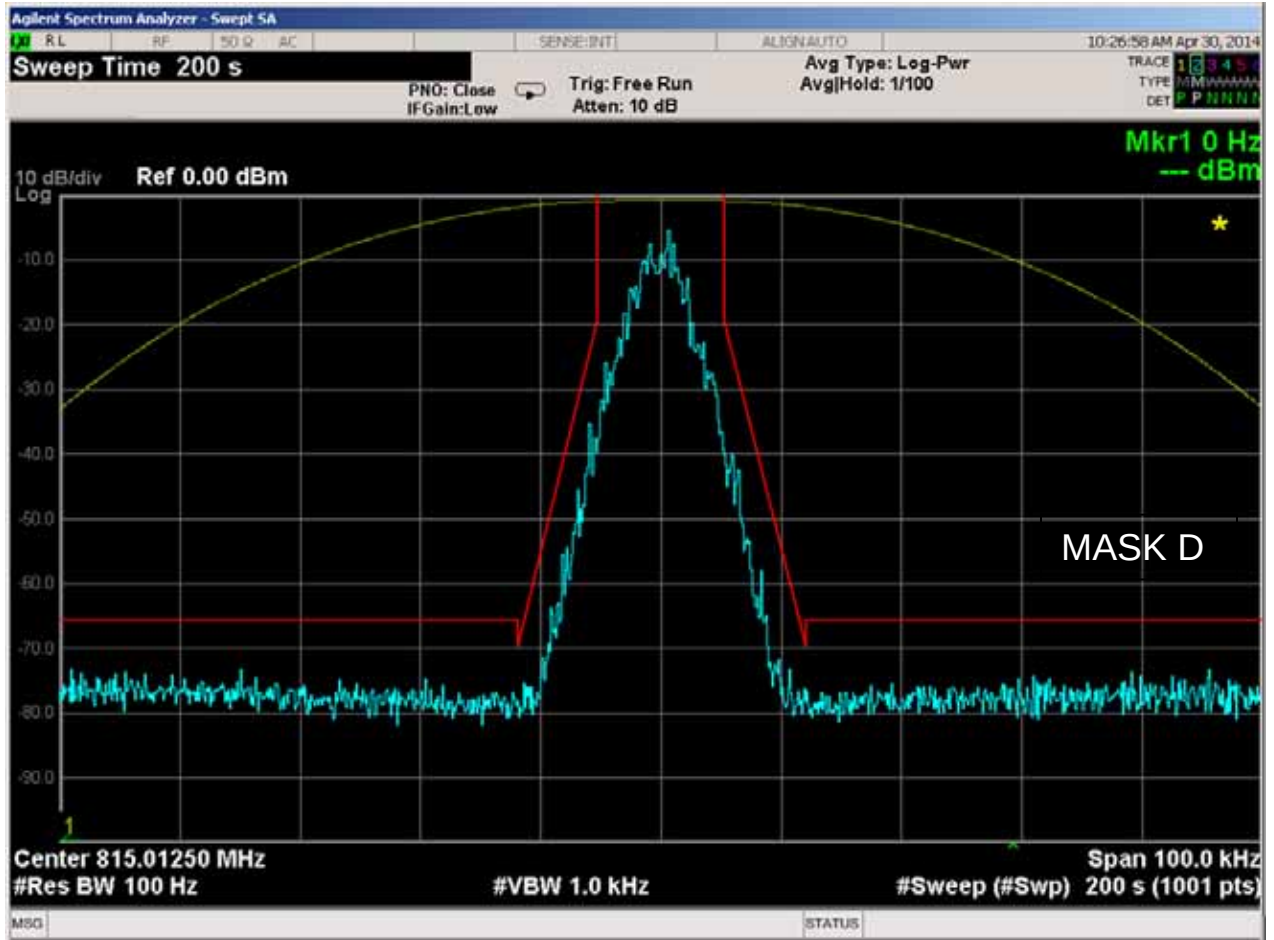
Figure 6E-55: 815.0125 MHz, 4-Level FSK Data Modulation only, 7K60FXD Mask D
