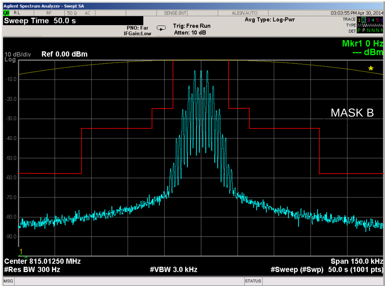
Figure 6E-13: 815.0125 MHz, 25 kHz Channel Spacing, 2000/3000 Hz FSK Data and DPL Tone Modulation, 16K0F3E Mask B
