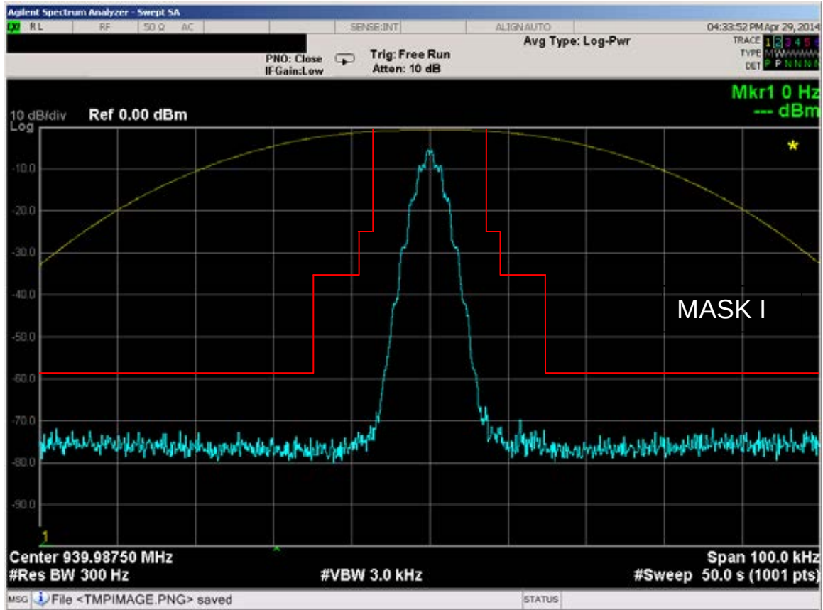
Figure 6E-48: 939.9875 MHz, 12.5 kHz Channel Spacing, DTMF and TPL Tone Modulation, 11K0F3E Mask I
