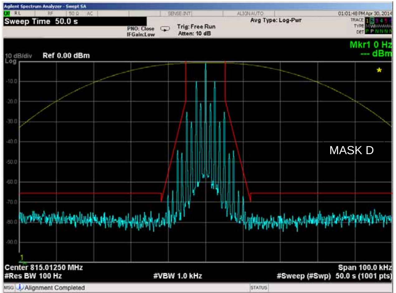
Figure 6E-31: 815.0125 MHz, 12.5 kHz Channel Spacing, 2000/3000 Hz FSK Data Modulation Only, 11K0F3E Mask D
