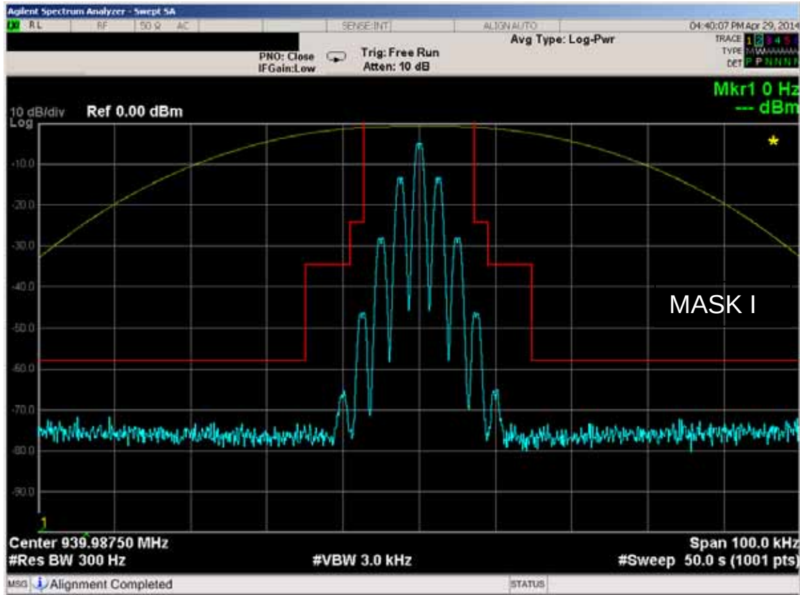
Figure 6E-42: 939.9875 MHz, 12.5 kHz Channel Spacing, 2500Hz Audio and TPL Tone Modulation, 11K0F3E Mask I
