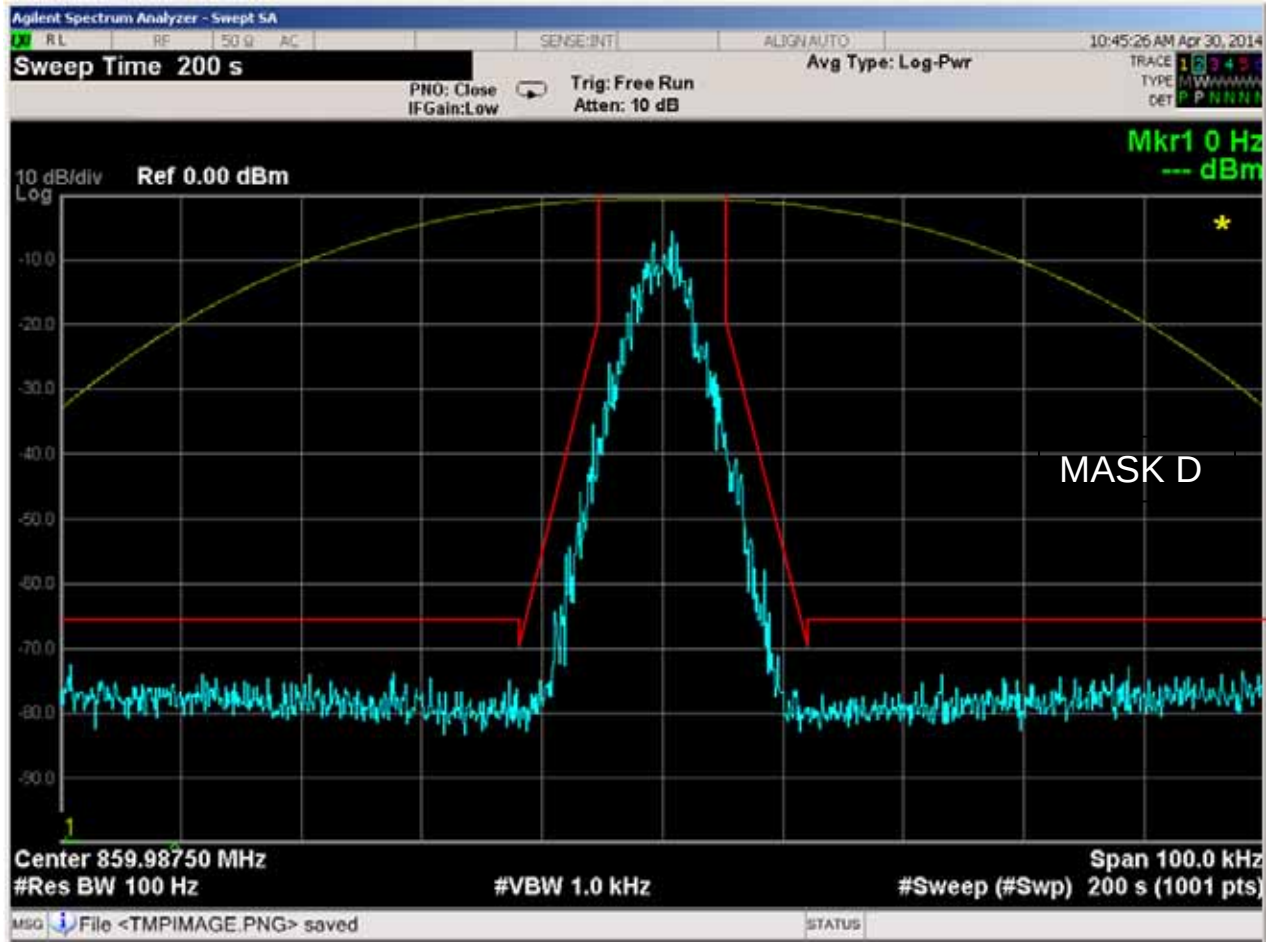
Figure 6E-68: 859.9875 MHz, 4-Level FSK Voice Modulation only, 7K60F1E Mask D
