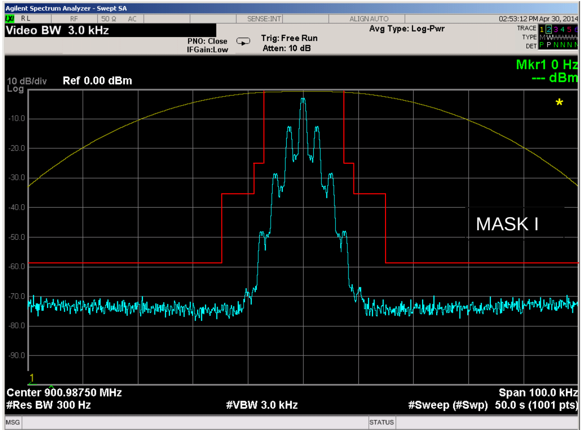
Figure 6E-51: 900.9875 MHz, 12.5 kHz Channel Spacing, 2000/3000 Hz FSK Data and TPL Tone Modulation, 11K0F3E Mask I
