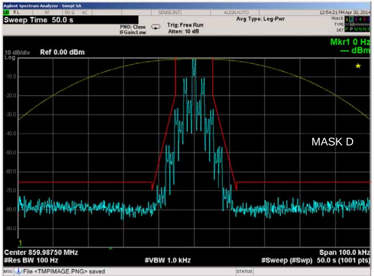
Figure 6E-35: 859.9875 MHz, 12.5 kHz Channel Spacing, 2000/3000 Hz FSK Data and DPL Tone Modulation, 11K0F3E Mask D
