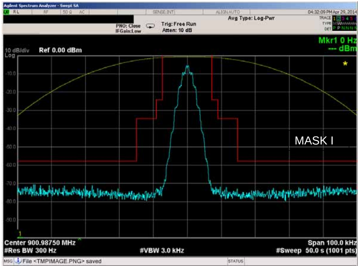
Figure 6E-45: 900.9875 MHz, 12.5 kHz Channel Spacing, DTMF and TPL Tone Modulation, 11K0F3E Mask I
