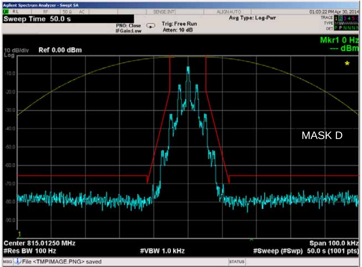
Figure 6E-33: 815.0125 MHz, 12.5 kHz Channel Spacing, 2000/3000 Hz FSK Data and TPL Tone Modulation, 11K0F3E Mask D
