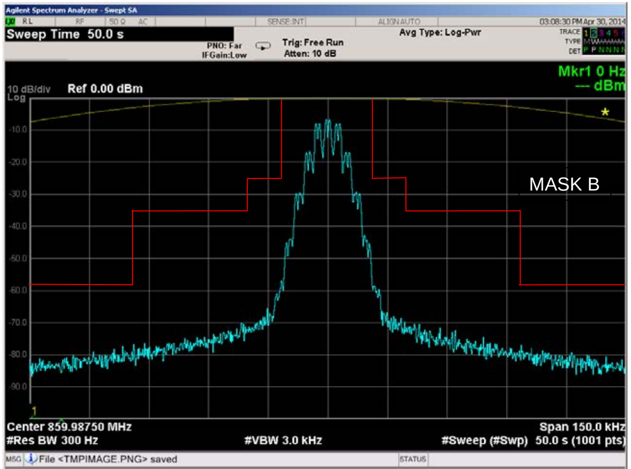
Figure 6E-17: 859.9875 MHz, 25 kHz Channel Spacing, 2000/3000 Hz FSK Data and TPL Tone Modulation, 16K0F3E Mask B
