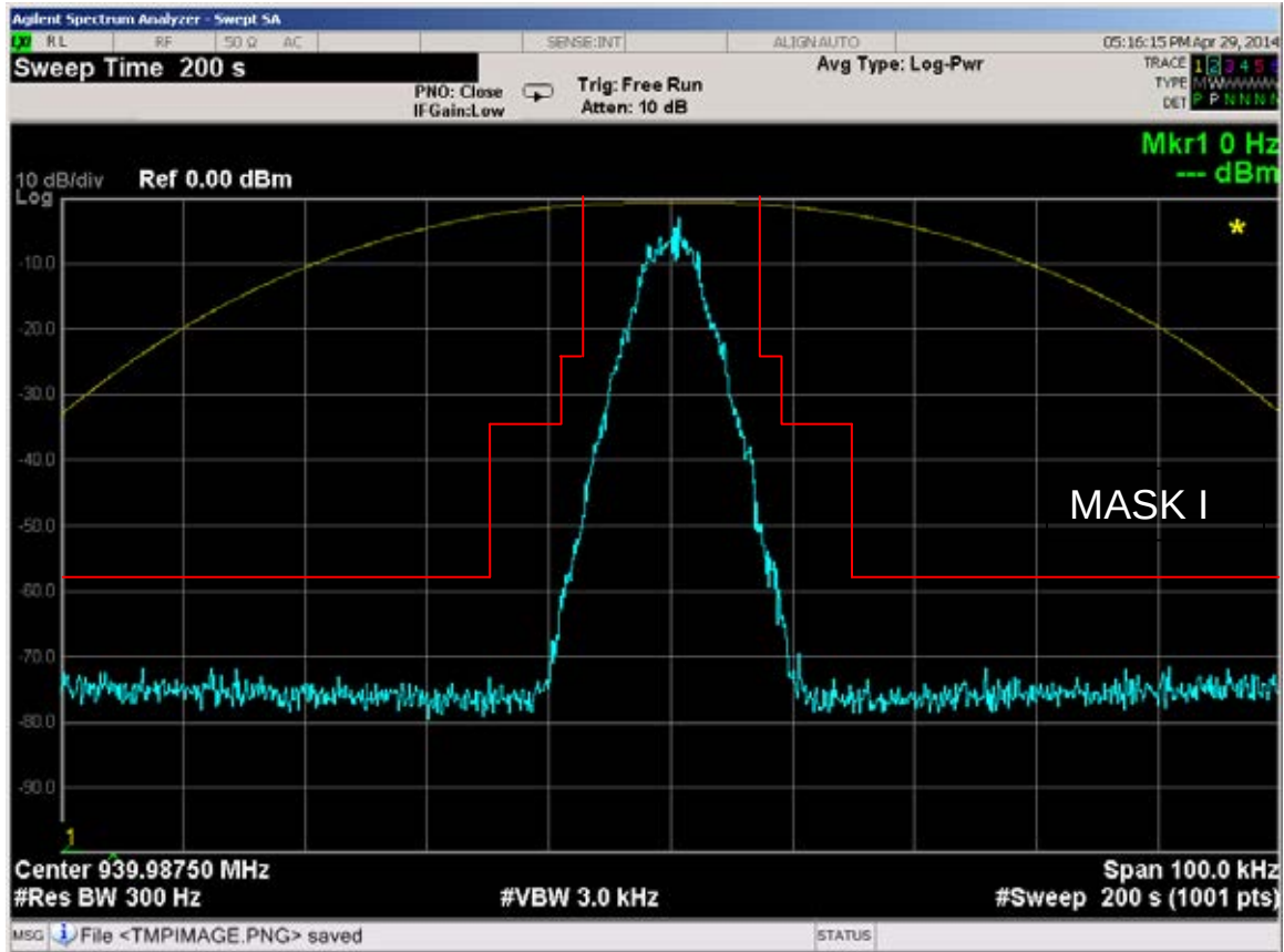
Figure 6E-59: 939.9875 MHz, 4-Level FSK Data Modulation only, 7K60FXD Mask I
