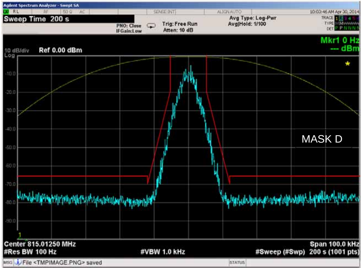
Figure 6E-67: 815.0125 MHz, 4-Level FSK Voice Modulation only, 7K60F1E Mask D
