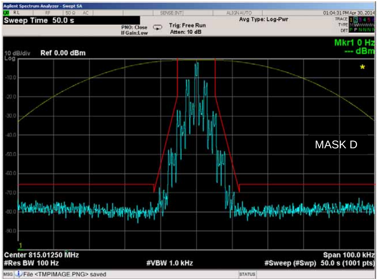
Figure 6E-32: 815.0125 MHz, 12.5 kHz Channel Spacing, 2000/3000 Hz FSK Data and DPL Tone Modulation, 11K0F3E Mask D
