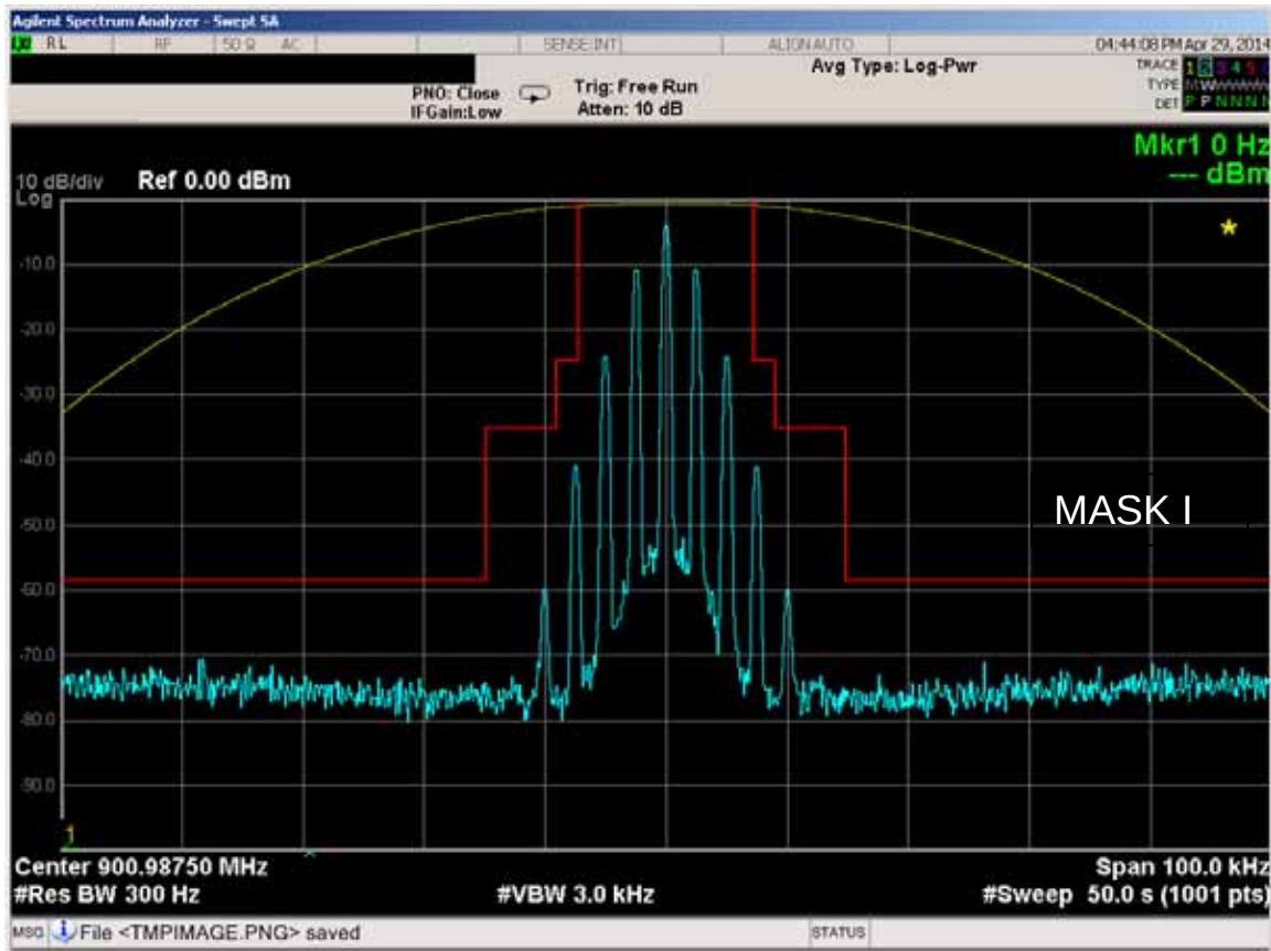
Figure 6E-37: 900.9875 MHz, 12.5 kHz Channel Spacing, 2500Hz Audio Modulation only, 11K0F3E Mask I
