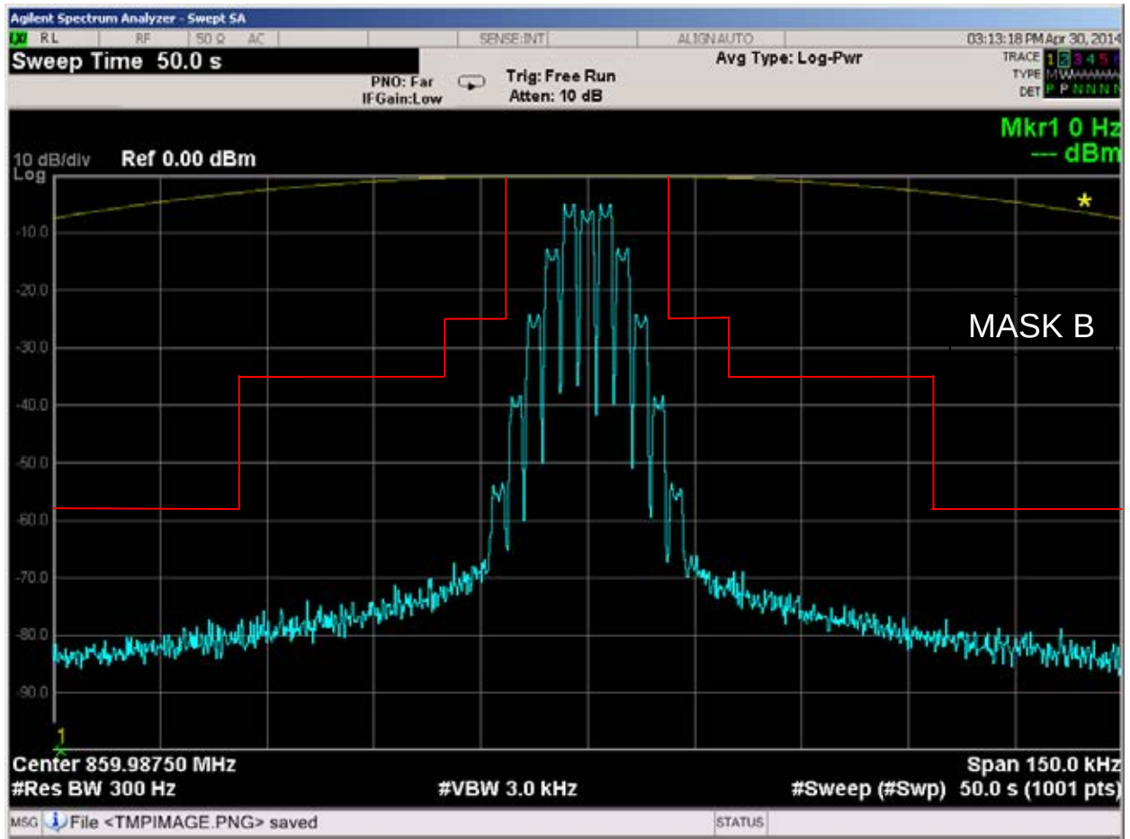
Figure 6E-4: 859.9875MHz, 25 kHz Channel Spacing, 2500Hz Audio and DPL Tone Modulation, 16K0F3E Mask B
