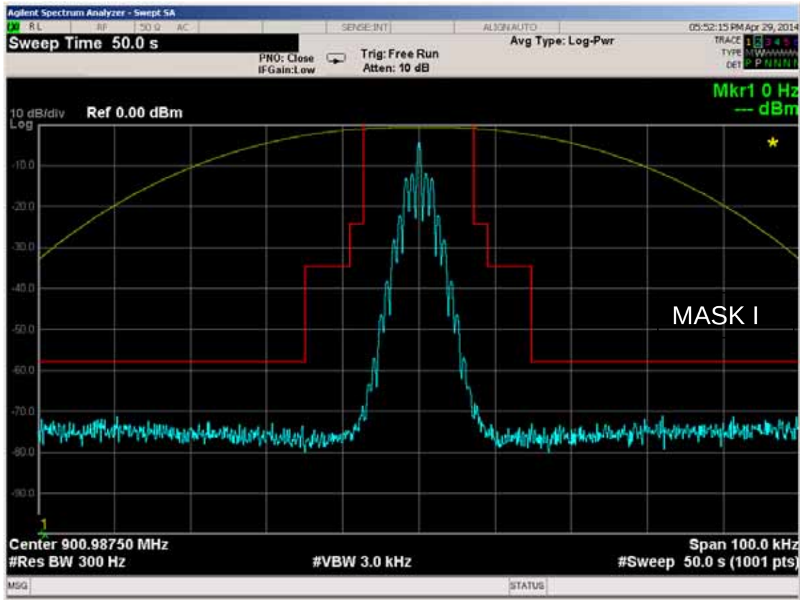
Figure 6E-43: 900.9875 MHz, 12.5 kHz Channel Spacing, DTMF Modulation only, 11K0F3E Mask I
