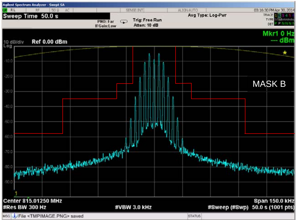
Figure 6E-3: 815.0125 MHz, 25 kHz Channel Spacing, 2500Hz Audio Modulation only, Modulation, 16K0F3E Mask B
