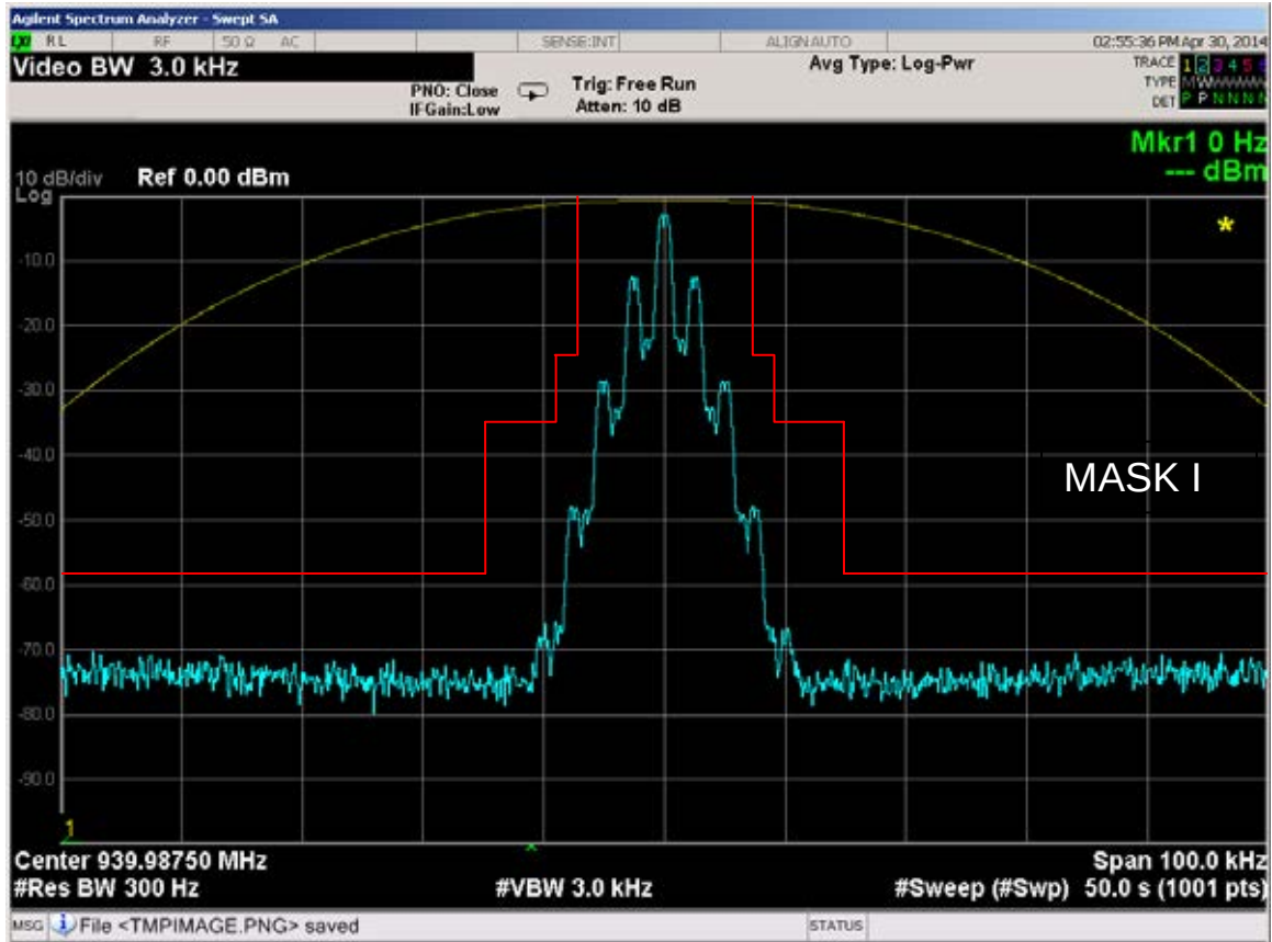
Figure 6E-54: 939.9875 MHz, 12.5 kHz Channel Spacing, 2000/3000 Hz FSK Data and TPL Tone Modulation, 11K0F3E Mask I
