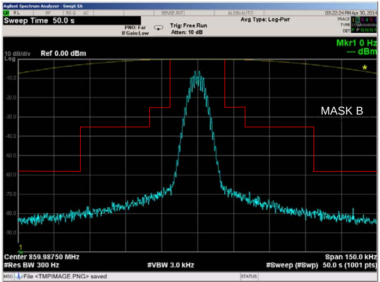
Figure 6E-12: 859.9875 MHz, 25 kHz Channel Spacing, DTMF Modulation only, 16K0F3E Mask B
