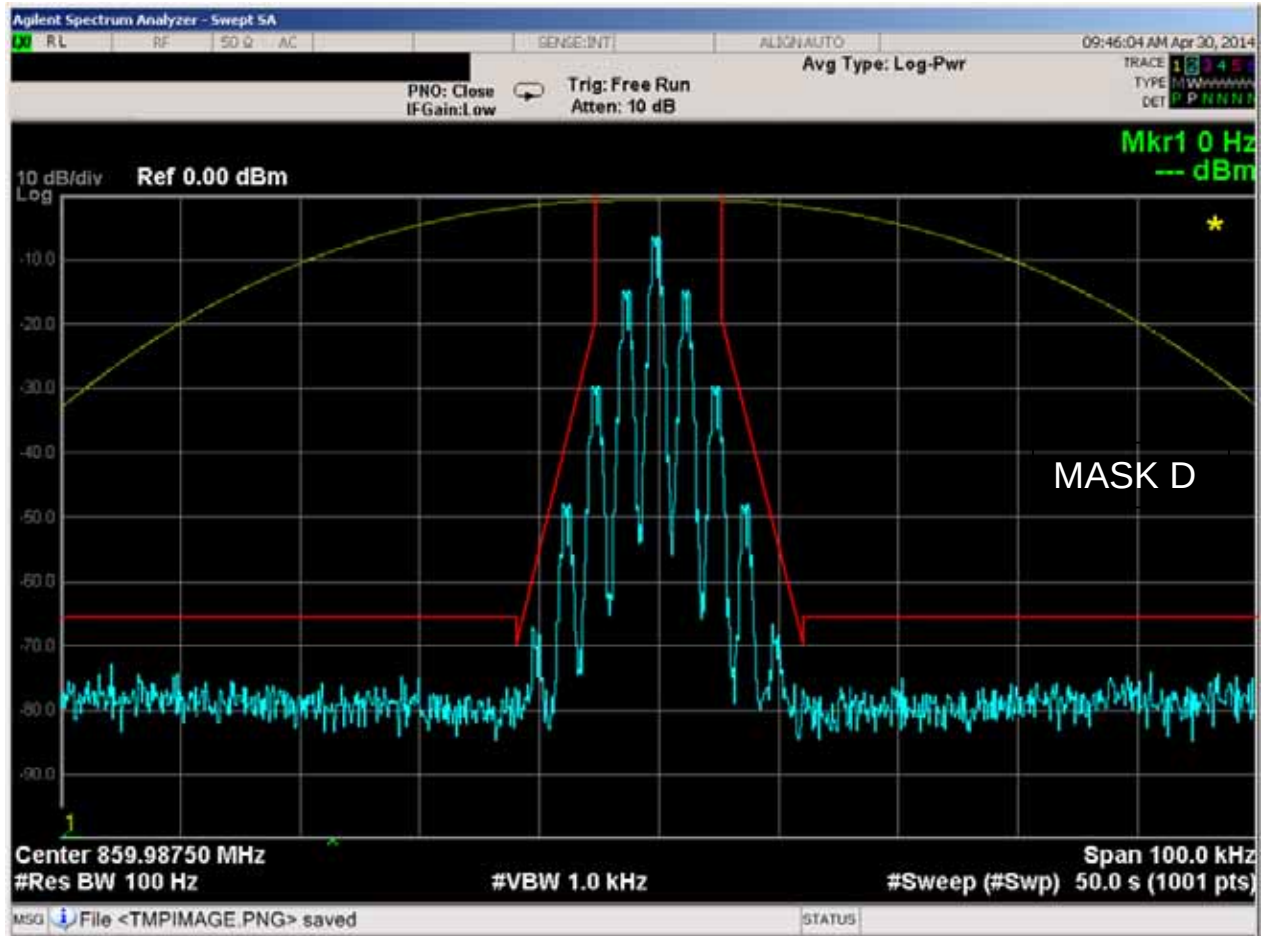
Figure 6E-24: 859.9875MHz, 12.5 kHz Channel Spacing, 2500Hz Audio and TPL Tone Modulation, 11K0F3E Mask D
