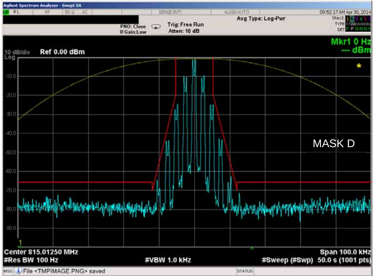
Figure 6E-20: 815.0125 MHz, 12.5 kHz Channel Spacing, 2500Hz Audio and DPL Tone Modulation, 11K0F3E Mask D
