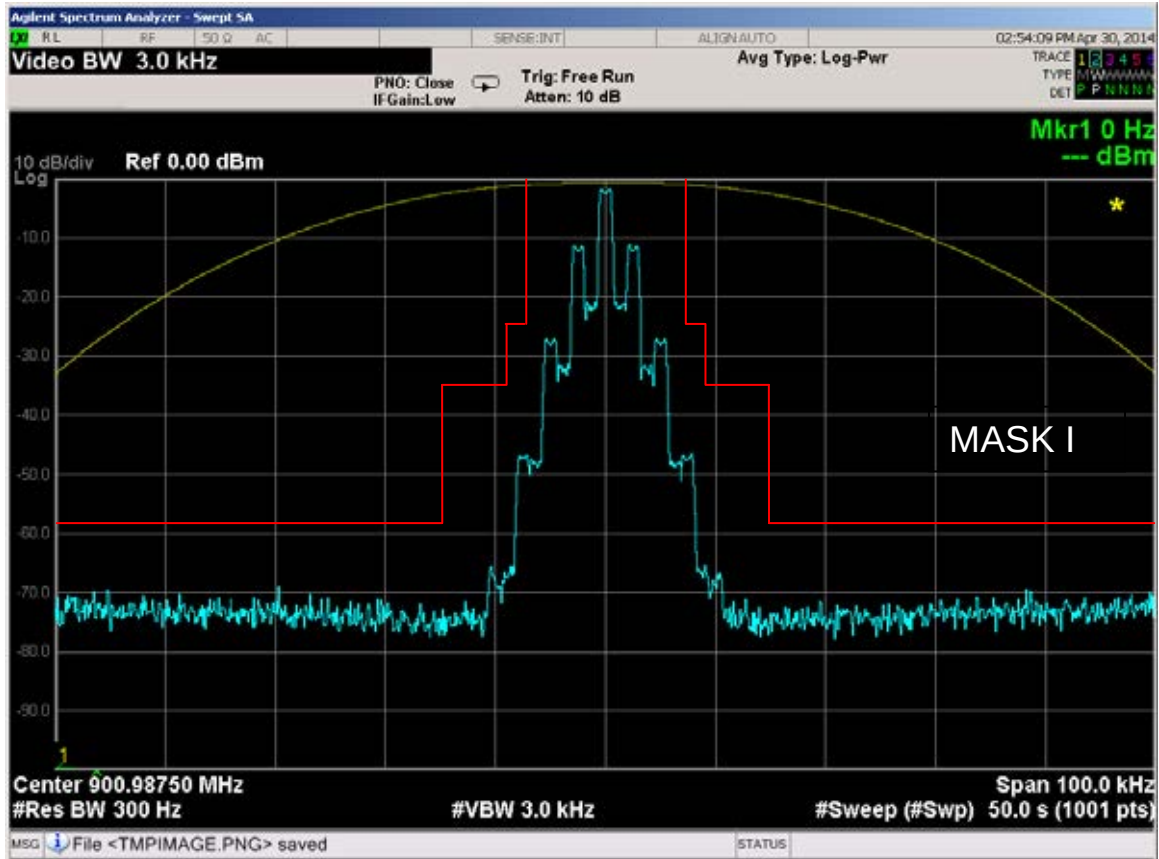
Figure 6E-50: 900.9875 MHz, 12.5 kHz Channel Spacing, 2000/3000 Hz FSK Data and DPL Tone Modulation, 11K0F3E Mask I
