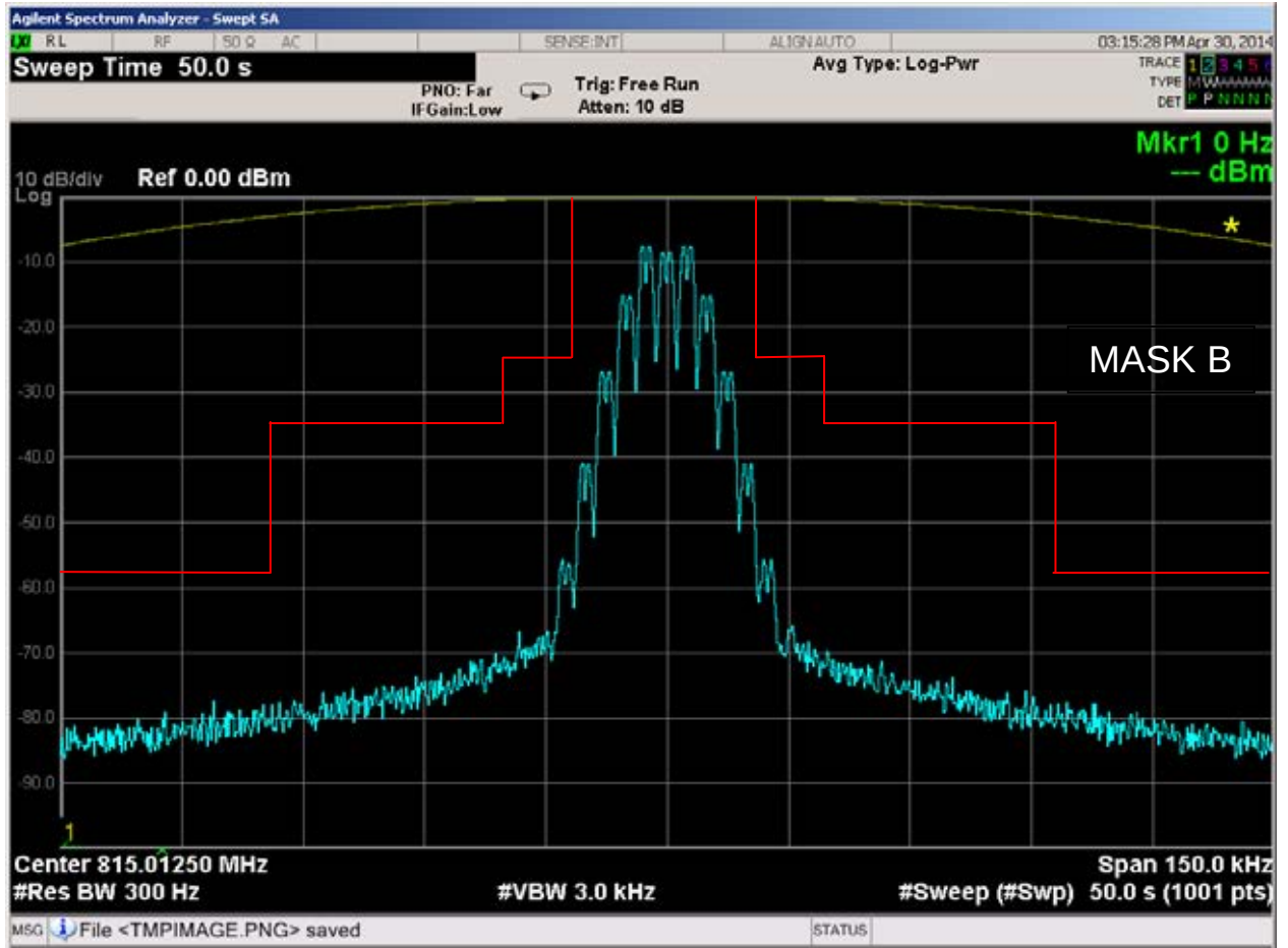
Figure 6E-2: 815.0125 MHz, 25 kHz Channel Spacing, 2500Hz Audio and TPL Tone Modulation, 16K0F3E Mask B
