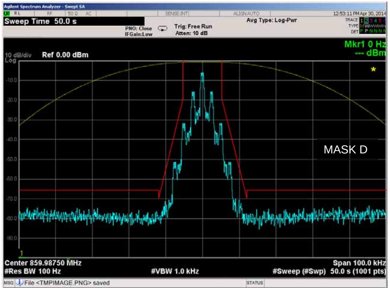
Figure 6E-36: 859.9875 MHz, 12.5 kHz Channel Spacing, 2000/3000 Hz FSK Data and TPL Tone Modulation, 11K0F3E Mask D
