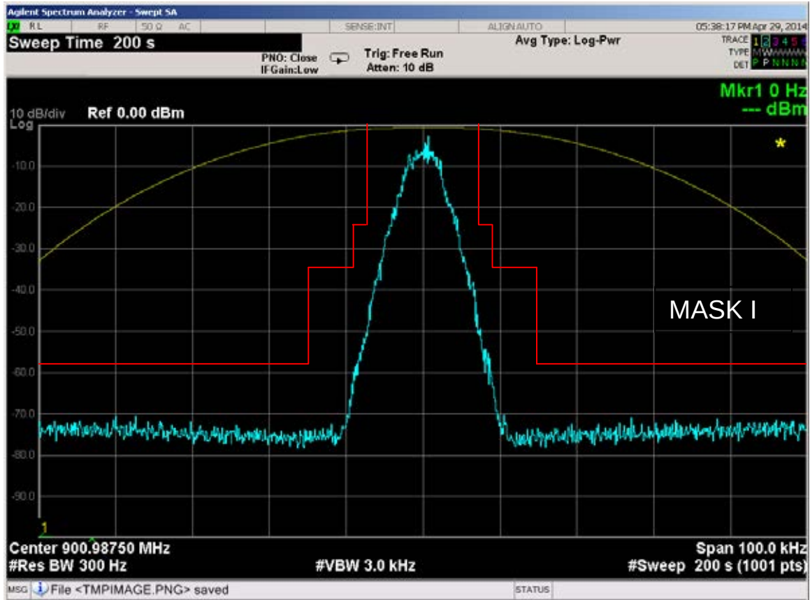
Figure 6E-63: 900.9875 MHz, 4-Level FSK Voice and Data Modulation, 7K60F1W Mask I
