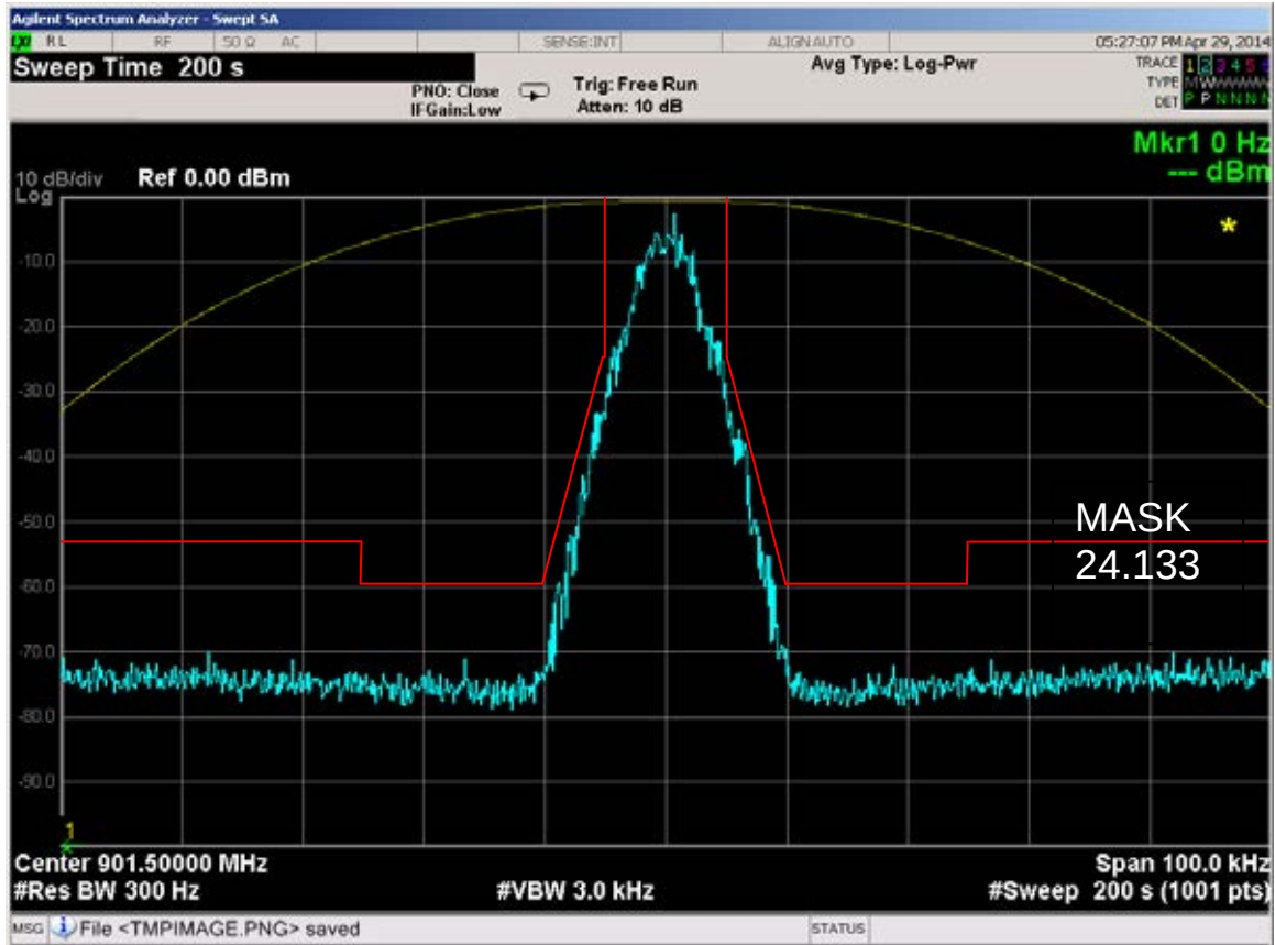
Figure 6E-70: 901.5 MHz, 9W, 4-Level FSK Voice Modulation only, 7K60F1E Mask 24.133
