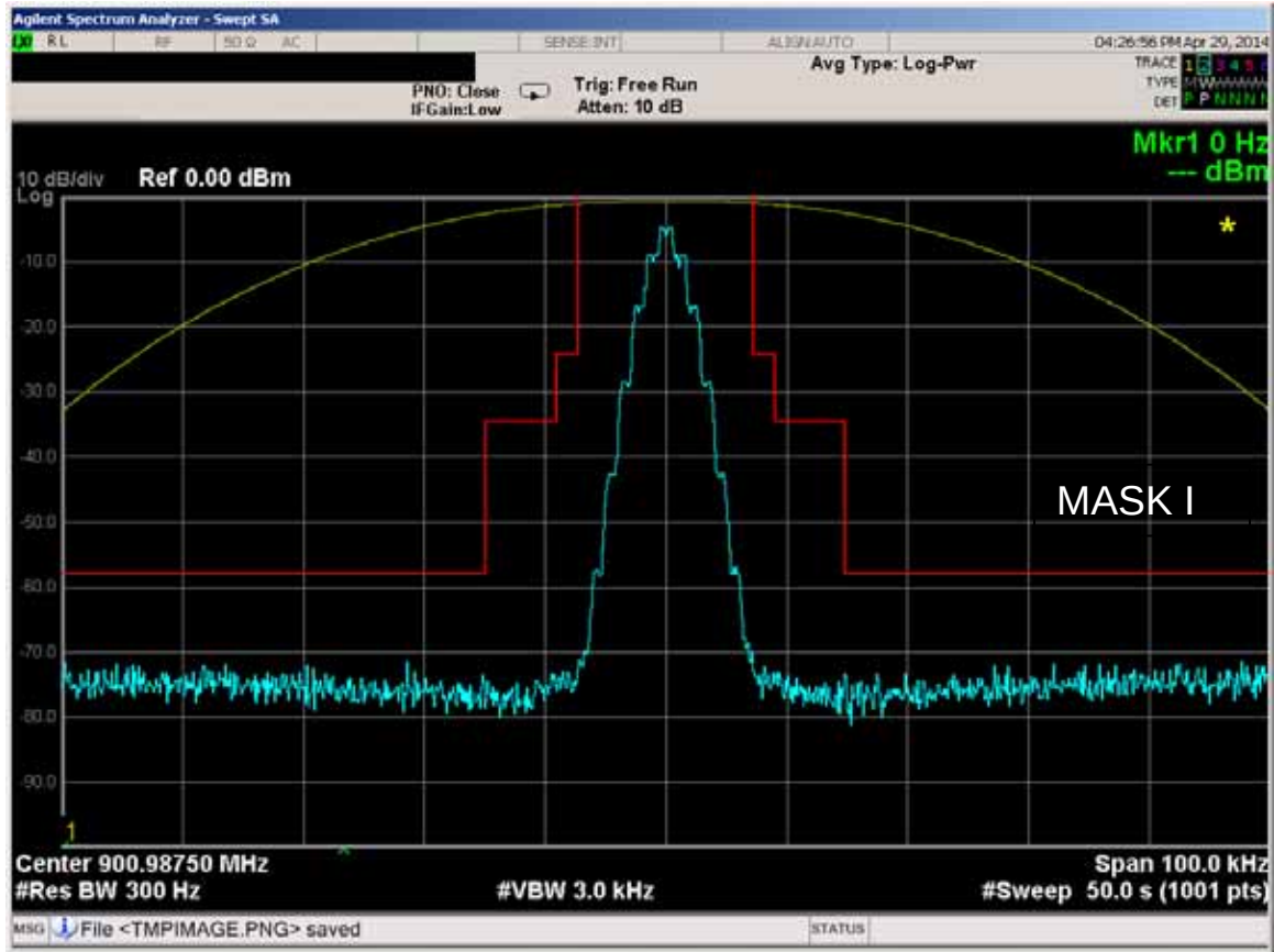
Figure 6E-44: 900.9875 MHz, 12.5 kHz Channel Spacing, DTMF and DPL Tone Modulation, 11K0F3E Mask I
