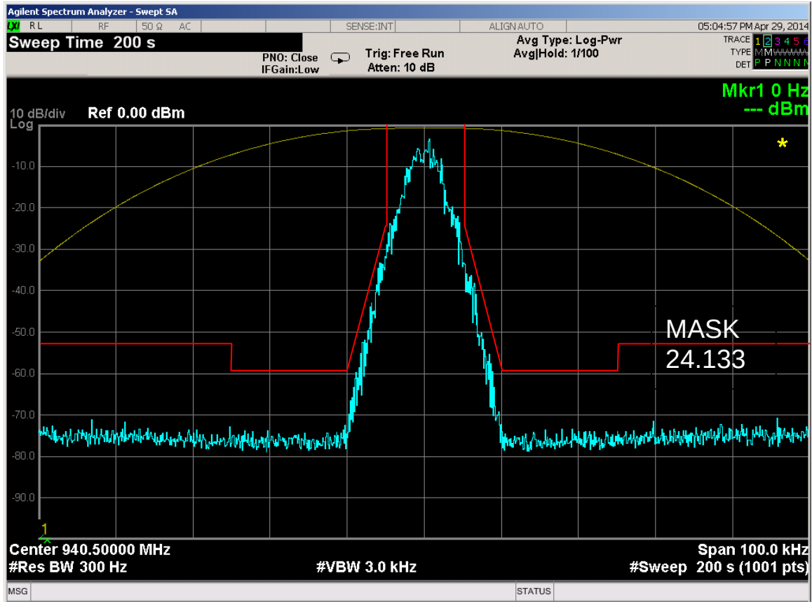
Figure 6E-72: 940.5 MHz, 9W, 4-Level FSK Voice Modulation only, 7K60F1E Mask 24.133
