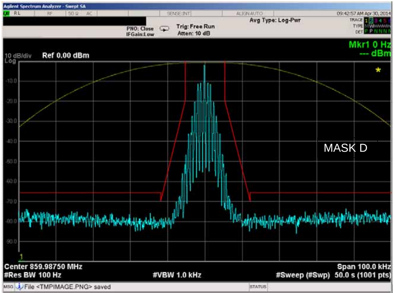
Figure 6E-28: 859.9875 MHz, 12.5 kHz Channel Spacing, DTMF Modulation only, 11K0F3E Mask D
