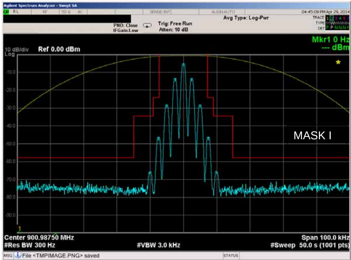
Figure 6E-39: 900.9875 MHz, 12.5 kHz Channel Spacing, 2500Hz Audio and TPL Tone Modulation, 11K0F3E Mask I
