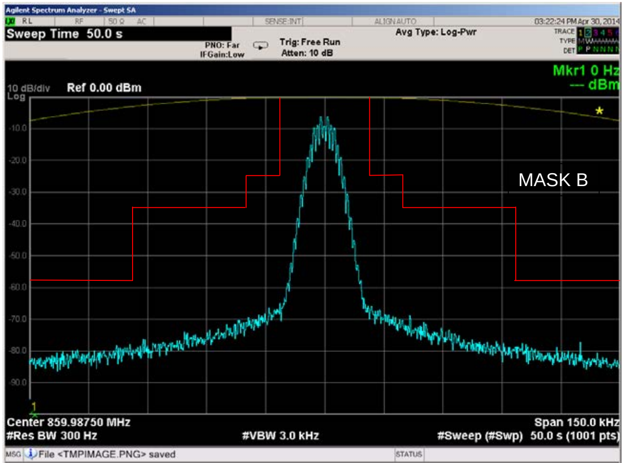
Figure 6E-10: 859.9875 MHz, 25 kHz Channel Spacing, DTMF and DPL Tone Modulation, 16K0F3E Mask B
