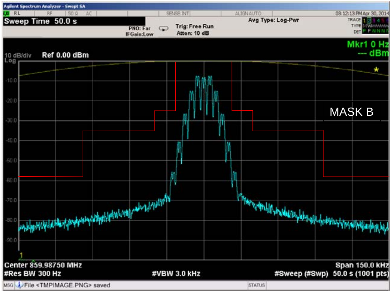
Figure 6E-5: 859.9875MHz, 25 kHz Channel Spacing, 2500Hz Audio and TPL Tone Modulation, 16K0F3E Mask B
