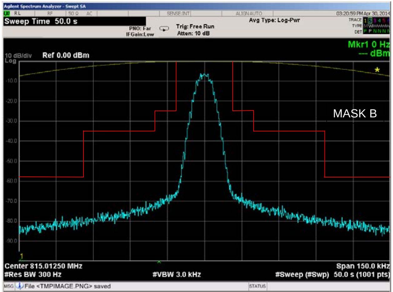
Figure 6E-7: 815.0125 MHz, 25 kHz Channel Spacing, DTMF and DPL Tone Modulation, 16K0F3E Mask B
