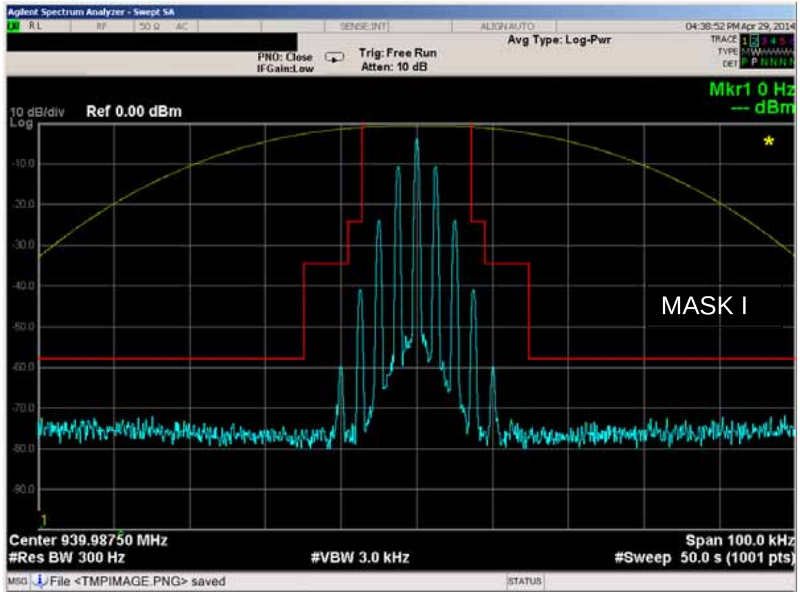
Figure 6E-40: 939.9875 MHz, 12.5 kHz Channel Spacing, 2500Hz Audio Modulation only, 11K0F3E Mask I
