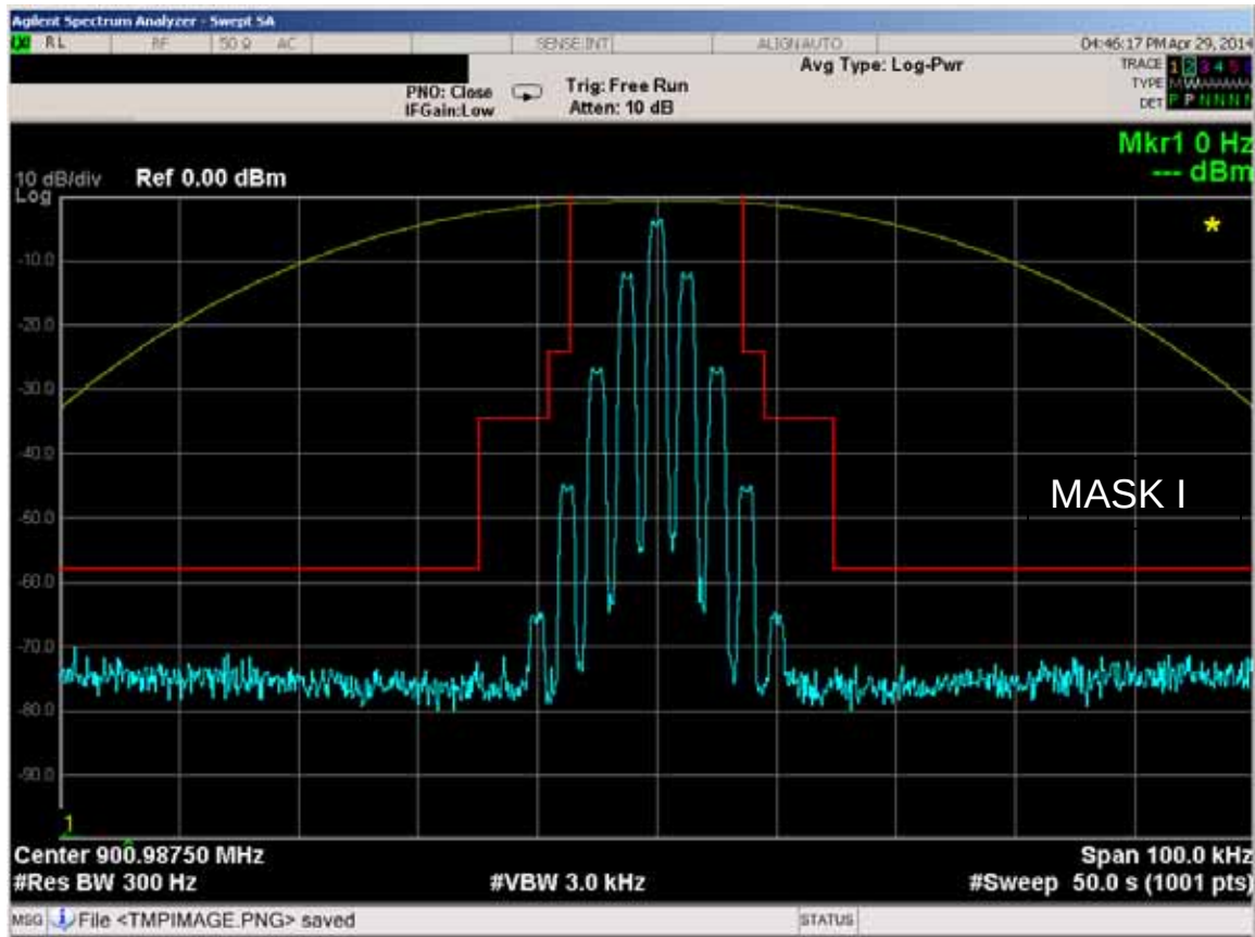
Figure 6E-38: 900.9875 MHz, 12.5 kHz Channel Spacing, 2500Hz Audio and DPL Tone Modulation, 11K0F3E Mask I
