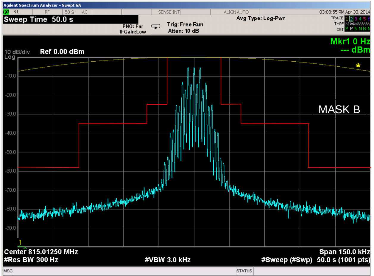
Figure 6E-15: 815.0125 MHz, 25 kHz Channel Spacing, 2000/3000 Hz FSK Data Modulation Only, 16K0F3E Mask B
