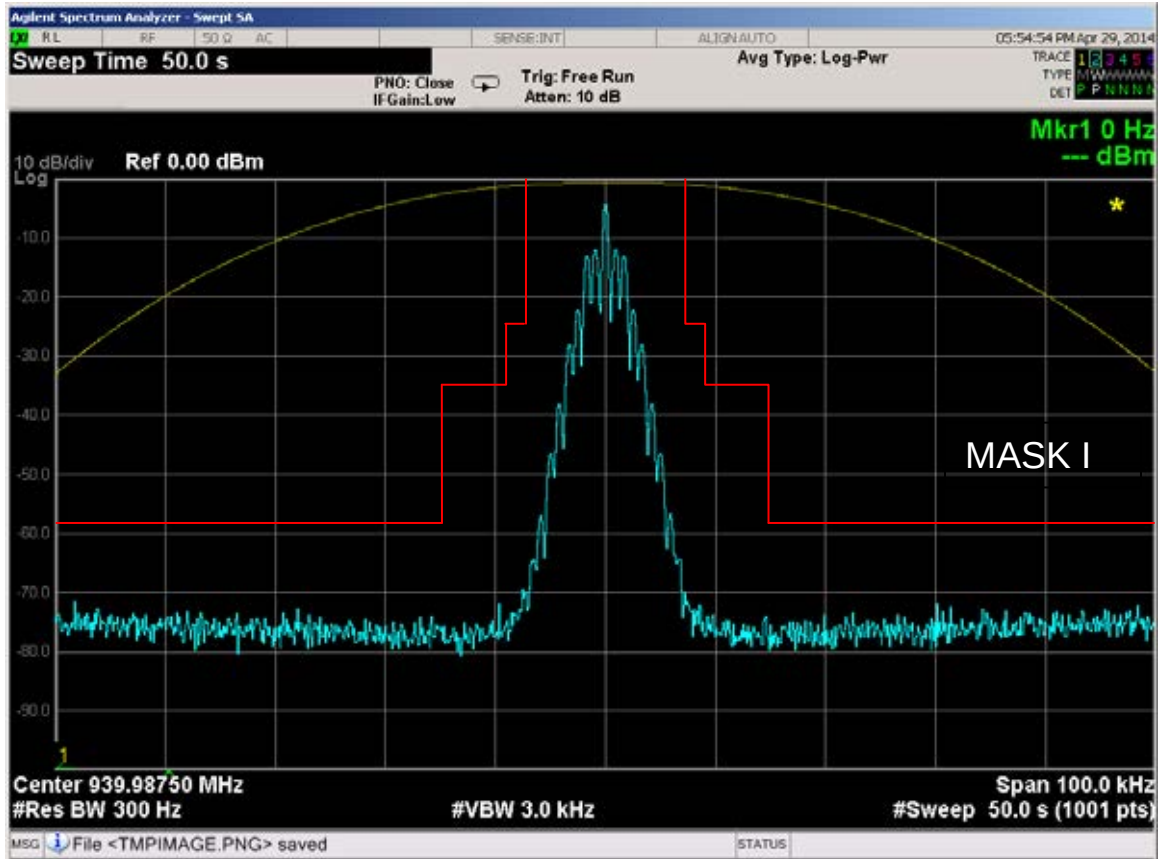
Figure 6E-46: 939.9875 MHz, 12.5 kHz Channel Spacing, DTMF Modulation only, 11K0F3E Mask I
