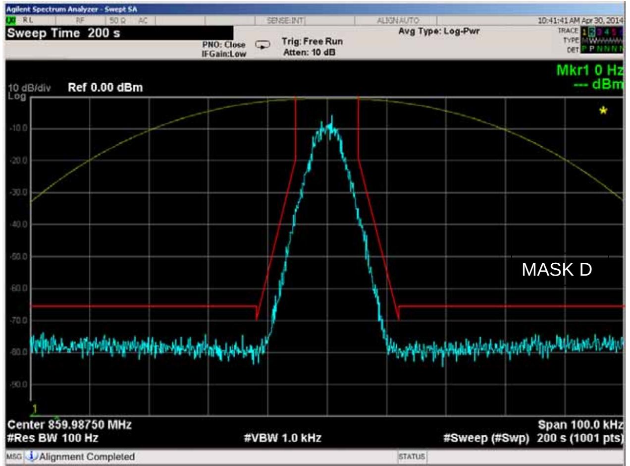
Figure 6E-56: 859.9875 MHz, 4-Level FSK Data Modulation only, 7K60FXD Mask D
