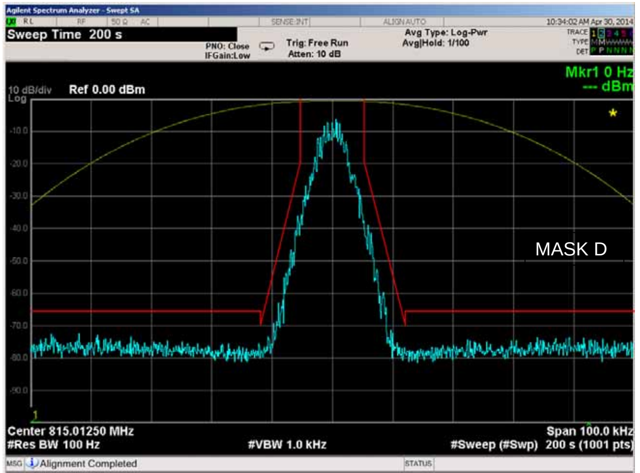
Figure 6E-61: 815.0125 MHz, 4-Level FSK Voice and Data Modulation, 7K60F1W Mask D
