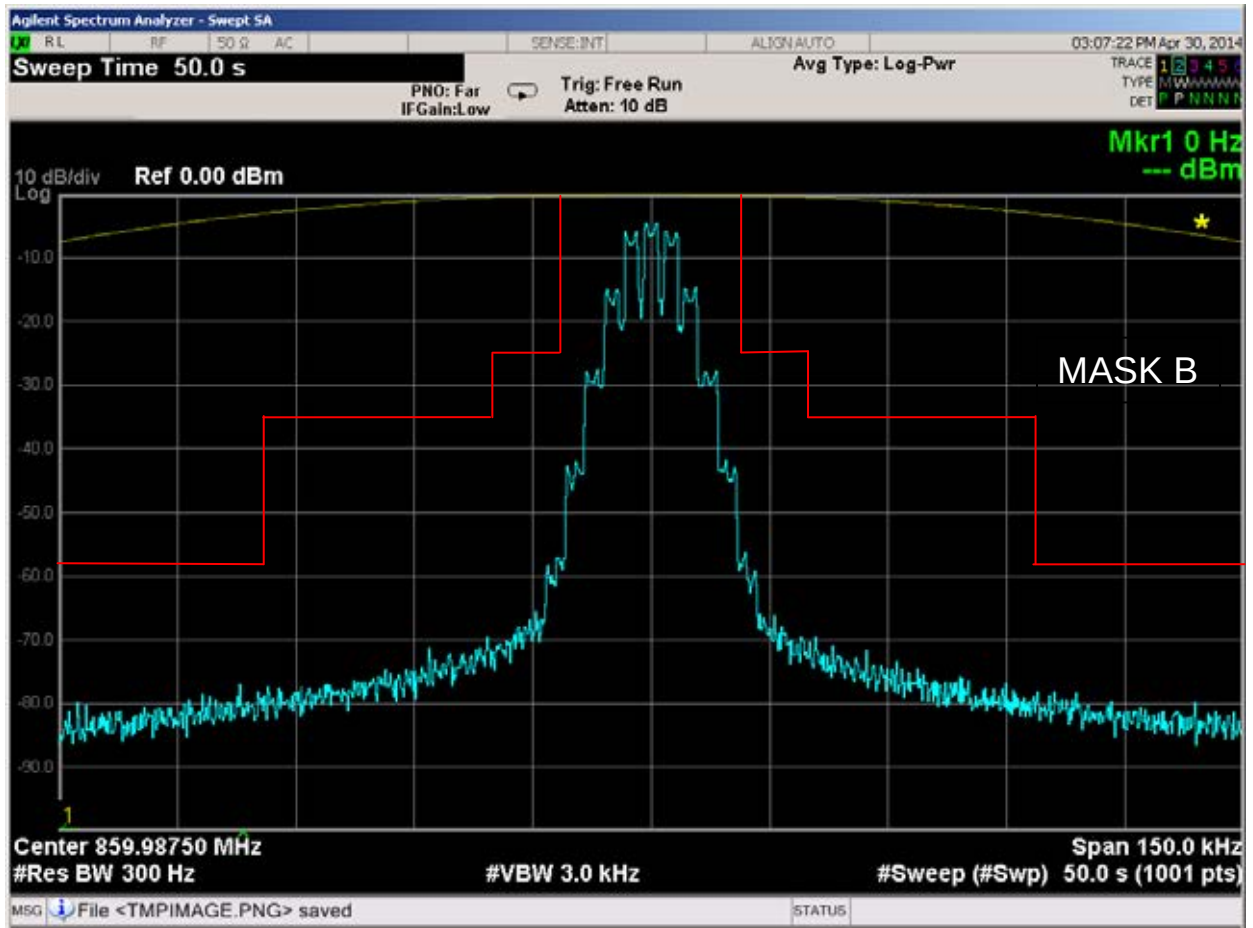
Figure 6E-16: 859.9875 MHz, 25 kHz Channel Spacing, 2000/3000 Hz FSK Data and DPL Tone Modulation, 16K0F3E Mask B
