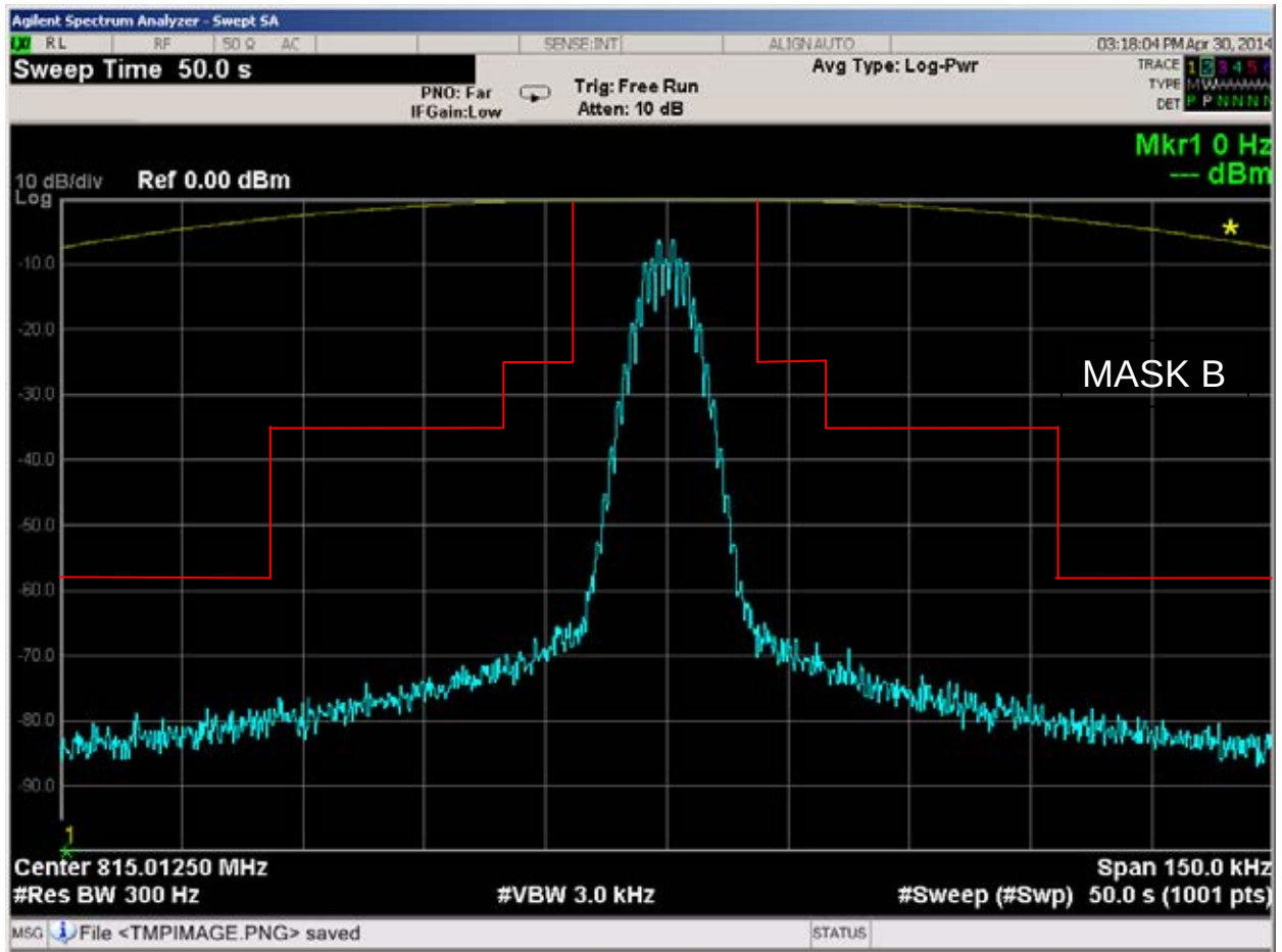
Figure 6E-9: 815.0125 MHz, 25 kHz Channel Spacing, DTMF Modulation only, 16K0F3E Mask B
