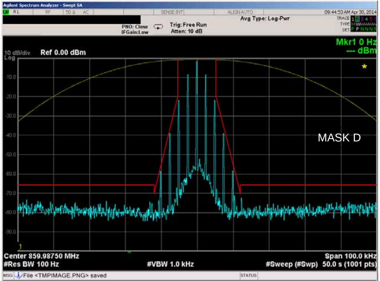
Figure 6E-22: 859.9875MHz, 12.5 kHz Channel Spacing, 2500Hz Audio Modulation only, 11K0F3E Mask D
