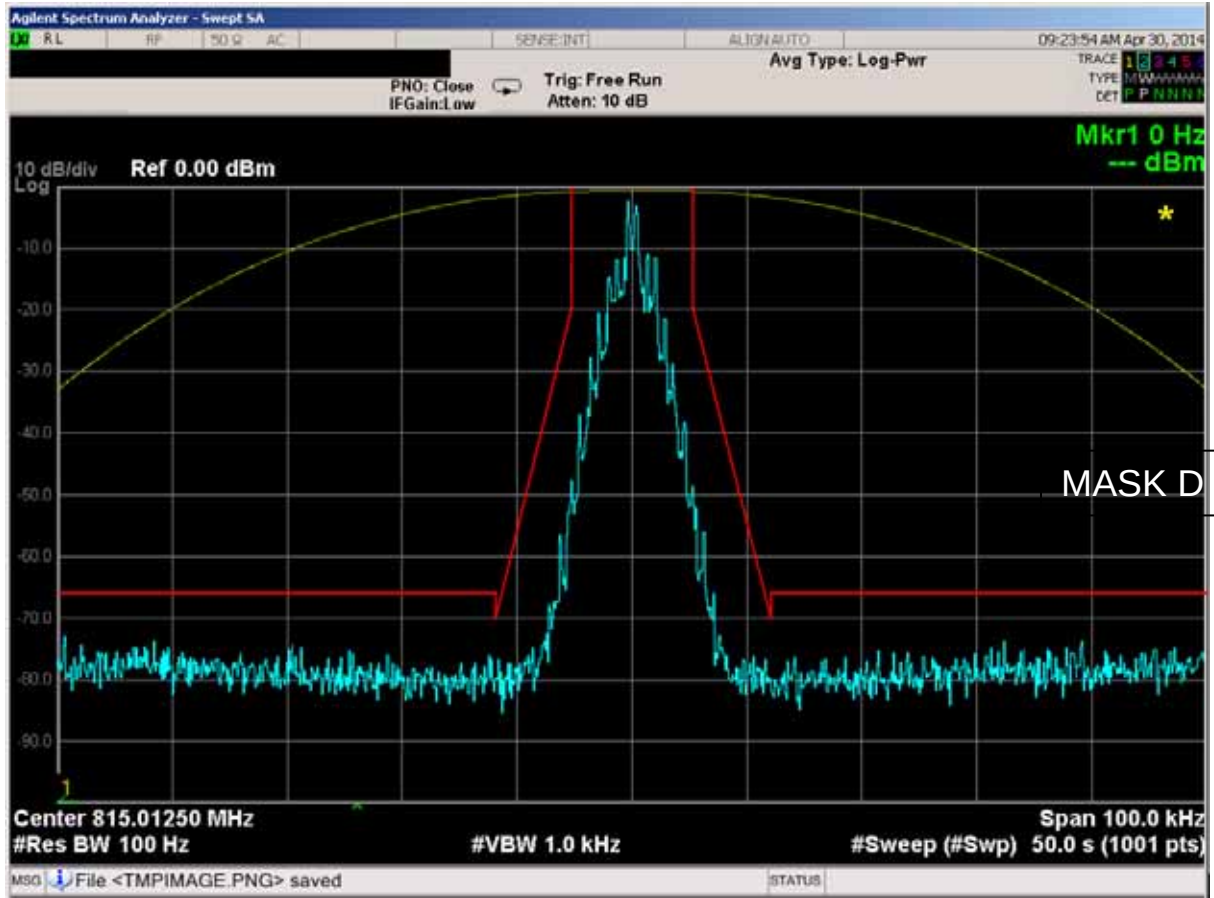
Figure 6E-26: 815.0125 MHz, 12.5 kHz Channel Spacing, DTMF and DPL Tone Modulation, 11K0F3E Mask D
