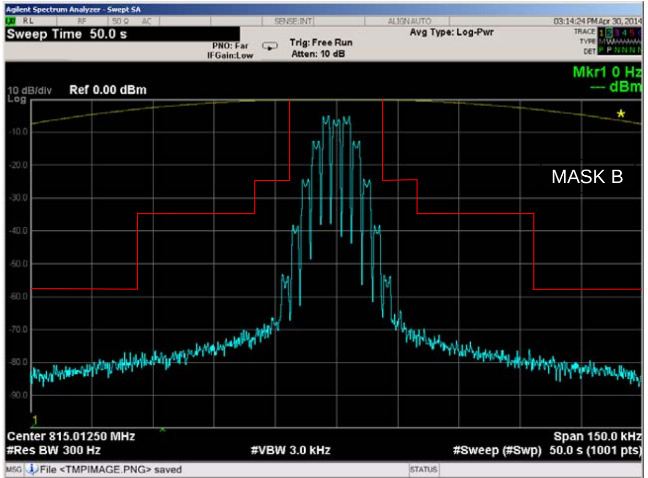
Figure 6E-1: 815.0125 MHz, 25 kHz Channel Spacing, 2500Hz Audio and DPL Tone Modulation, 16K0F3E Mask B
