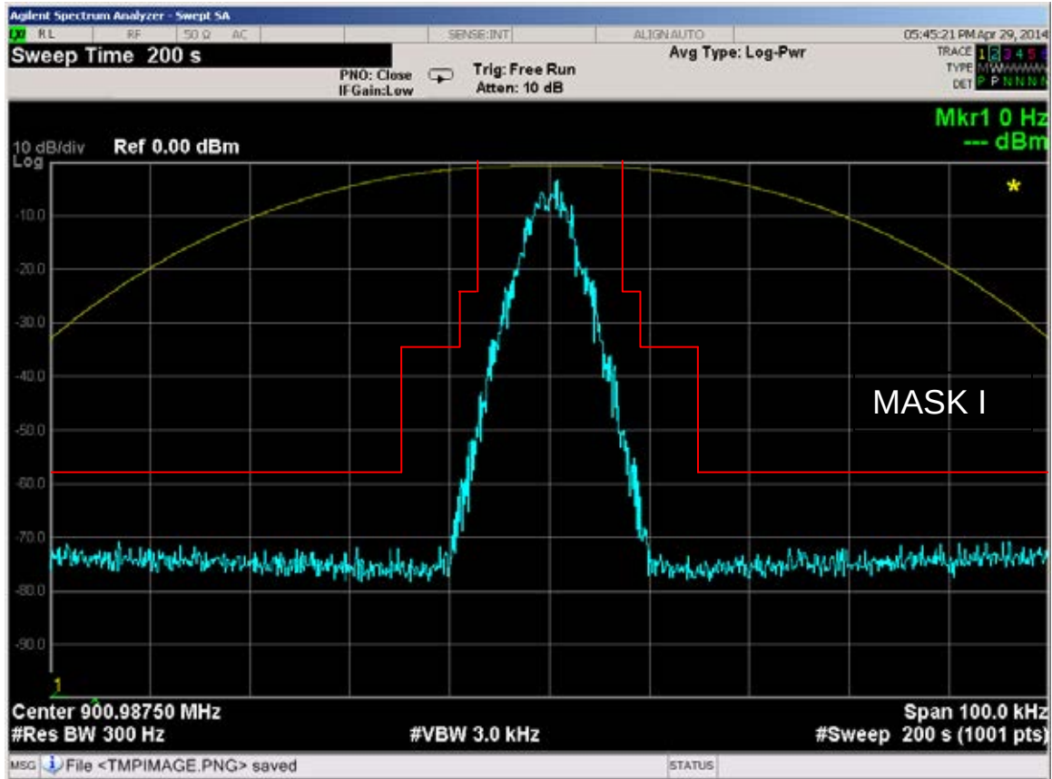
Figure 6E-69: 900.9875 MHz, 4-Level FSK Voice Modulation only, 7K60F1E Mask I
