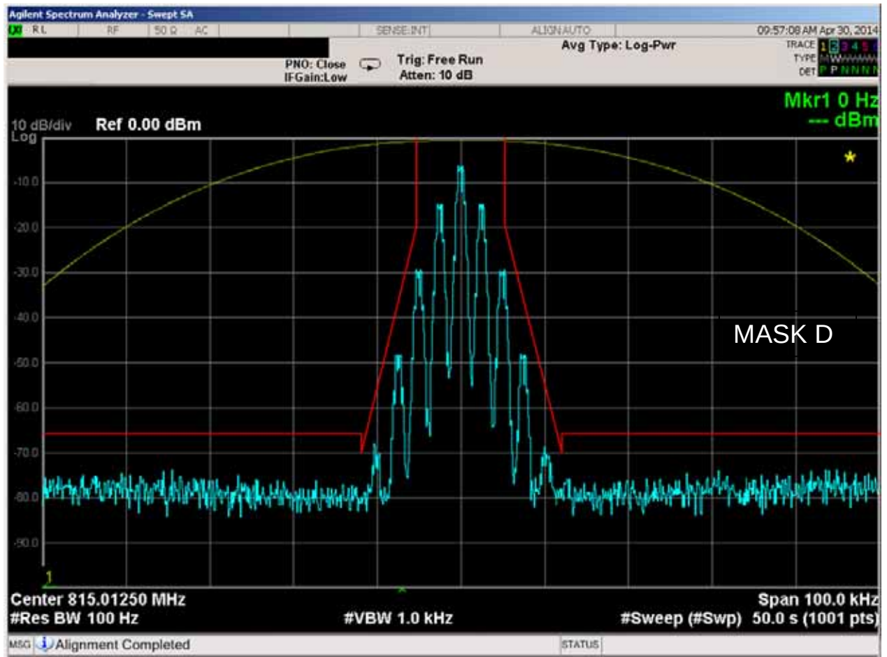
Figure 6E-21: 815.0125 MHz, 12.5 kHz Channel Spacing, 2500Hz Audio and TPL Tone Modulation, 11K0F3E Mask D
