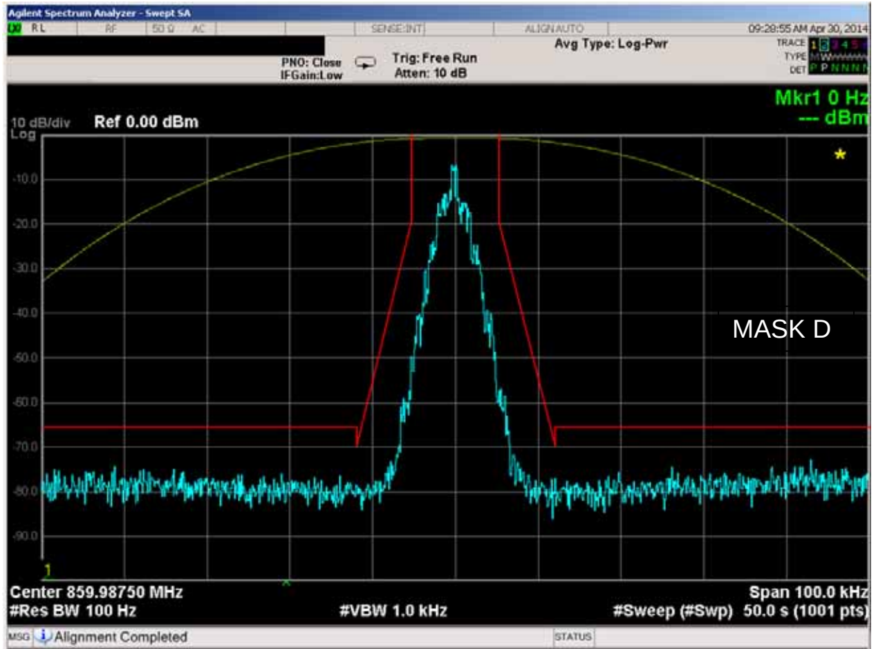
Figure 6E-30: 859.9875 MHz, 12.5 kHz Channel Spacing, DTMF and TPL Tone Modulation, 11K0F3E Mask D
