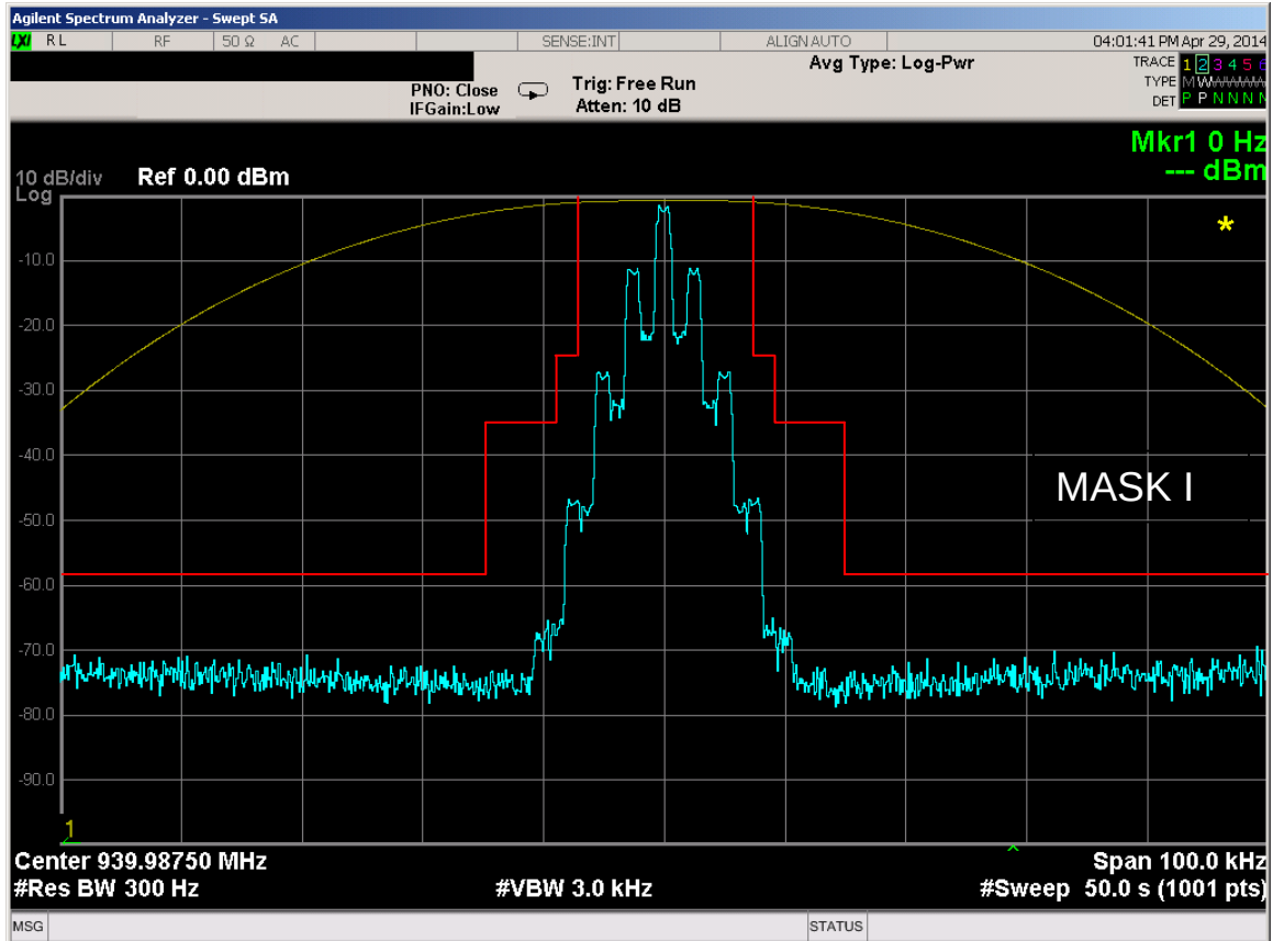
Figure 6E-53: 939.9875 MHz, 12.5 kHz Channel Spacing, 2000/3000 Hz FSK Data and DPL Tone Modulation, 11K0F3E Mask I
