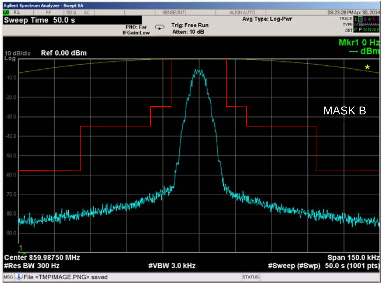
Figure 6E-11: 859.9875 MHz, 25 kHz Channel Spacing, DTMF and TPL Tone Modulation, 16K0F3E Mask B
