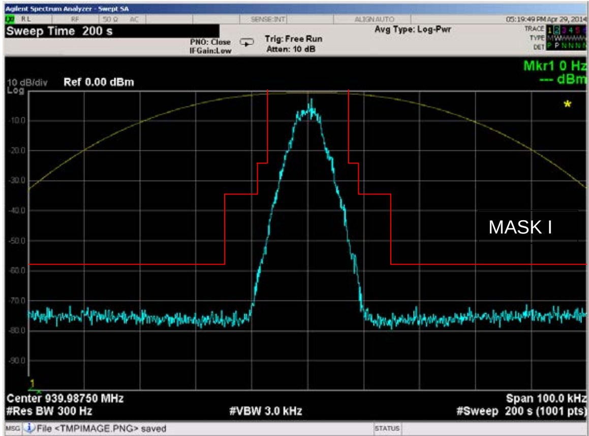
Figure 6E-65: 939.9875 MHz, 4-Level FSK Voice and Data Modulation, 7K60F1W Mask I
