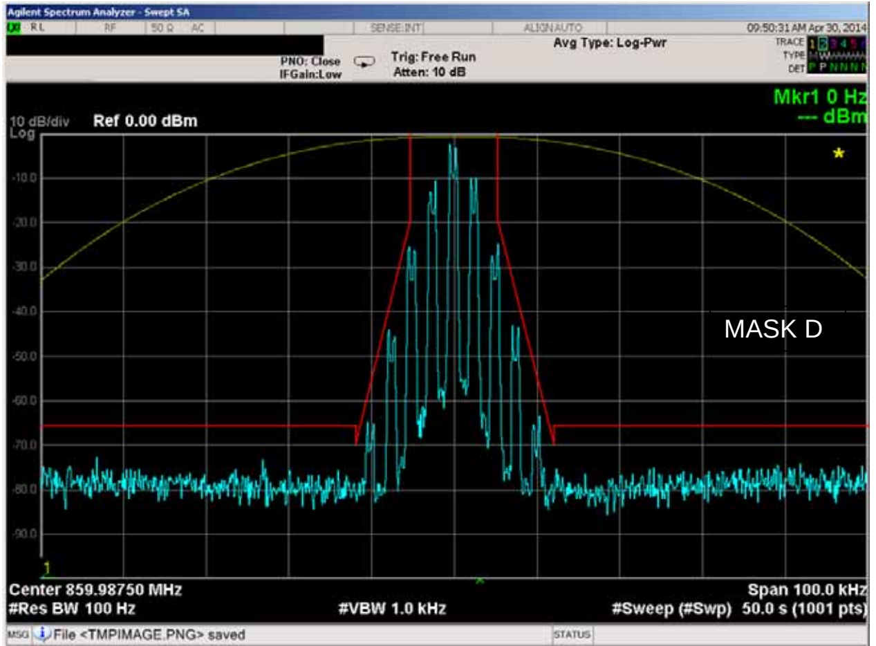
Figure 6E-23: 859.9875MHz, 12.5 kHz Channel Spacing, 2500Hz Audio and DPL Tone Modulation, 11K0F3E Mask D
