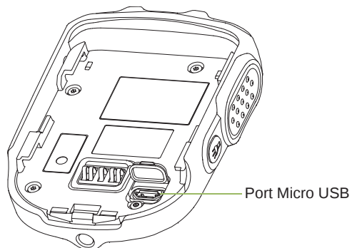
Figure 2.14: Emplacement du port micro USB
