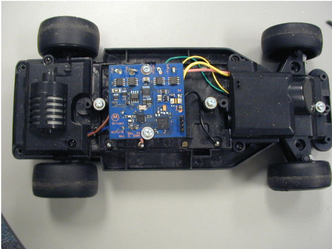
Photograph 9-1: Top side view of Car PC Board
