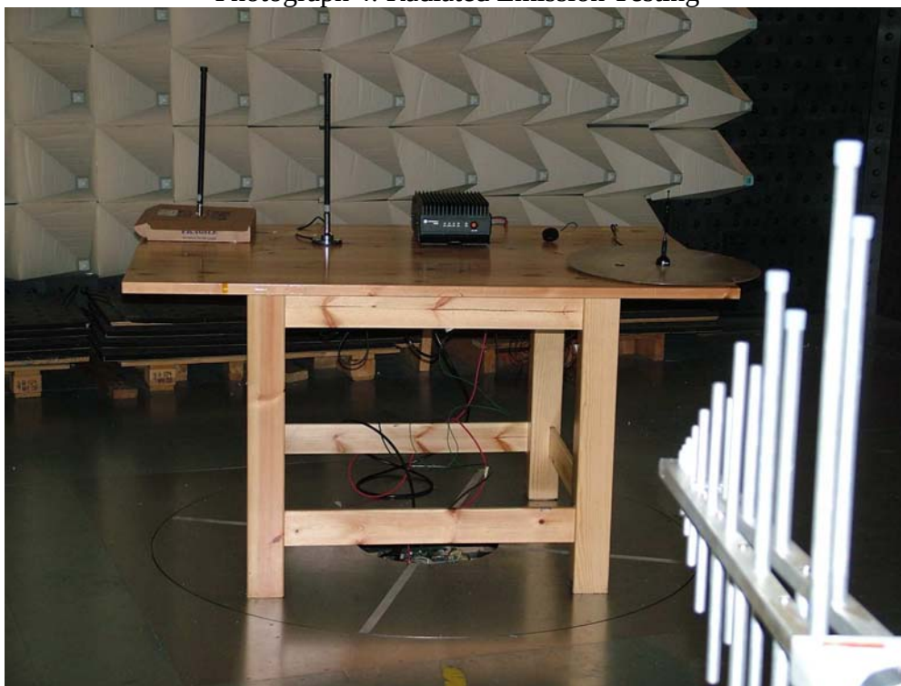
Photograph 4: Radiated Emission Testing
