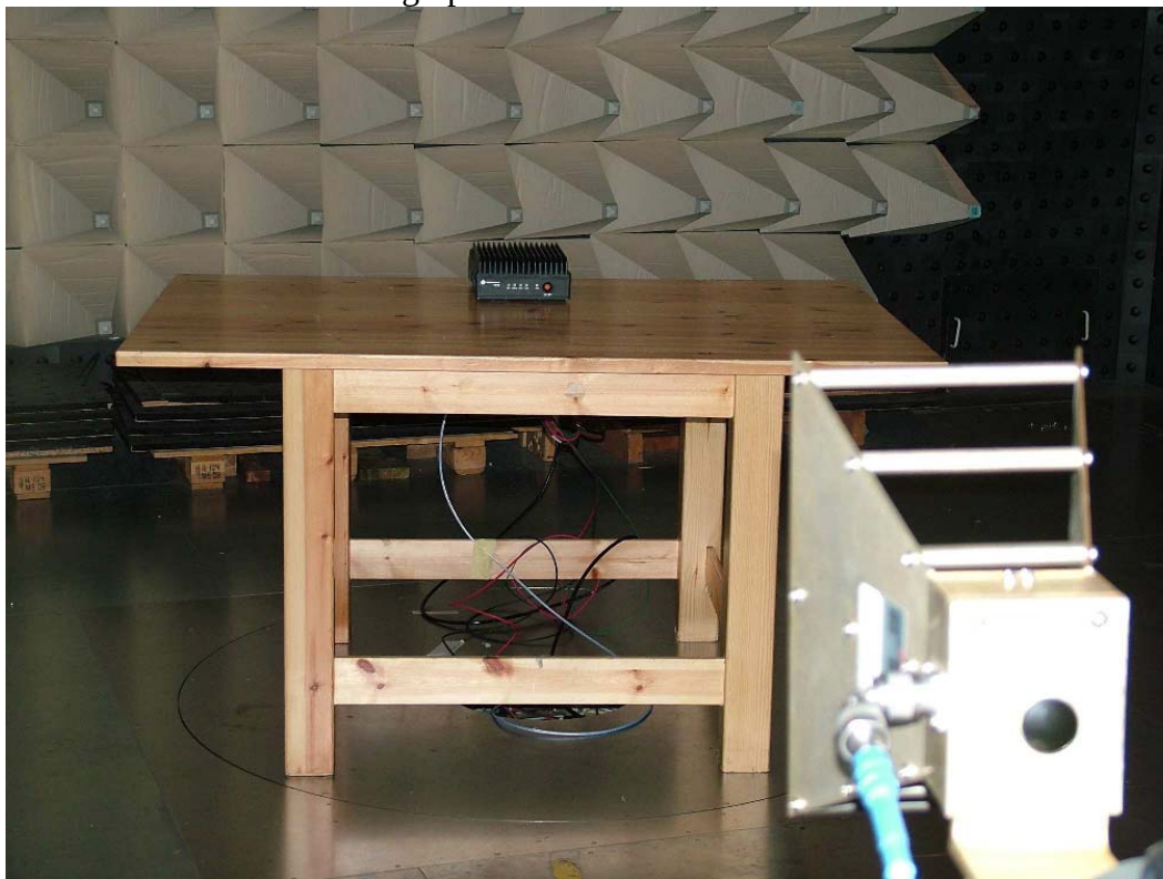
Photograph 2: Radiated measurements
