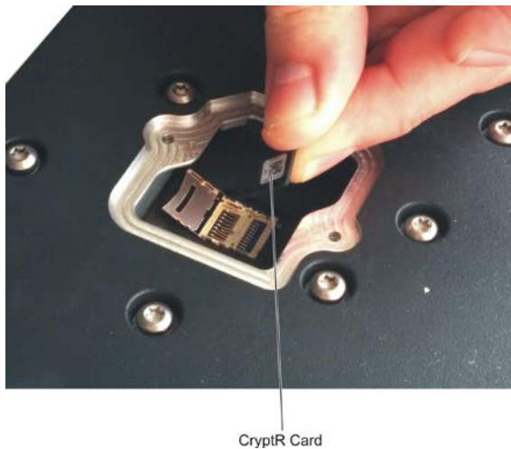
Figure 13 Installing the CRYPTR Card
