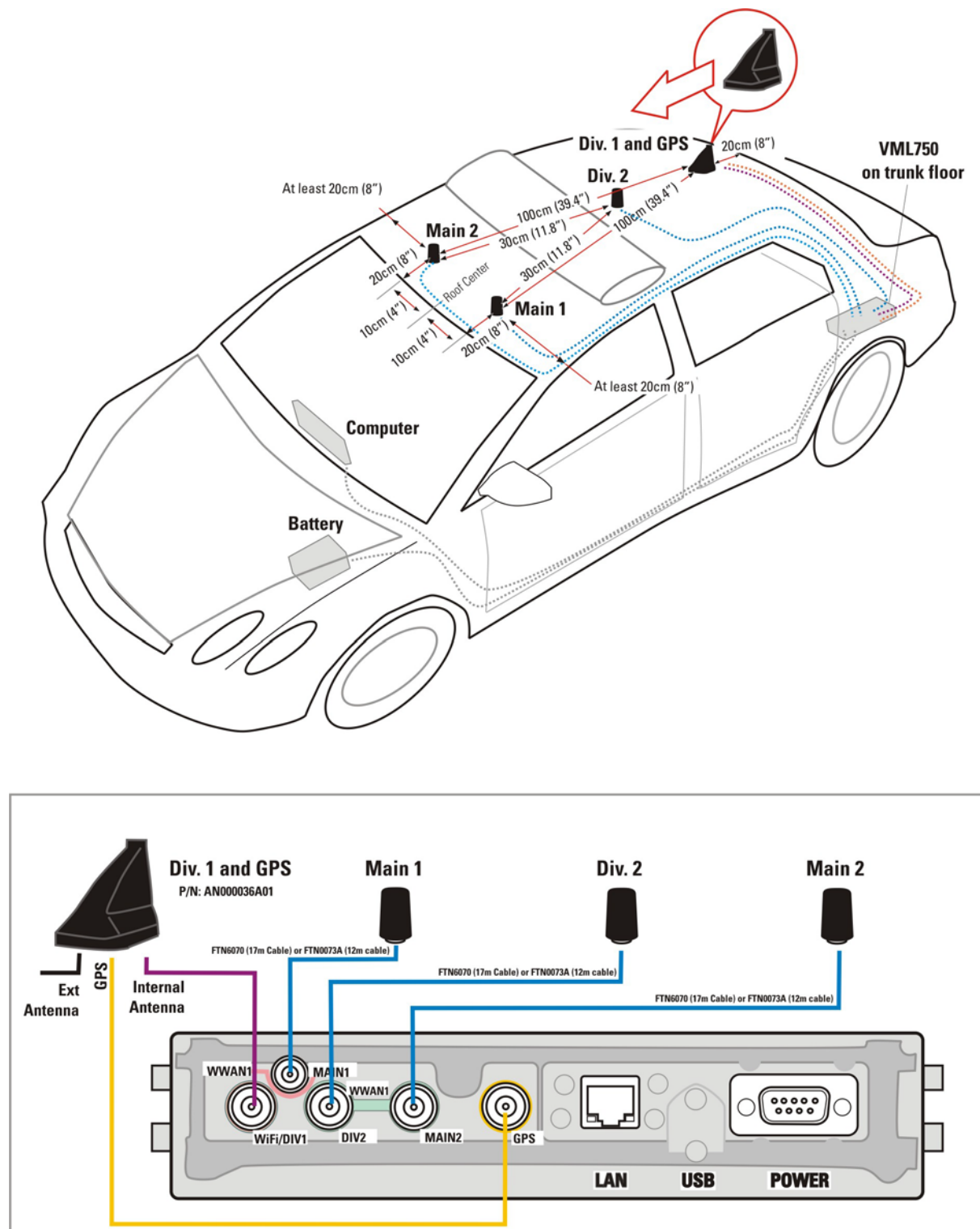
Figure 8 Schematic Installation Diagram for Sub-model FLN5059A
