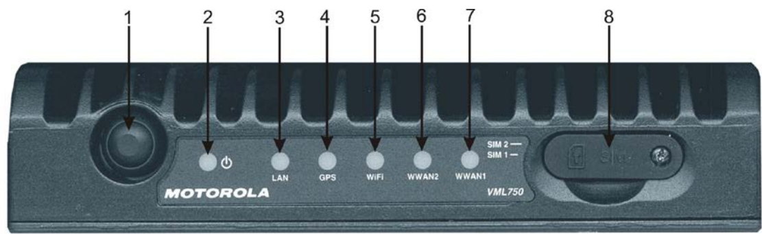
Figure 2 Front Panel
