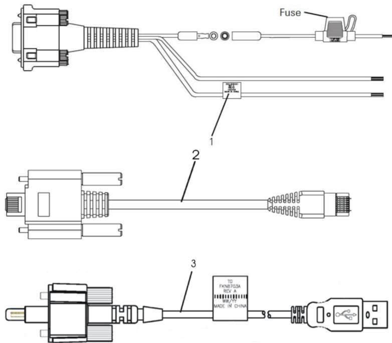
Figure 9 Available Cables
