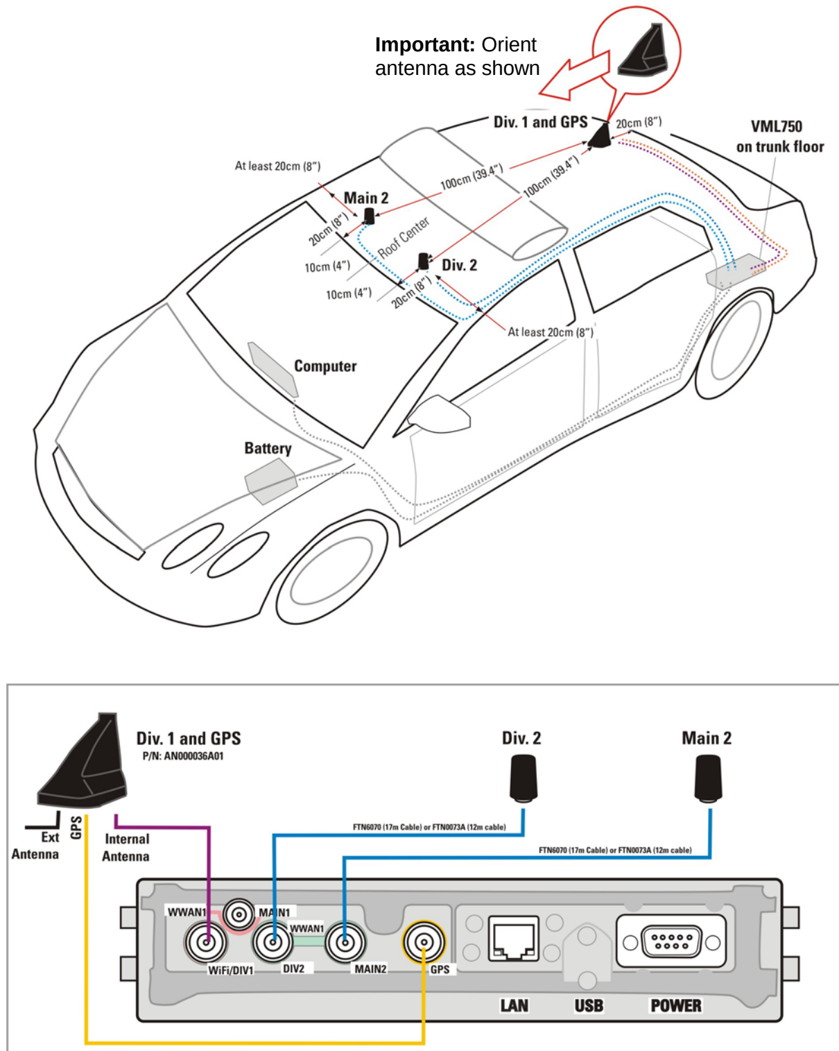
Figure 7 Schematic Installation Diagram for Sub-models WWAN2 Only FLN1057A/FLN2057A/FLN5057A/FLN5058A
