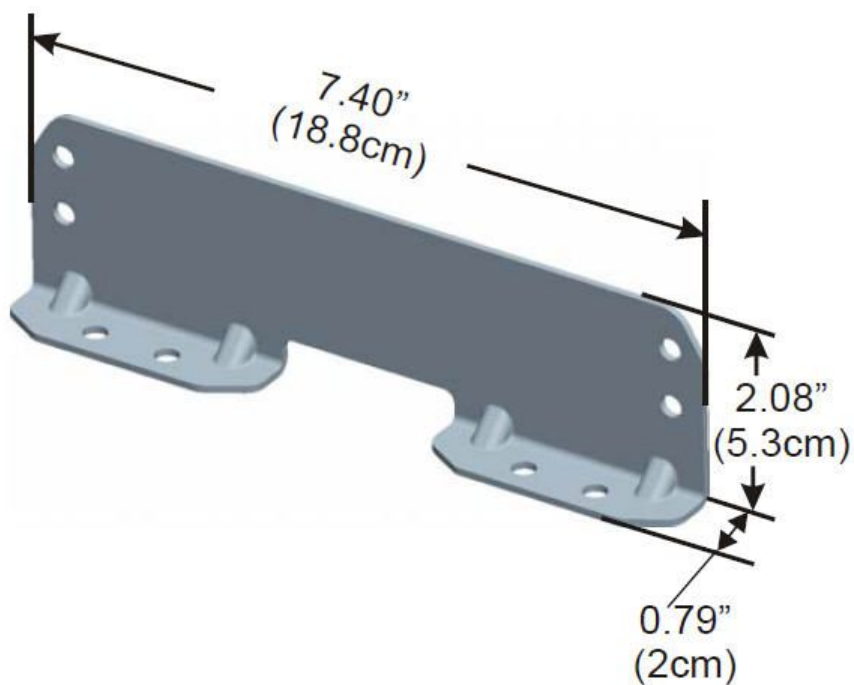
Figure 2-9 Bracket Dimensions
