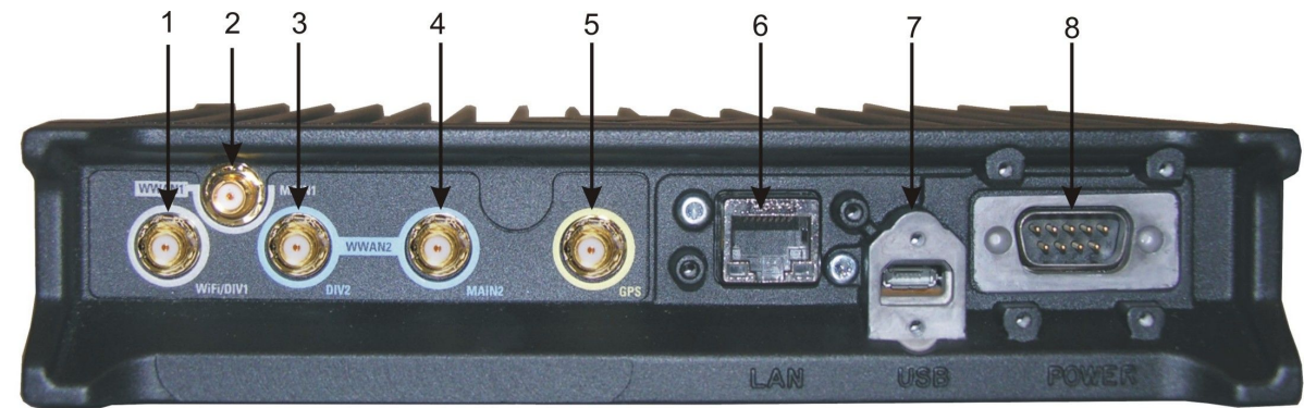
Figure 1-2 Connector Panel
