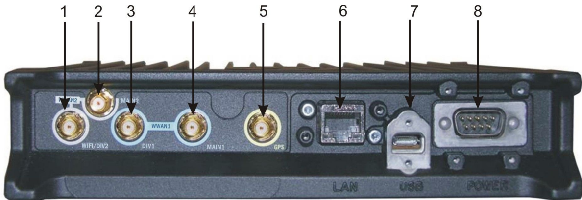
Figure 1-3 Connector Panel
