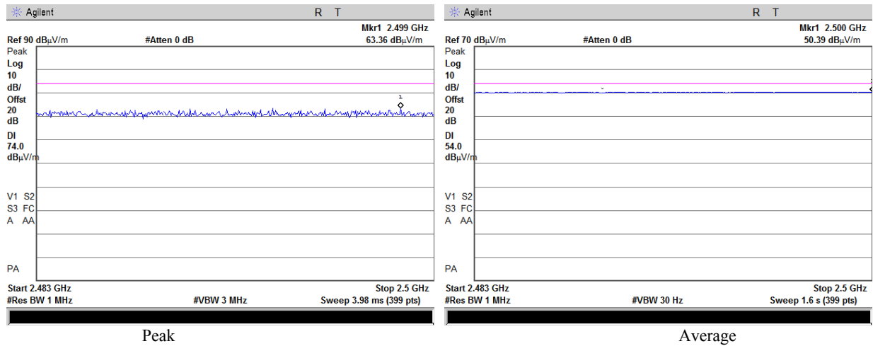
Plot 4.5.12 Radiated Spurious Emission, 802.11n 20MHz, Fc = 2462 MHz, MCS7, Vertical
