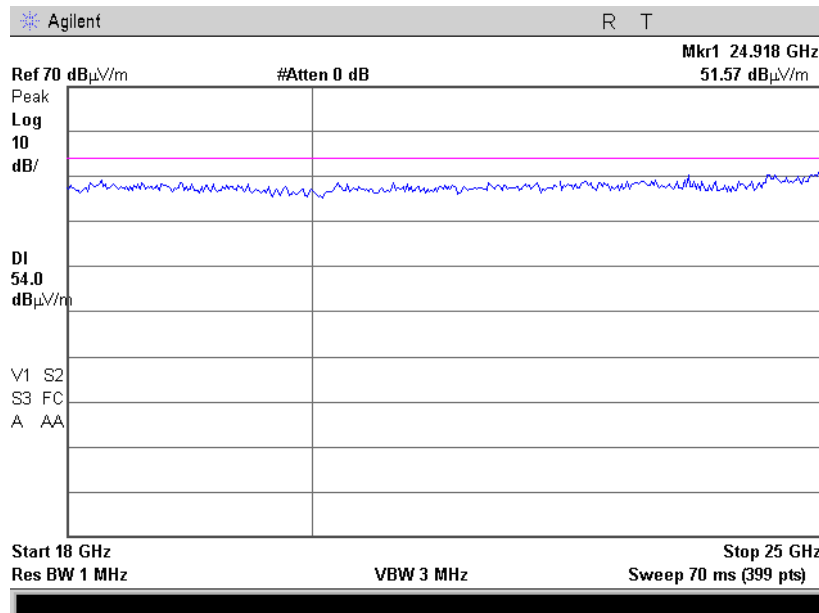
Plot 4.6.26 Radiated Spurious Emission in 18-25GHz range, 802.11n 20MHz, Fc = 2437 MHz, MCS7, Horizontal & Vertical, Peak
