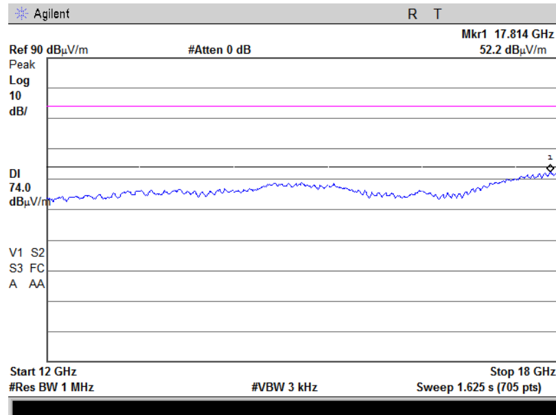
Plot 4.6.25 Radiated Spurious Emission in 12-18GHz range, 802.11n 20MHz, Fc = 2437 MHz, MCS7, Horizontal & Vertical, Average
