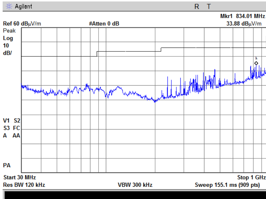
Plot 4.6.1 Radiated Spurious Emission in 30MHz-1GHz range, Worst case for all modes and all frequencies, Horizontal
