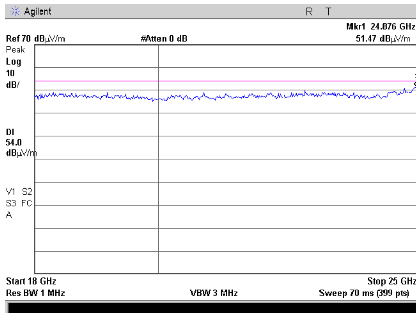
Plot 4.6.14 Radiated Spurious Emission in 18-25GHz range, 802.11g, Fc = 2412 MHz, 54Mbps, Horizontal & Vertical, Peak
