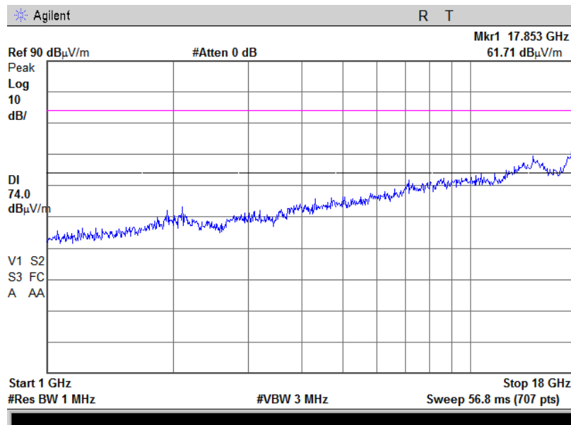
Plot 4.6.6 Radiated Spurious Emission in 1-18GHz range, 802.11b, Fc = 2437 MHz, 11Mbps, Horizontal & Vertical, Peak
