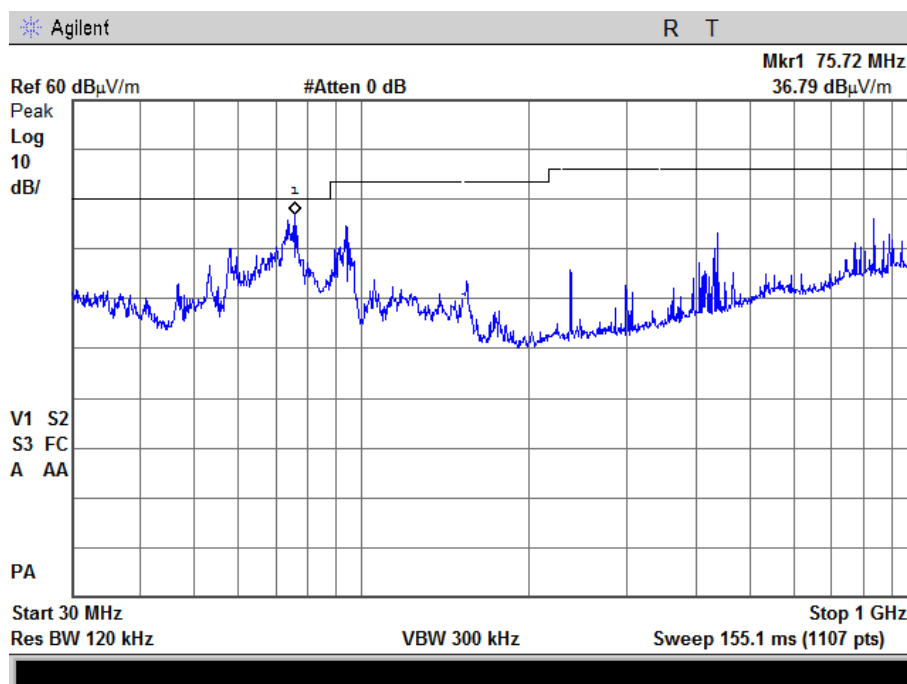
Plot 4.6.2 Radiated Spurious Emission in 30MHz-1GHz range, Worst case for all modes and all frequencies, Vertical
