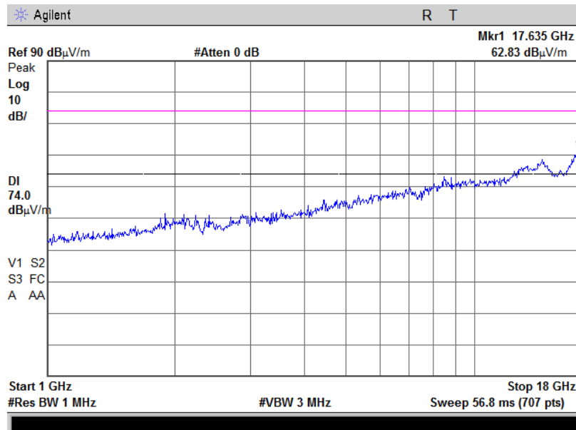
Plot 4.6.12 Radiated Spurious Emission in 1-18GHz range, 802.11g, Fc = 2412 MHz, 54Mbps, Horizontal & Vertical, Peak
