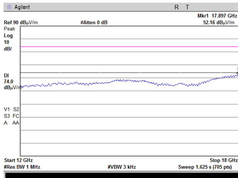
Plot 4.6.28 Radiated Spurious Emission in 12-18GHz range, 802.11n 20MHz, Fc = 2462 MHz, MCS7, Horizontal & Vertical, Average
