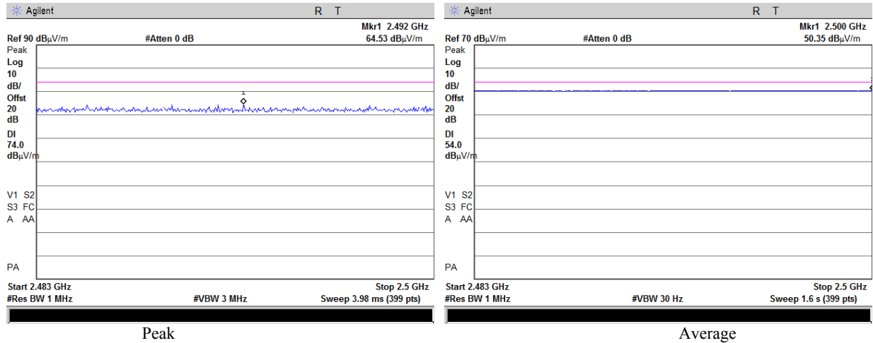
Plot 4.5.3 Radiated Spurious Emission, 802.11b, Fc = 2462 MHz, 11Mbps, Horizontal
