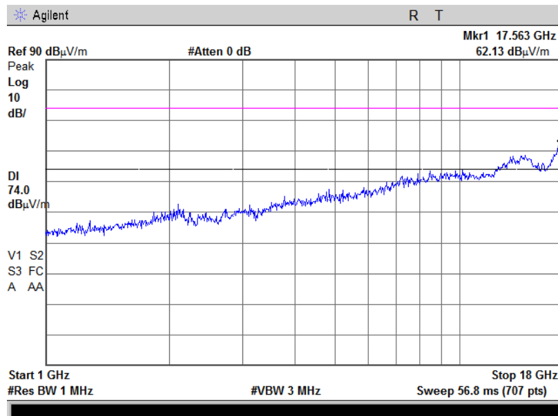
Plot 4.6.18 Radiated Spurious Emission in 1-18GHz range, 802.11g, Fc = 2462 MHz, 54Mbps, Horizontal & Vertical, Peak
