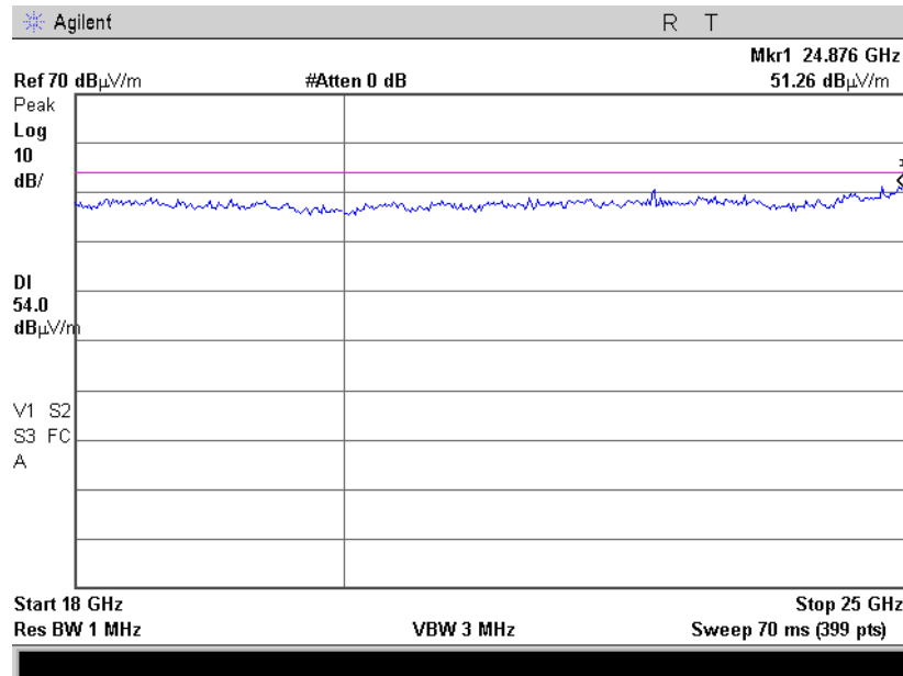
Plot 4.6.17 Radiated Spurious Emission in 18-25GHz range, 802.11g, Fc = 2437 MHz, 54Mbps, Horizontal & Vertical, Peak
