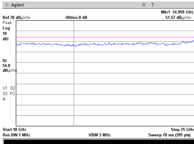
Plot 4.6.8 Radiated Spurious Emission in 18-25GHz range, 802.11b, Fc = 2437 MHz, 11Mbps, Horizontal & Vertical, Peak
