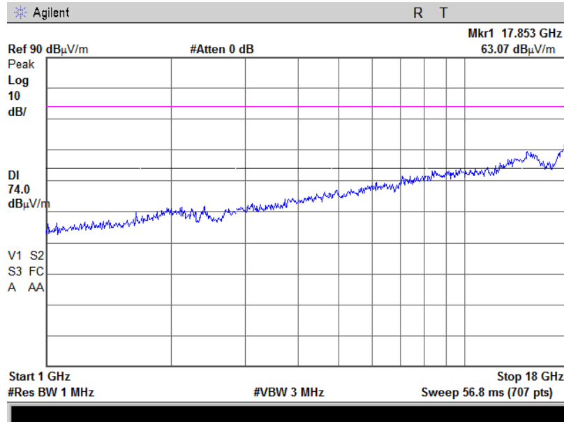
Plot 4.6.21 Radiated Spurious Emission in 1-18GHz range, 802.11n 20MHz, Fc = 2412 MHz, MCS7, Horizontal & Vertical, Peak
