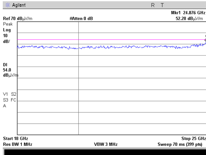
Plot 4.6.11 Radiated Spurious Emission in 18-25GHz range, 802.11b, Fc = 2462 MHz, 11Mbps, Horizontal & Vertical, Peak
