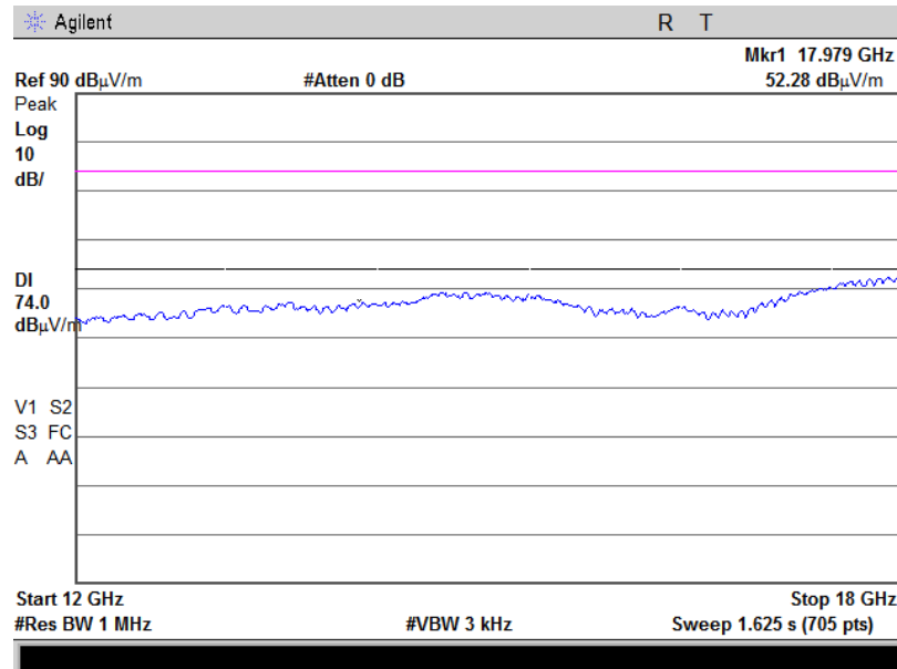
Plot 4.6.19 Radiated Spurious Emission in 12-18GHz range, 802.11g, Fc = 2462 MHz, 54Mbps, Horizontal & Vertical, Average
