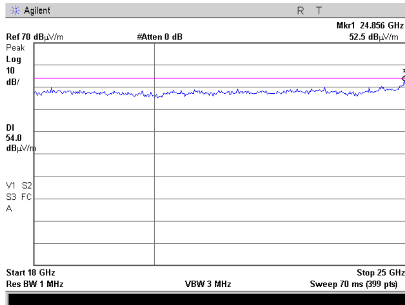
Plot 4.6.5 Radiated Spurious Emission in 18-25GHz range, 802.11b, Fc = 2412 MHz, 11Mbps, Horizontal & Vertical, Peak
