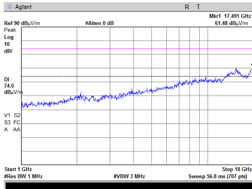
Plot 4.6.3 Radiated Spurious Emission in 1-18GHz range, 802.11b, Fc = 2412 MHz, 11Mbps, Horizontal & Vertical, Peak
