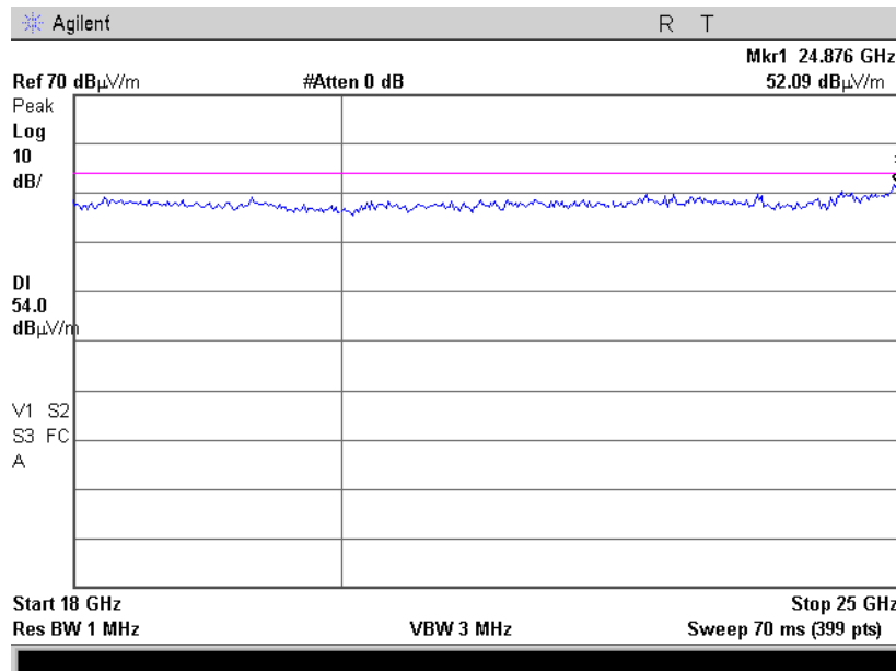
Plot 4.6.20 Radiated Spurious Emission in 18-25GHz range, 802.11g, Fc = 2462 MHz, 54Mbps, Horizontal & Vertical, Peak
