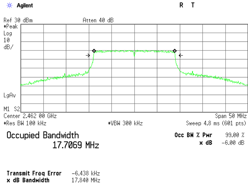
Plot 4.1.9 6dB bandwidth test results, 802.11n 20MHz Mode, Fc = 2462 MHz
