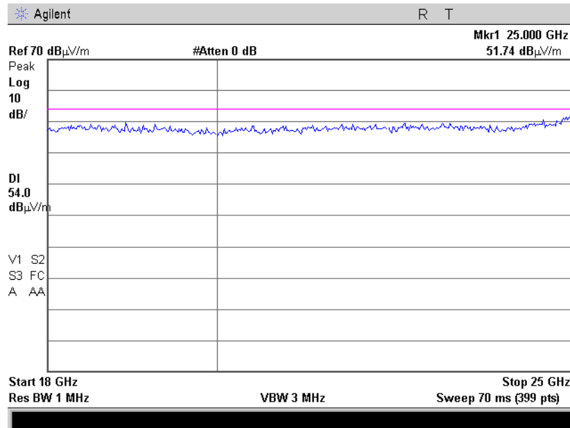
Plot 4.6.23 Radiated Spurious Emission in 18-25GHz range, 802.11n 20MHz, Fc = 2412 MHz, MCS7, Horizontal & Vertical, Peak
