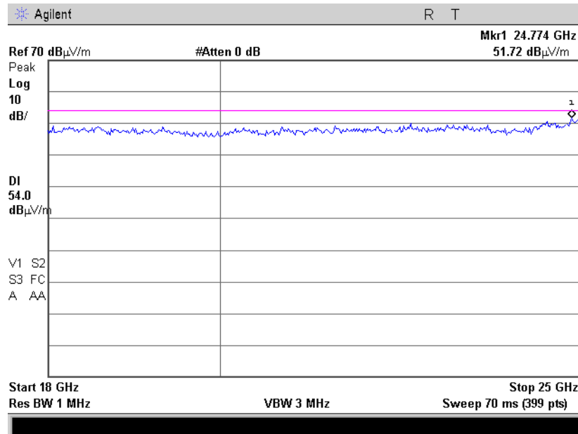
Plot 4.6.29 Radiated Spurious Emission in 18-25GHz range, 802.11n 20MHz, Fc = 2462 MHz, MCS7, Horizontal & Vertical, Peak
