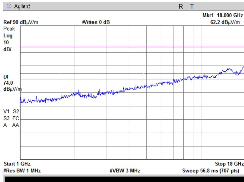
Plot 4.6.24 Radiated Spurious Emission in 1-18GHz range, 802.11n 20MHz, Fc = 2437 MHz, MCS7, Horizontal & Vertical, Peak
