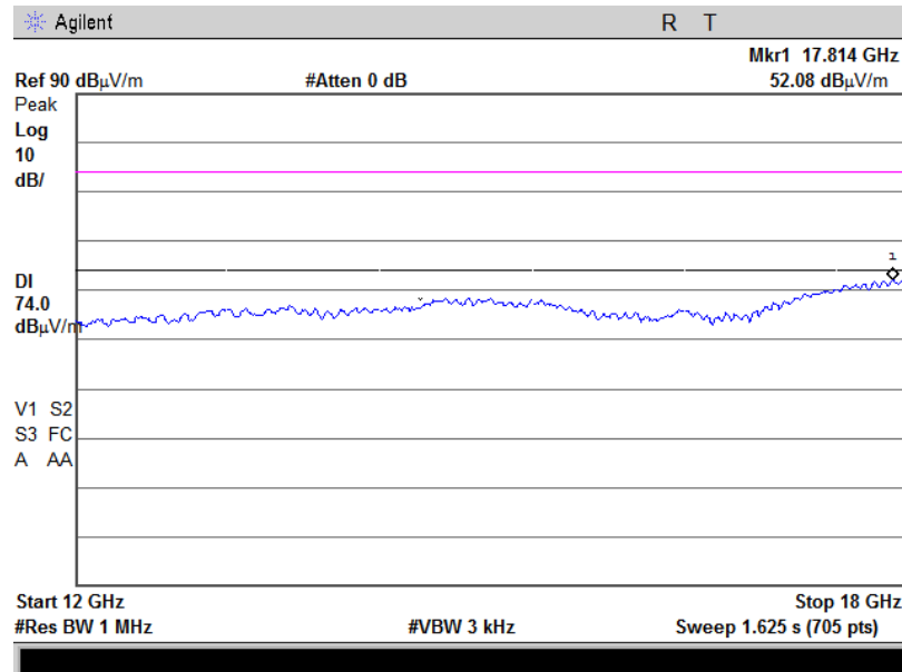
Plot 4.6.13 Radiated Spurious Emission in 12-18GHz range, 802.11g, Fc = 2412 MHz, 54Mbps, Horizontal & Vertical, Average
