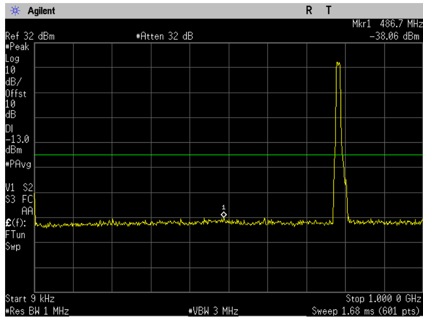
782 MHz 16 QAM - RB size 50, RB Offset 0 Plot 4.3.15
