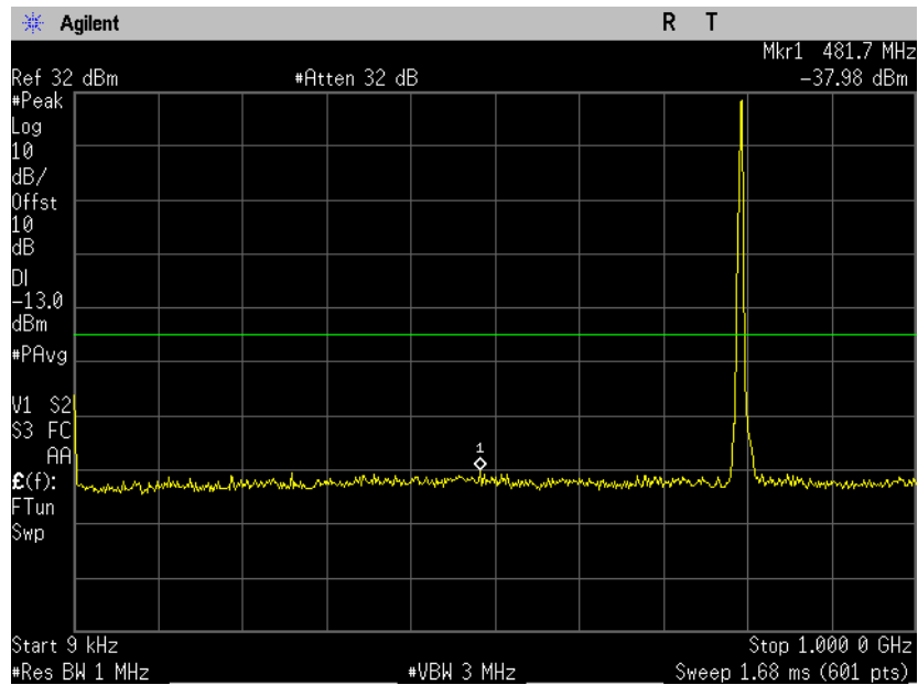
790.5 MHz QPSK - RB size 1, RB Offset 24 Plot 4.6.3
