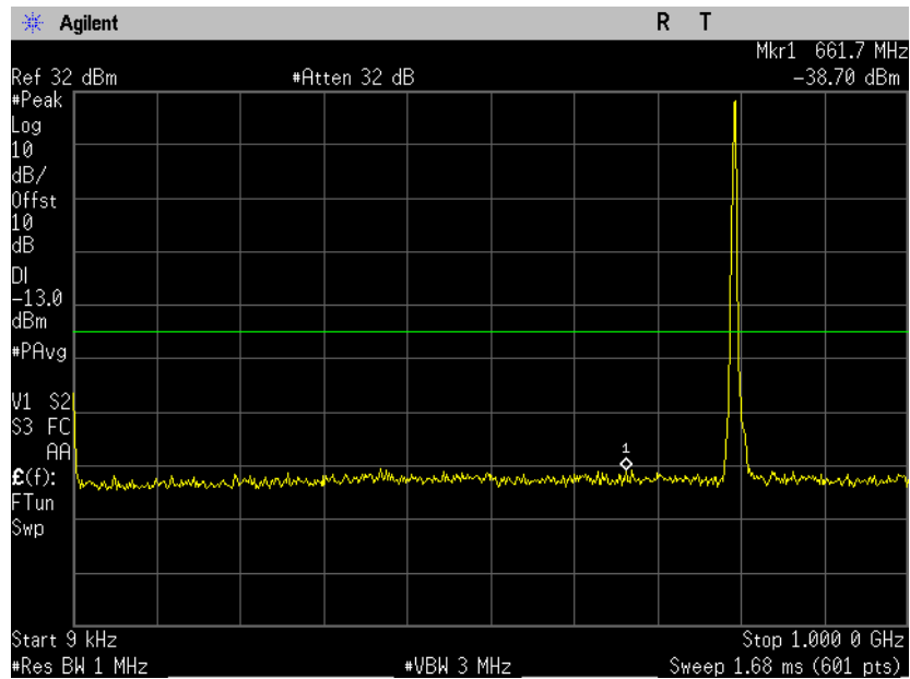
790.5 MHz 16 QAM - RB size 1, RB Offset 24 Plot 4.6.11
