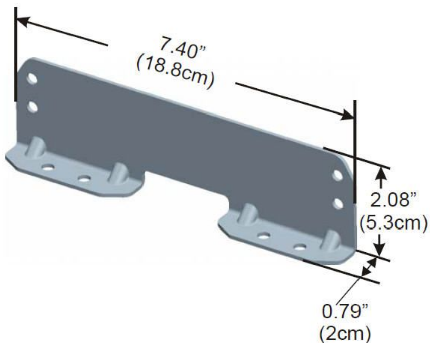
Figure 2-8 Bracket Dimensions
