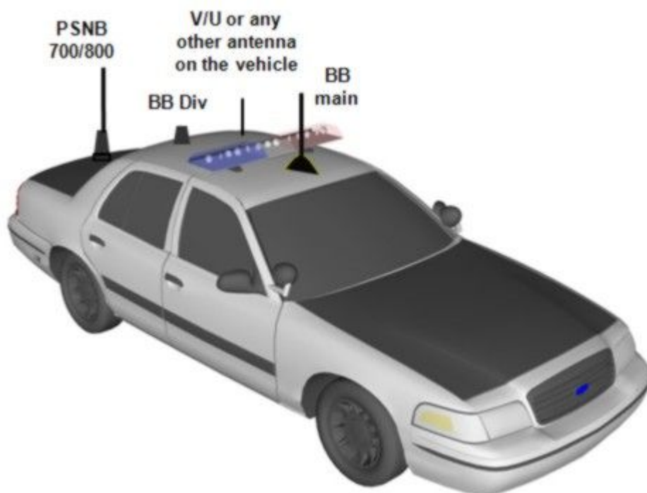
Figure C-1 Police Patrol Vehicle — Antennas Location Suggestion
