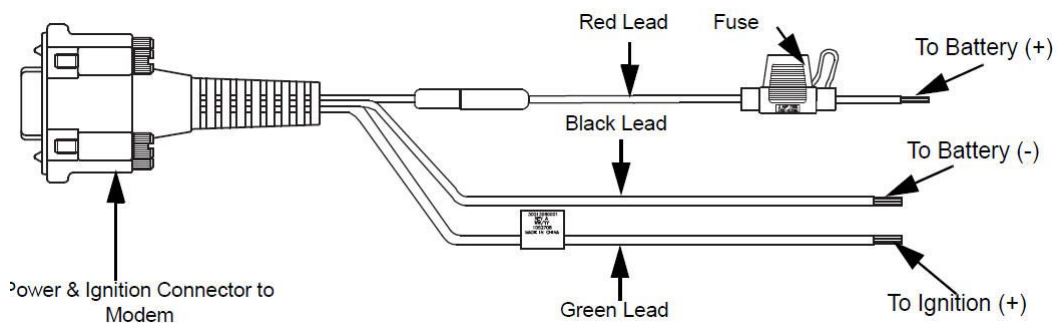
Figure 2-10 DC Power and Ignition Cable Routing Into Engine Compartment
