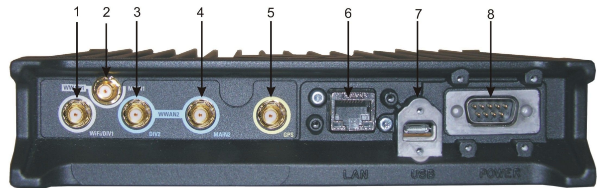
Figure 1-2 Connector Panel
