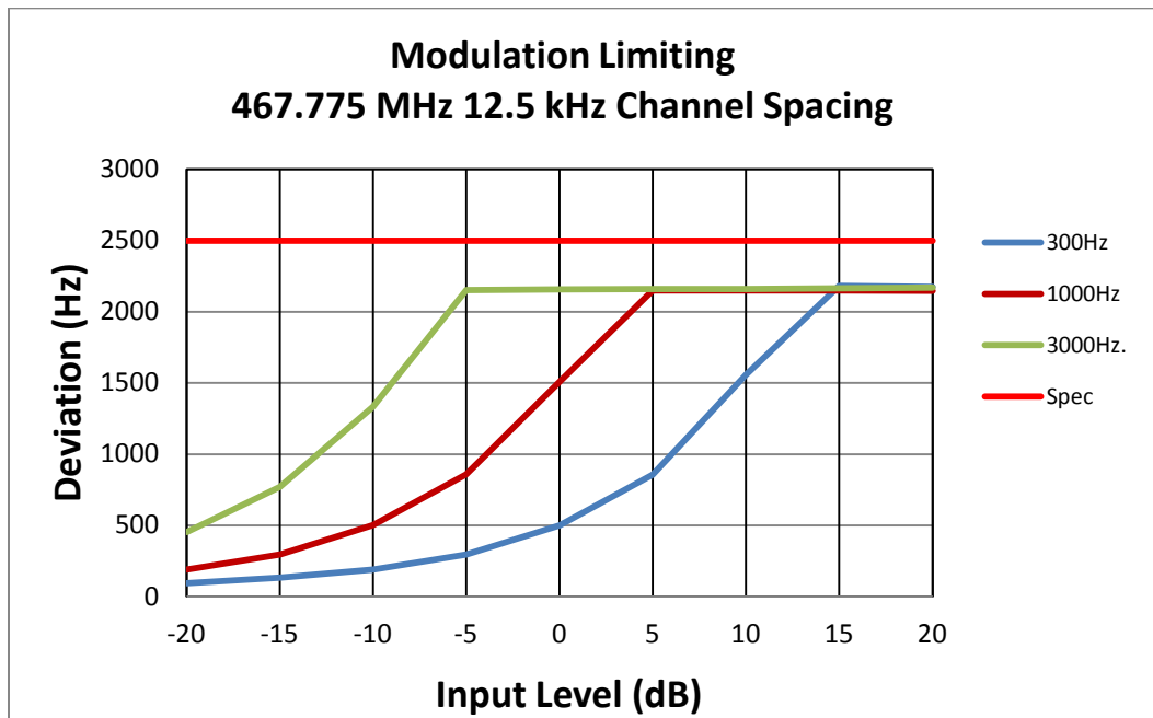
Figure 6D-1: 467.775 MHz, 12.5 KHz Channel Spacing, Modulation Limiting
