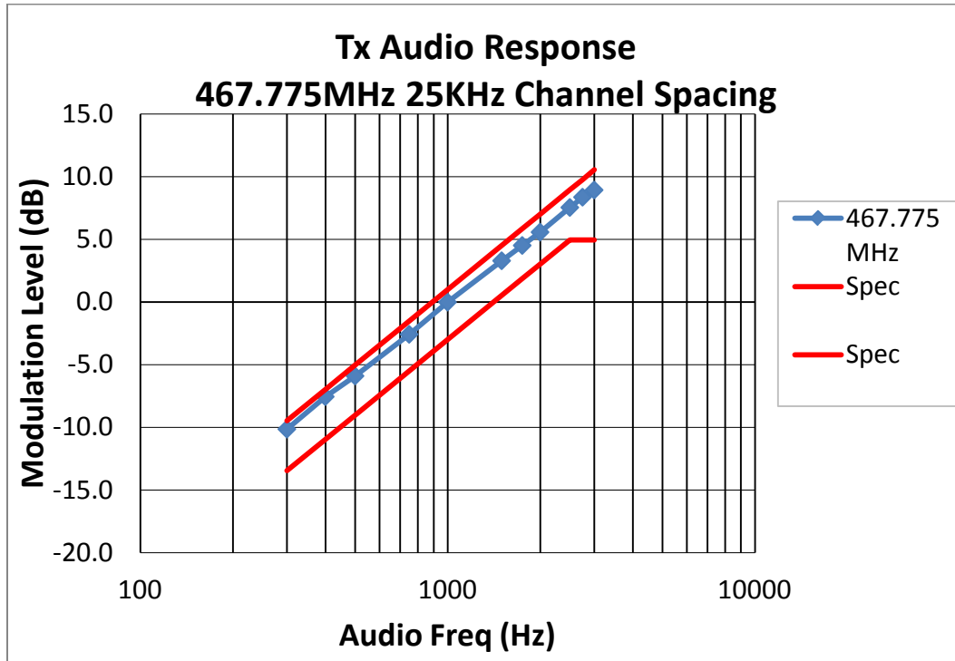
Figure 6B-2: 467.775 MHz, 25 kHz Channel Spacing, Transmit Audio Frequency Response
