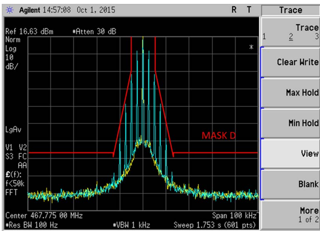
Figure 6E-10: 467.775 MHz, 12.5 kHz Channel Spacing, 2500Hz Audio Modulation only, 11K0F3E Mask D
