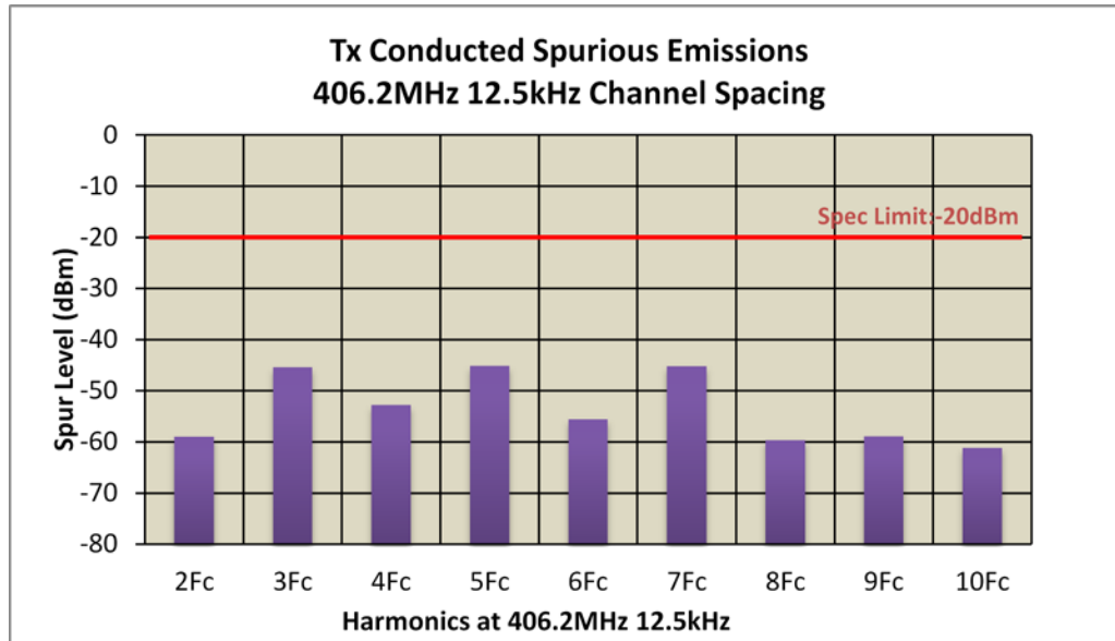
Figure 6F-1: 48 W Harmonic of Carrier 406.2 MHz, Digital 12.5 kHz Channel Spacing
