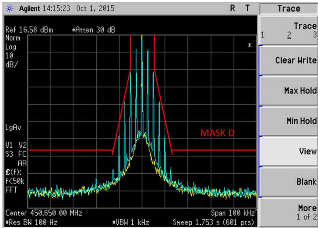
Figure 6E-5: 450.65 MHz, 12.5 kHz Channel Spacing, 2500Hz Audio Modulation only, 11K0F3E Mask D
