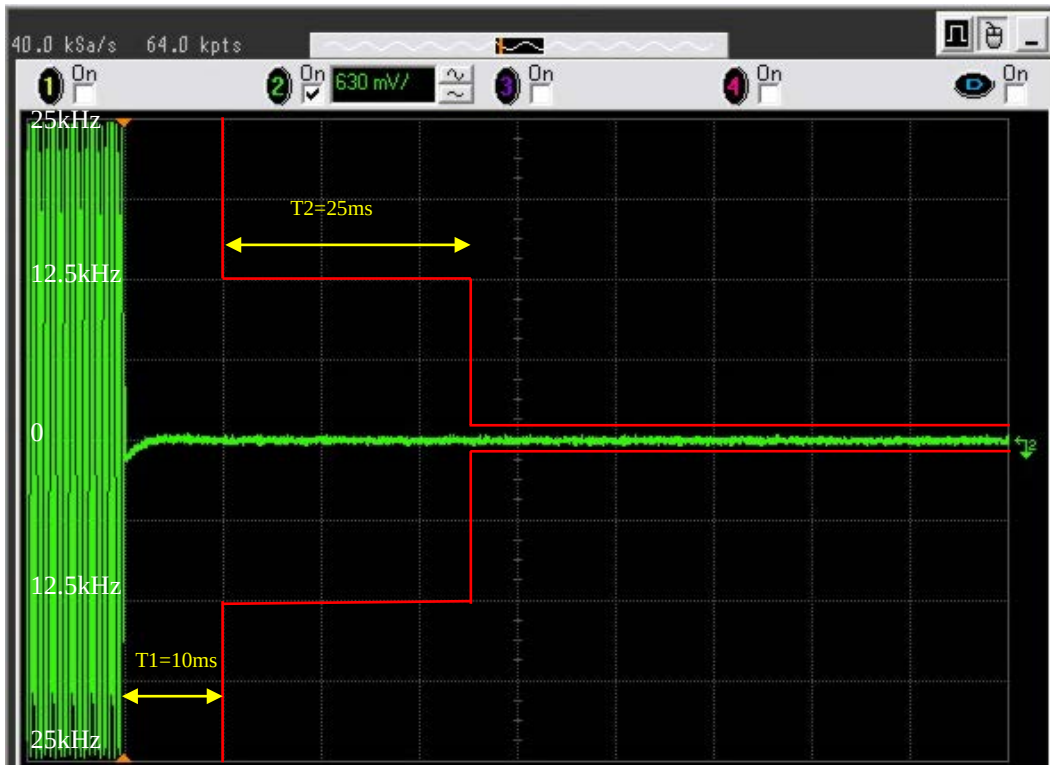
6I-3 – 467.775 MHz, 25 kHz Channel Spacing Key-Up Attack Time
