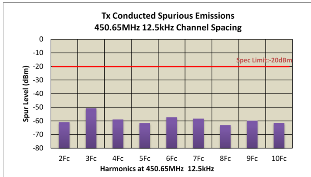
Figure 6F-5: 25W Harmonic of Carrier 450.65 MHz, Digital 12.5 kHz Channel Spacing
