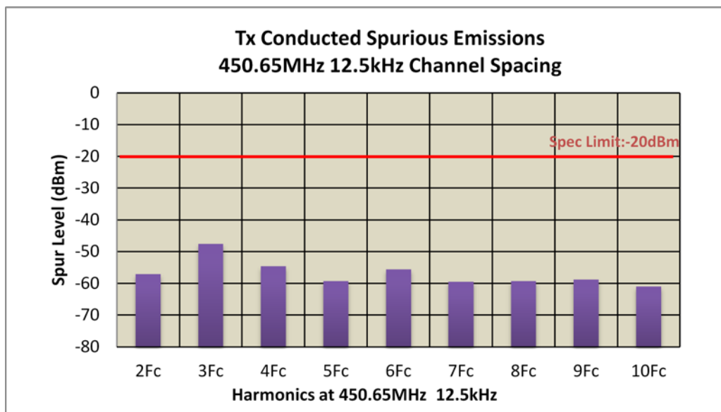
Figure 6F-2: 48 W Harmonic of Carrier 450.65 MHz, Digital 12.5 kHz Channel Spacing
