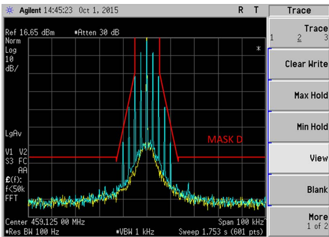
Figure 6E-9: 459.125 MHz, 12.5 kHz Channel Spacing, 2500Hz Audio Modulation only, 11K0F3E Mask D
