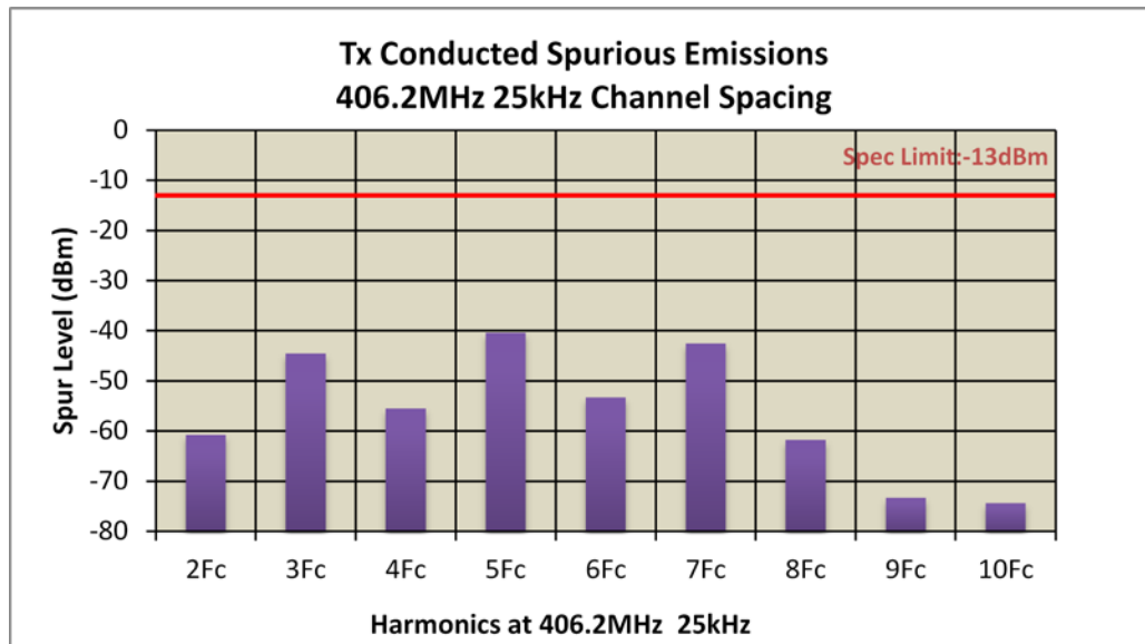
Figure 6F-7: 48 W Harmonic of Carrier 406.2 MHz, Analog 25 kHz Channel Spacing (Not for FCC Review)
