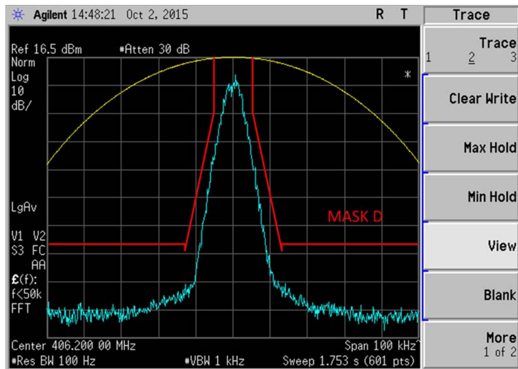
Figure 6E-2: 406.2 MHz, O.153 Test Pattern 4FSK Voice and Data Modulation, 7K60F1W Mask D
