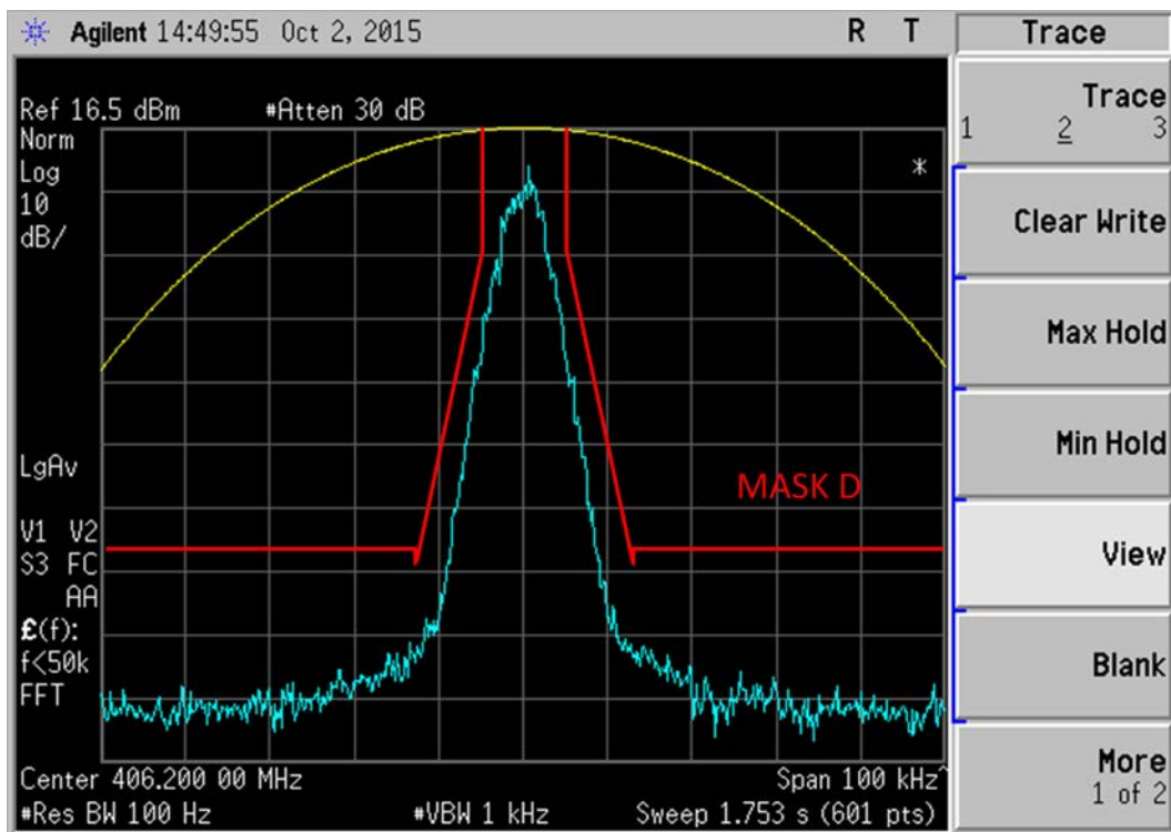
Figure 6E-4: 406.2 MHz, O.153 Test Pattern 4FSK Voice Modulation only, 7K60F1E Mask D
