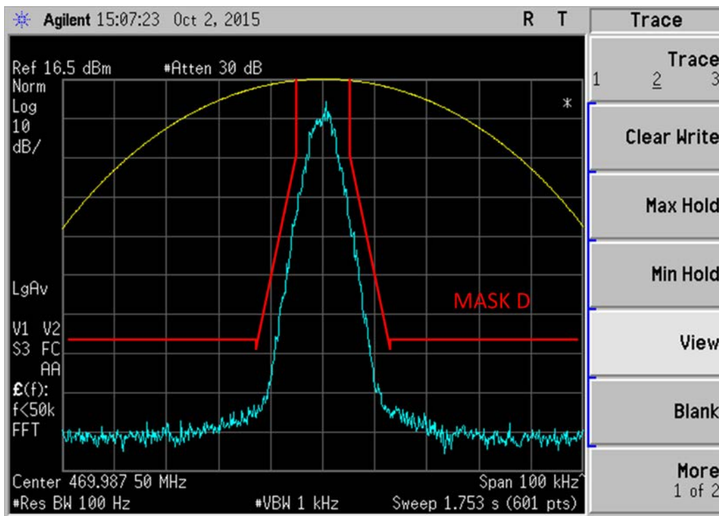
Figure 6E-14: 469.9875 MHz, O.153 Test Pattern 4FSK Voice Modulation only, 7K60F1E Mask D
