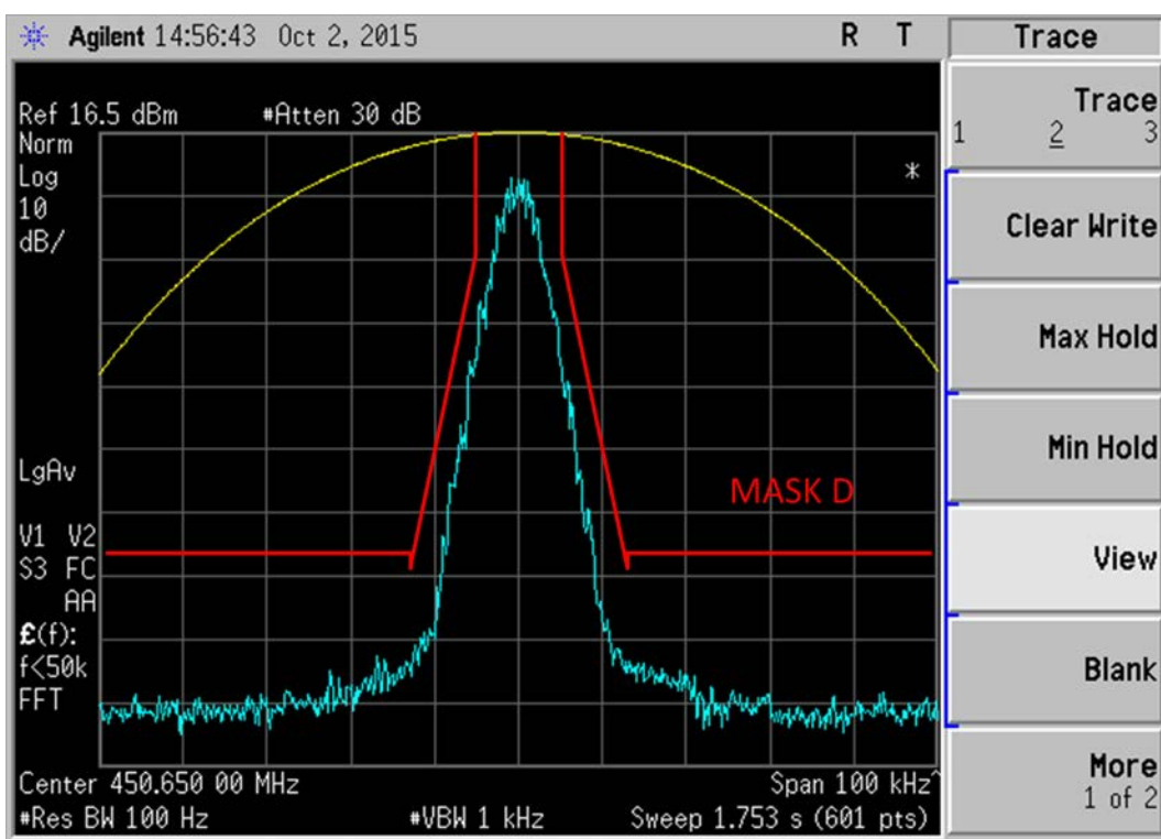
Figure 6E-7: 450.65 MHz, O.153 Test Pattern 4FSK Data Modulation only, 7K60F1D Mask D
