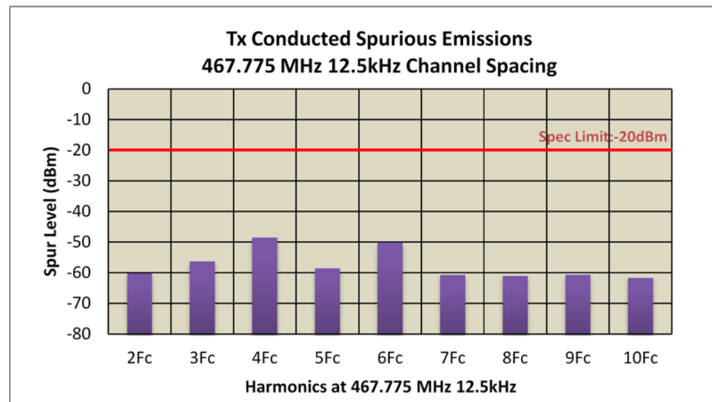
Figure 6F-6: 25W Harmonic of Carrier 467.775 MHz, Digital 12.5 kHz Channel Spacing
