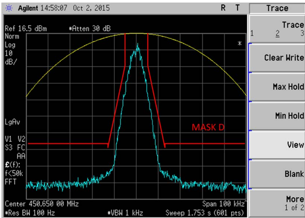
Figure 6E-6: 450.65 MHz, O.153 Test Pattern 4FSK Voice and Data Modulation, 7K60F1W Mask D
