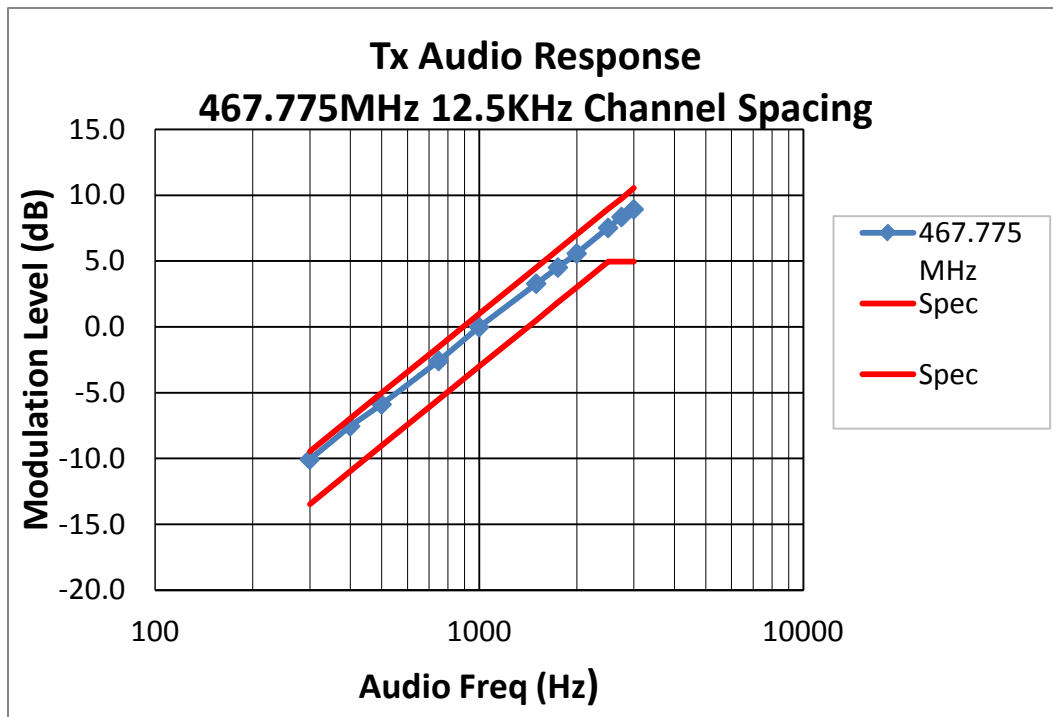
Figure 6B-1: 467.775 MHz, 12.5 kHz Channel Spacing, Transmit Audio Frequency Response
