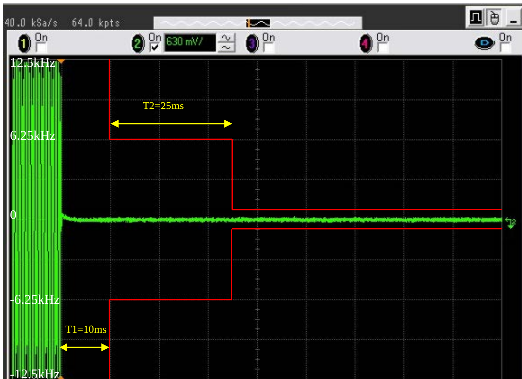
6I-1 – 467.775 MHz, 12.5 kHz Channel Spacing Key-Up Attack Time
