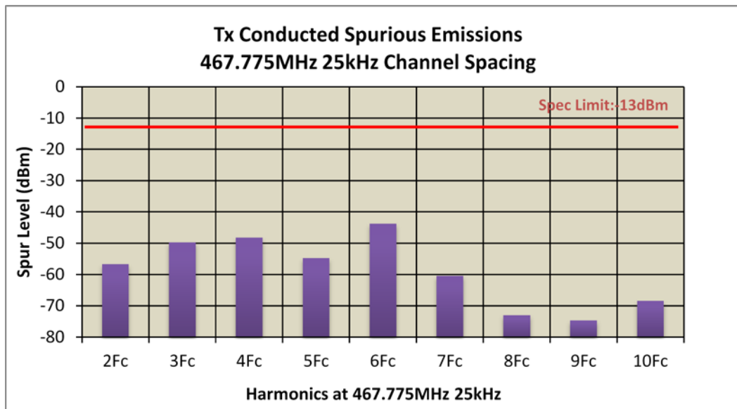
Figure 6F-10: 48 W Harmonic of Carrier 467.775 MHz, Analog 25 kHz Channel Spacing
