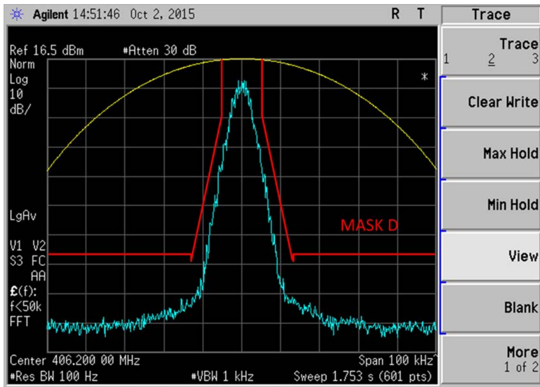
Figure 6E-3: 406.2 MHz, O.153 Test Pattern 4FSK Data Modulation only, 7K60F1D Mask D
