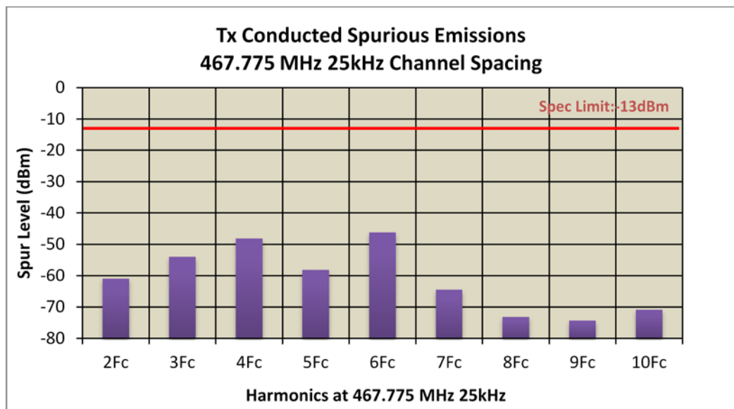
Figure 6F-12: 25W Harmonic of Carrier 467.775 MHz, Analog 25 kHz Channel Spacing
