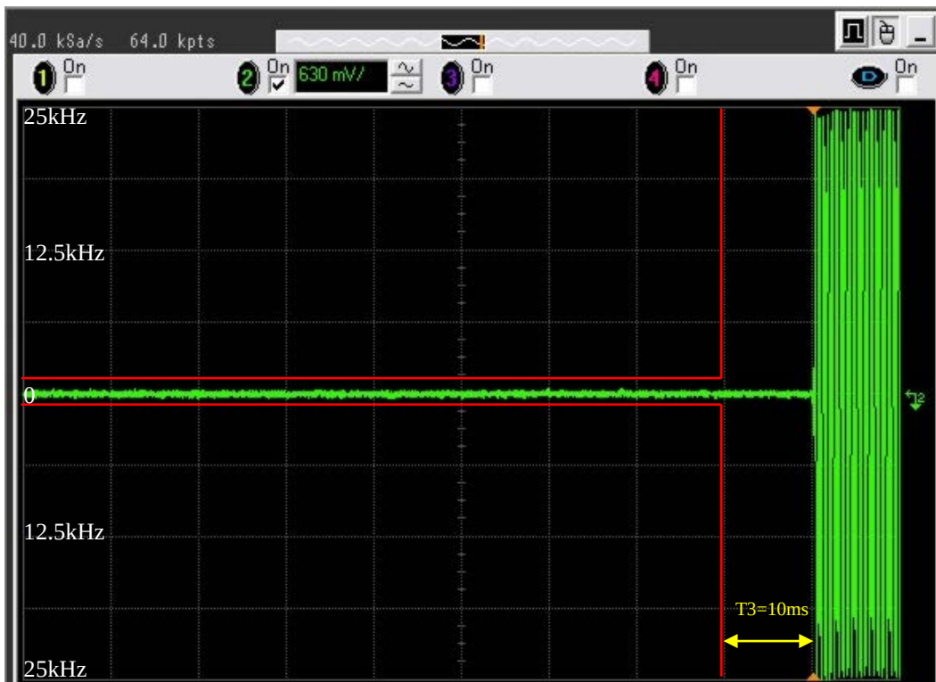
6I-4 – 467.775 MHz, 25 kHz Channel Spacing De-Key Decay Time
