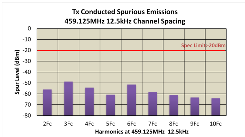
Figure 6F-3: 48 W Harmonic of Carrier 459.125 MHz, Digital 12.5 kHz Channel Spacing
