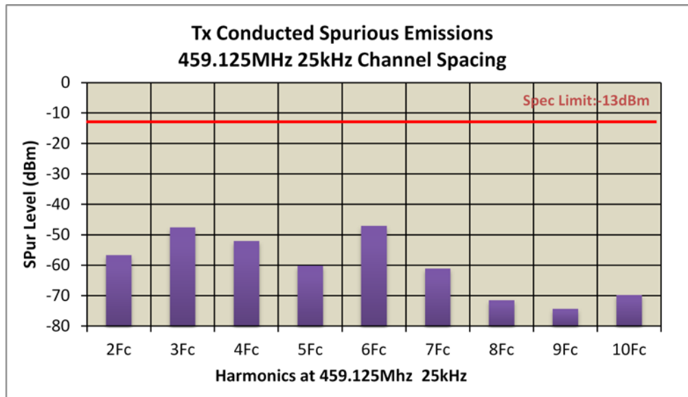
Figure 6F-9: 48 W Harmonic of Carrier 459.125 MHz, Analog 25 kHz Channel Spacing
