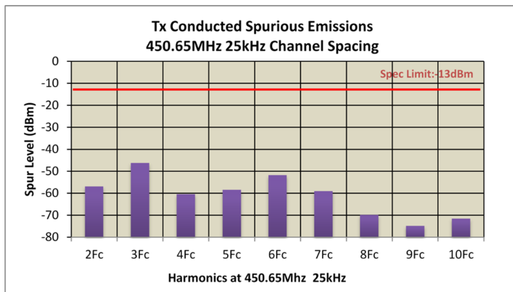
Figure 6F-8: 48 W Harmonic of Carrier 450.65 MHz, Analog 25 kHz Channel Spacing
