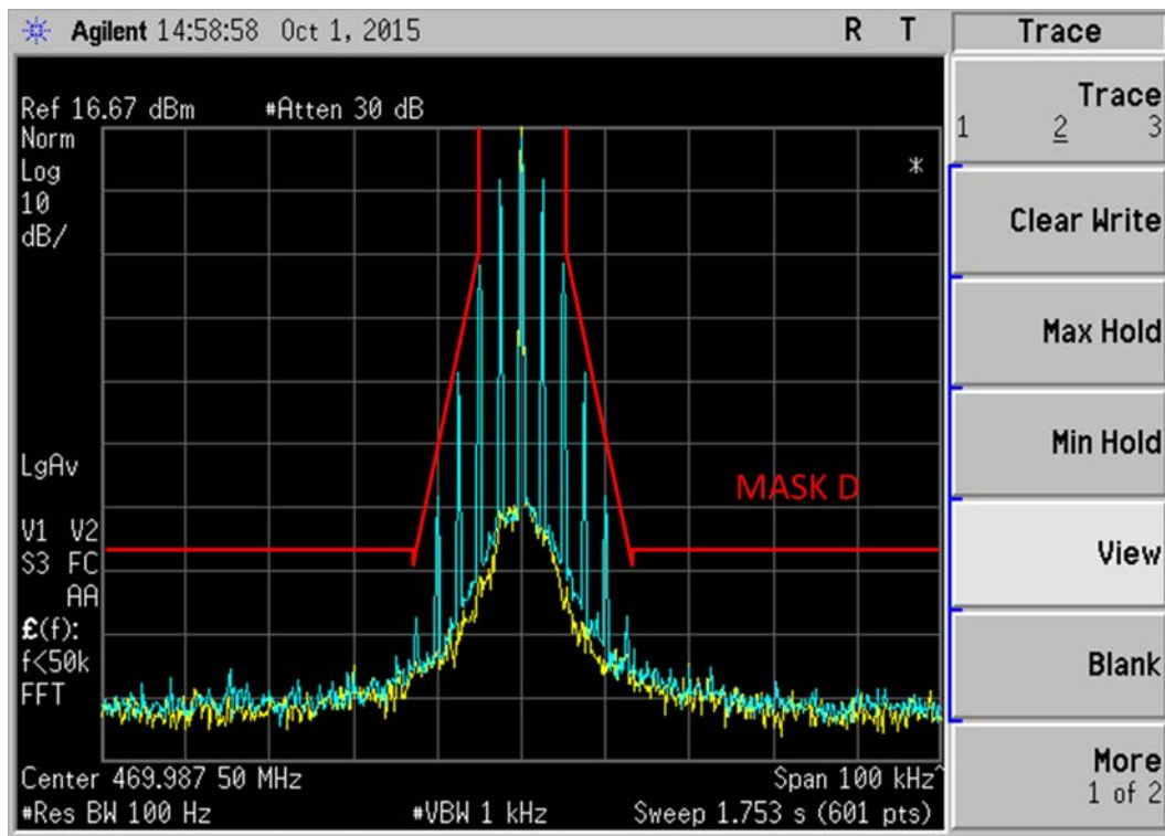
Figure 6E-11: 469.9875 MHz, 12.5 kHz Channel Spacing, 2500Hz Audio Modulation only, 11K0F3E Mask D
