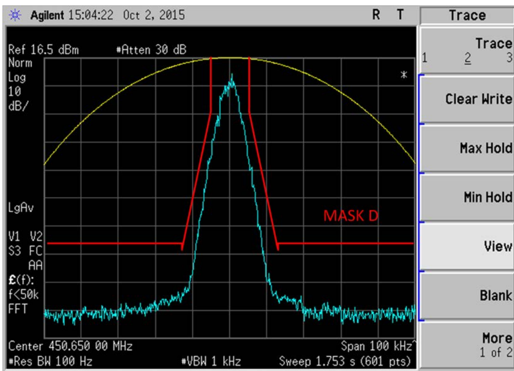
Figure 6E-8: 450.65 MHz, O.153 Test Pattern 4FSK Voice Modulation only, 7K60F1E Mask D
