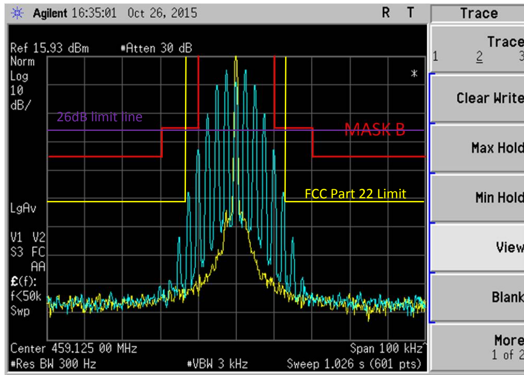
Figure 6E-17: 459.125 MHz, 25 kHz Channel Spacing, 2500Hz Audio Modulation only, 16K0F3E Mask B, Part 22 FCC Limit
