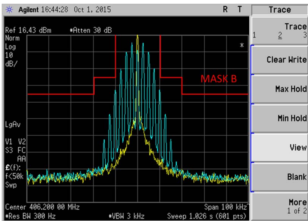
Figure 6E-15: 406.2 MHz, 25 kHz Channel Spacing, 2500Hz Audio Modulation only, 16K0F3E Mask B (Not for FCC Review)
