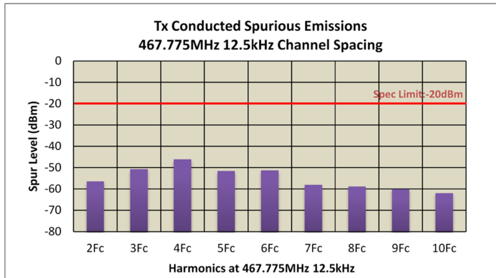
Figure 6F-4: 48 W Harmonic of Carrier 467.775 MHz, Digital 12.5 kHz Channel Spacing
