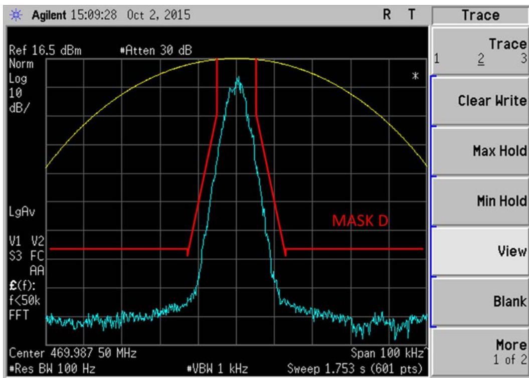
Figure 6E-12: 469.9875 MHz, 0.153 Test Pattern 4FSK Voice and Data Modulation, 7K60F1W Mask D
