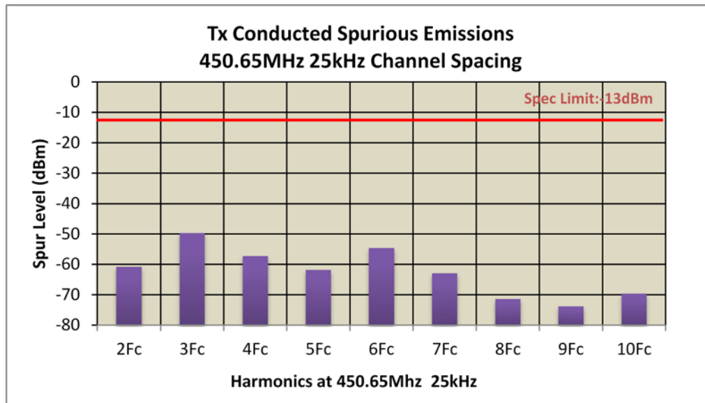
Figure 6F-11: 25W Harmonic of Carrier 450.65 MHz, Analog 25 kHz Channel Spacing
