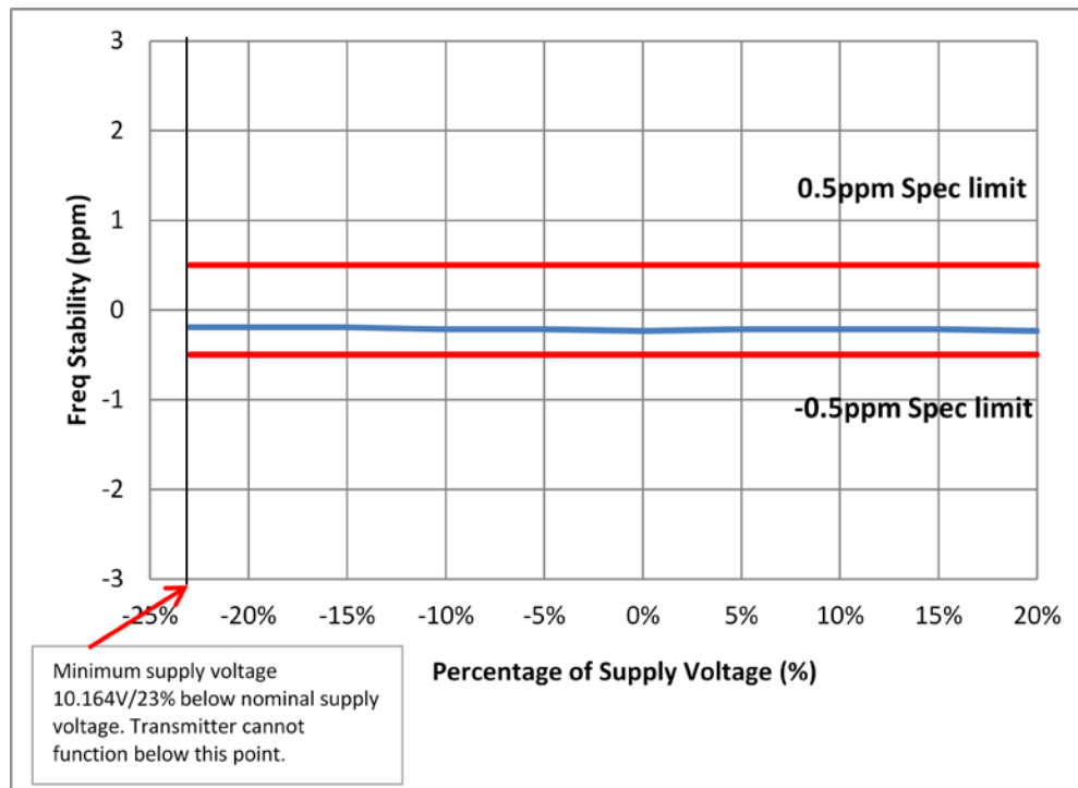
6H-2 – 467.775 MHz Frequency Stability vs. Supply Voltage
