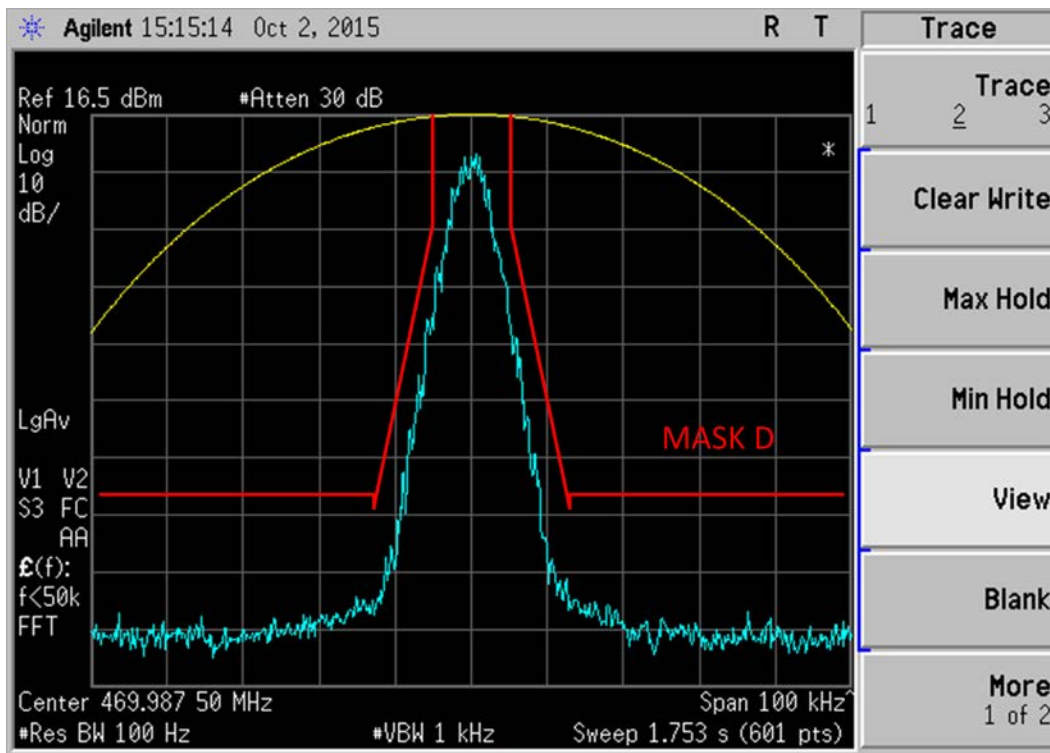
Figure 6E-13: 469.9875 MHz, O.153 Test Pattern 4FSK Data Modulation only, 7K60F1D Mask D
