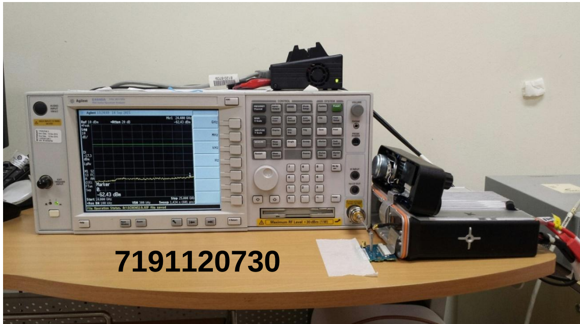
Peak Power Spectral Density Test Setup
