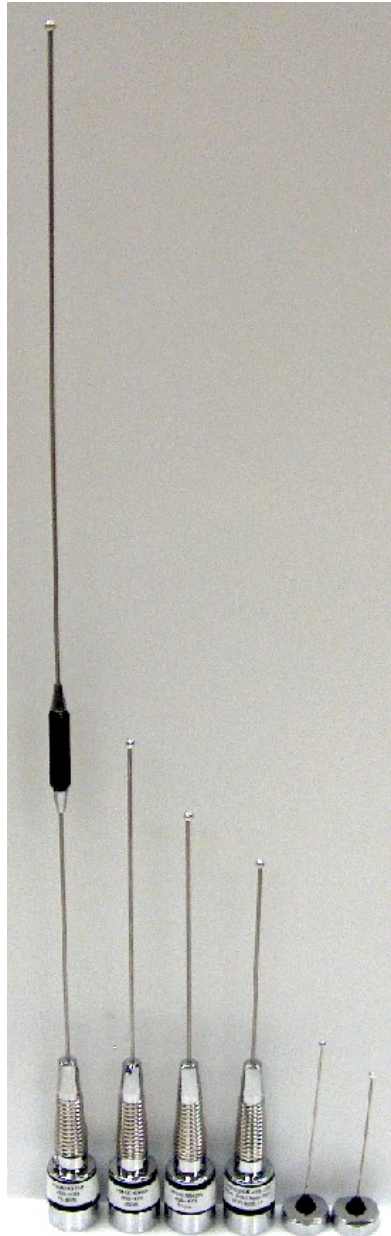
UHF Antenna kit numbers, from left to right: PMAE4043A, PMAE4040A, PMAE4042A, HAE6029A, PMAE4039A & PMAE4041A
