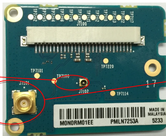
GPS/BT/Wifi board (Top)
