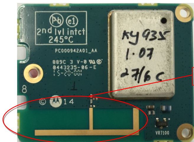
GPS/BT/Wifi board with shield (Bottom)
